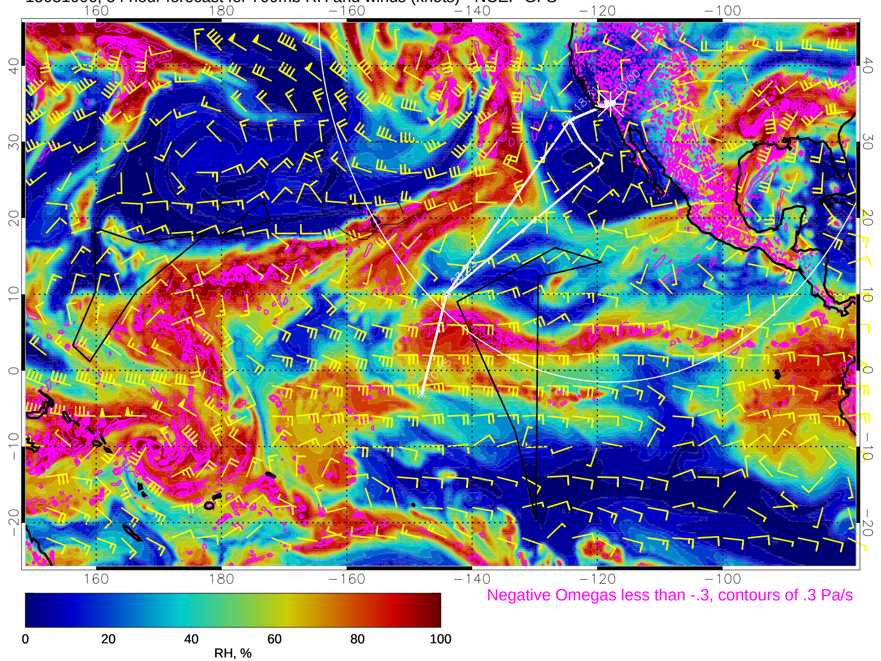
15031006, 54 hour forecast for 700mb RH and winds (knots) - NCEP GFS
