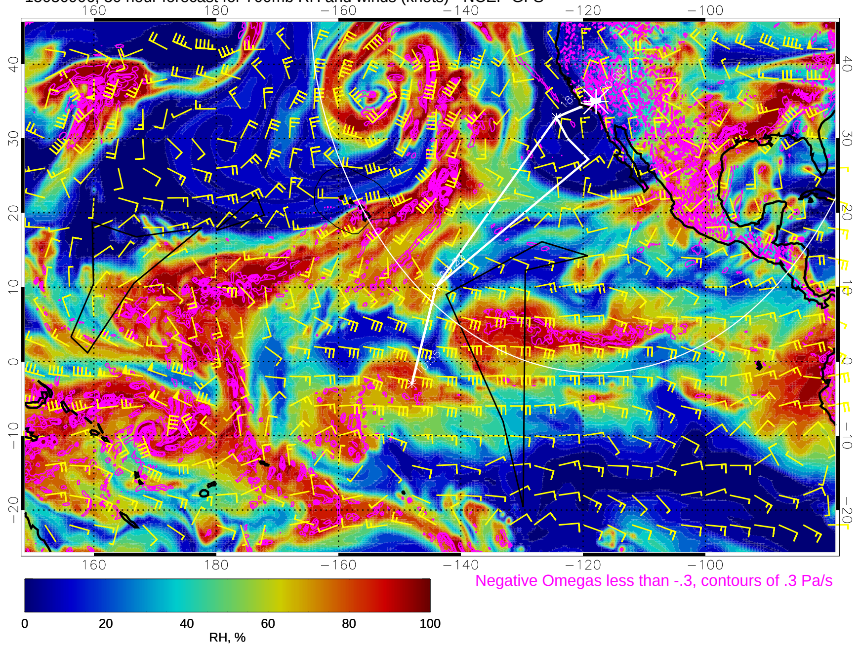
15030906, 30 hour forecast for 700mb RH and winds (knots) - NCEP GFS
