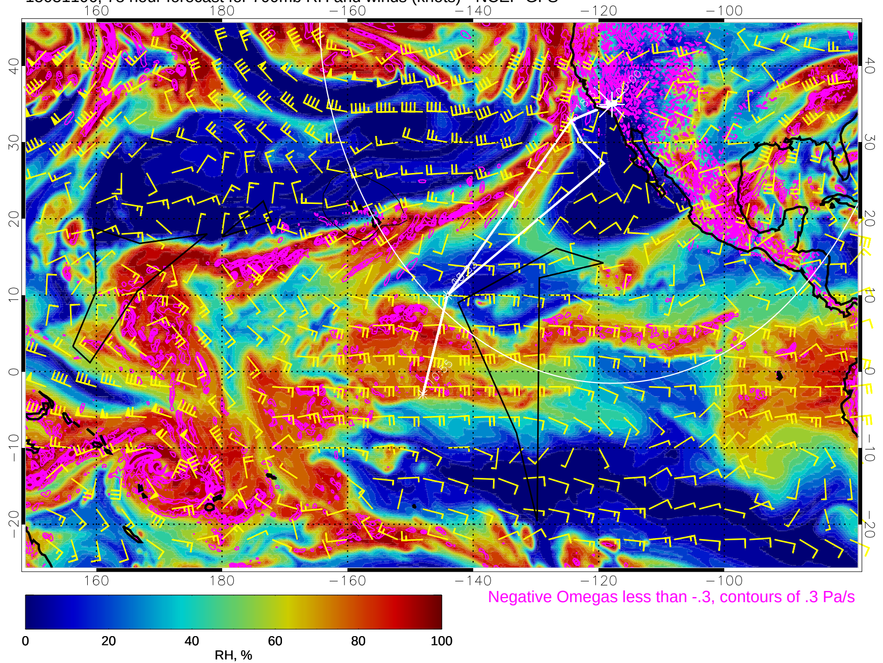
15031106, 78 hour forecast for 700mb RH and winds (knots) - NCEP GFS
