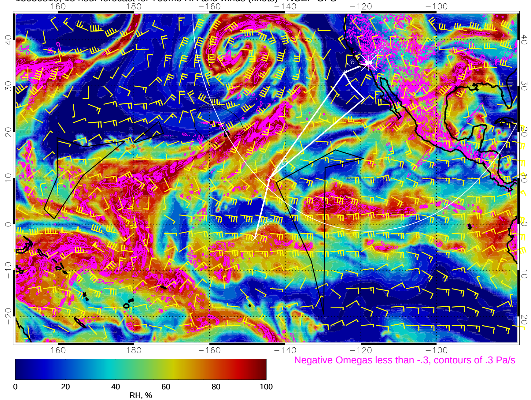
15030818, 18 hour forecast for 700mb RH and winds (knots) - NCEP GFS
