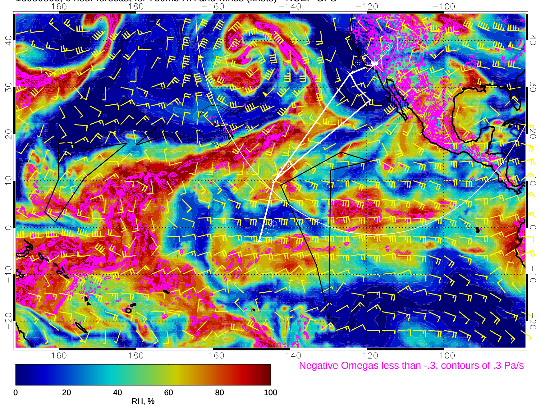
15030806, 6 hour forecast for 700mb RH and winds (knots) - NCEP GFS
