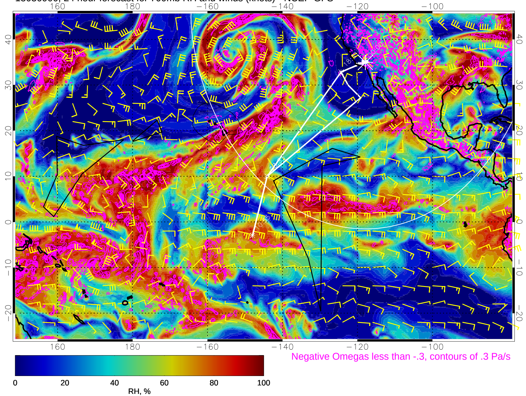
15030900, 24 hour forecast for 700mb RH and winds (knots) - NCEP GFS
