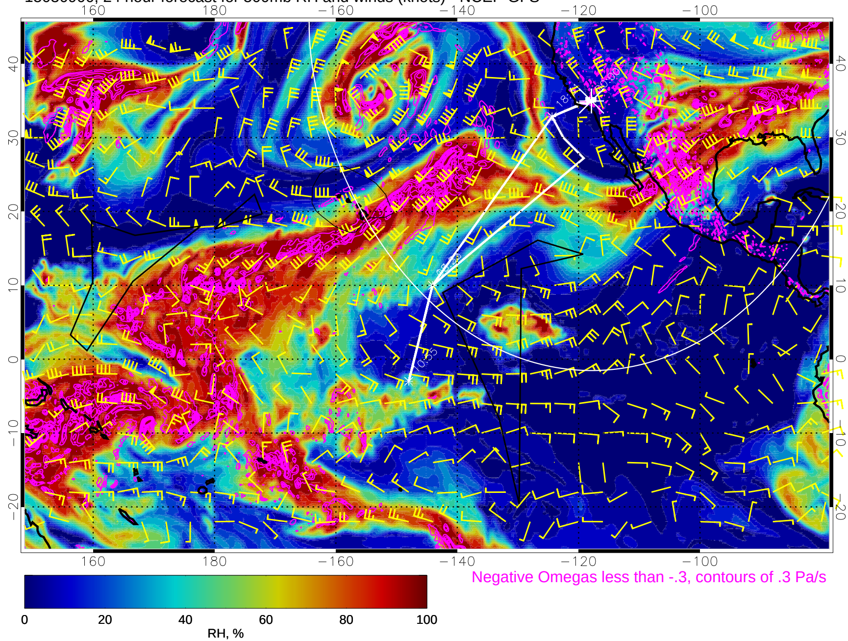
15030900, 24 hour forecast for 500mb RH and winds (knots) - NCEP GFS
