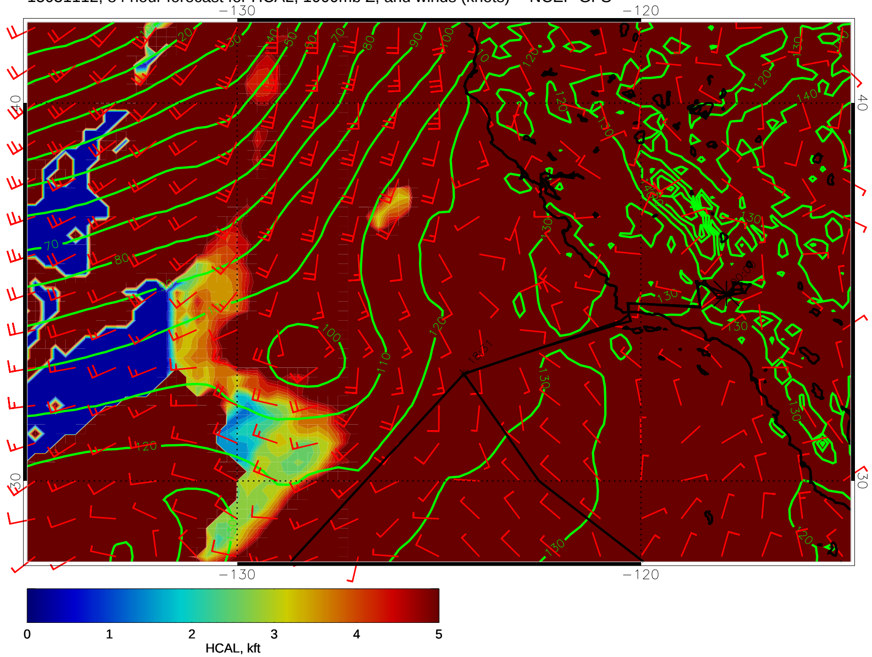
15031112, 84 hour forecast for HCAL, 1000mb Z, and winds (knots) -- NCEP GFS
