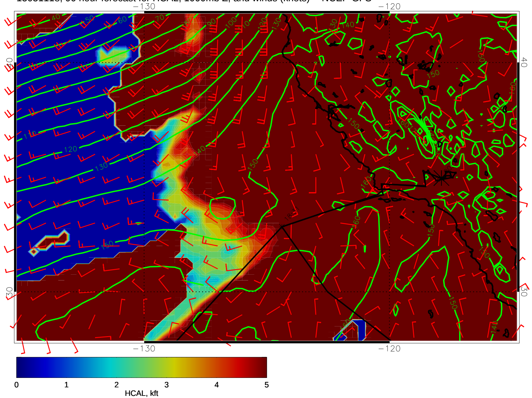
15031118, 90 hour forecast for HCAL, 1000mb Z, and winds (knots) -- NCEP GFS
