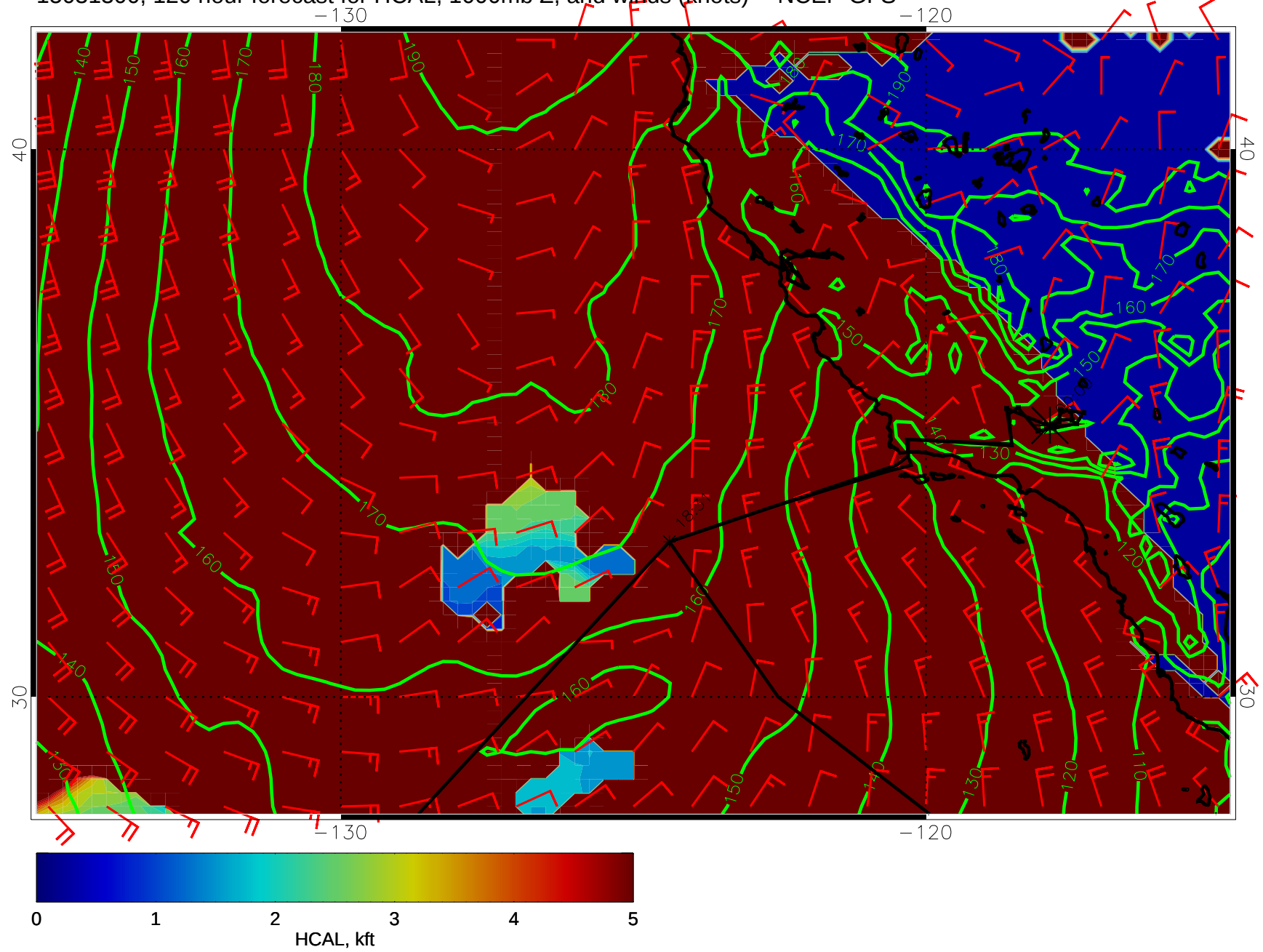
15031300, 120 hour forecast for HCAL, 1000mb Z, and winds (knots) -- NCEP GFS
