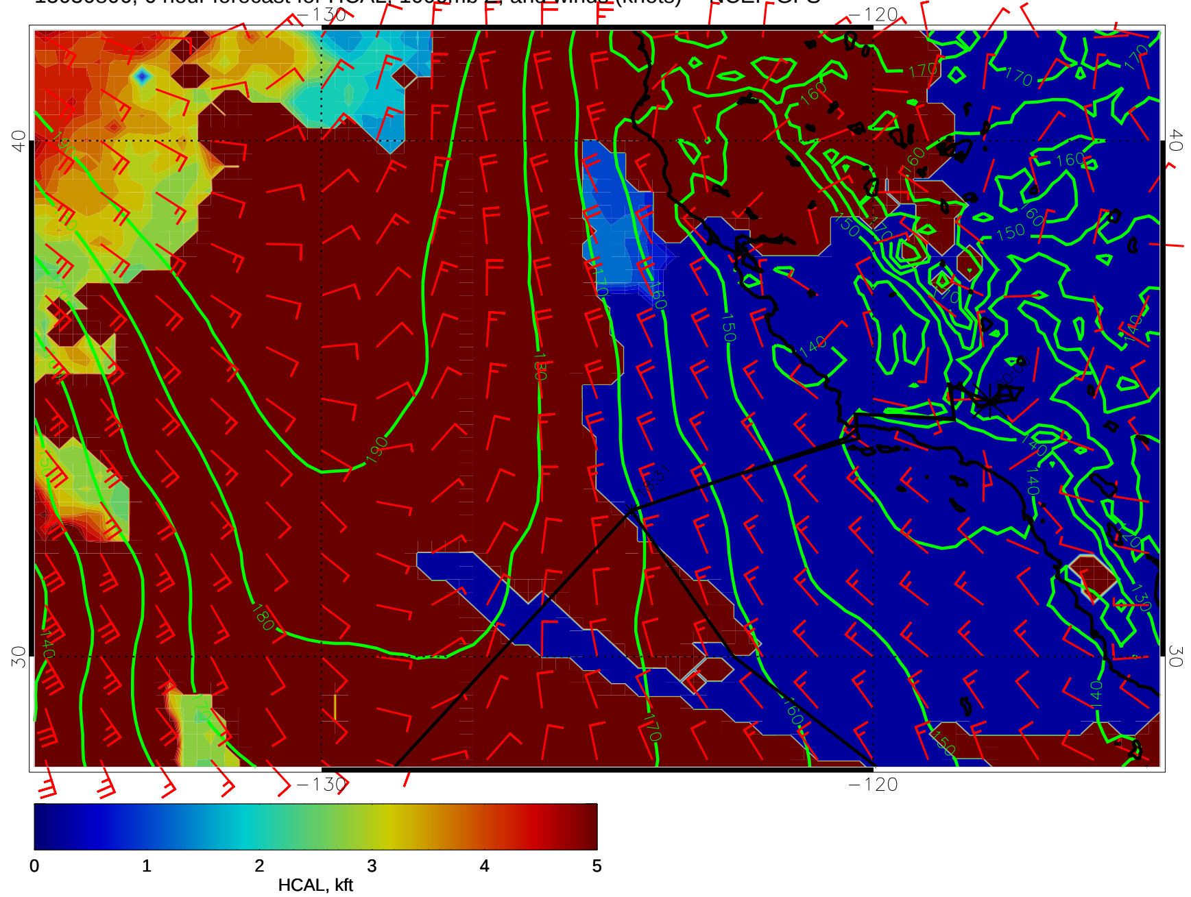
15030806, 6 hour forecast for HCAL, 1000mb Z, and winds (knots) -- NCEP GFS
