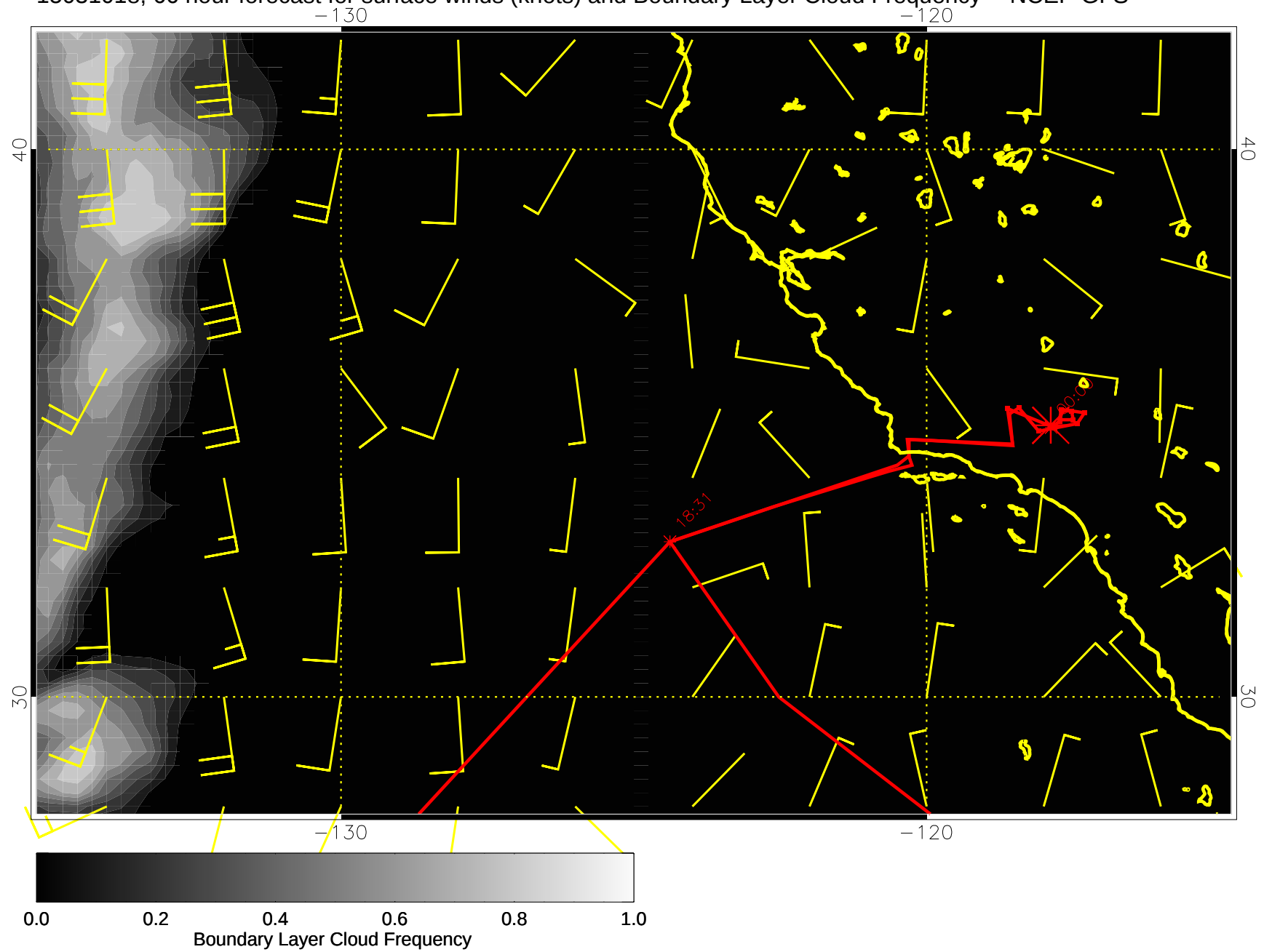
15031018, 66 hour forecast for surface winds (knots) and Boundary Layer Cloud Frequency -- NCEP GFS
