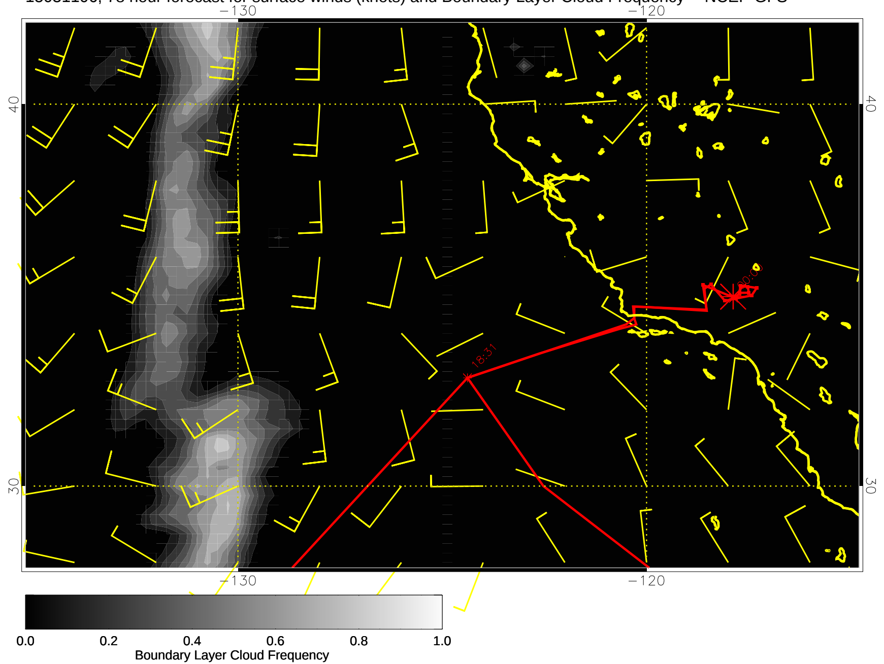
15031106, 78 hour forecast for surface winds (knots) and Boundary Layer Cloud Frequency -- NCEP GFS
