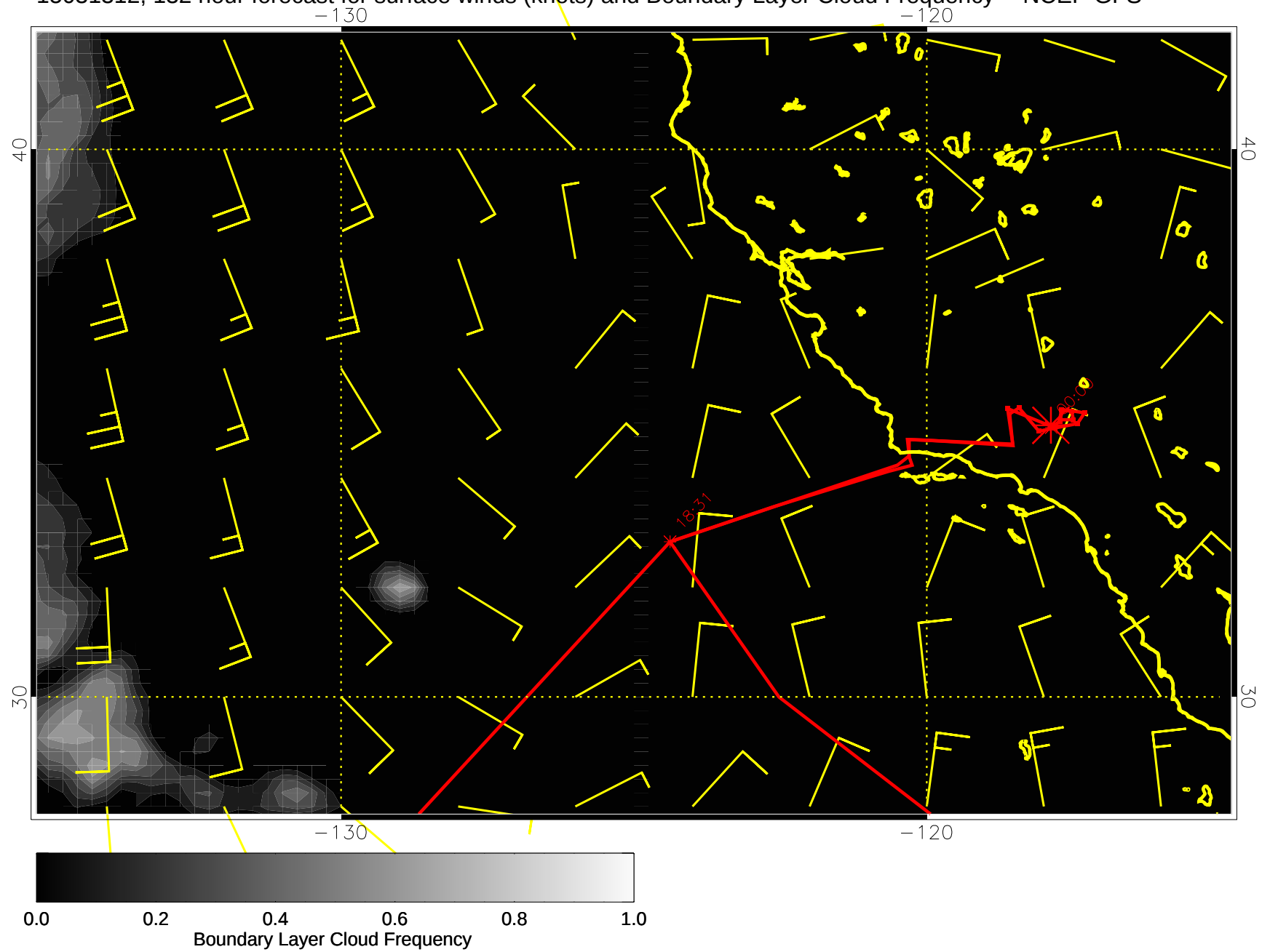
15031312, 132 hour forecast for surface winds (knots) and Boundary Layer Cloud Frequency -- NCEP GFS
