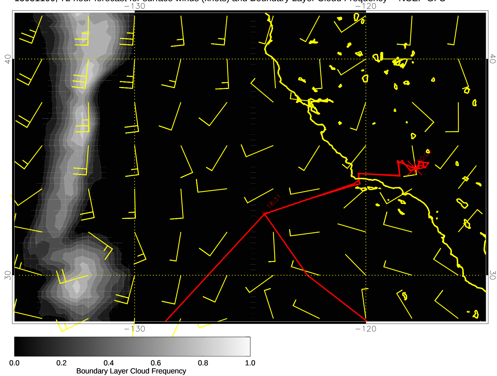
15031100, 72 hour forecast for surface winds (knots) and Boundary Layer Cloud Frequency -- NCEP GFS
