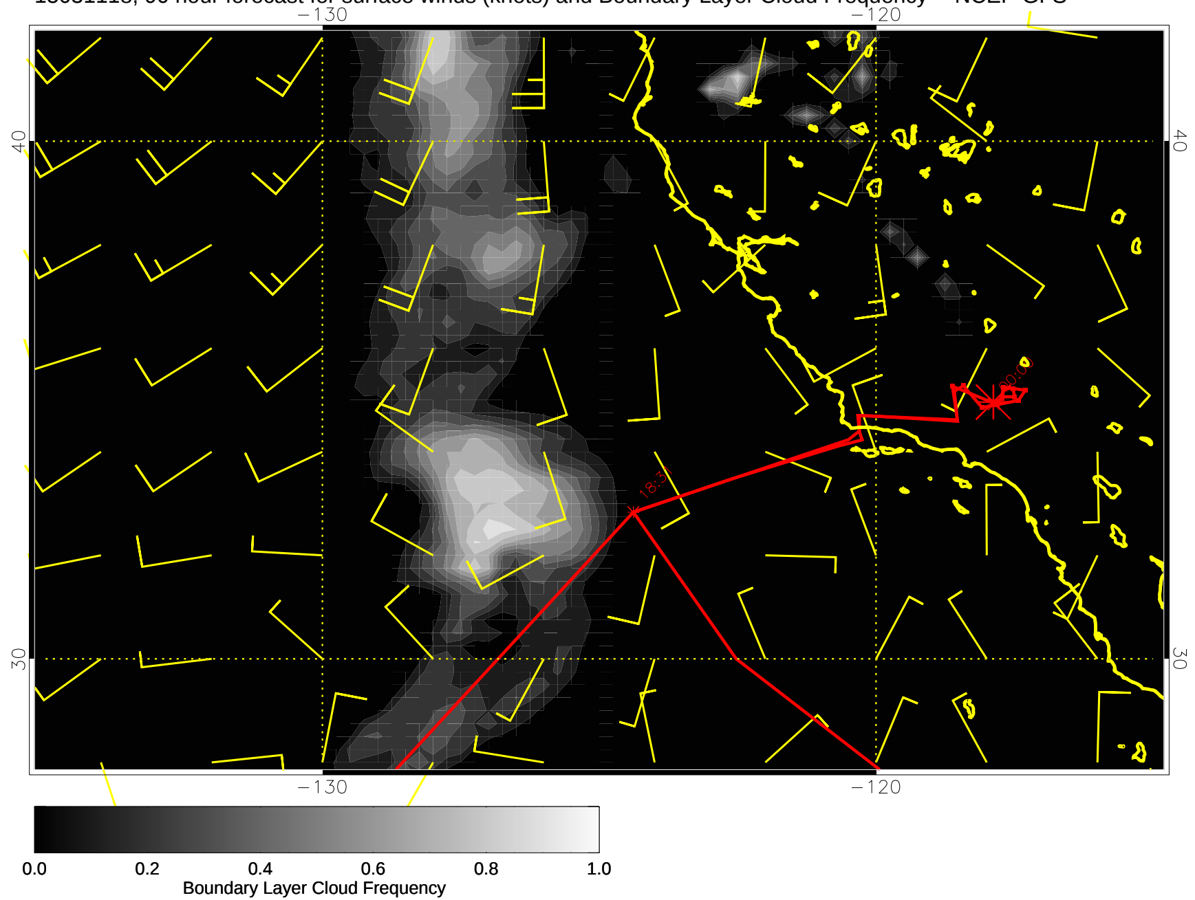
15031118, 90 hour forecast for surface winds (knots) and Boundary Layer Cloud Frequency -- NCEP GFS
