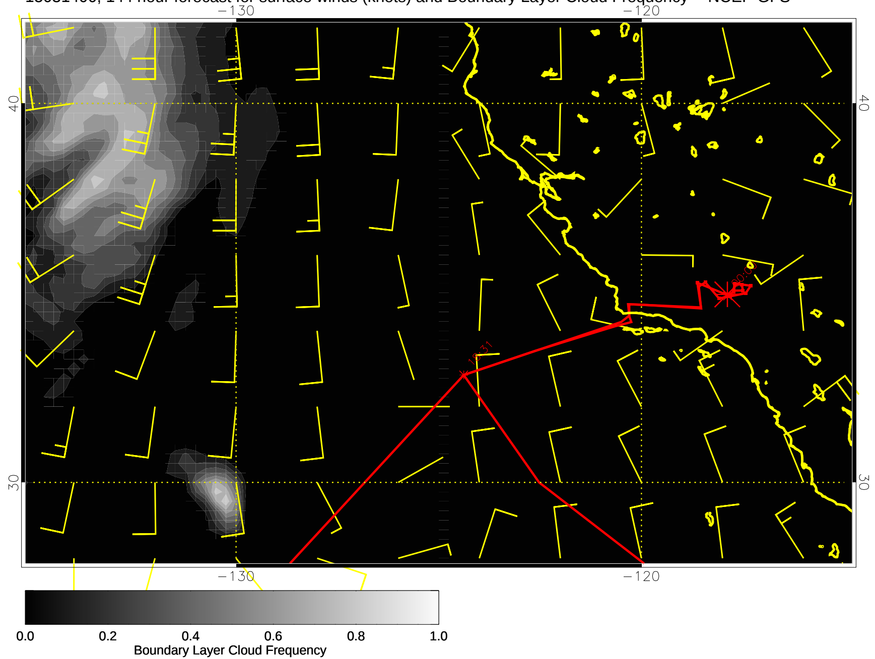
15031400, 144 hour forecast for surface winds (knots) and Boundary Layer Cloud Frequency -- NCEP GFS
