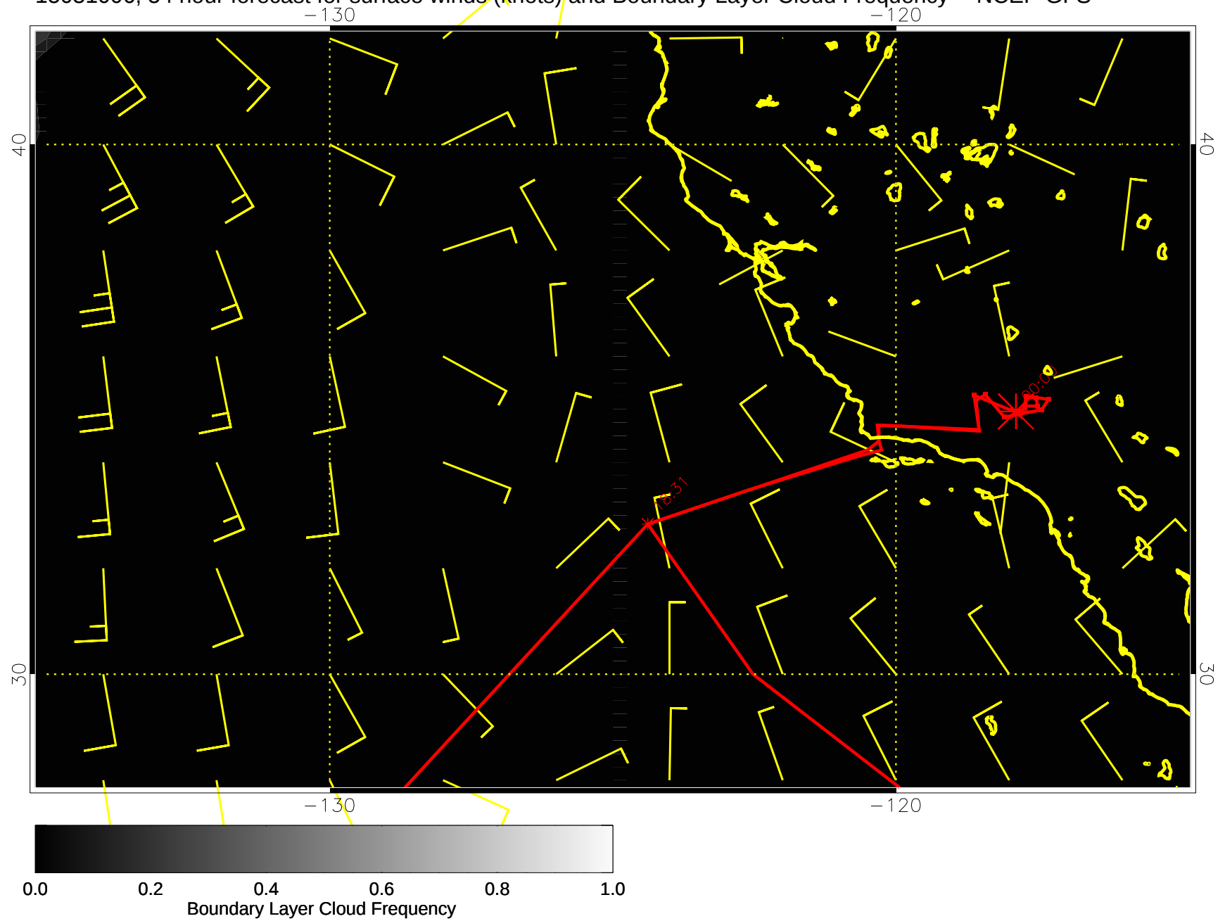
15031006, 54 hour forecast for surface winds (knots) and Boundary Layer Cloud Frequency -- NCEP GFS
