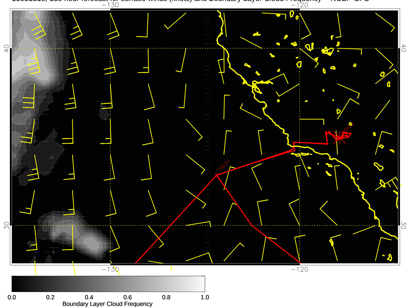
15031318, 138 hour forecast for surface winds (knots) and Boundary Layer Cloud Frequency -- NCEP GFS
