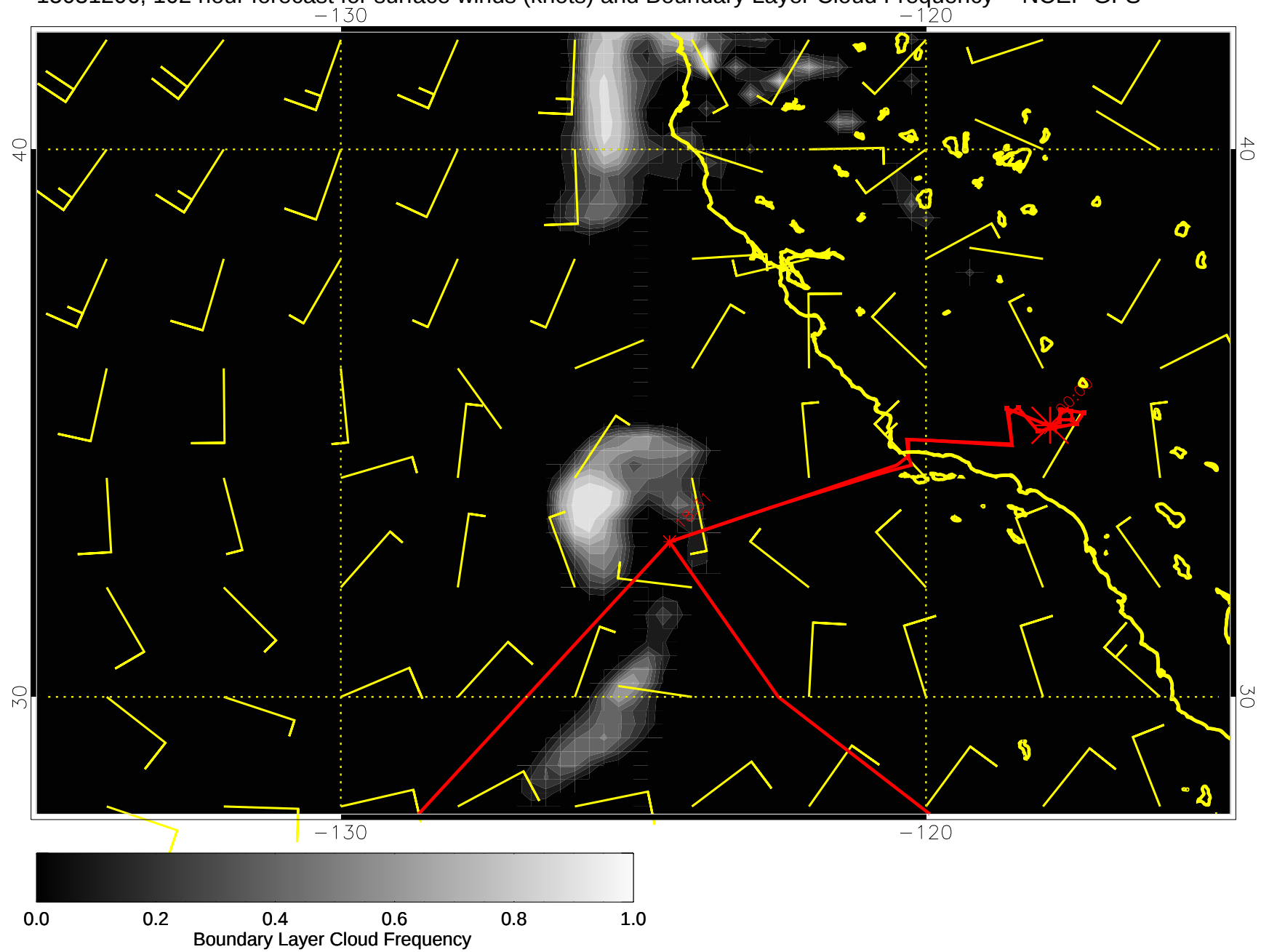
15031206, 102 hour forecast for surface winds (knots) and Boundary Layer Cloud Frequency -- NCEP GFS
