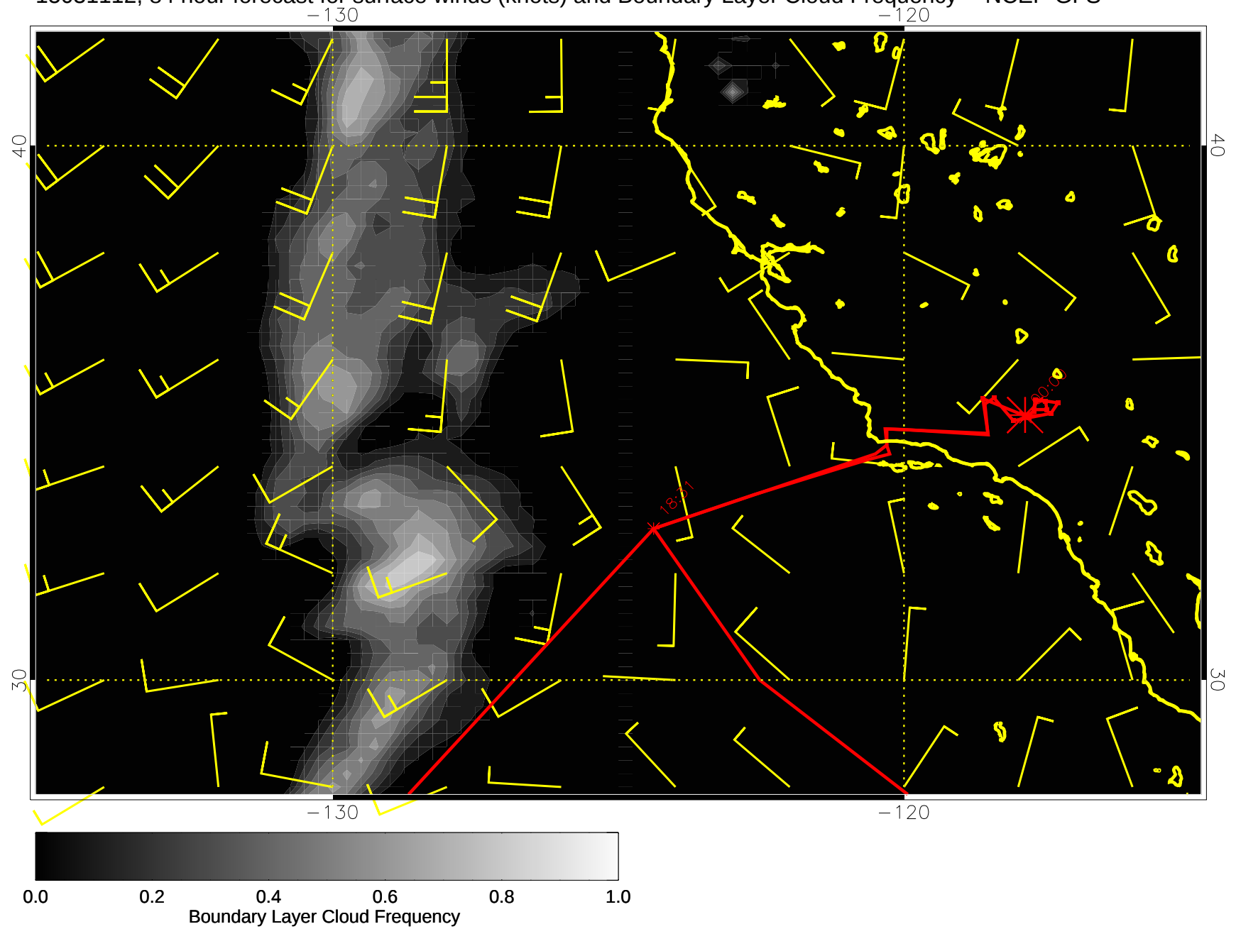
15031112, 84 hour forecast for surface winds (knots) and Boundary Layer Cloud Frequency -- NCEP GFS
