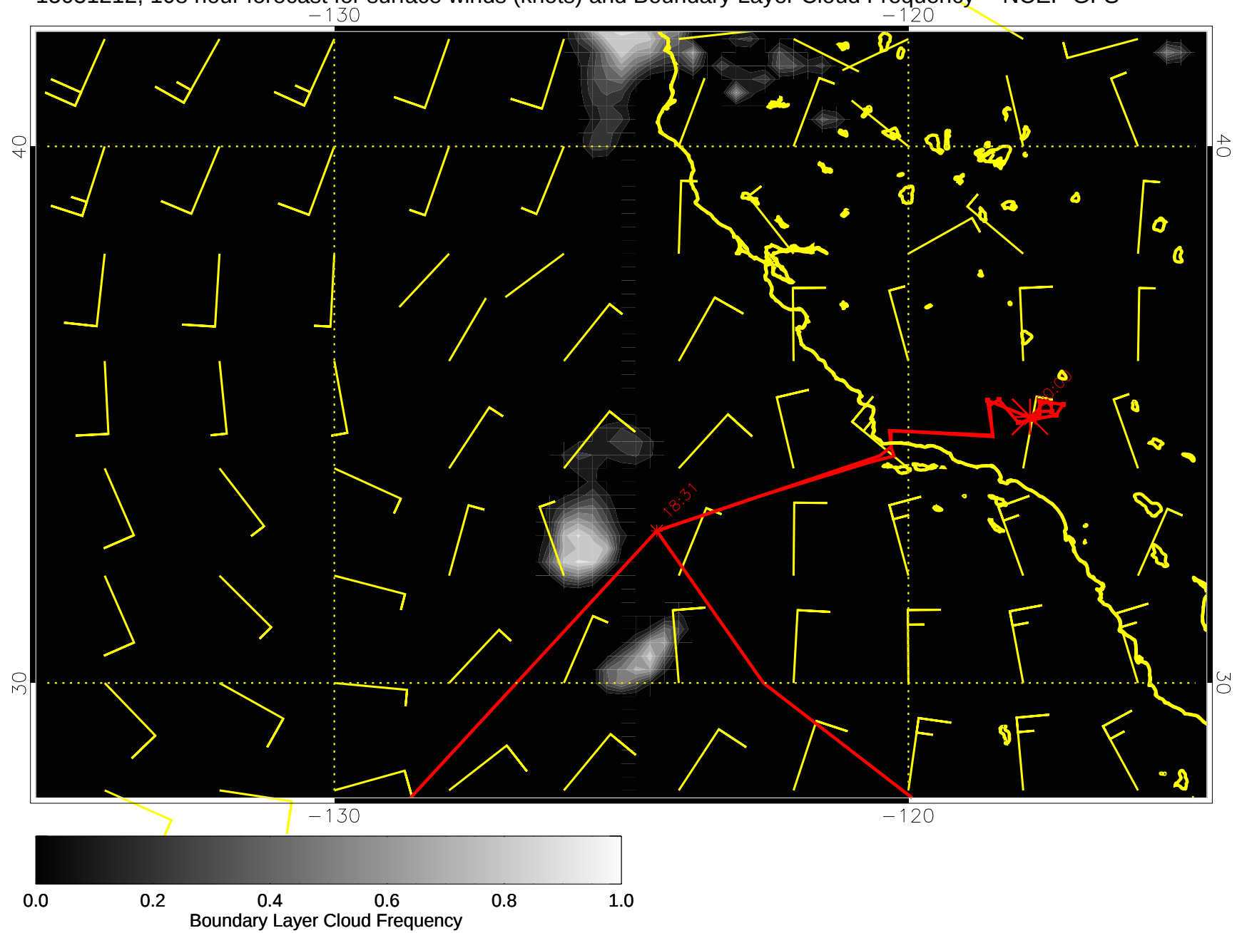
15031212, 108 hour forecast for surface winds (knots) and Boundary Layer Cloud Frequency -- NCEP GFS
