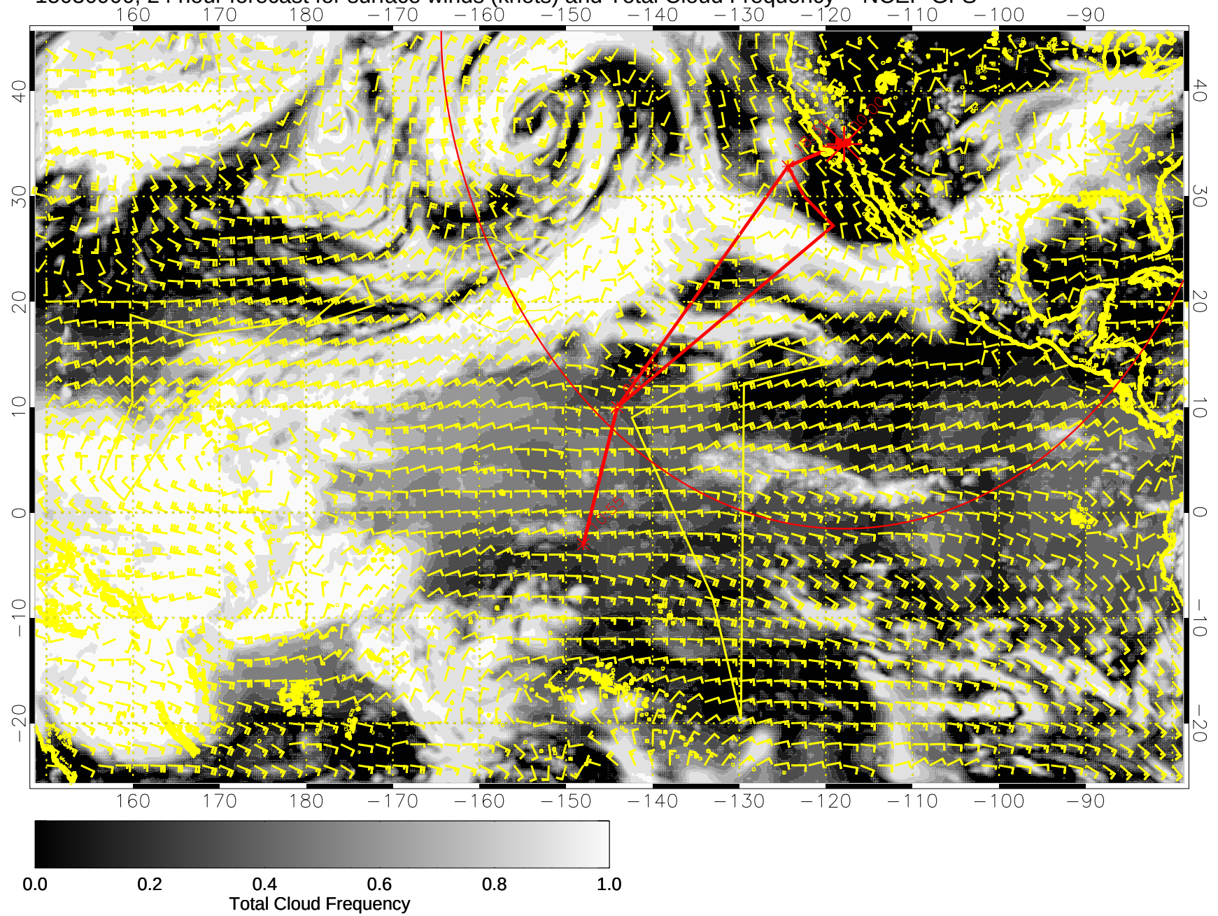
15030900, 24 hour forecast for surface winds (knots) and Total Cloud Frequency -- NCEP GFS
