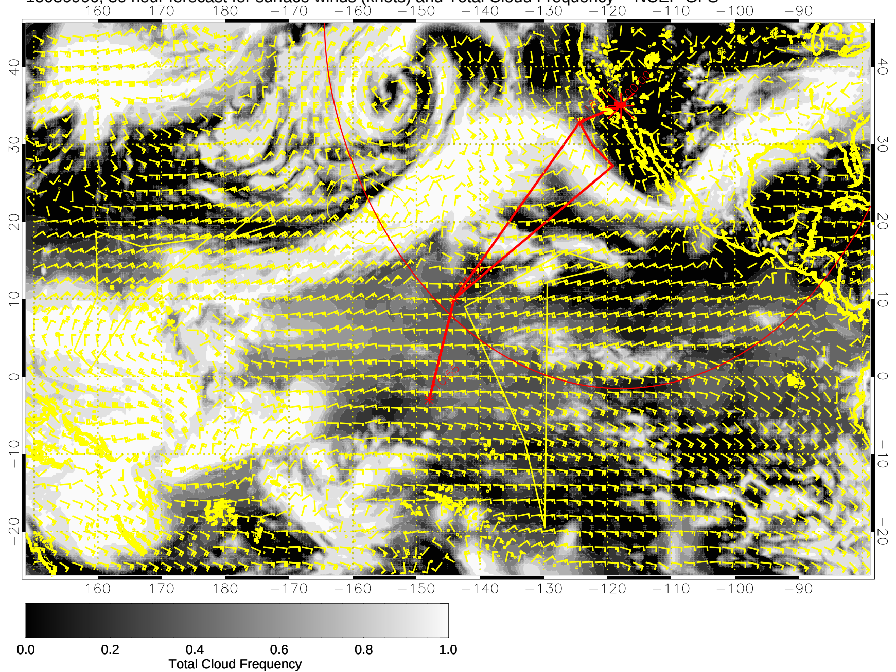
15030906, 30 hour forecast for surface winds (knots) and Total Cloud Frequency -- NCEP GFS
