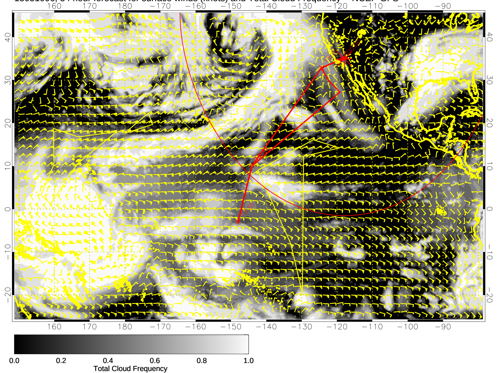
15031006, 54 hour forecast for surface winds (knots) and Total Cloud Frequency -- NCEP GFS
