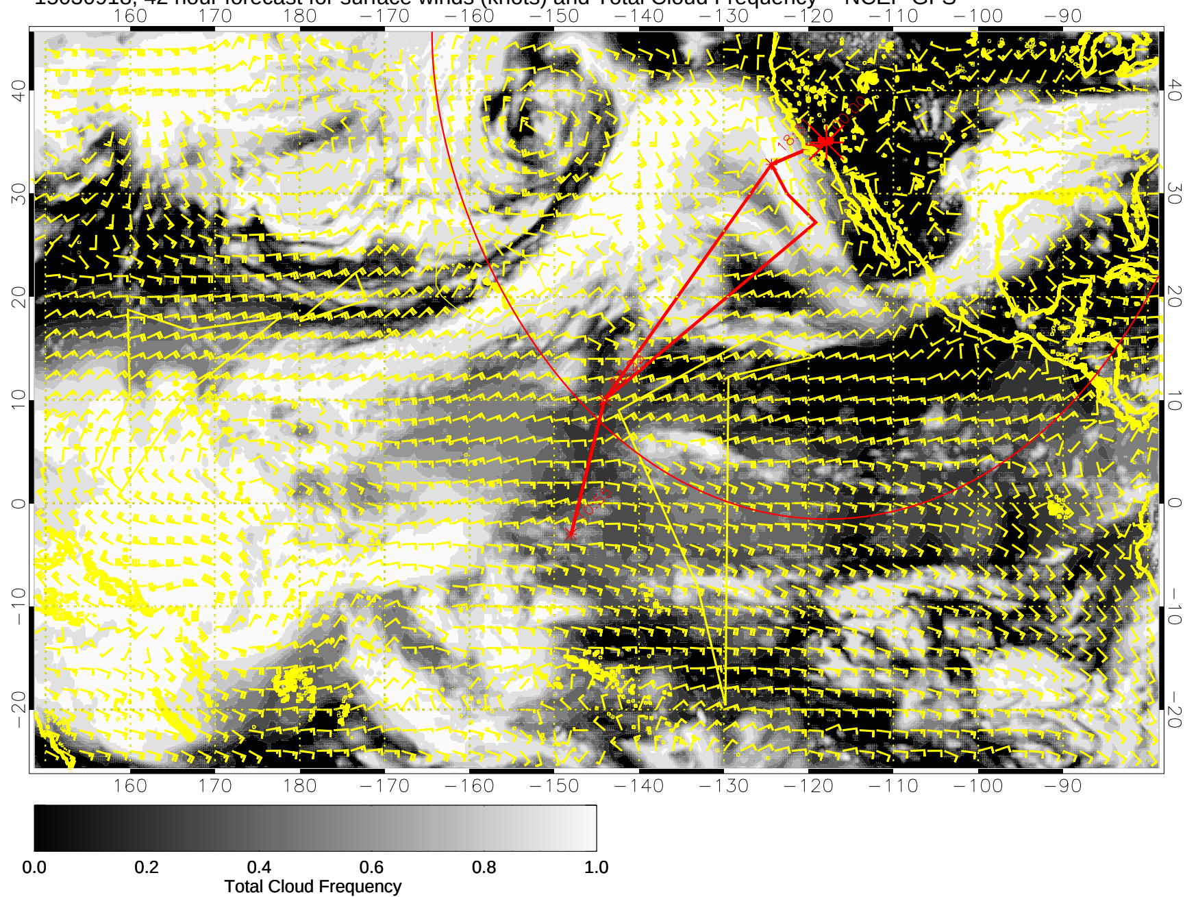
15030918, 42 hour forecast for surface winds (knots) and Total Cloud Frequency -- NCEP GFS
