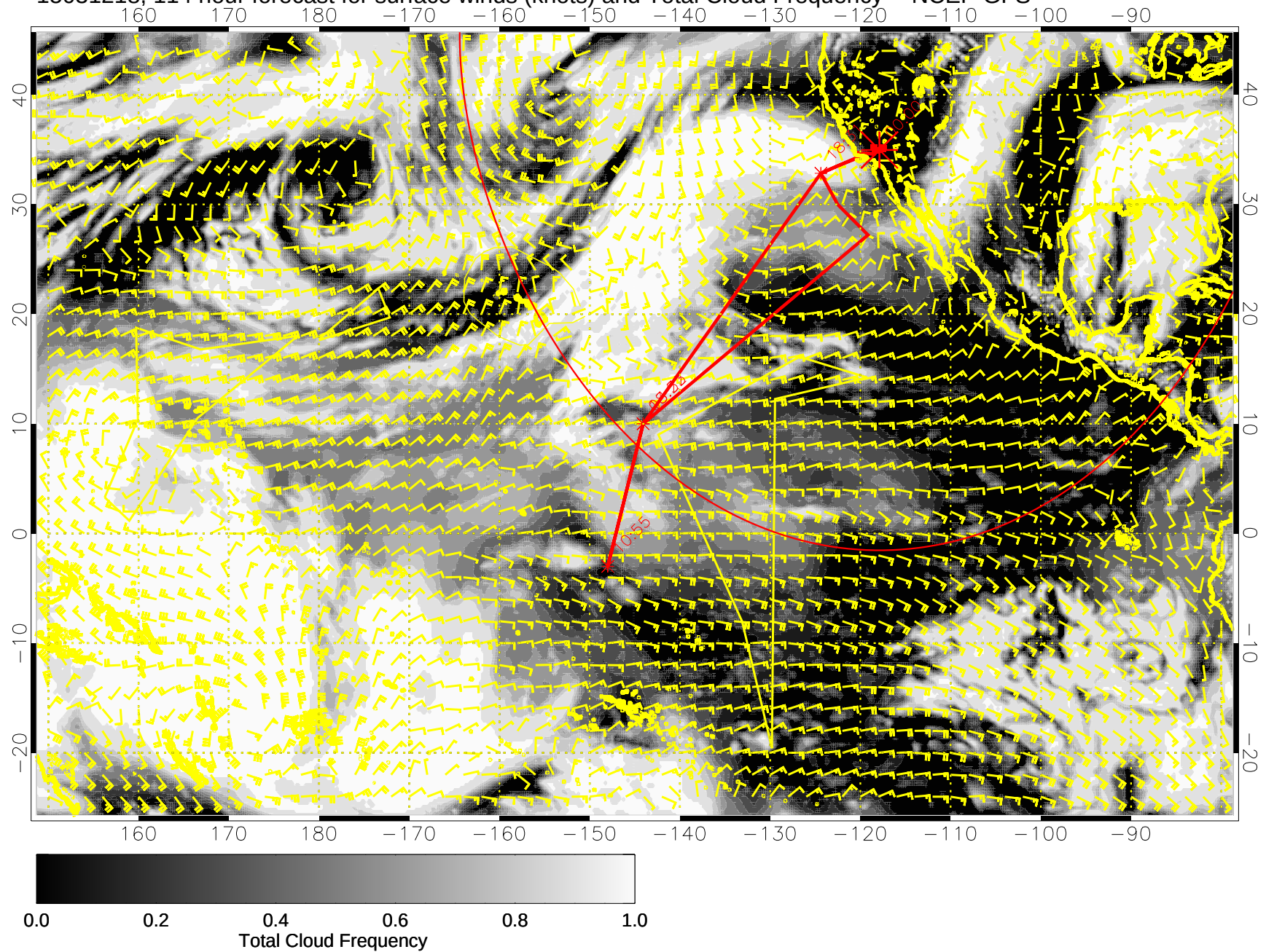
15031218, 114 hour forecast for surface winds (knots) and Total Cloud Frequency -- NCEP GFS
