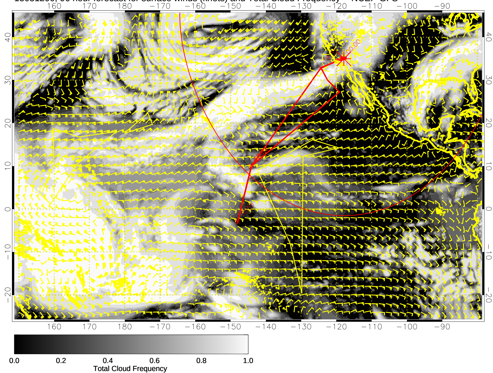
15031200, 96 hour forecast for surface winds (knots) and Total Cloud Frequency -- NCEP GFS
