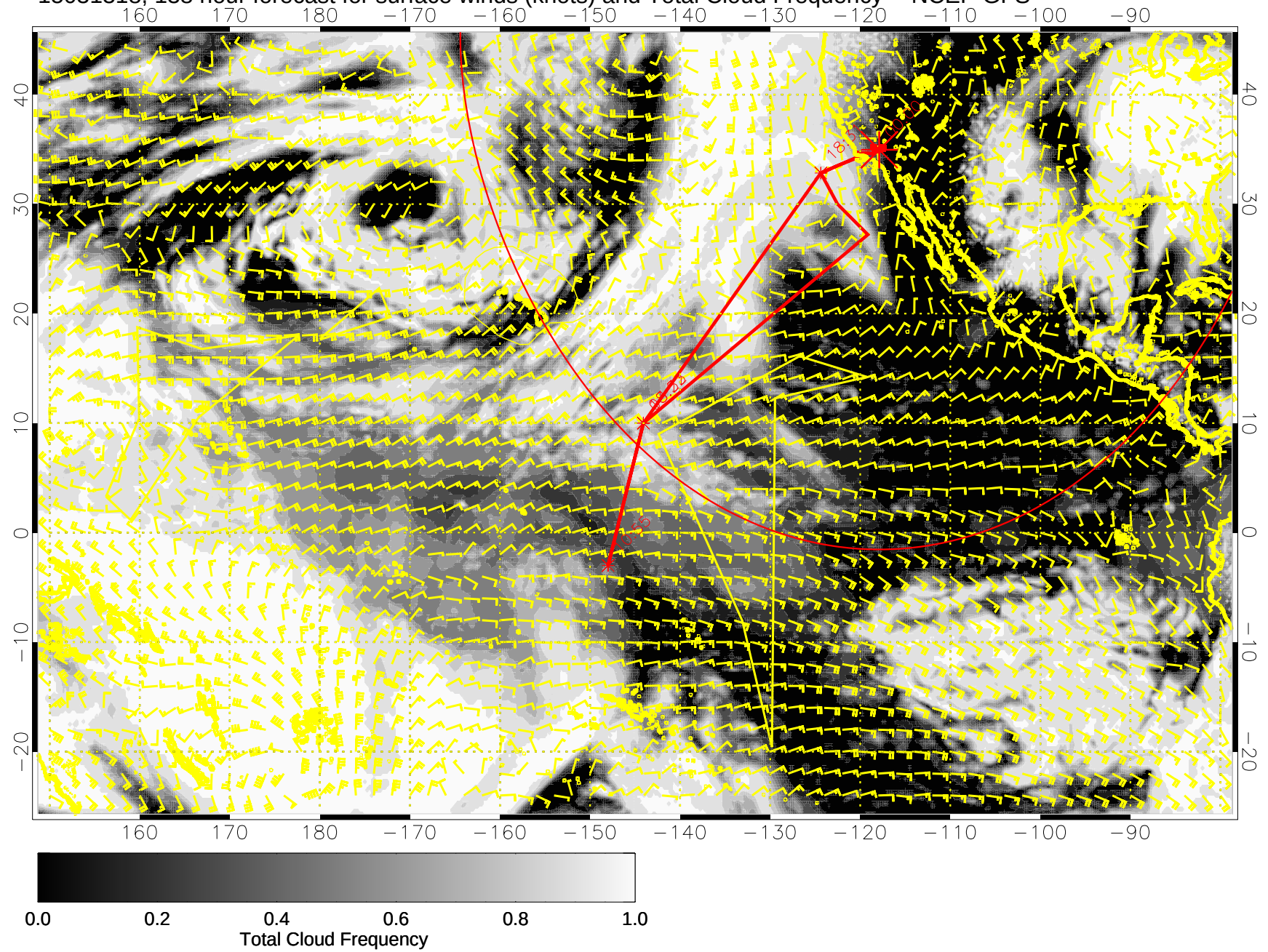
15031318, 138 hour forecast for surface winds (knots) and Total Cloud Frequency -- NCEP GFS
