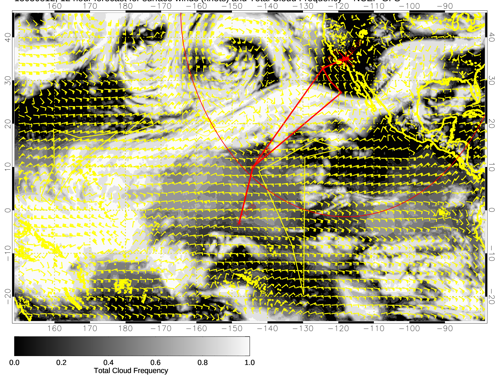
15030812, 12 hour forecast for surface winds (knots) and Total Cloud Frequency -- NCEP GFS
