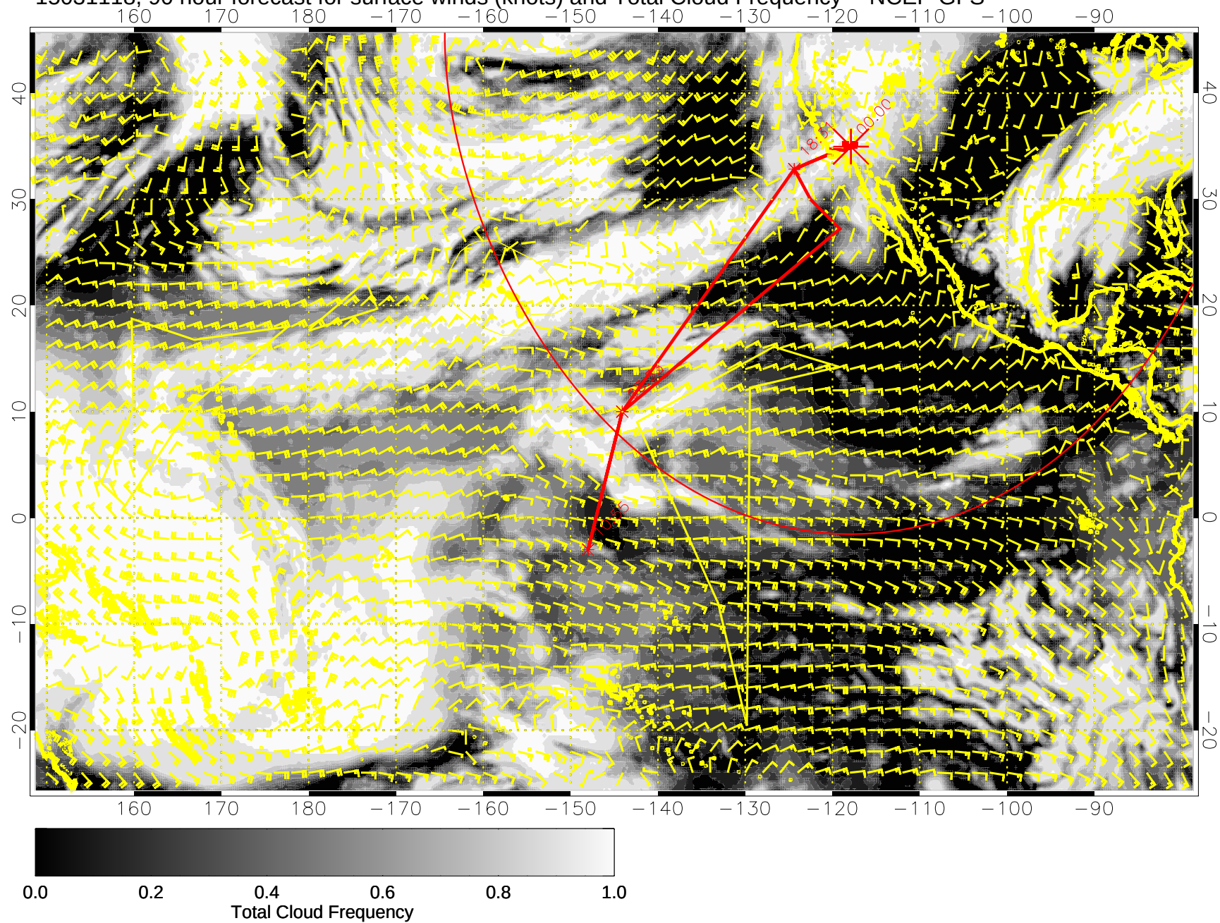
15031118, 90 hour forecast for surface winds (knots) and Total Cloud Frequency -- NCEP GFS
