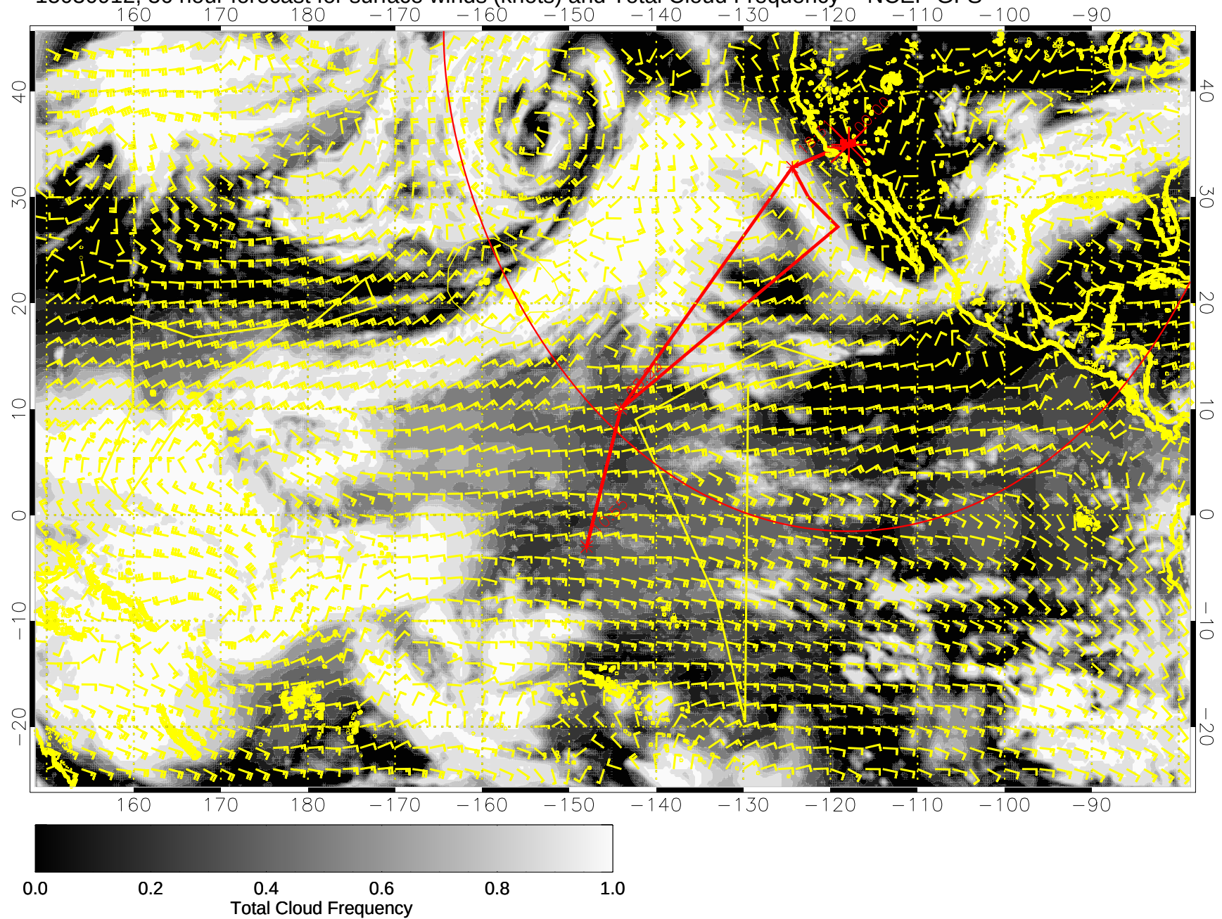
15030912, 36 hour forecast for surface winds (knots) and Total Cloud Frequency -- NCEP GFS
