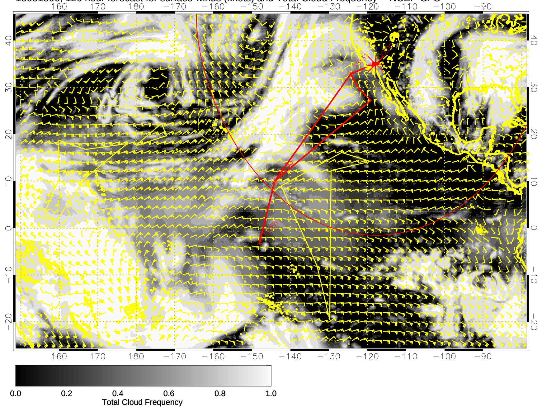
15031306, 126 hour forecast for surface winds (knots) and Total Cloud Frequency -- NCEP GFS
