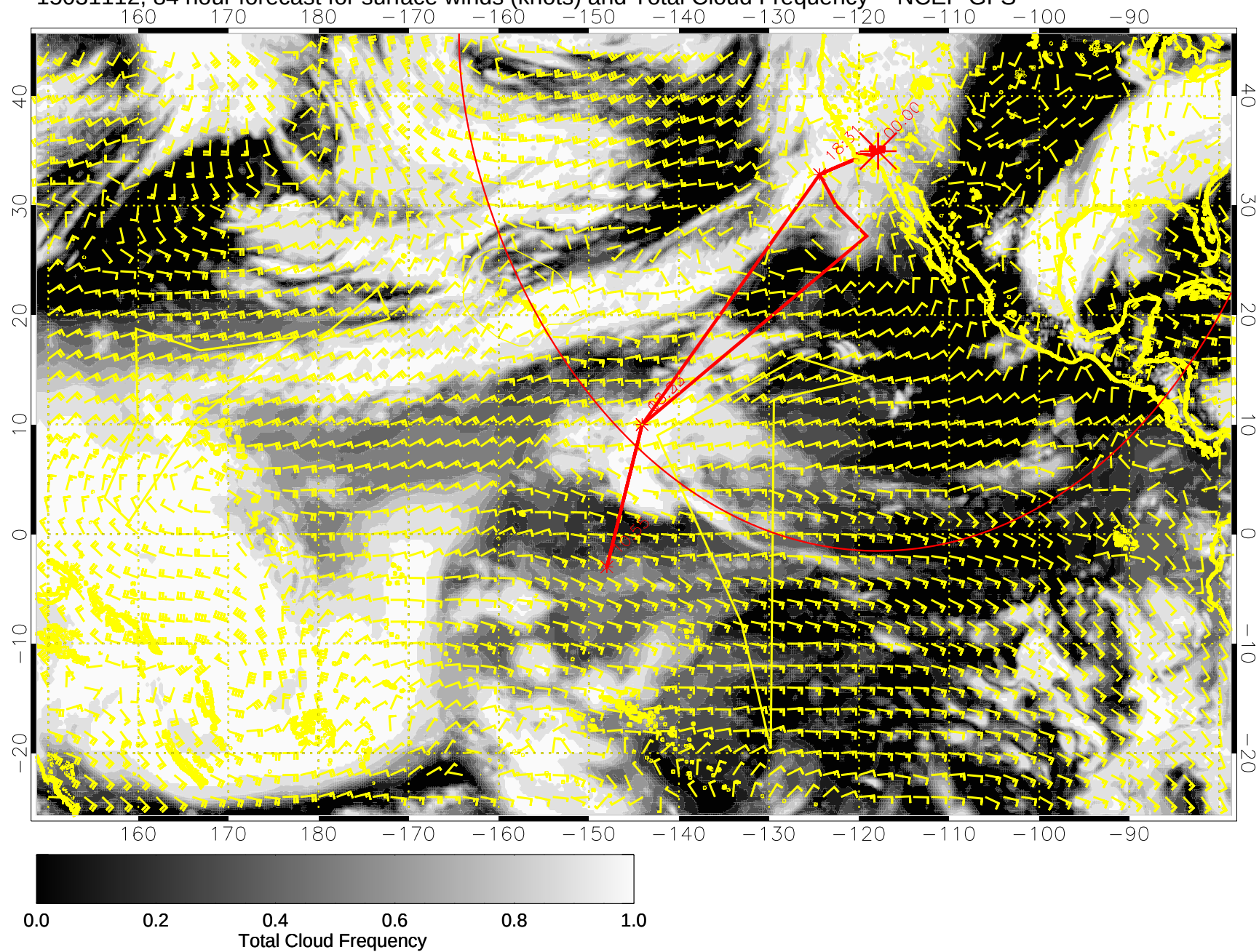
15031112, 84 hour forecast for surface winds (knots) and Total Cloud Frequency -- NCEP GFS
