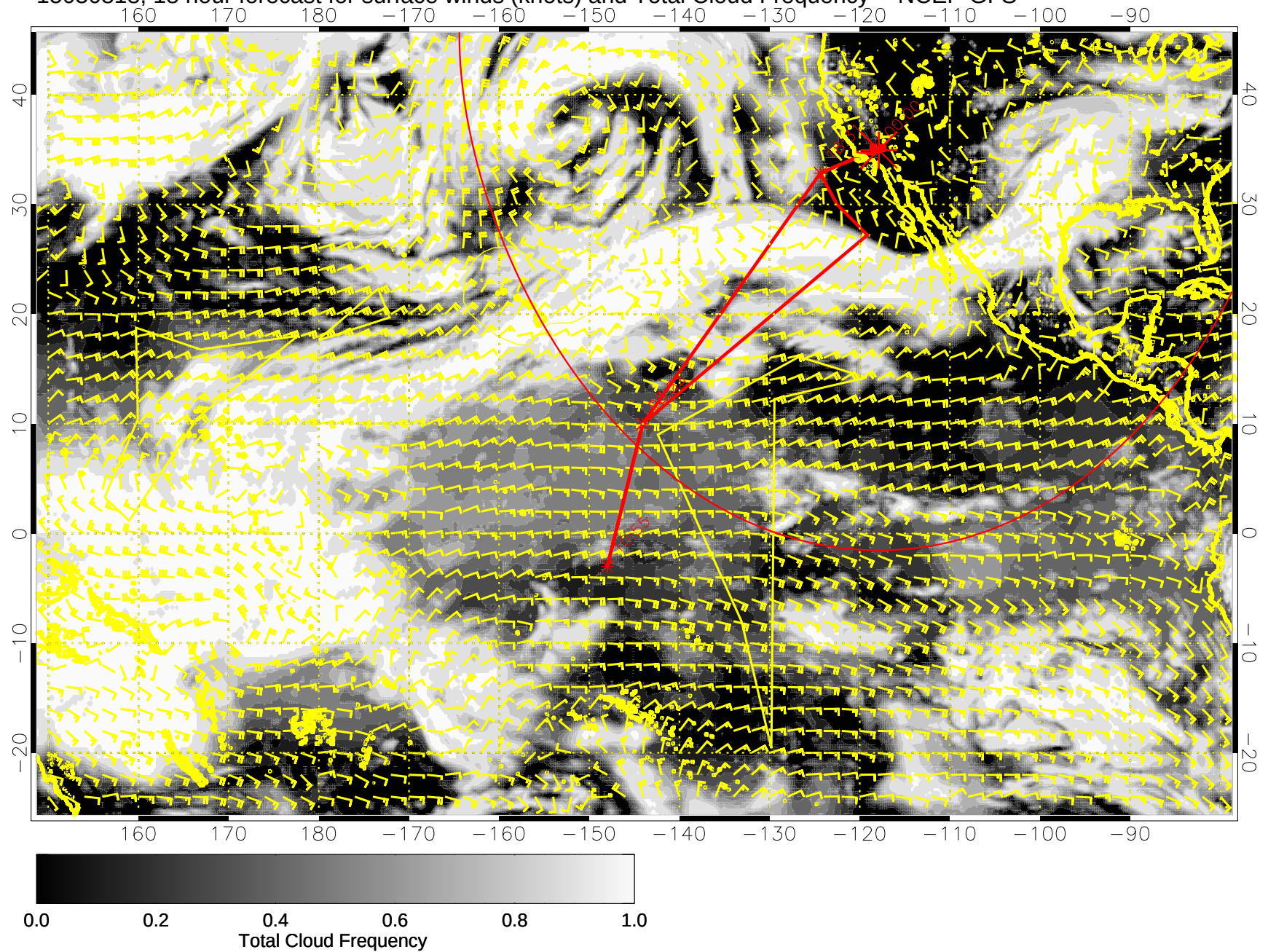
15030818, 18 hour forecast for surface winds (knots) and Total Cloud Frequency -- NCEP GFS
