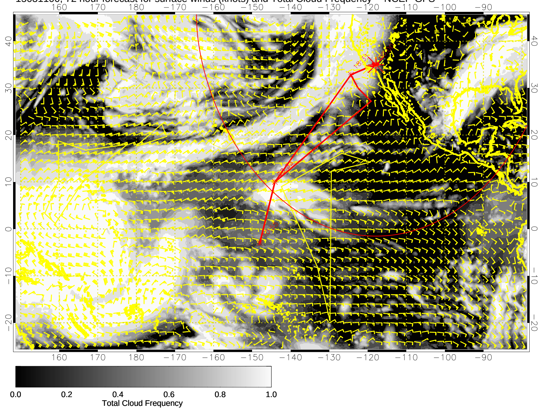
15031100, 72 hour forecast for surface winds (knots) and Total Cloud Frequency -- NCEP GFS
