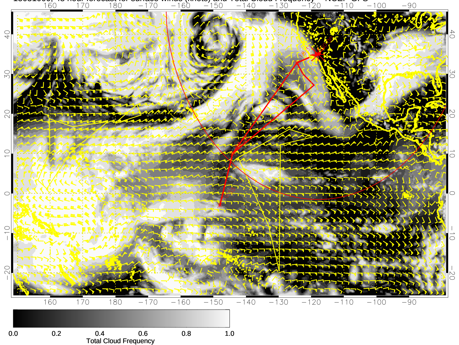
15031000, 48 hour forecast for surface winds (knots) and Total Cloud Frequency -- NCEP GFS
