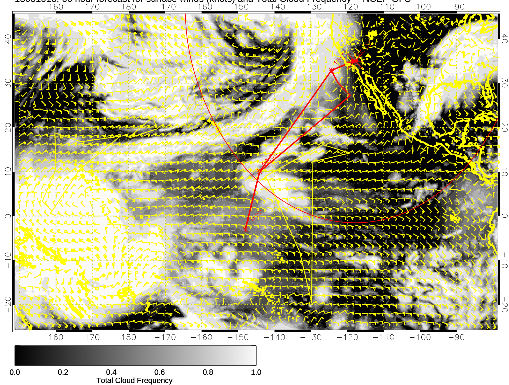
15031018, 66 hour forecast for surface winds (knots) and Total Cloud Frequency -- NCEP GFS
