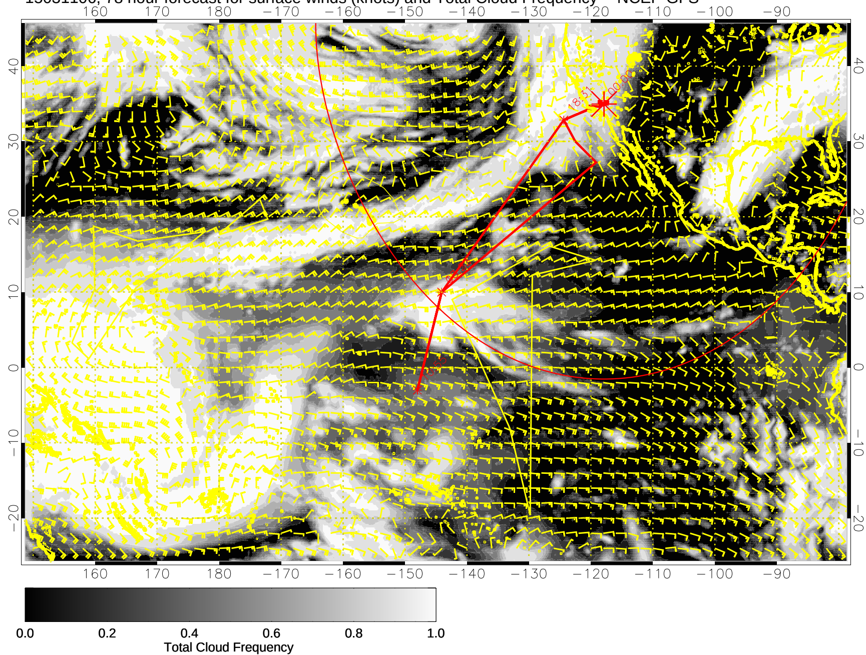
15031106, 78 hour forecast for surface winds (knots) and Total Cloud Frequency -- NCEP GFS
