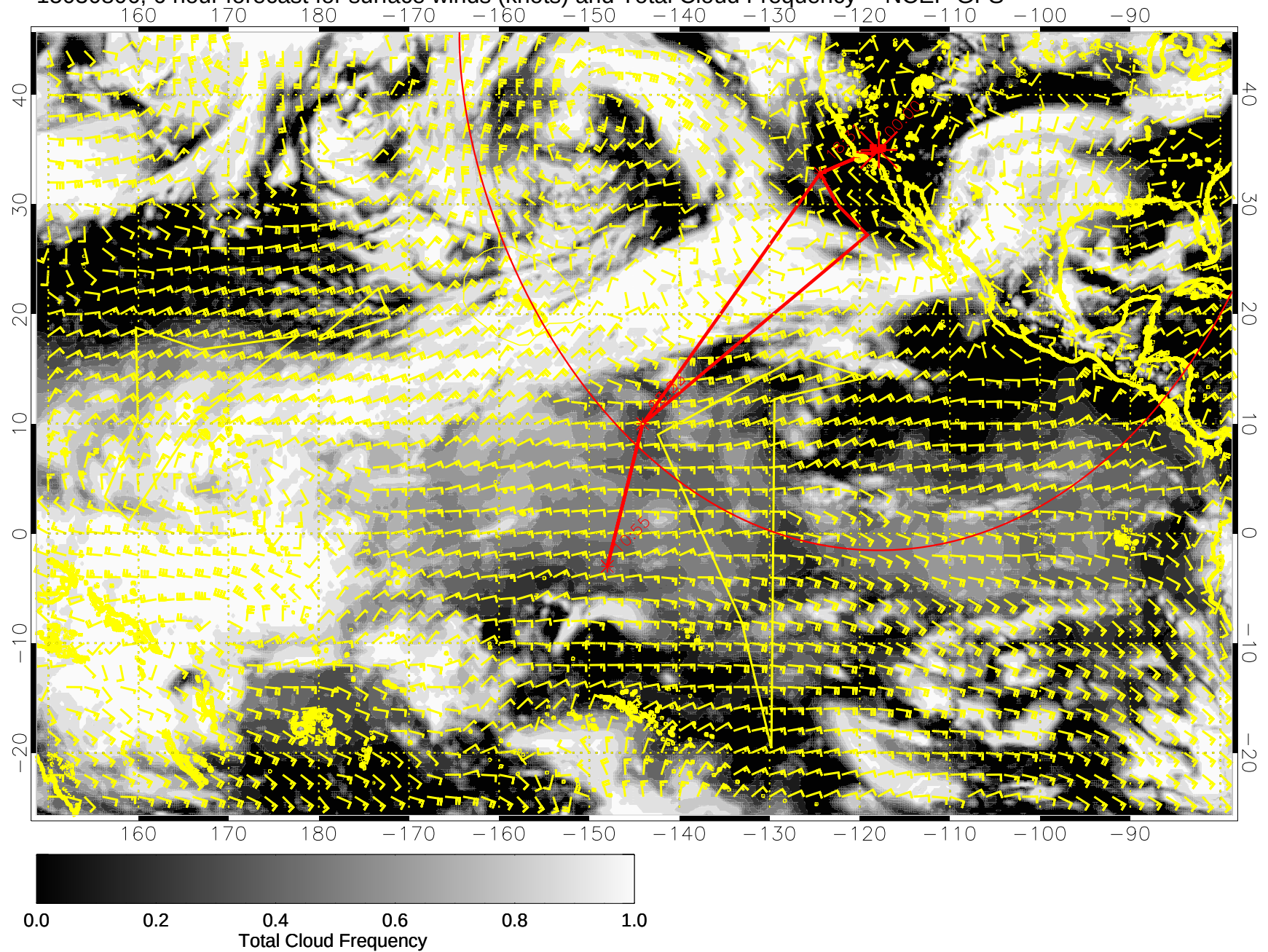
15030806, 6 hour forecast for surface winds (knots) and Total Cloud Frequency -- NCEP GFS
