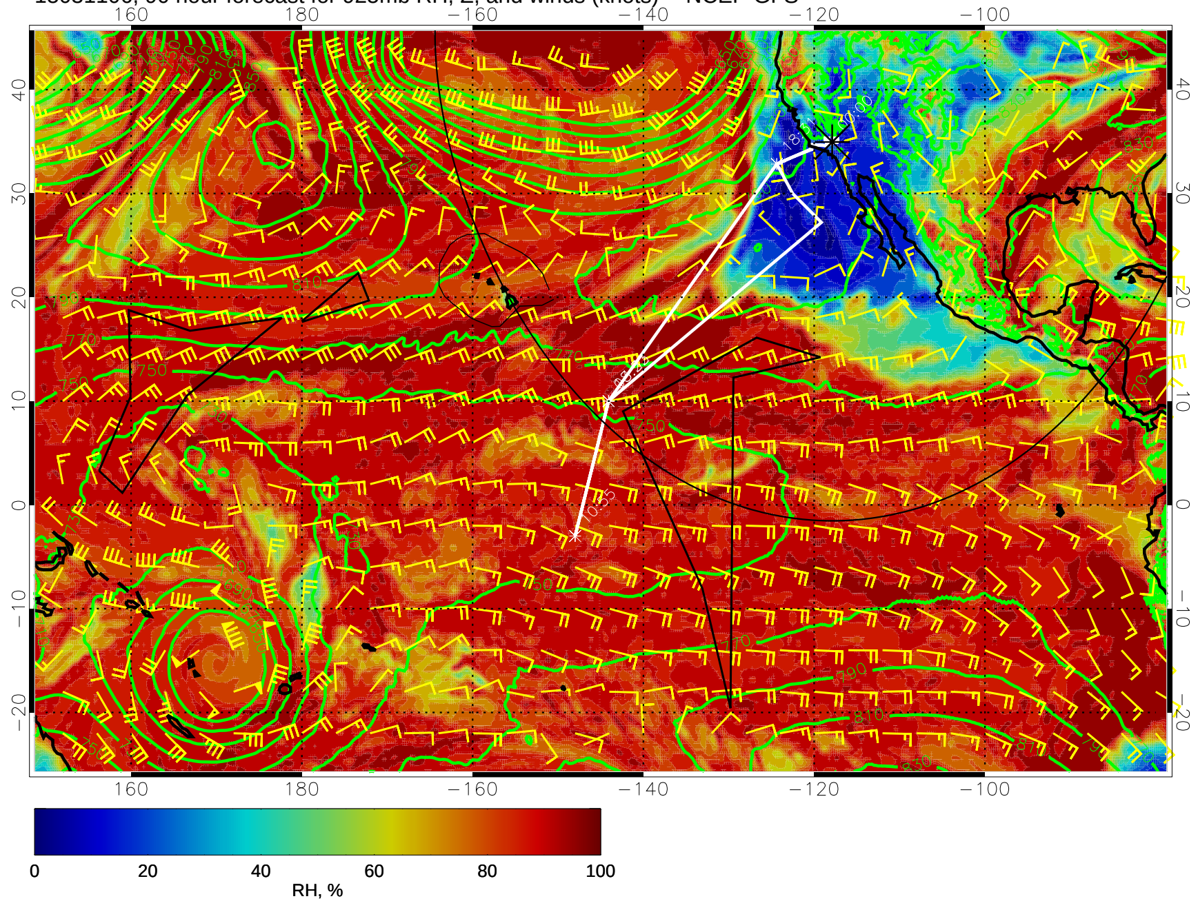
15031106, 90 hour forecast for 925mb RH, Z, and winds (knots) -- NCEP GFS
