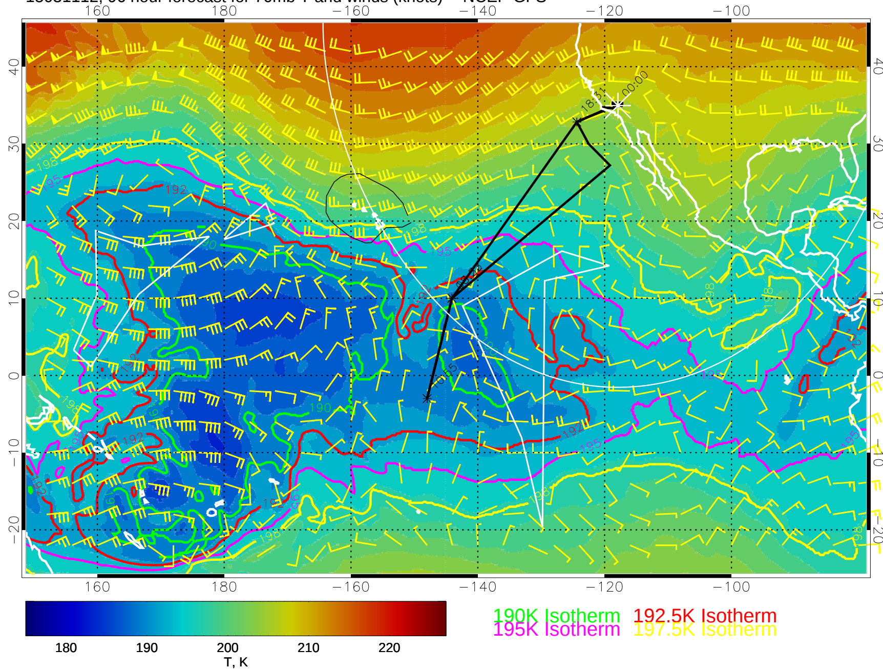
15031112, 96 hour forecast for 70mb T and winds (knots) -- NCEP GFS
