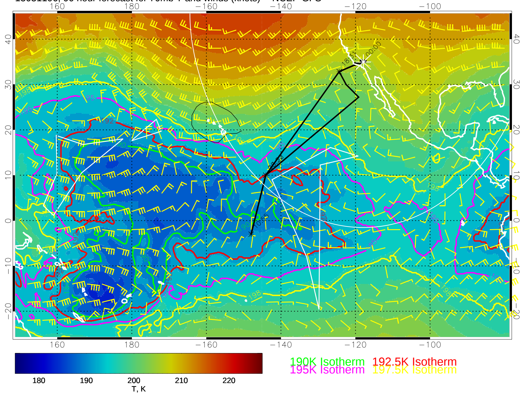
15031106, 90 hour forecast for 70mb T and winds (knots) -- NCEP GFS
