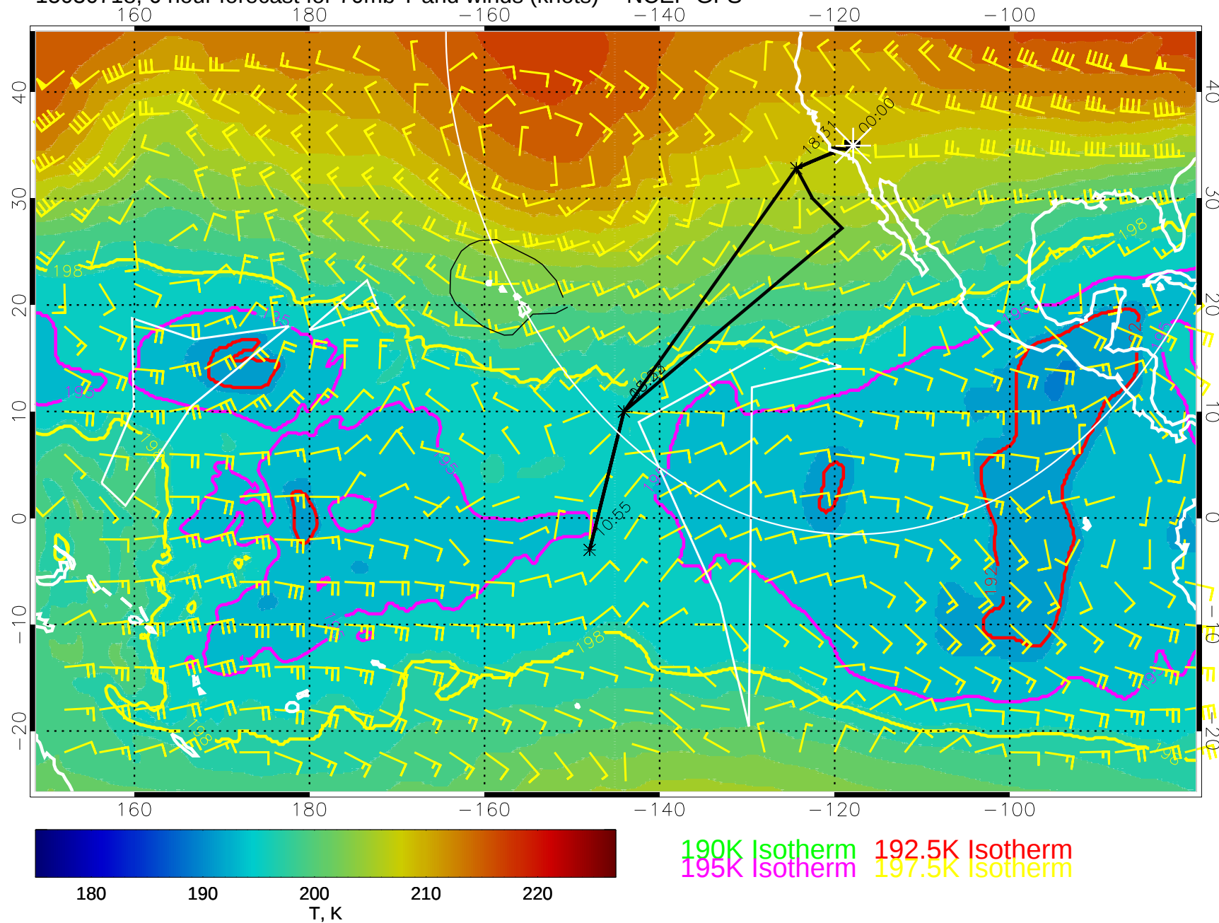
15030718, 6 hour forecast for 70mb T and winds (knots) -- NCEP GFS
