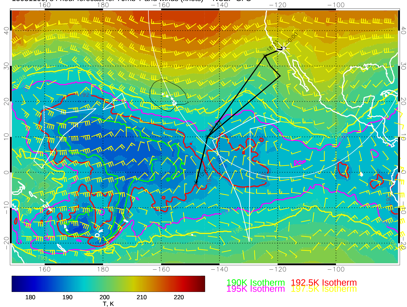
15031100, 84 hour forecast for 70mb T and winds (knots) -- NCEP GFS
