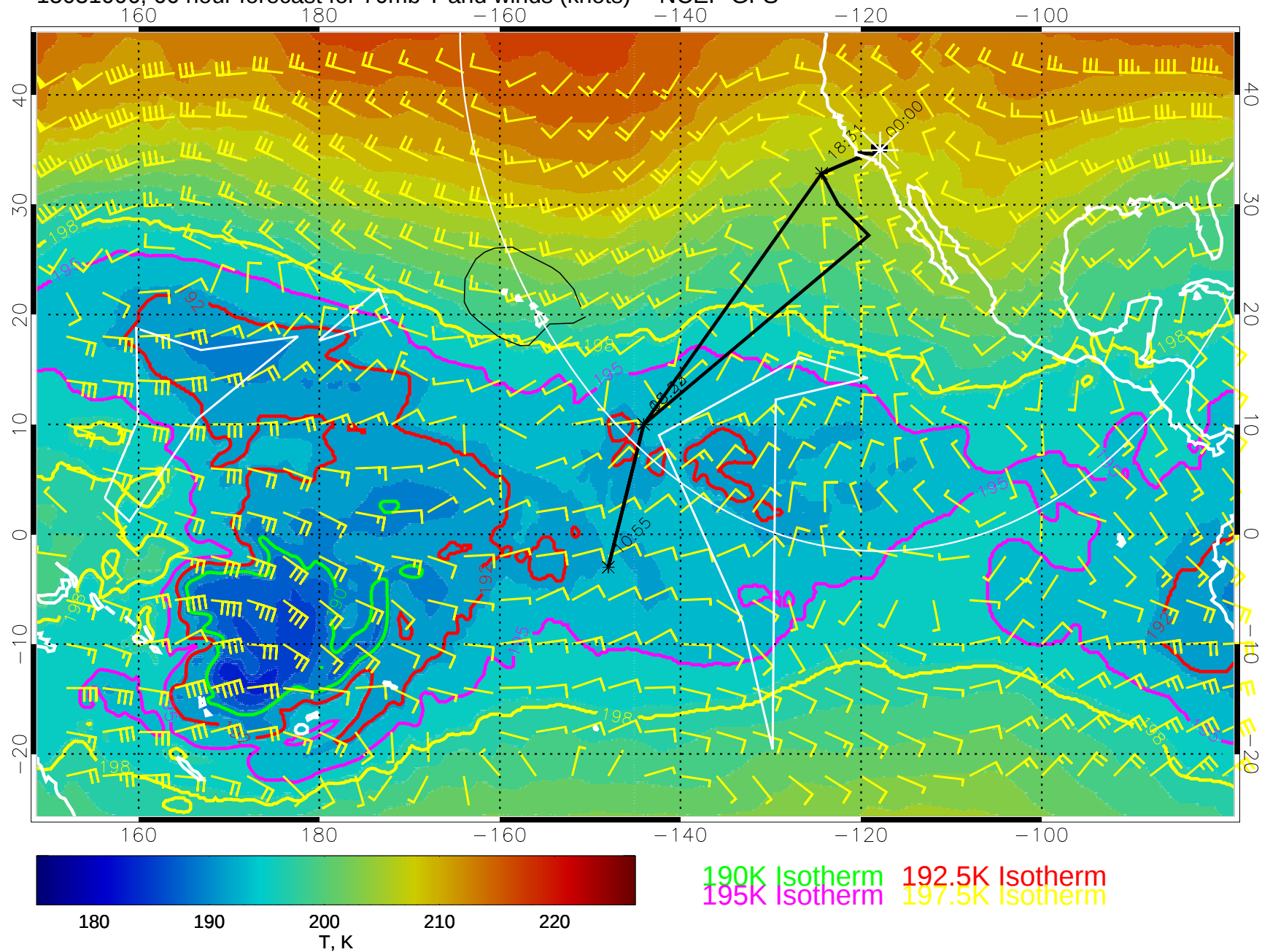
15031006, 66 hour forecast for 70mb T and winds (knots) -- NCEP GFS
