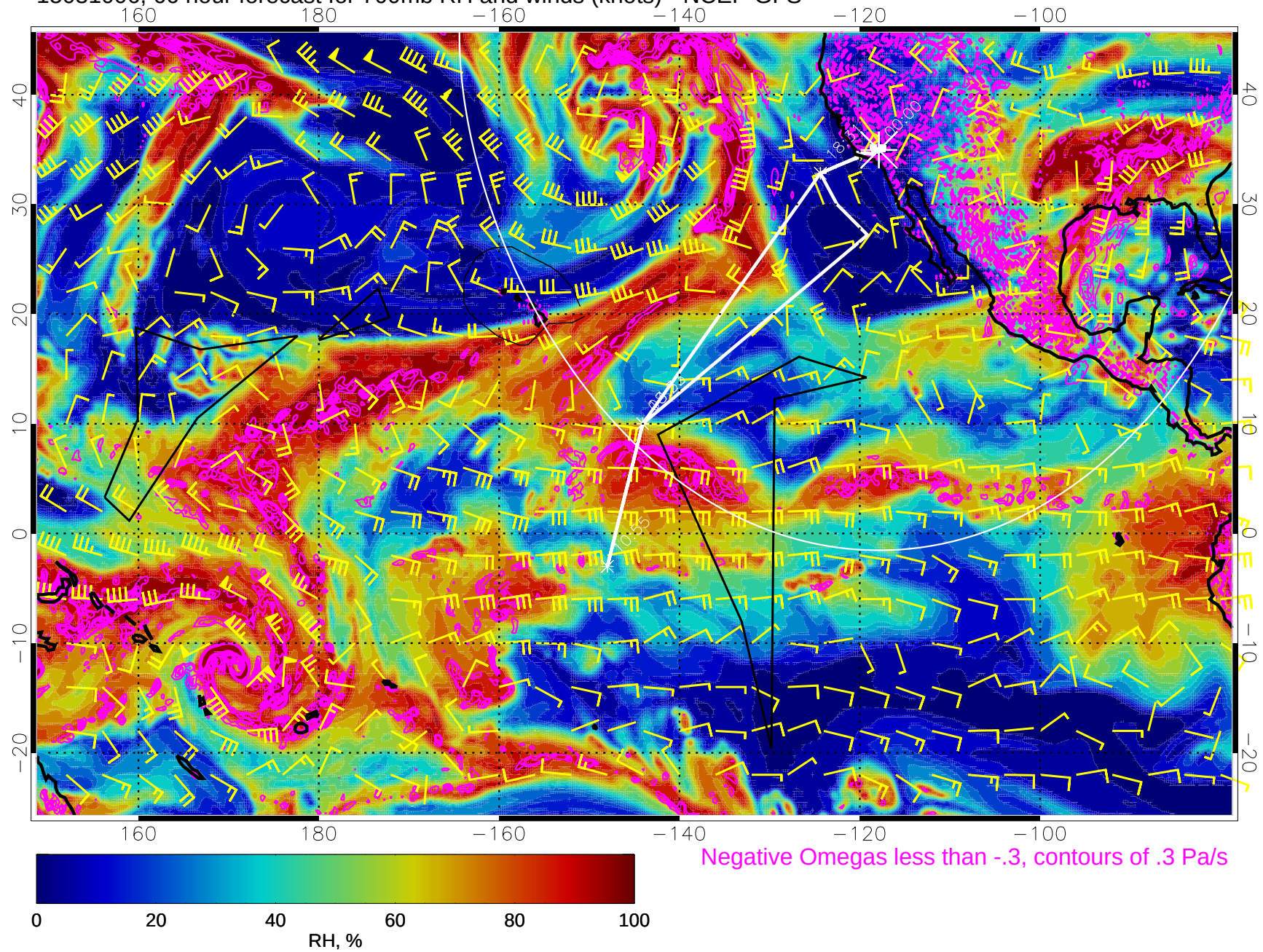
15031006, 66 hour forecast for 700mb RH and winds (knots) - NCEP GFS
