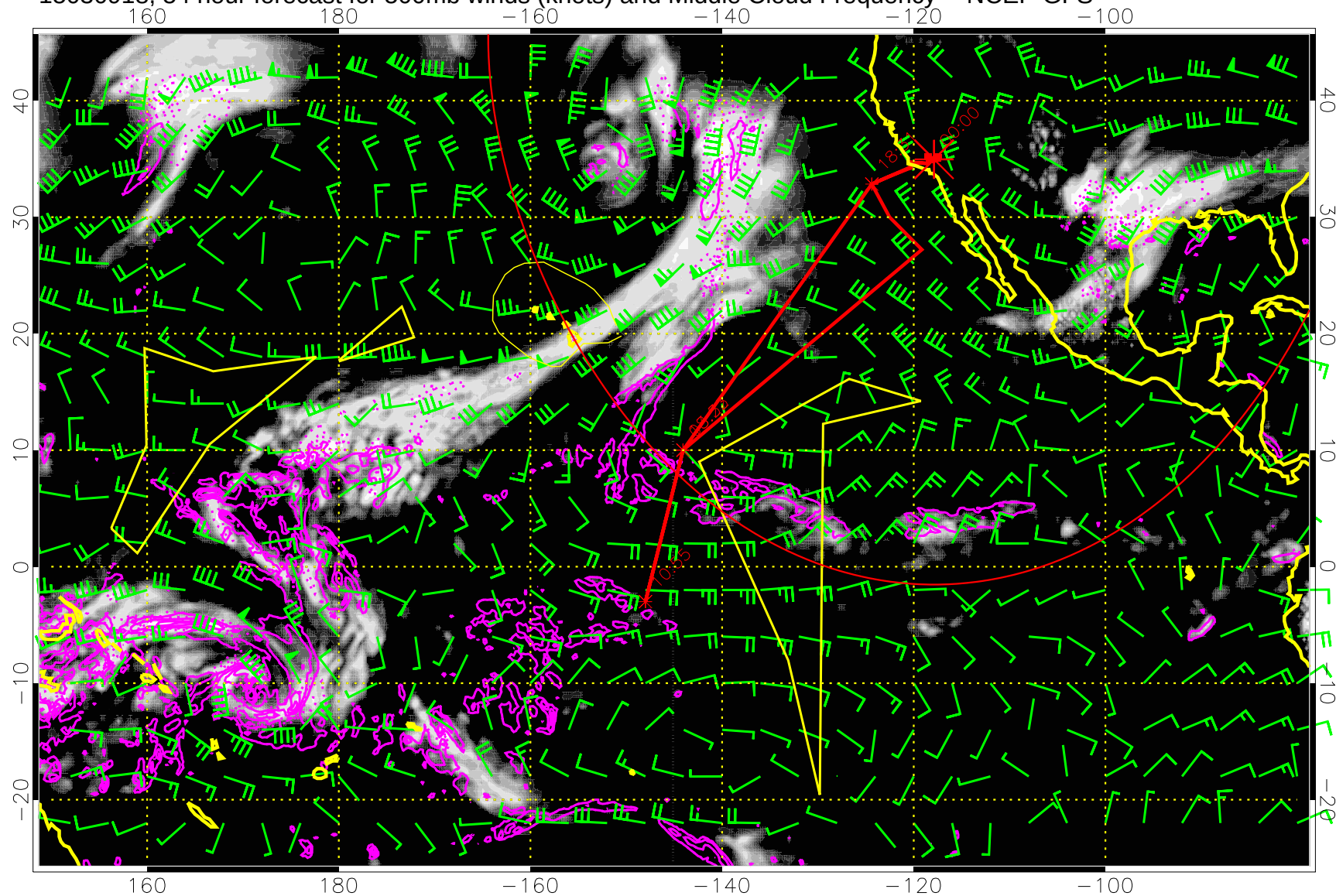
15030918, 54 hour forecast for 500mb winds (knots) and Middle Cloud Frequency -- NCEP GFS
