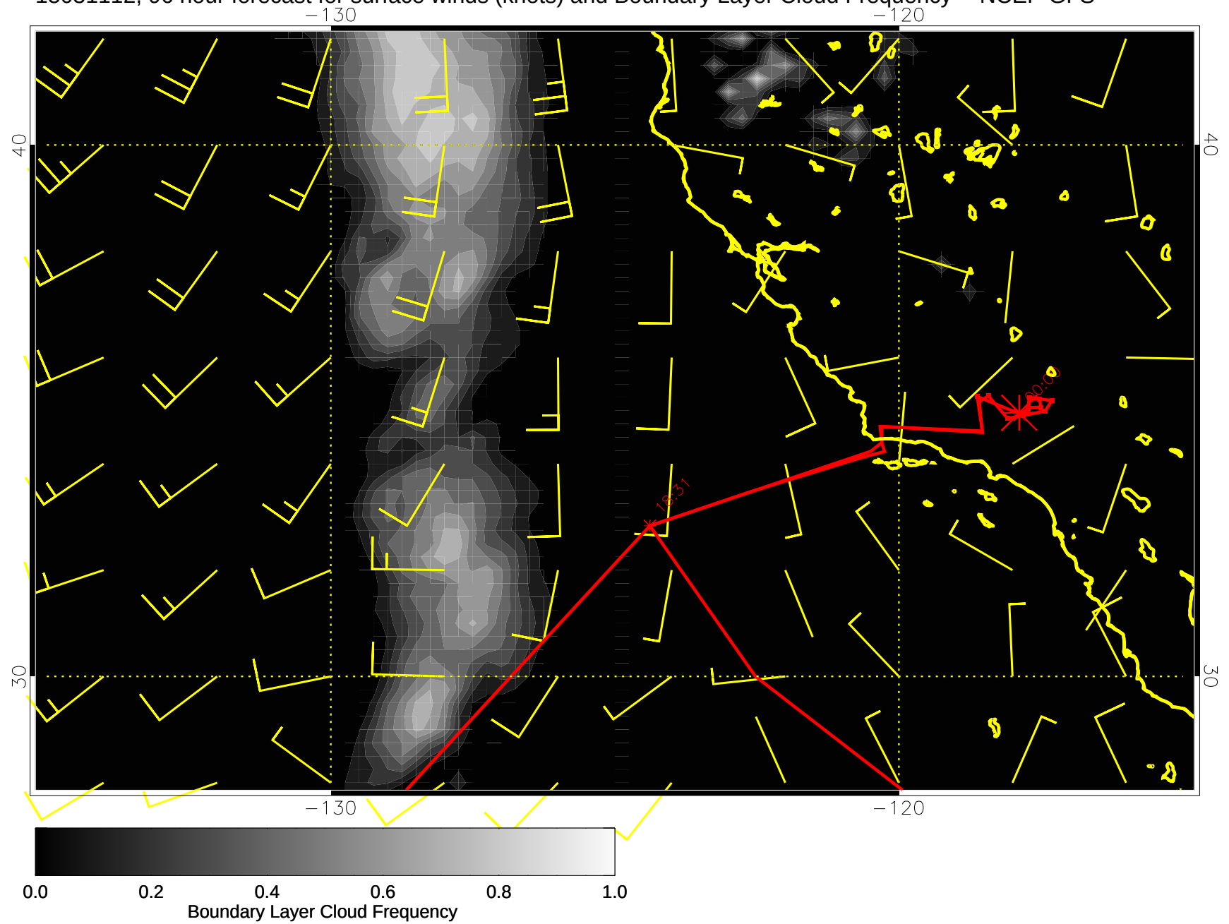
15031112, 96 hour forecast for surface winds (knots) and Boundary Layer Cloud Frequency -- NCEP GFS
