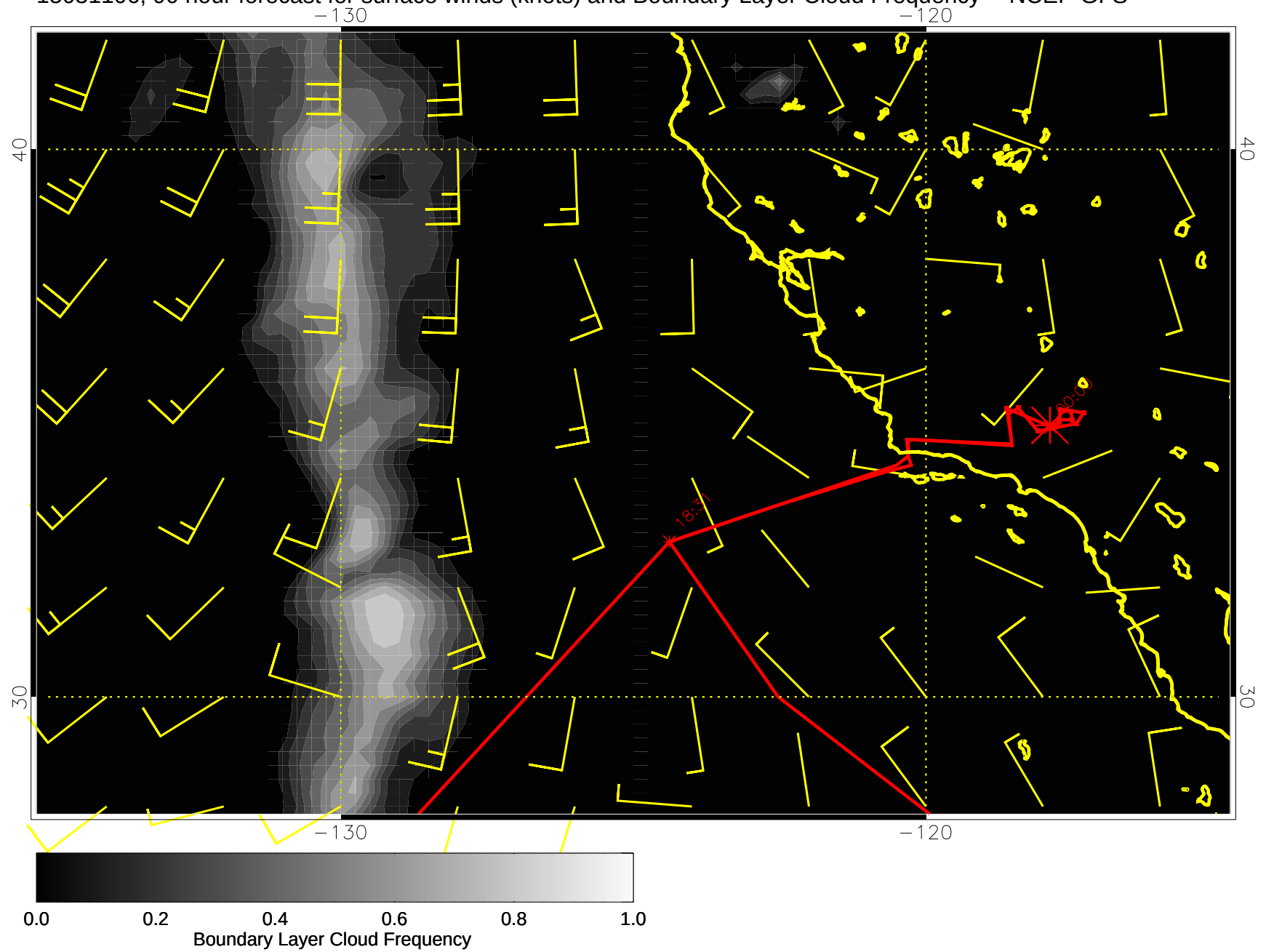
15031106, 90 hour forecast for surface winds (knots) and Boundary Layer Cloud Frequency -- NCEP GFS
