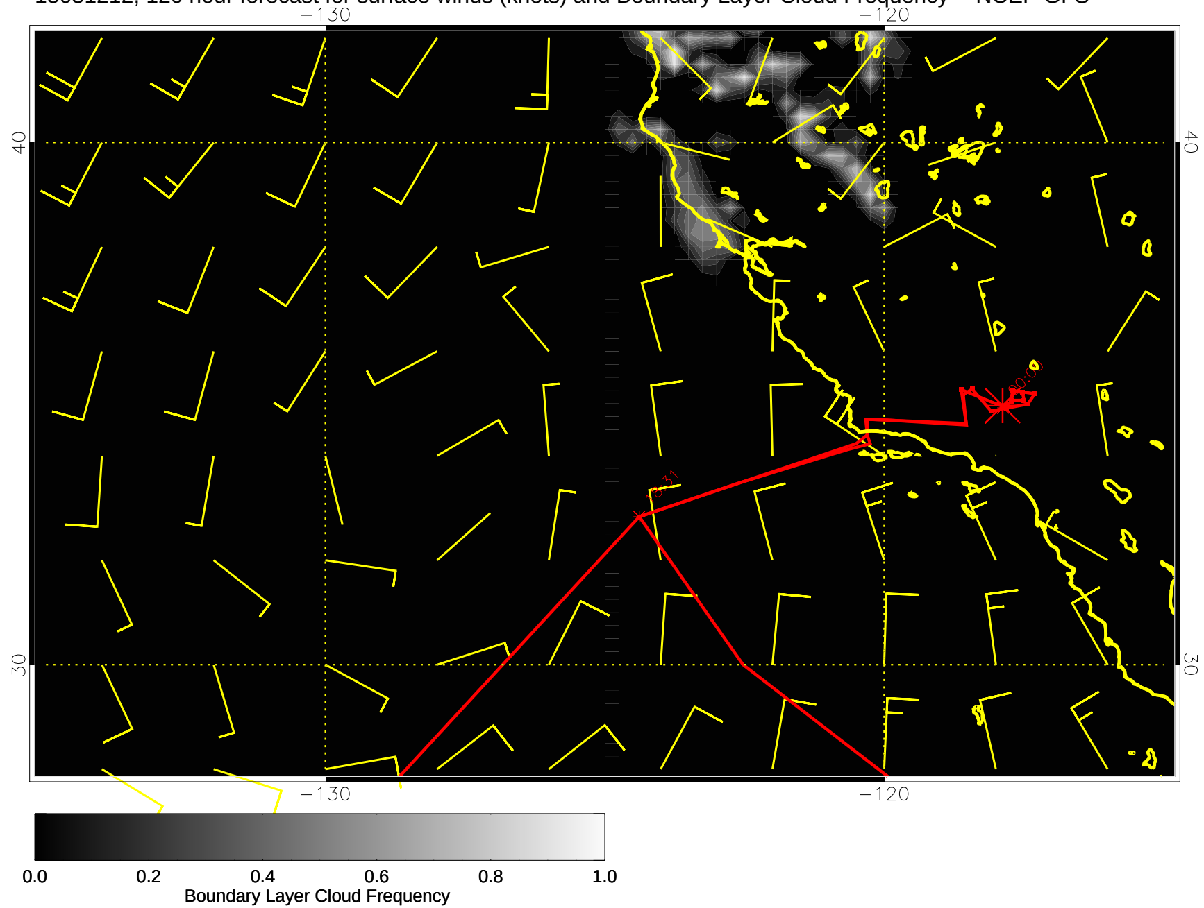
15031212, 120 hour forecast for surface winds (knots) and Boundary Layer Cloud Frequency -- NCEP GFS
