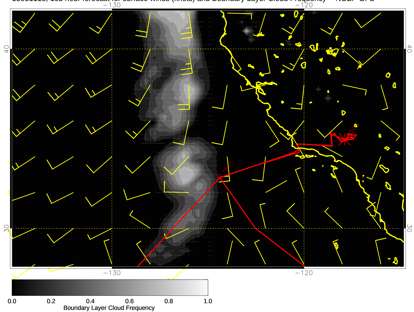
15031118, 102 hour forecast for surface winds (knots) and Boundary Layer Cloud Frequency -- NCEP GFS
