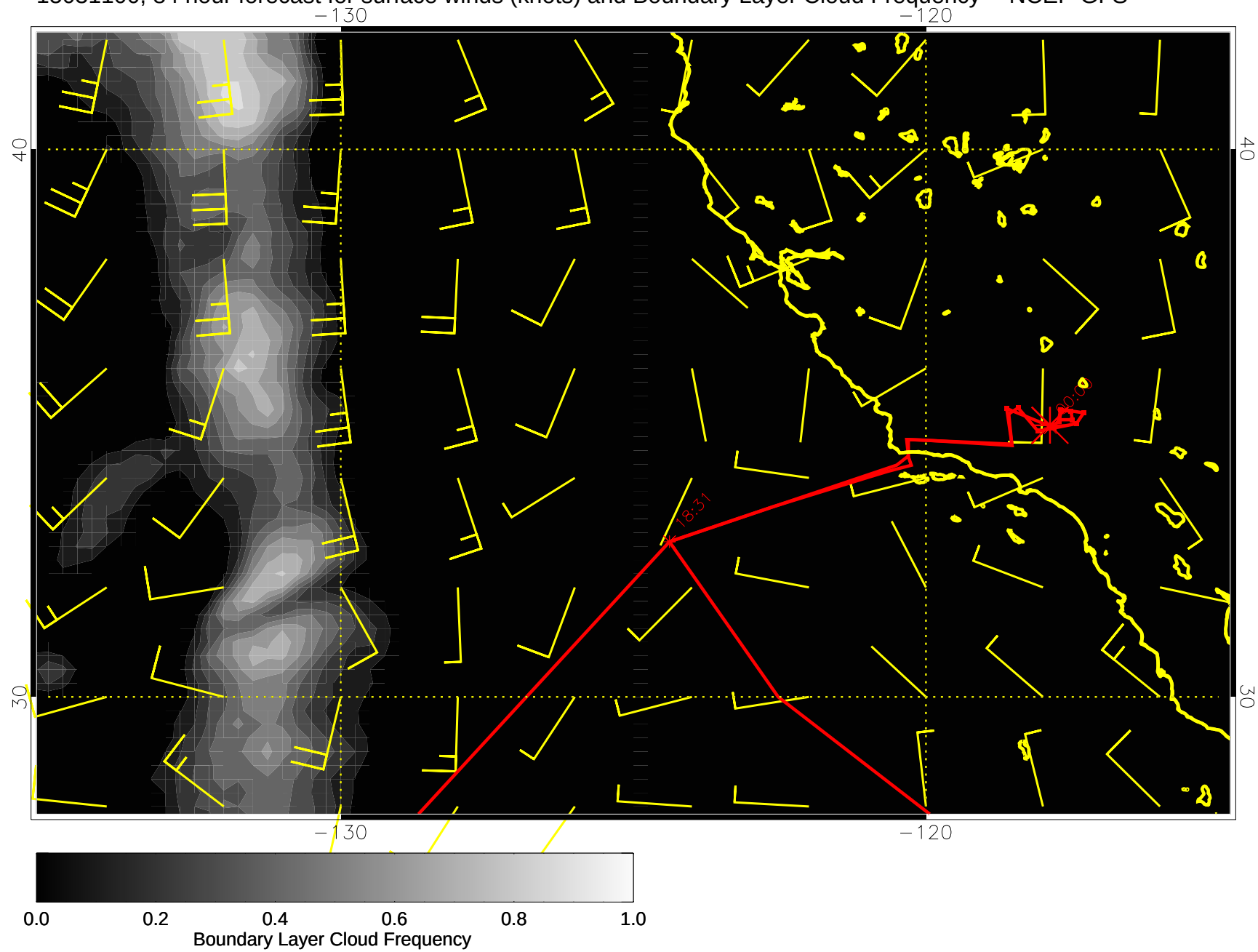
15031100, 84 hour forecast for surface winds (knots) and Boundary Layer Cloud Frequency -- NCEP GFS
