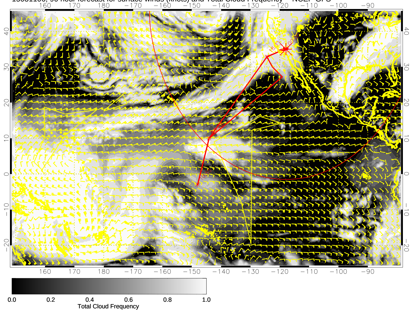
15031106, 90 hour forecast for surface winds (knots) and Total Cloud Frequency -- NCEP GFS
