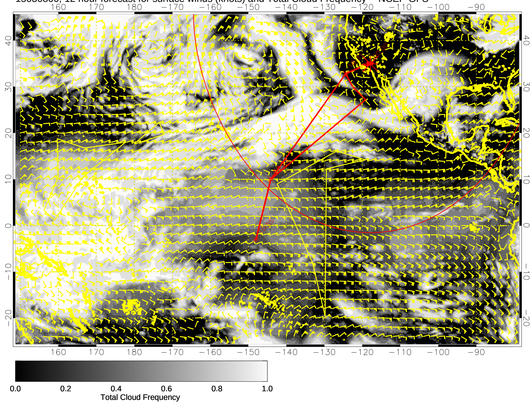
15030800, 12 hour forecast for surface winds (knots) and Total Cloud Frequency -- NCEP GFS
