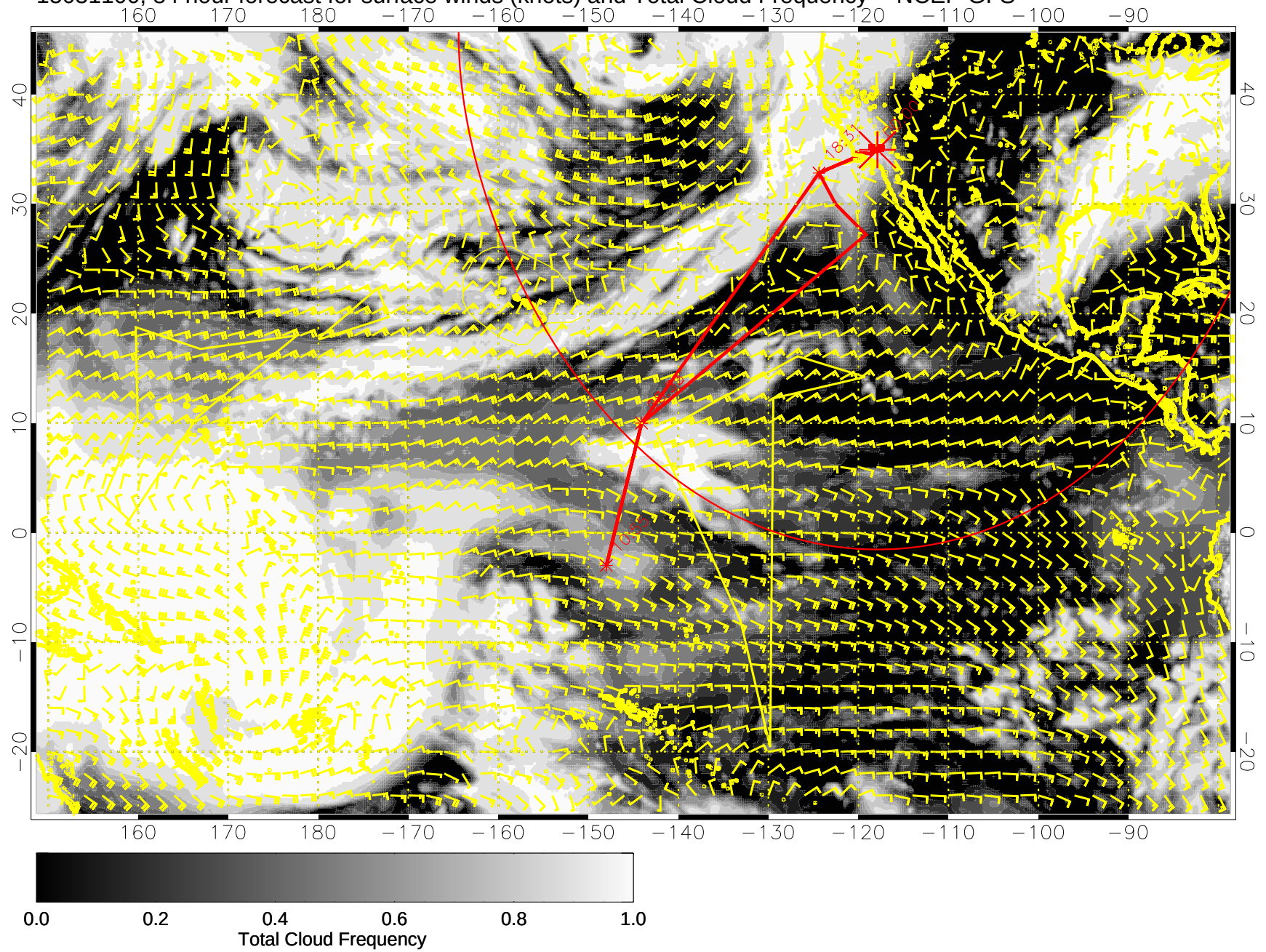
15031100, 84 hour forecast for surface winds (knots) and Total Cloud Frequency -- NCEP GFS
