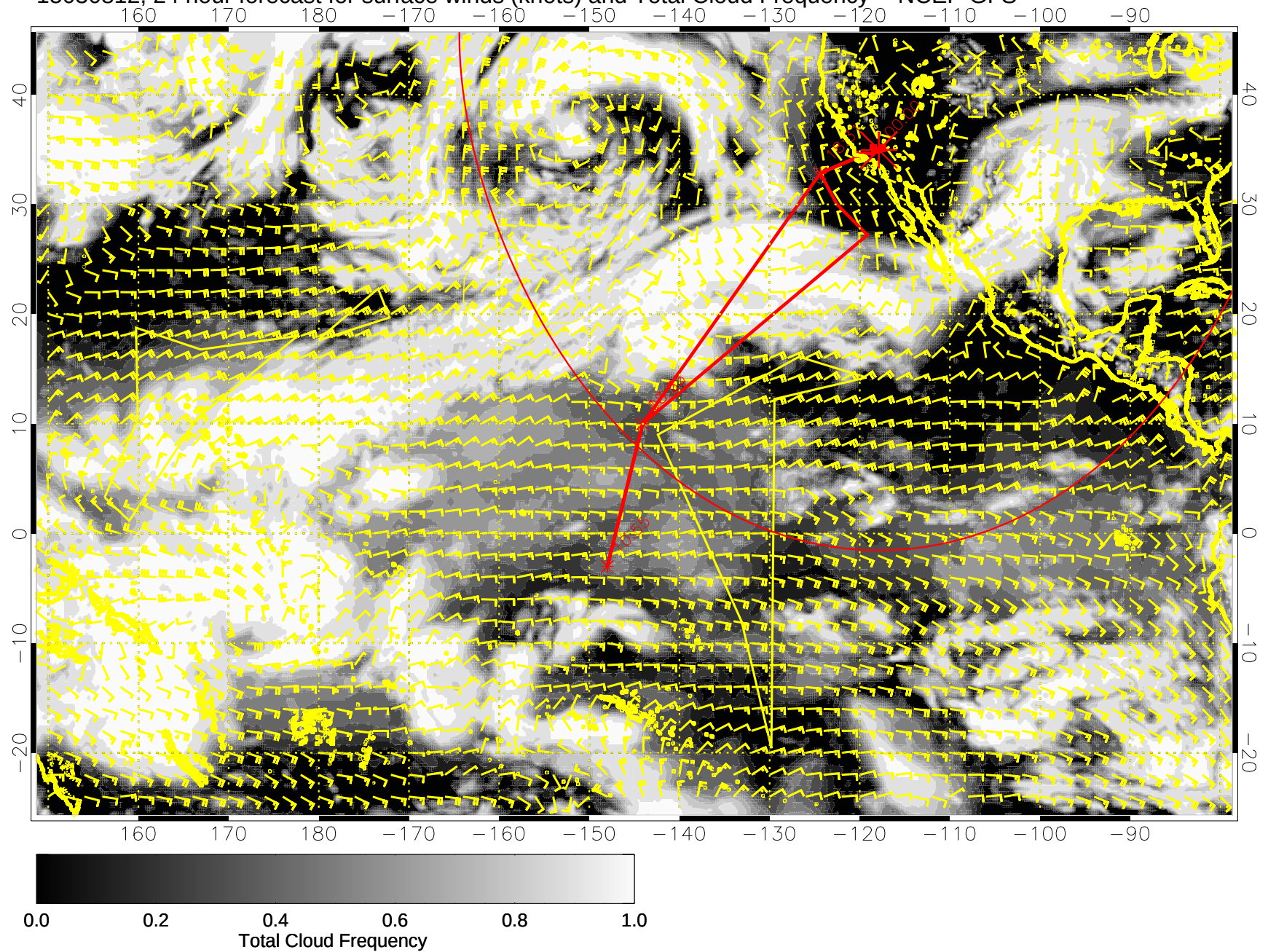
15030812, 24 hour forecast for surface winds (knots) and Total Cloud Frequency -- NCEP GFS
