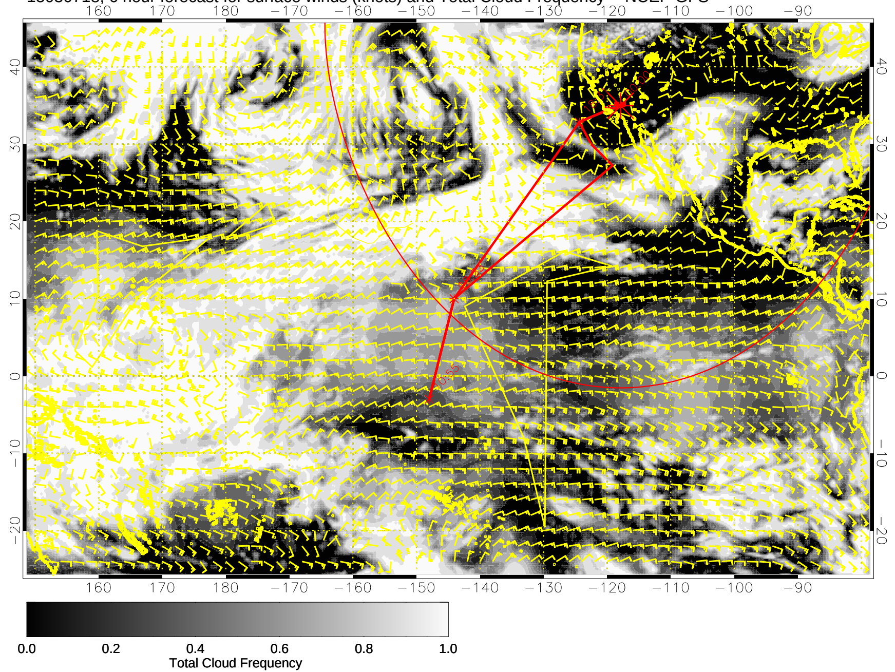
15030718, 6 hour forecast for surface winds (knots) and Total Cloud Frequency -- NCEP GFS
