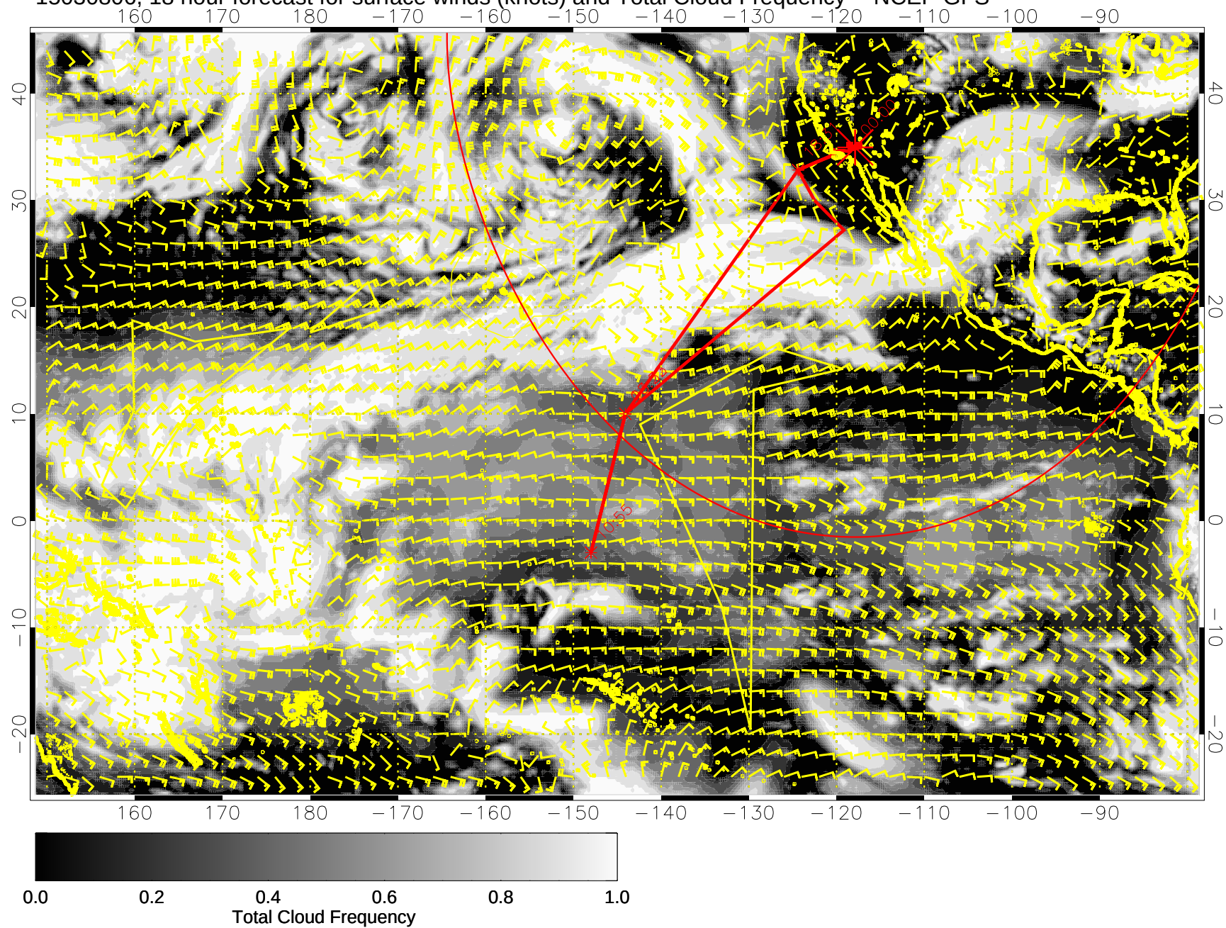
15030806, 18 hour forecast for surface winds (knots) and Total Cloud Frequency -- NCEP GFS
