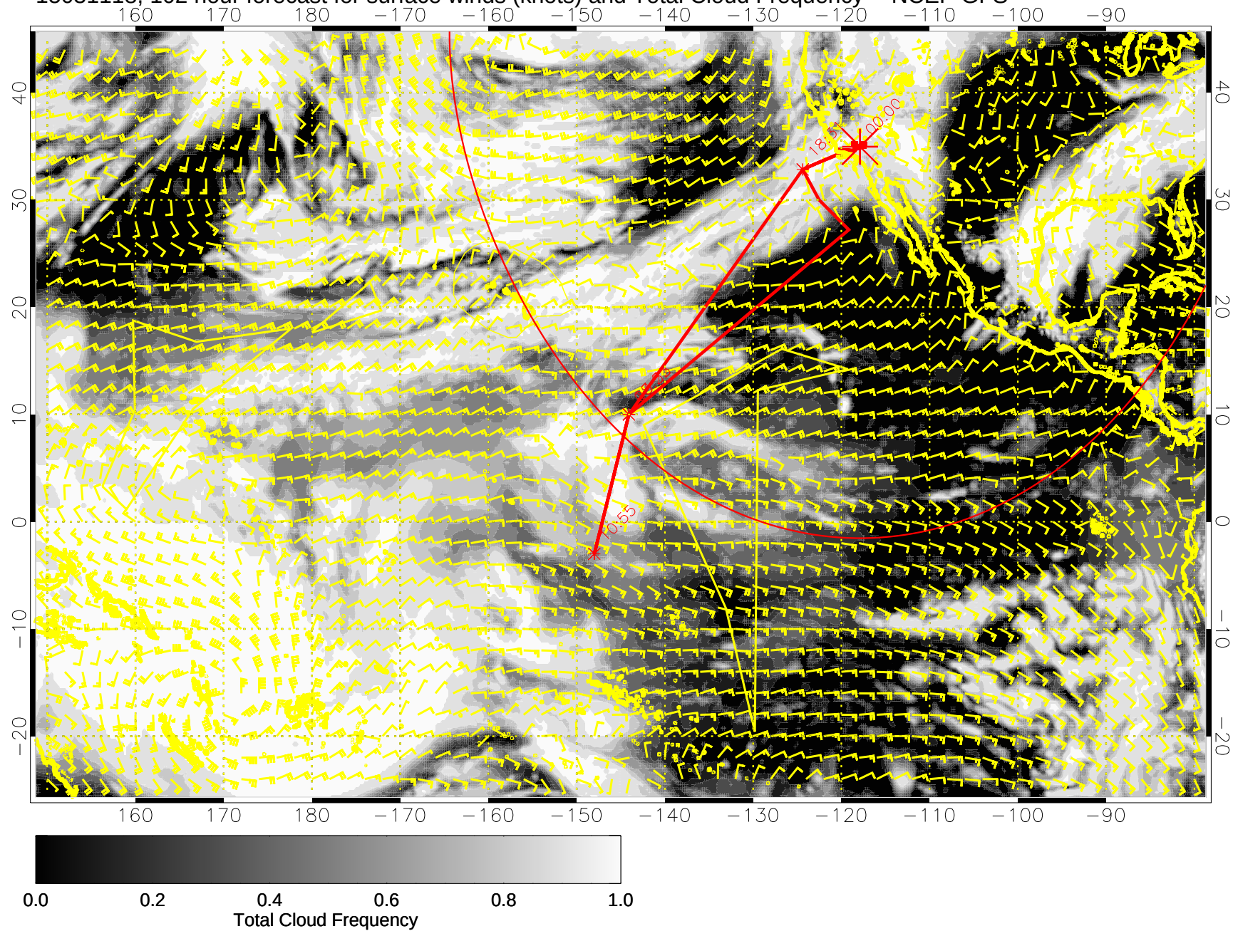
15031118, 102 hour forecast for surface winds (knots) and Total Cloud Frequency -- NCEP GFS
