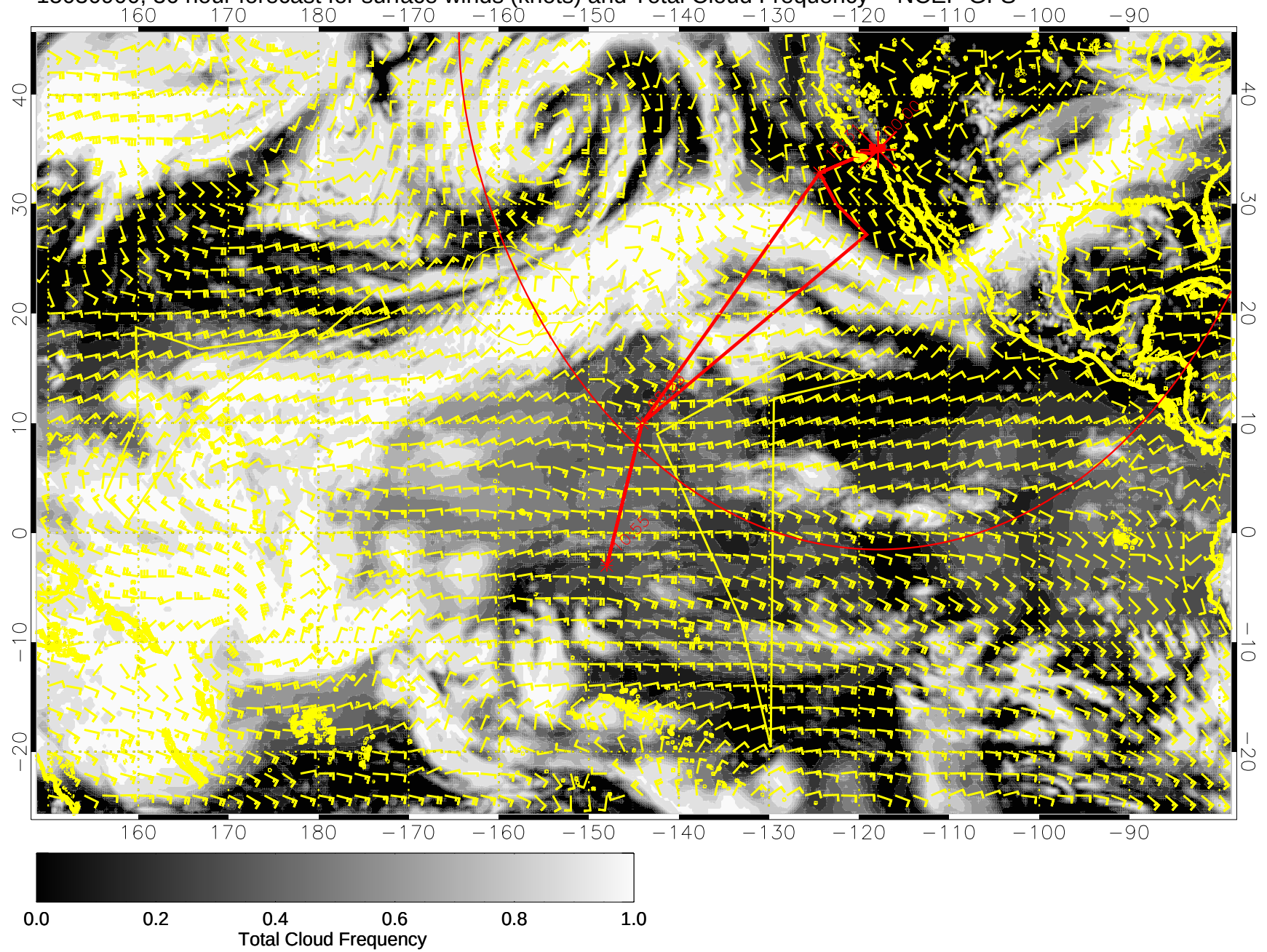
15030900, 36 hour forecast for surface winds (knots) and Total Cloud Frequency -- NCEP GFS
