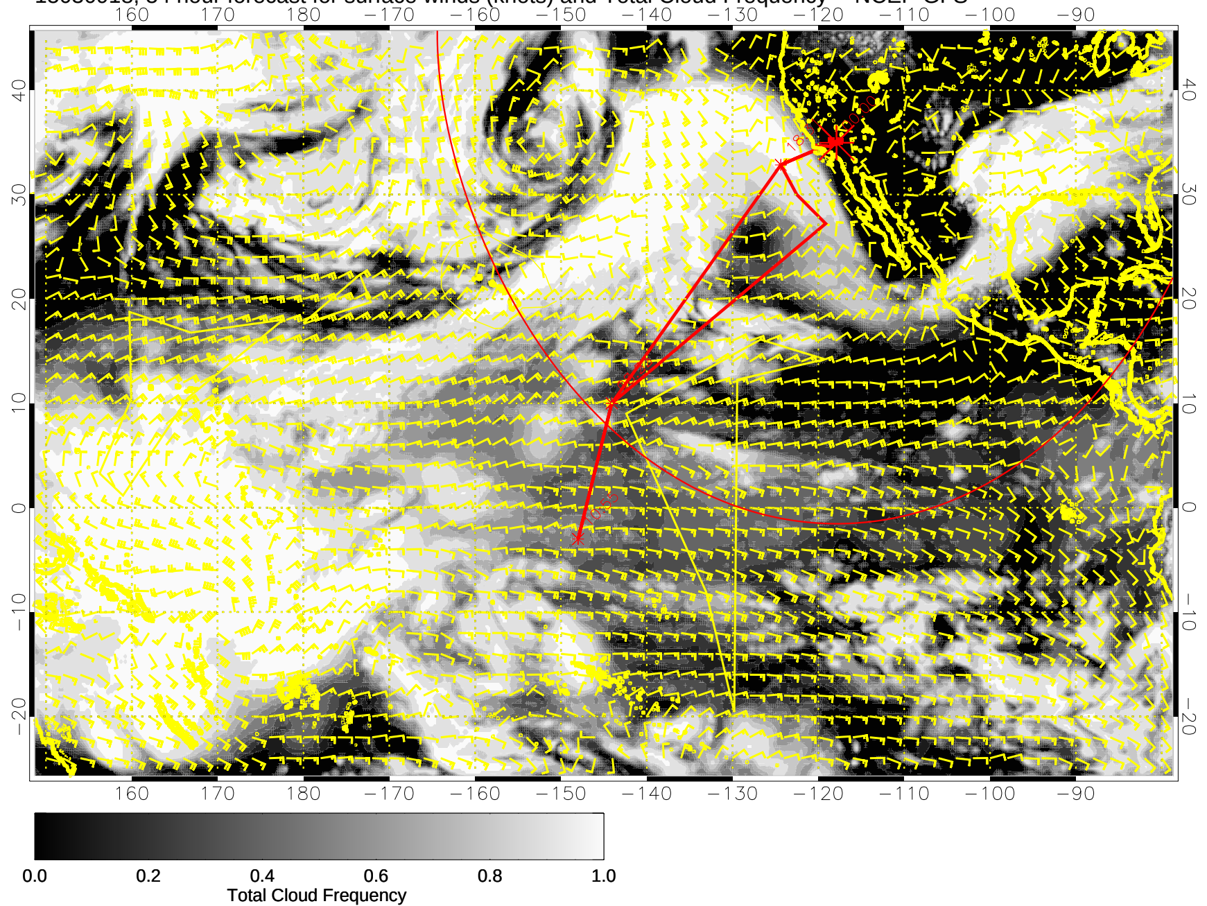
15030918, 54 hour forecast for surface winds (knots) and Total Cloud Frequency -- NCEP GFS
