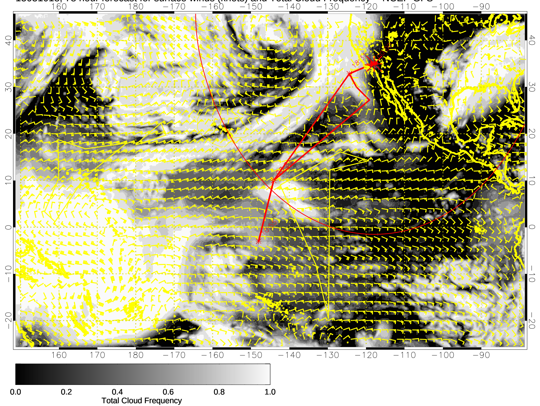
15031018, 78 hour forecast for surface winds (knots) and Total Cloud Frequency -- NCEP GFS
