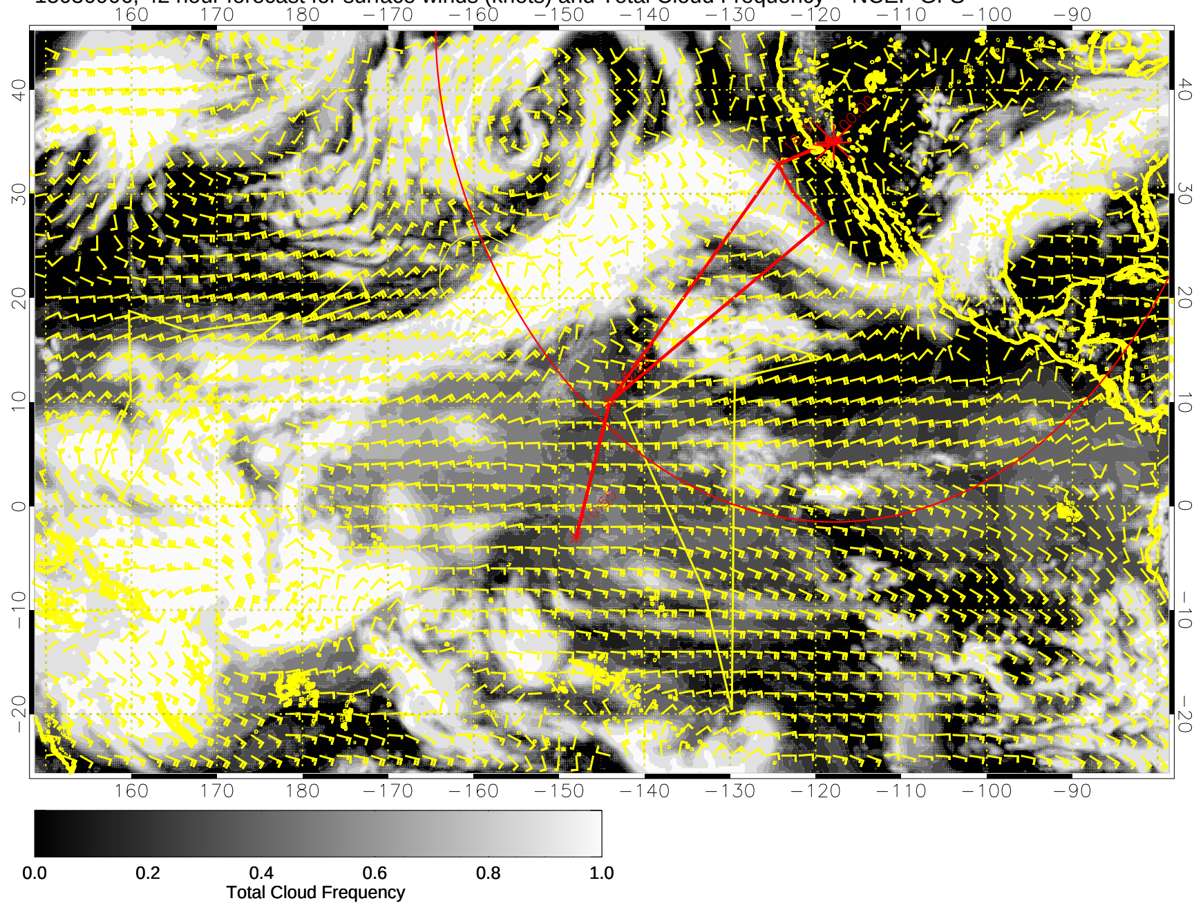
15030906, 42 hour forecast for surface winds (knots) and Total Cloud Frequency -- NCEP GFS
