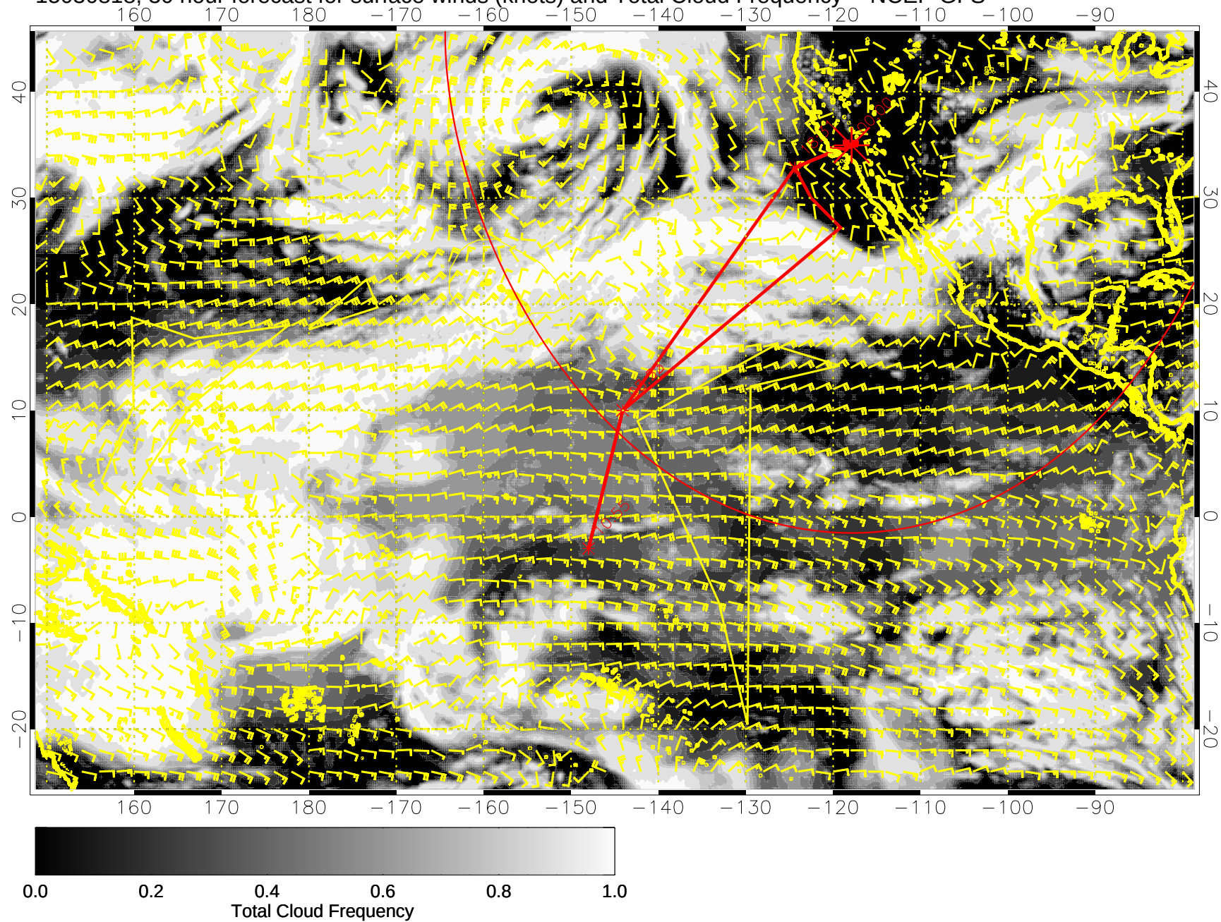
15030818, 30 hour forecast for surface winds (knots) and Total Cloud Frequency -- NCEP GFS
