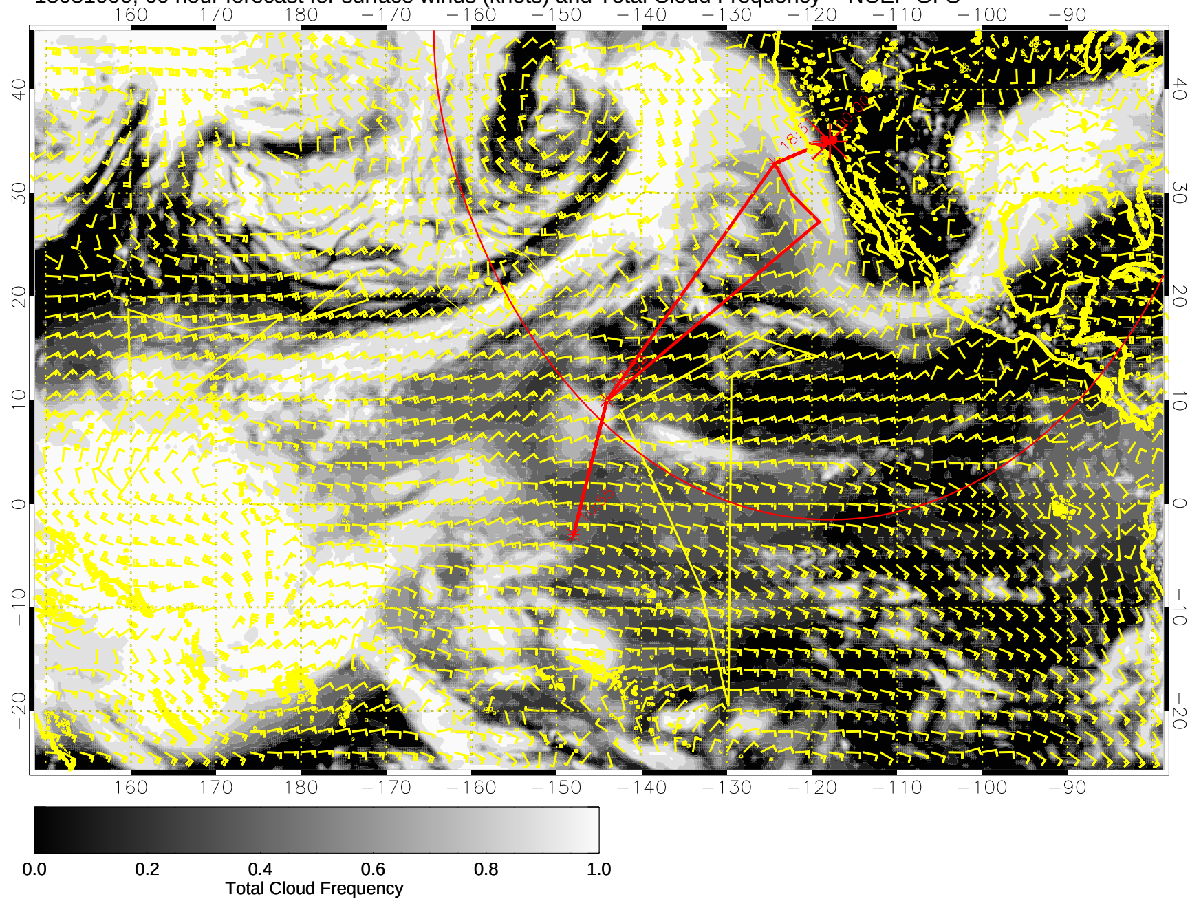
15031000, 60 hour forecast for surface winds (knots) and Total Cloud Frequency -- NCEP GFS
