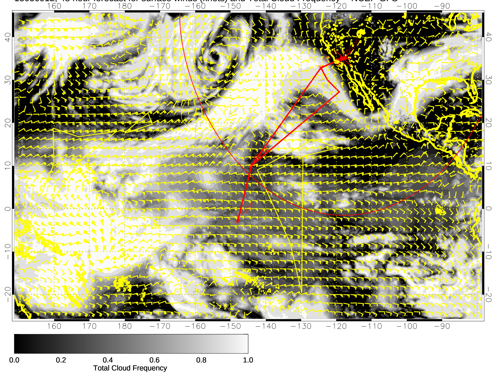
15030912, 48 hour forecast for surface winds (knots) and Total Cloud Frequency -- NCEP GFS
