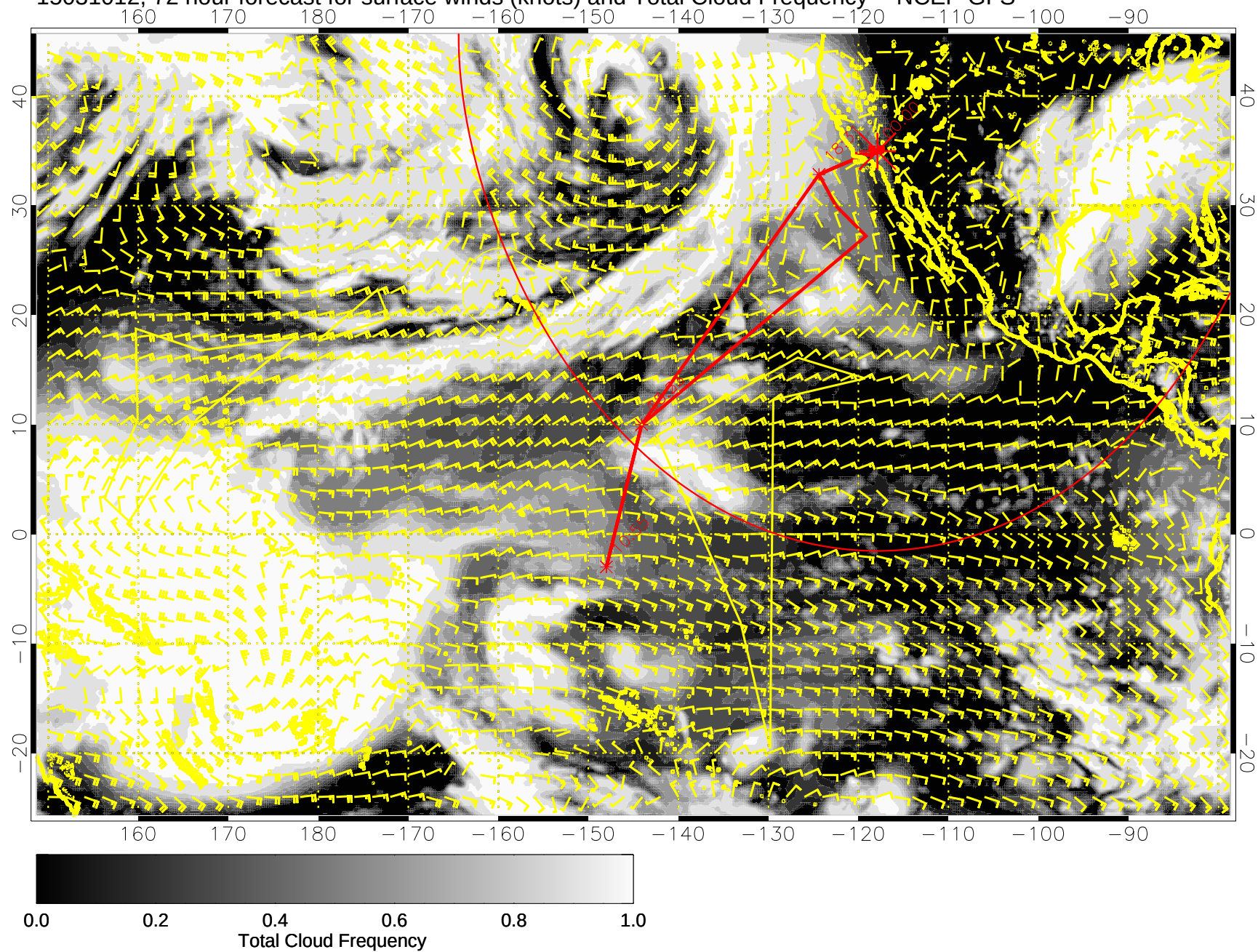
15031012, 72 hour forecast for surface winds (knots) and Total Cloud Frequency -- NCEP GFS
