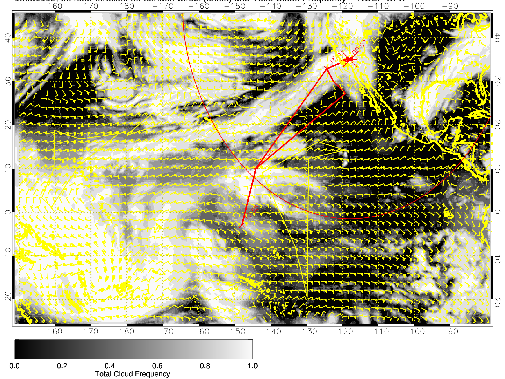
15031112, 96 hour forecast for surface winds (knots) and Total Cloud Frequency -- NCEP GFS
