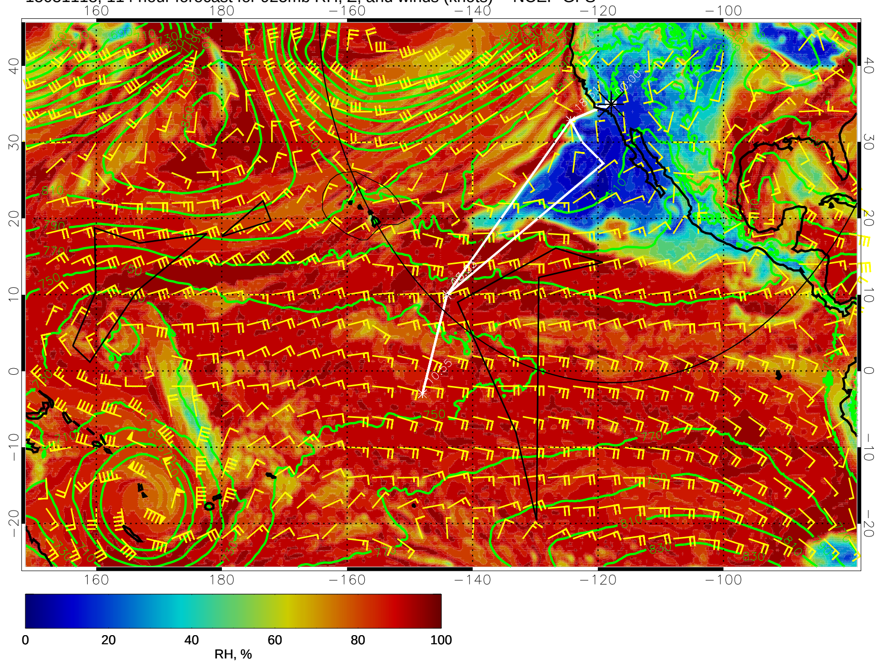
15031118, 114 hour forecast for 925mb RH, Z, and winds (knots) -- NCEP GFS
