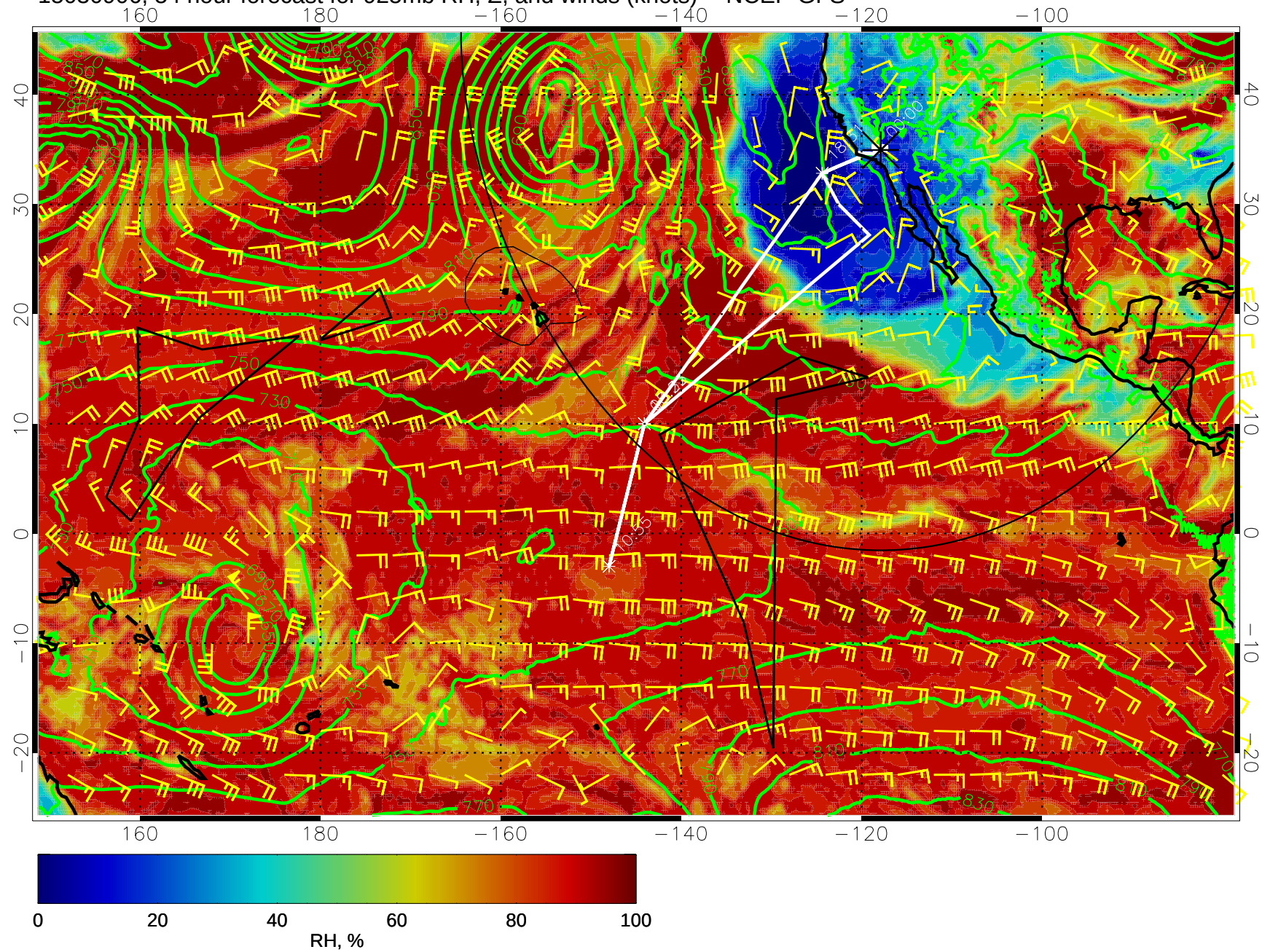
15030906, 54 hour forecast for 925mb RH, Z, and winds (knots) -- NCEP GFS
