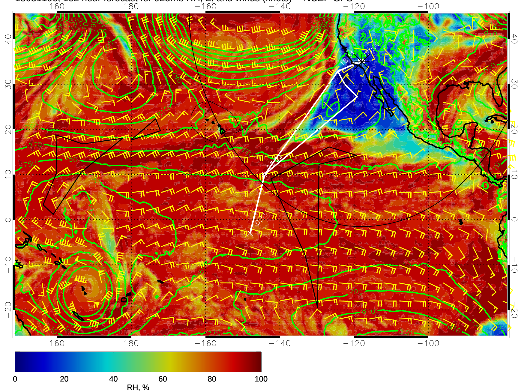
15031106, 102 hour forecast for 925mb RH, Z, and winds (knots) -- NCEP GFS
