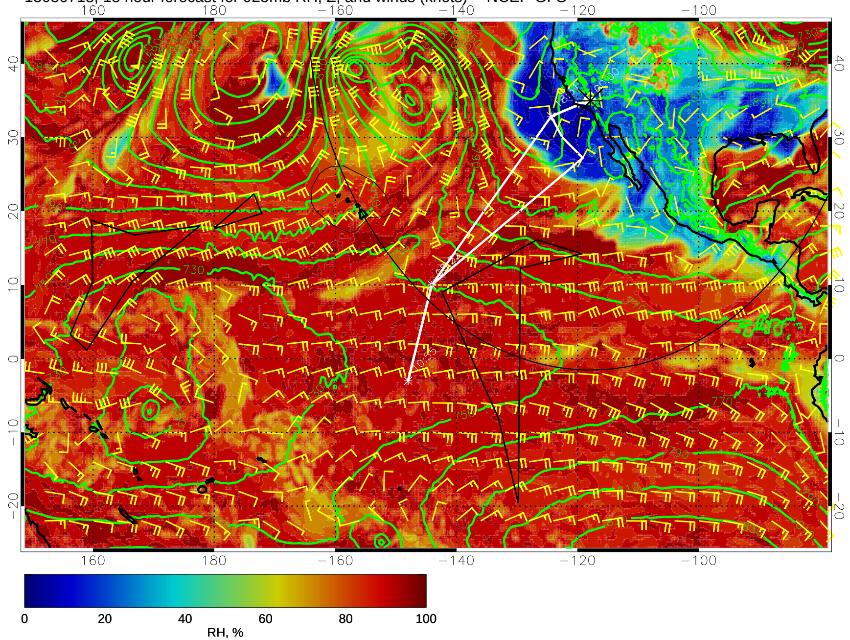
15030718, 18 hour forecast for 925mb RH, Z, and winds (knots) -- NCEP GFS
