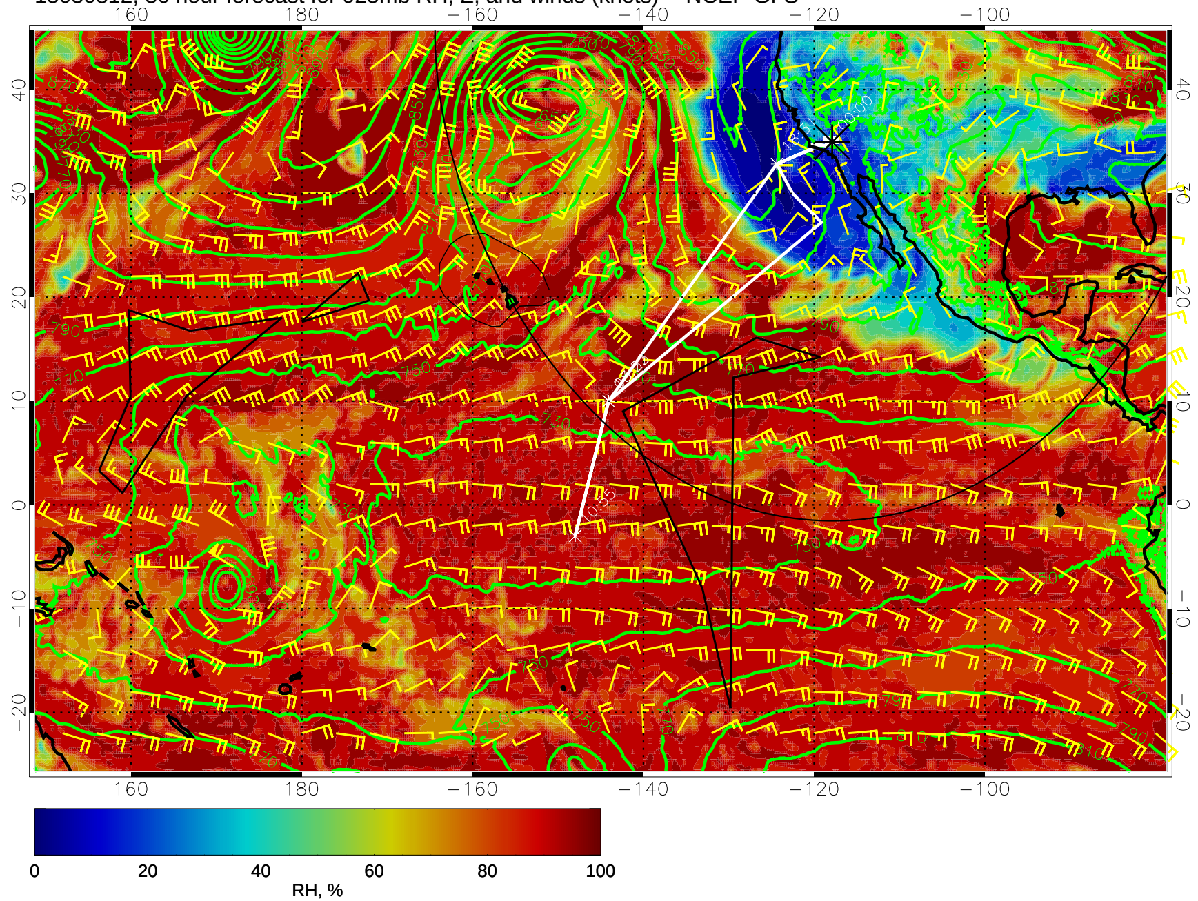
15030812, 36 hour forecast for 925mb RH, Z, and winds (knots) -- NCEP GFS
