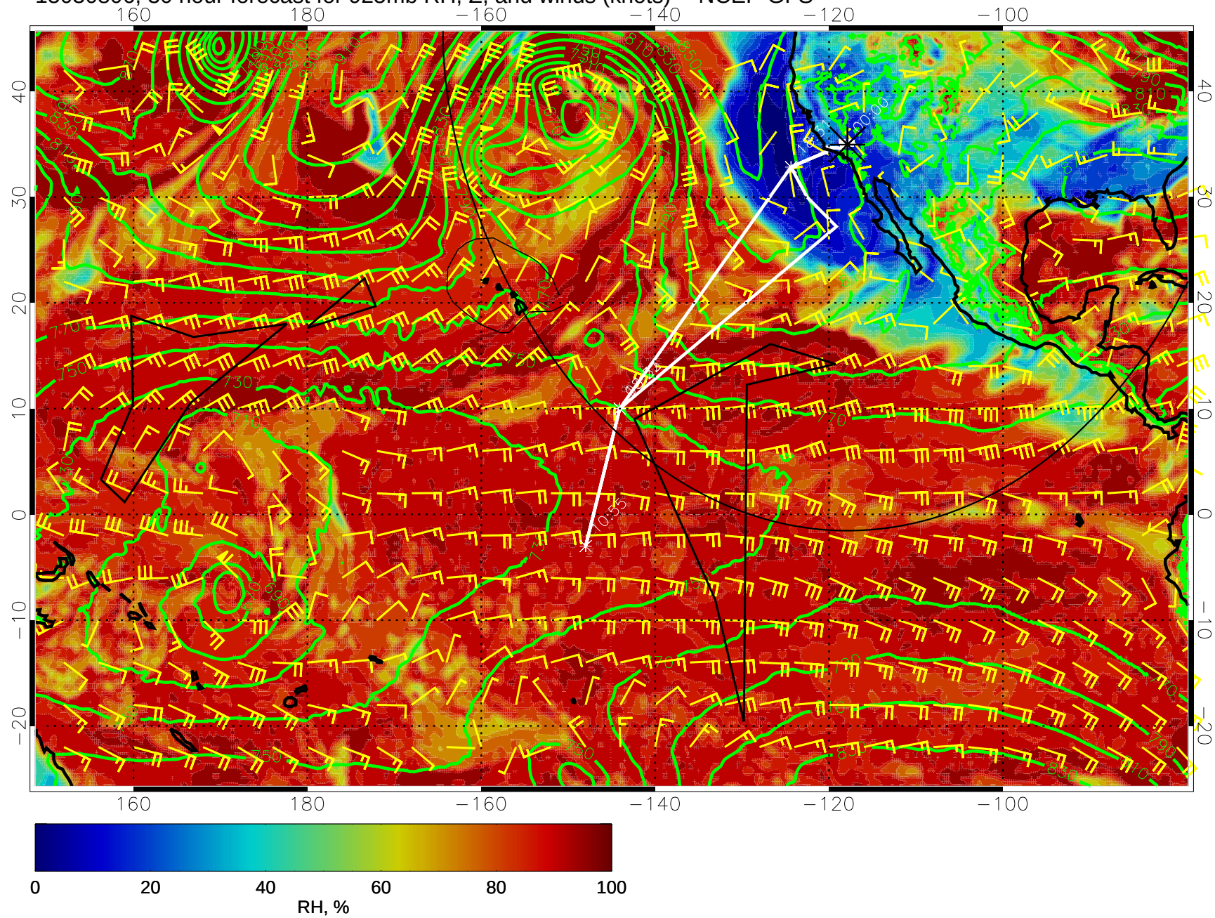
15030806, 30 hour forecast for 925mb RH, Z, and winds (knots) -- NCEP GFS
