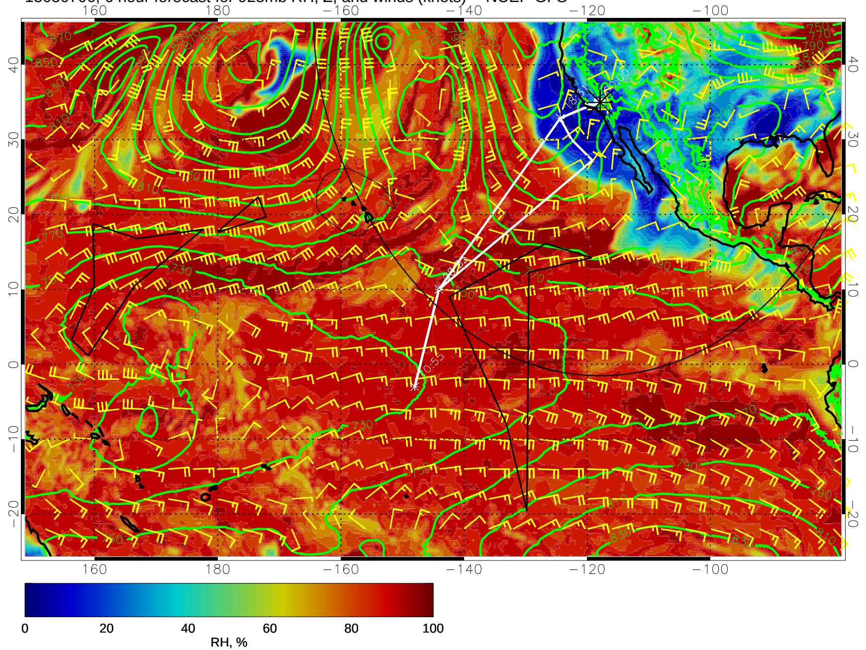
15030706, 6 hour forecast for 925mb RH, Z, and winds (knots) -- NCEP GFS
