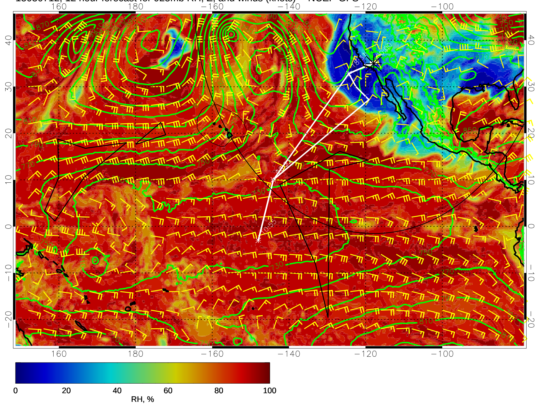
15030712, 12 hour forecast for 925mb RH, Z, and winds (knots) -- NCEP GFS
