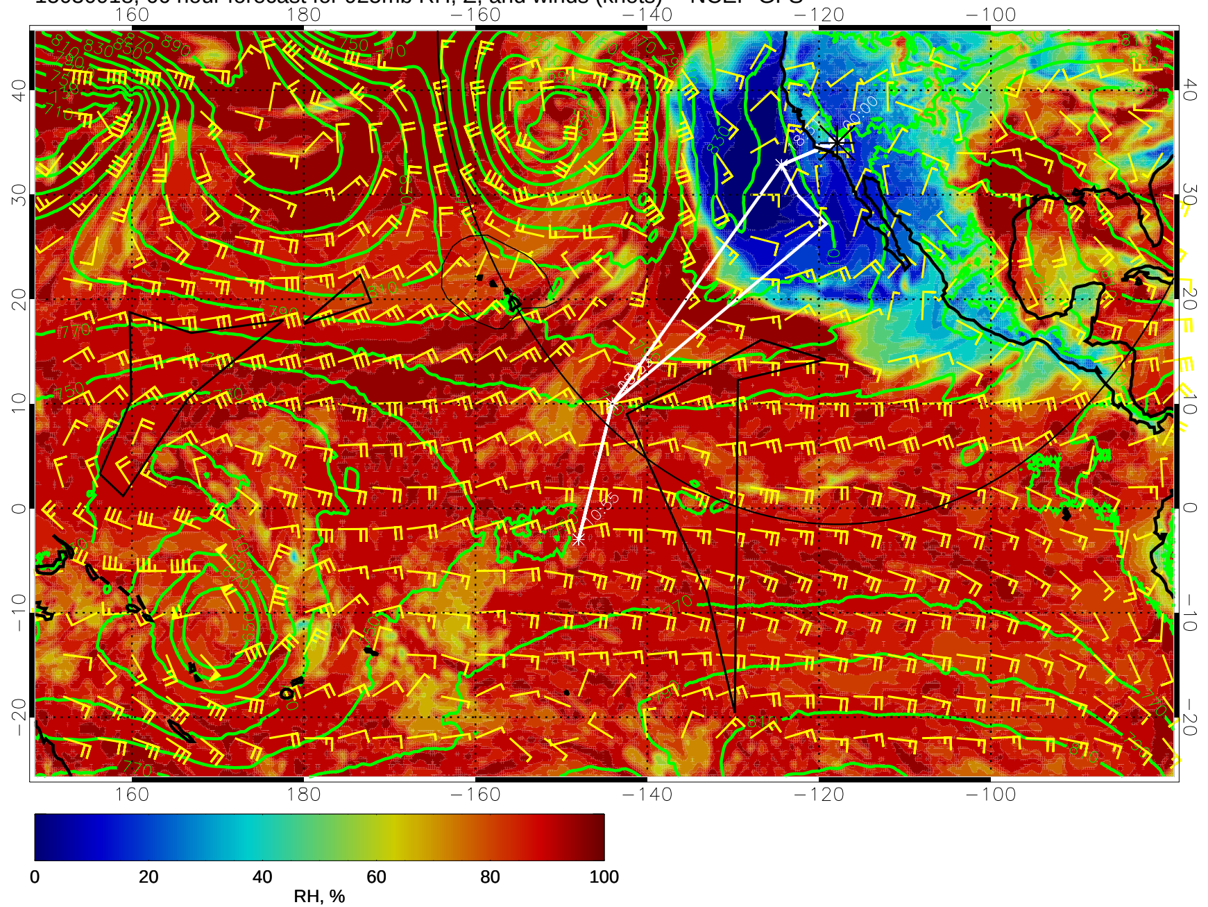
15030918, 66 hour forecast for 925mb RH, Z, and winds (knots) -- NCEP GFS
