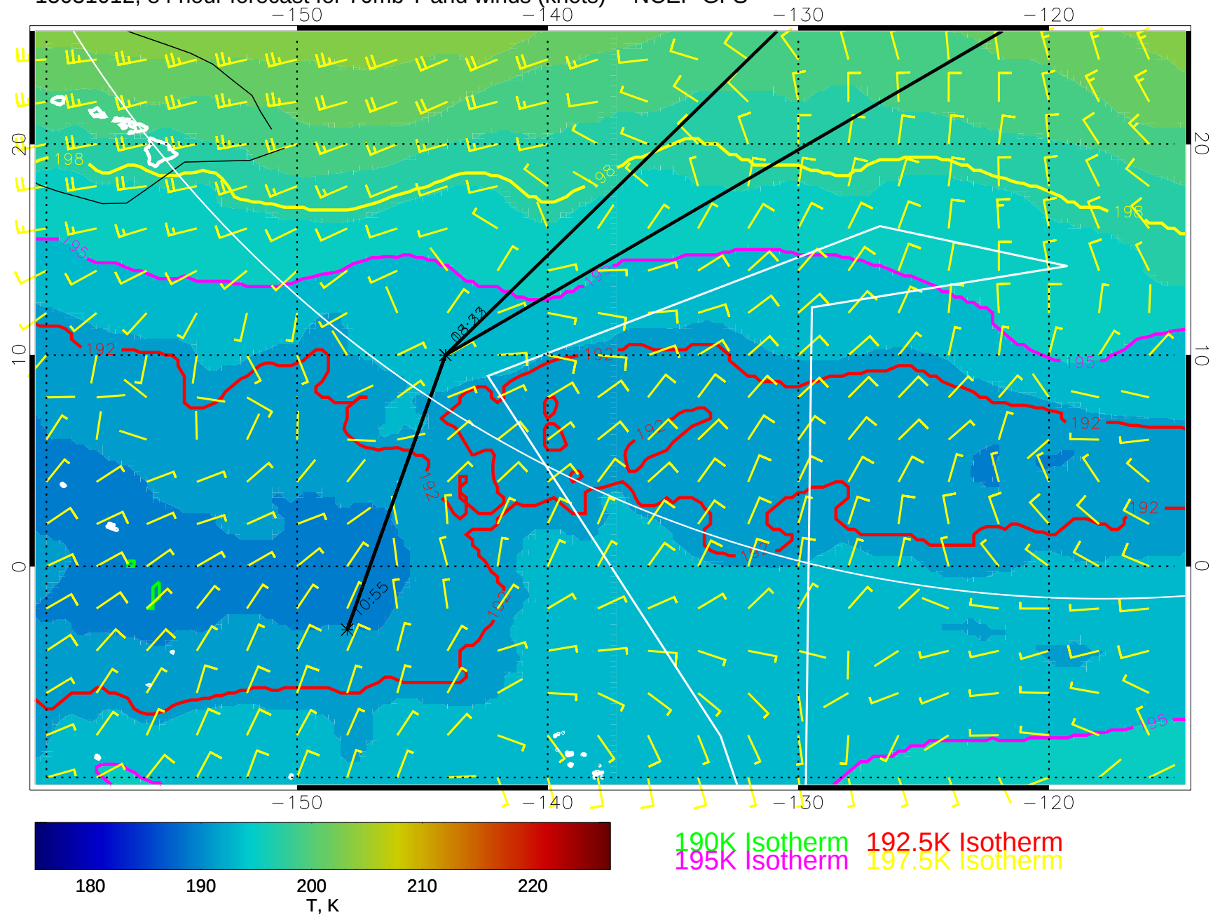
15031012, 84 hour forecast for 70mb T and winds (knots) -- NCEP GFS
