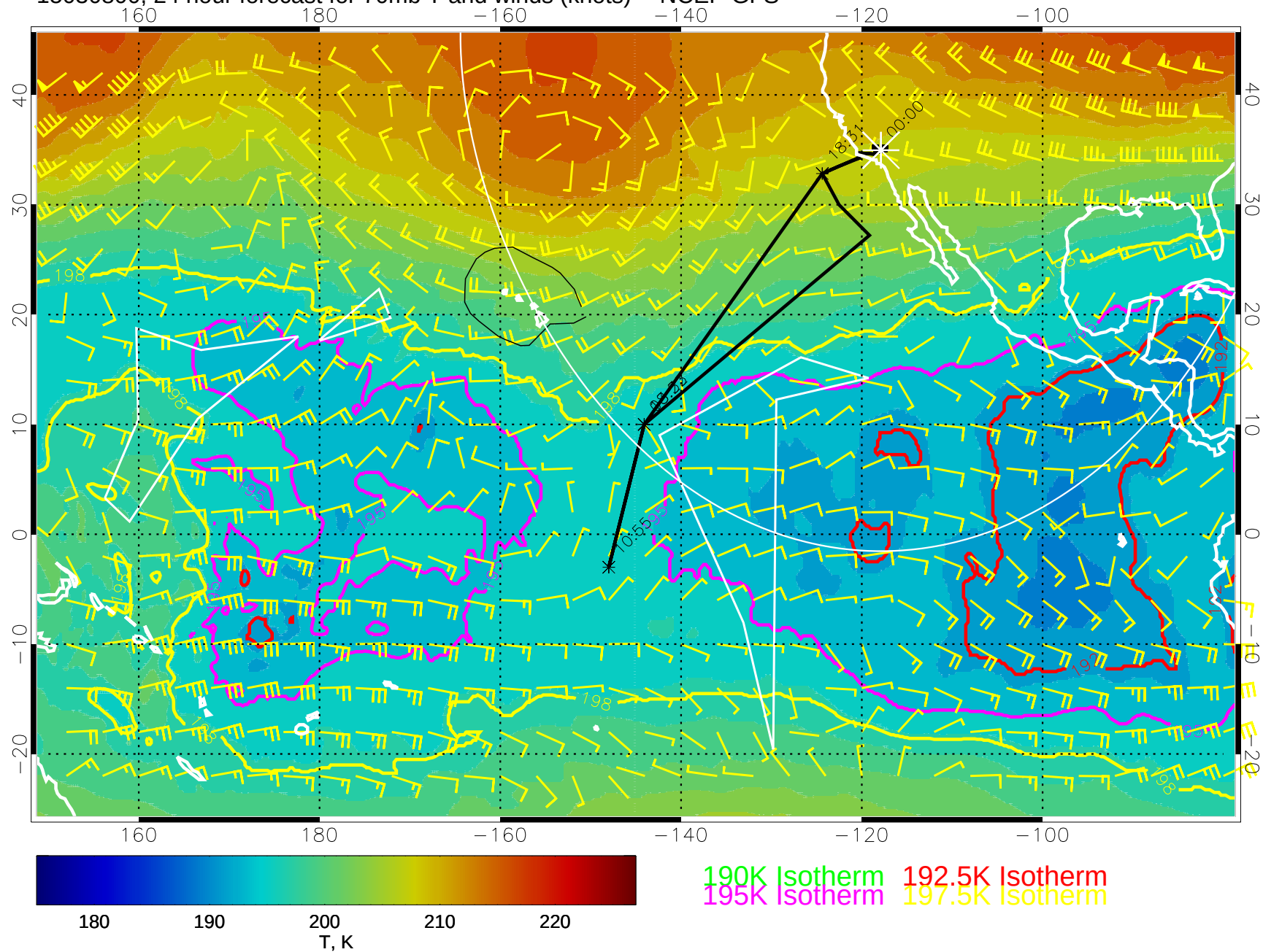
15030800, 24 hour forecast for 70mb T and winds (knots) -- NCEP GFS
