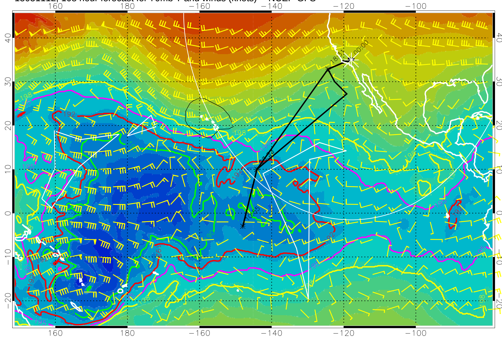
15031112, 108 hour forecast for 70mb T and winds (knots) -- NCEP GFS
