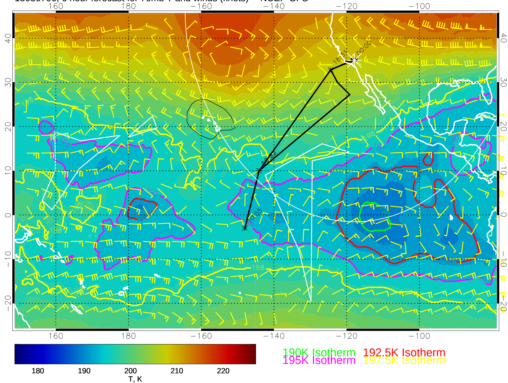
15030706, 6 hour forecast for 70mb T and winds (knots) -- NCEP GFS
