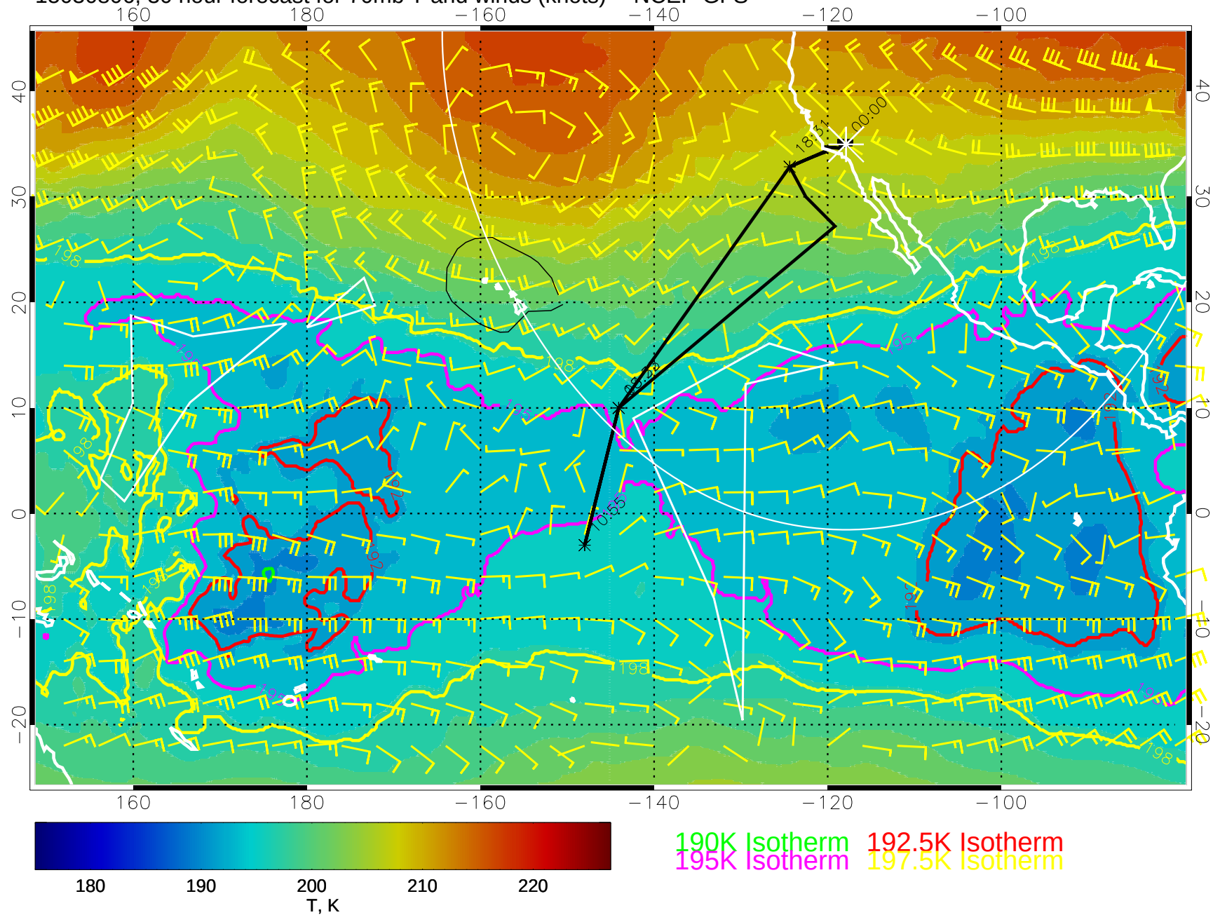
15030806, 30 hour forecast for 70mb T and winds (knots) -- NCEP GFS
