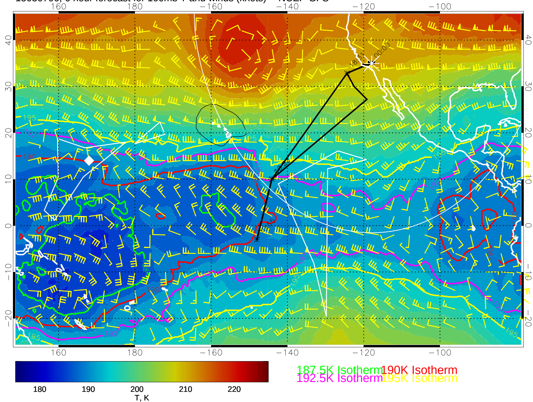
15030706, 6 hour forecast for 100mb T and winds (knots) -- NCEP GFS
