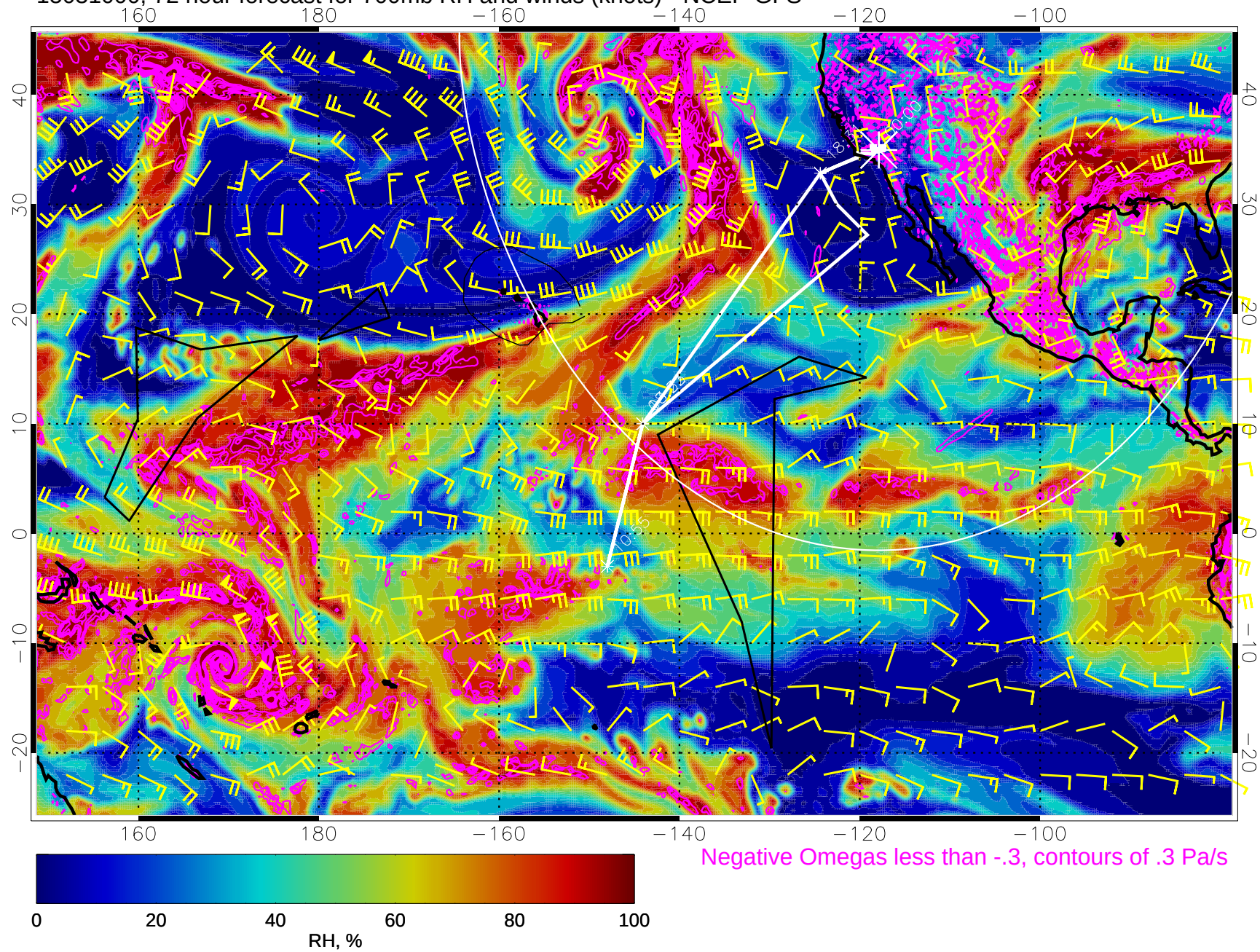
15031000, 72 hour forecast for 700mb RH and winds (knots) - NCEP GFS
