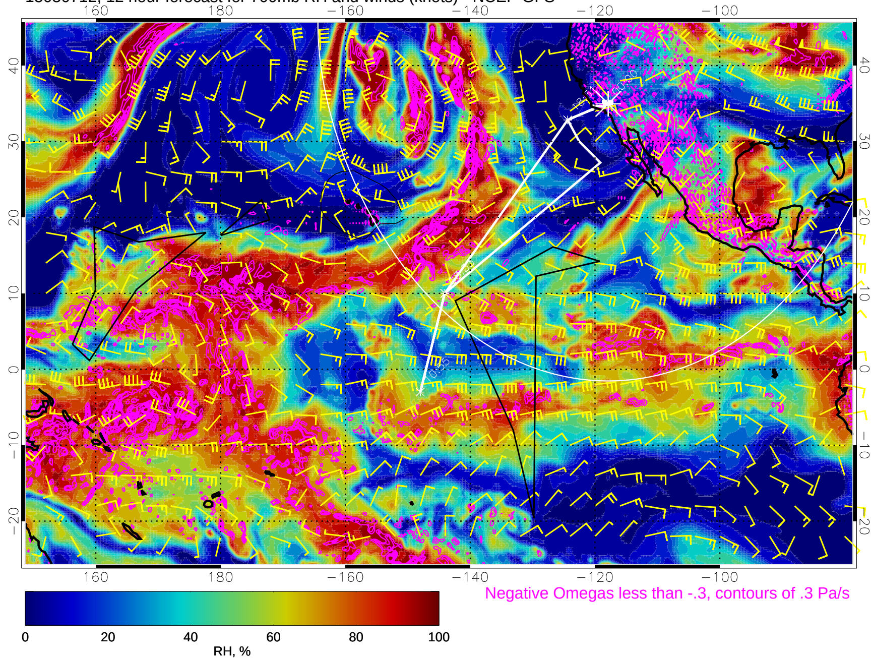
15030712, 12 hour forecast for 700mb RH and winds (knots) - NCEP GFS
