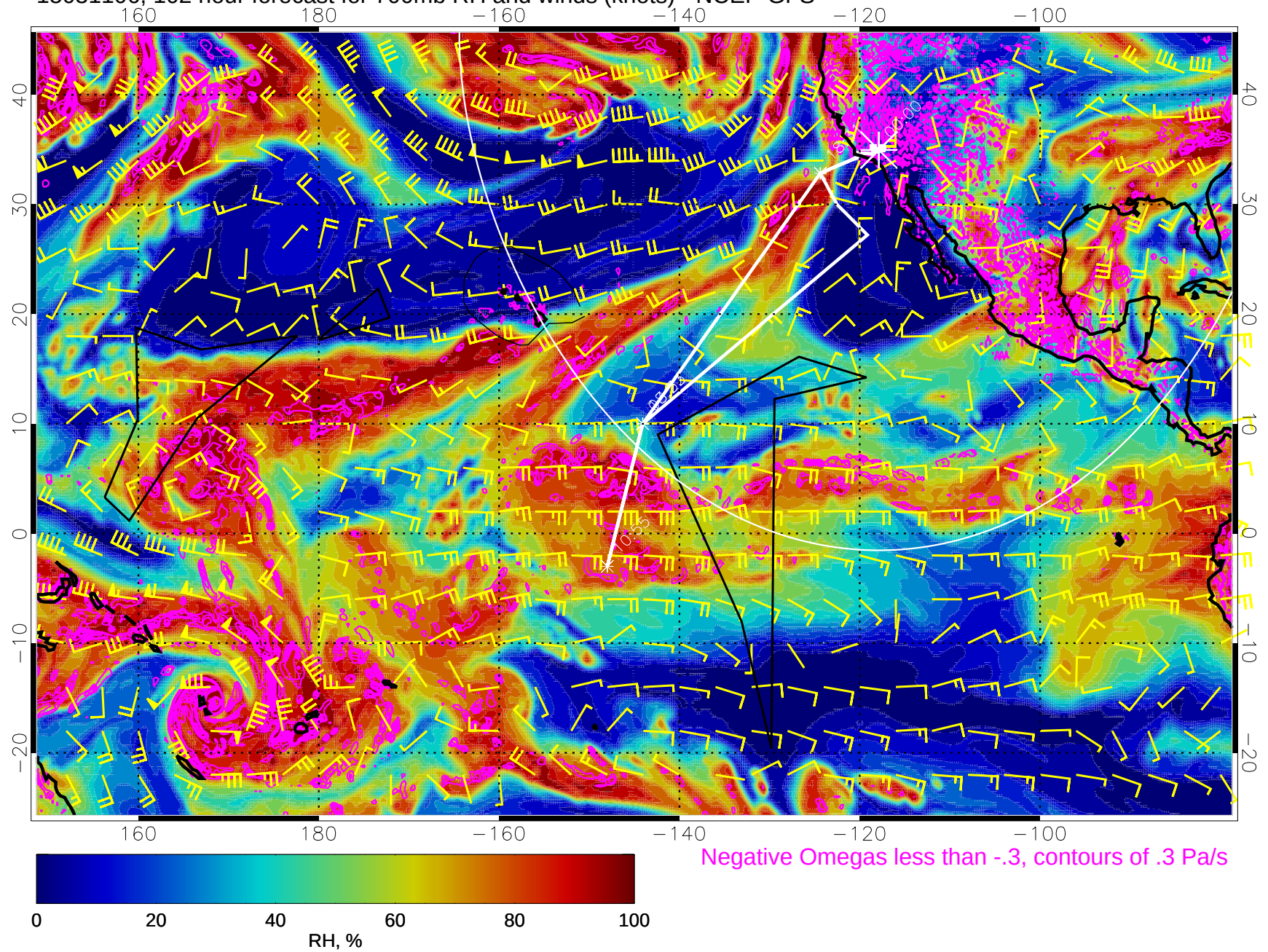
15031106, 102 hour forecast for 700mb RH and winds (knots) - NCEP GFS
