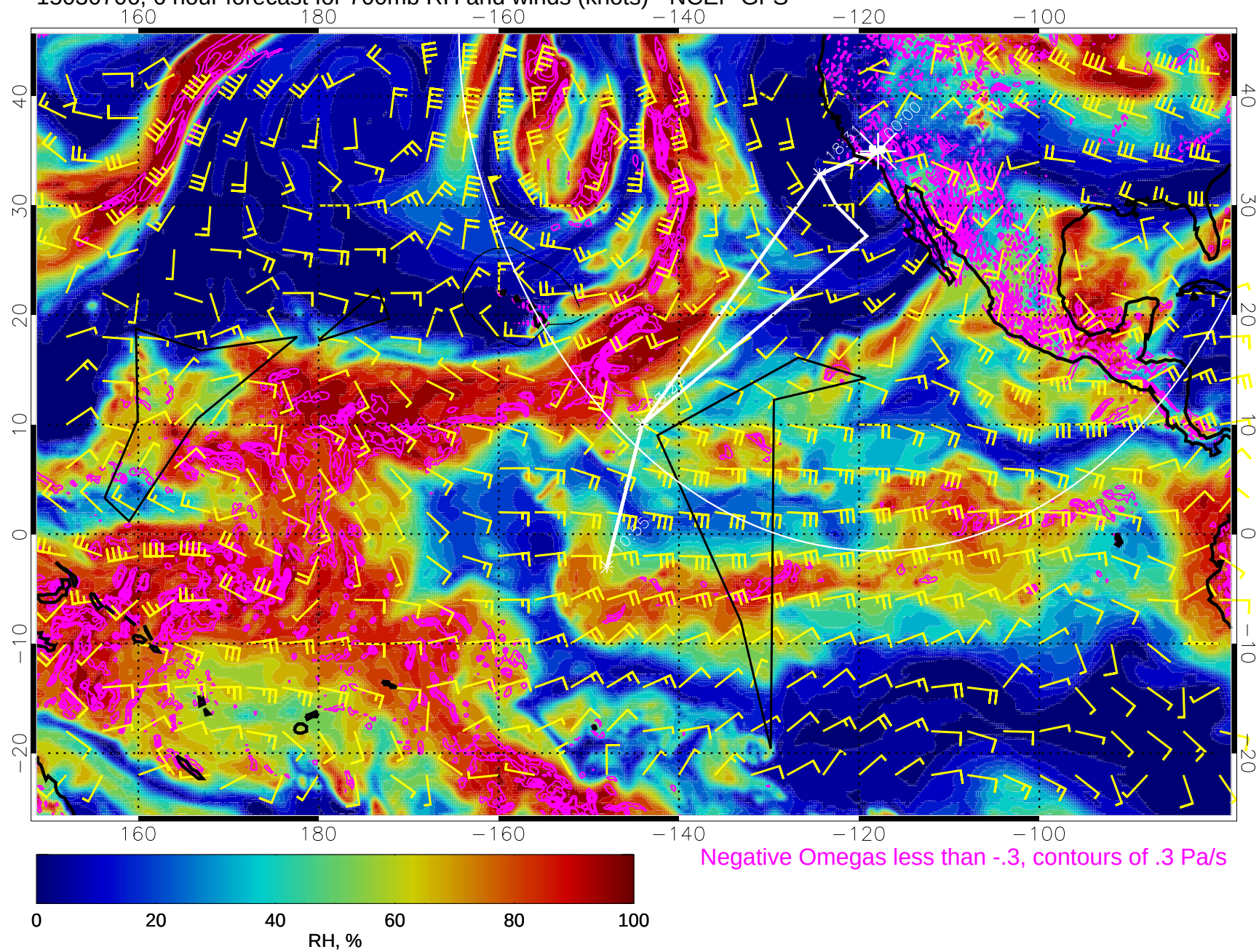
15030706, 6 hour forecast for 700mb RH and winds (knots) - NCEP GFS
