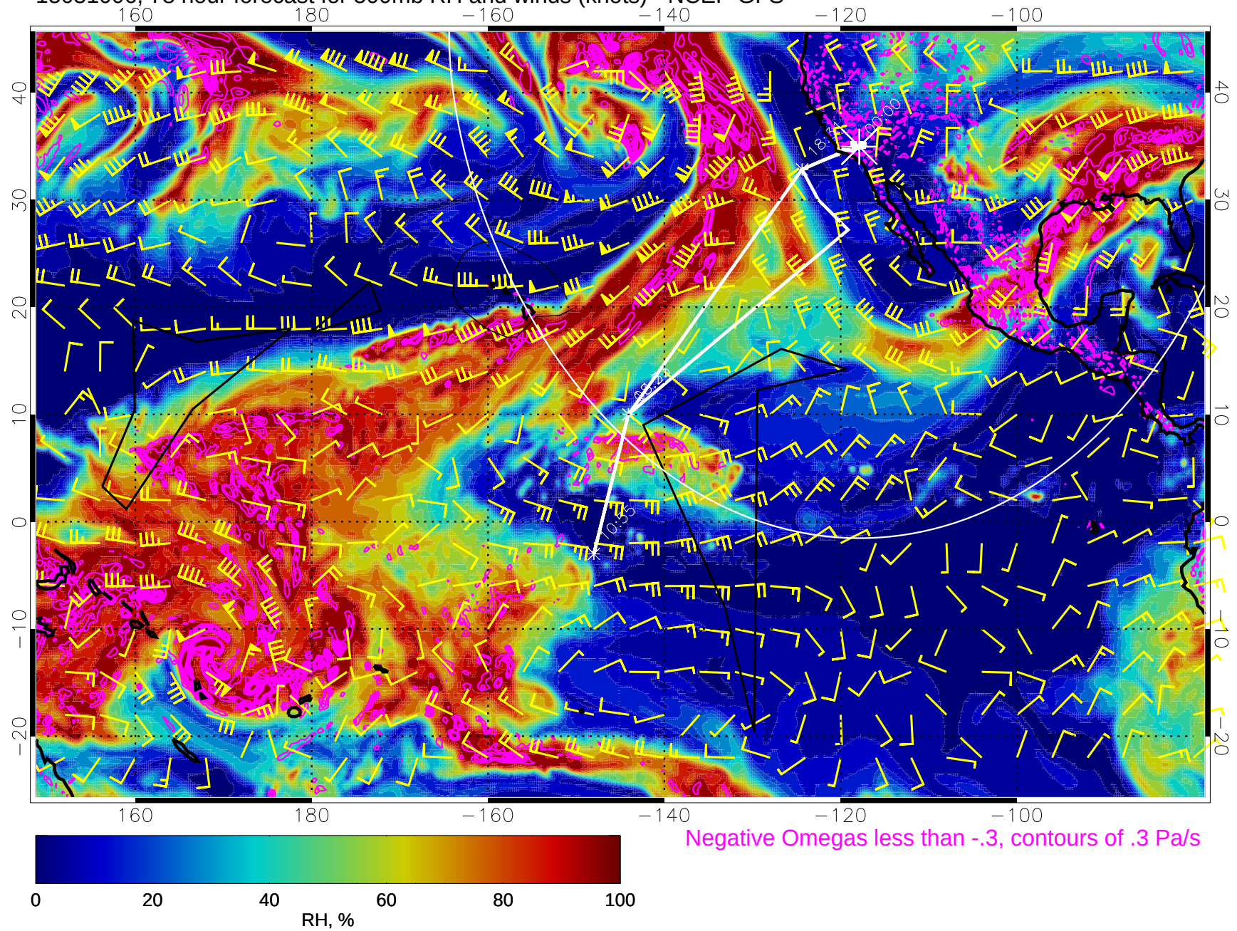
15031006, 78 hour forecast for 500mb RH and winds (knots) - NCEP GFS
