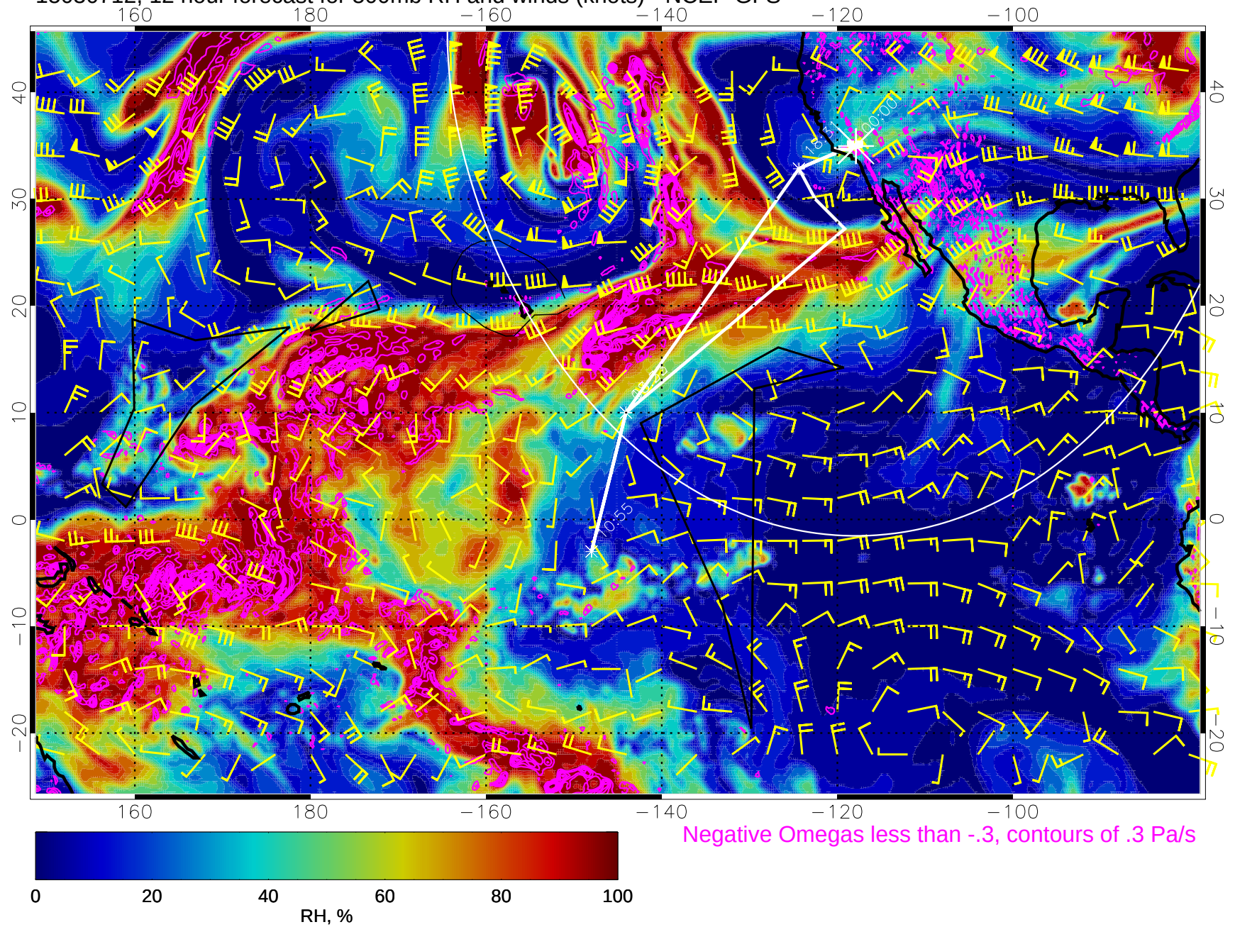
15030712, 12 hour forecast for 500mb RH and winds (knots) - NCEP GFS
