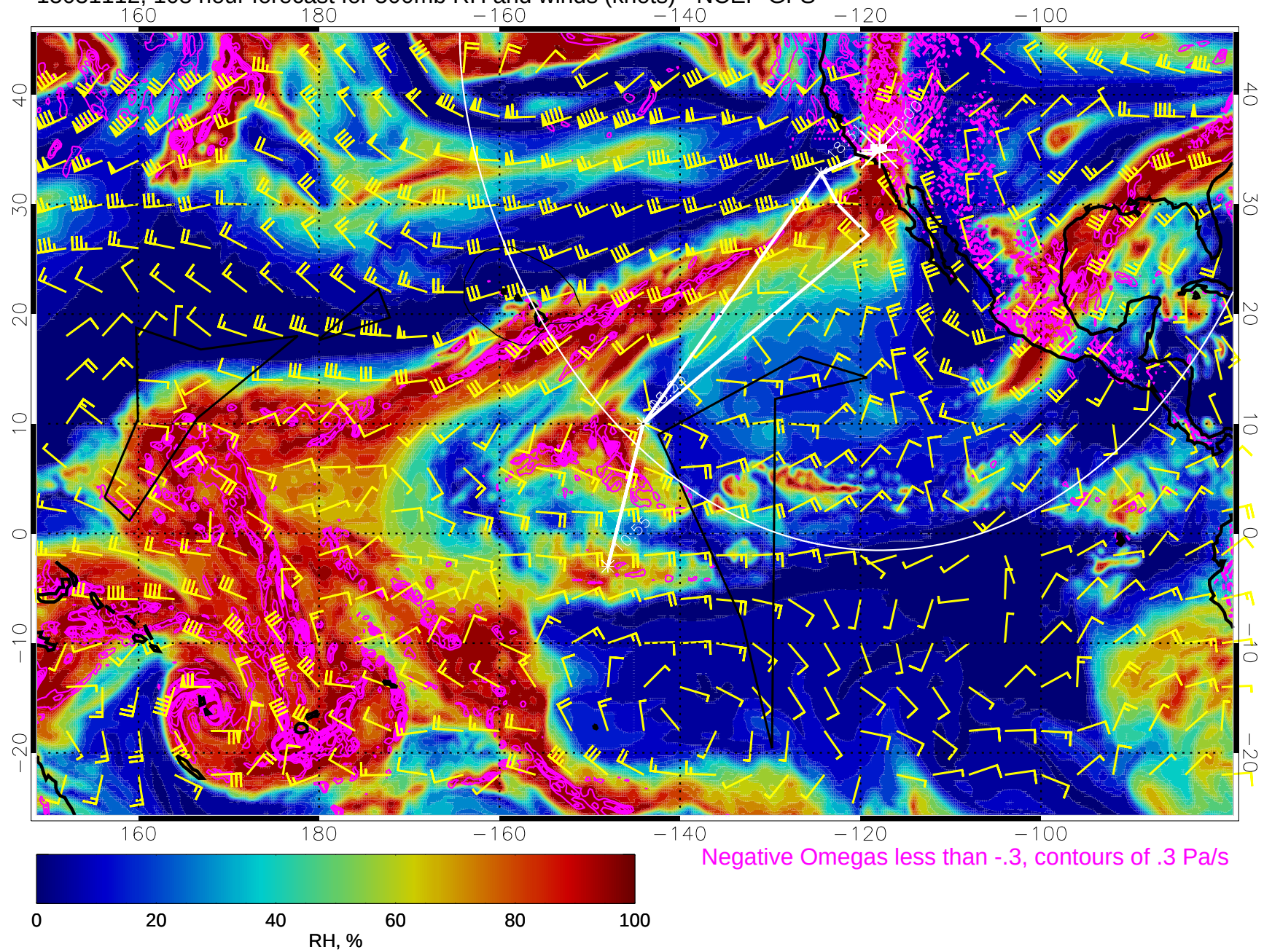
15031112, 108 hour forecast for 500mb RH and winds (knots) - NCEP GFS
