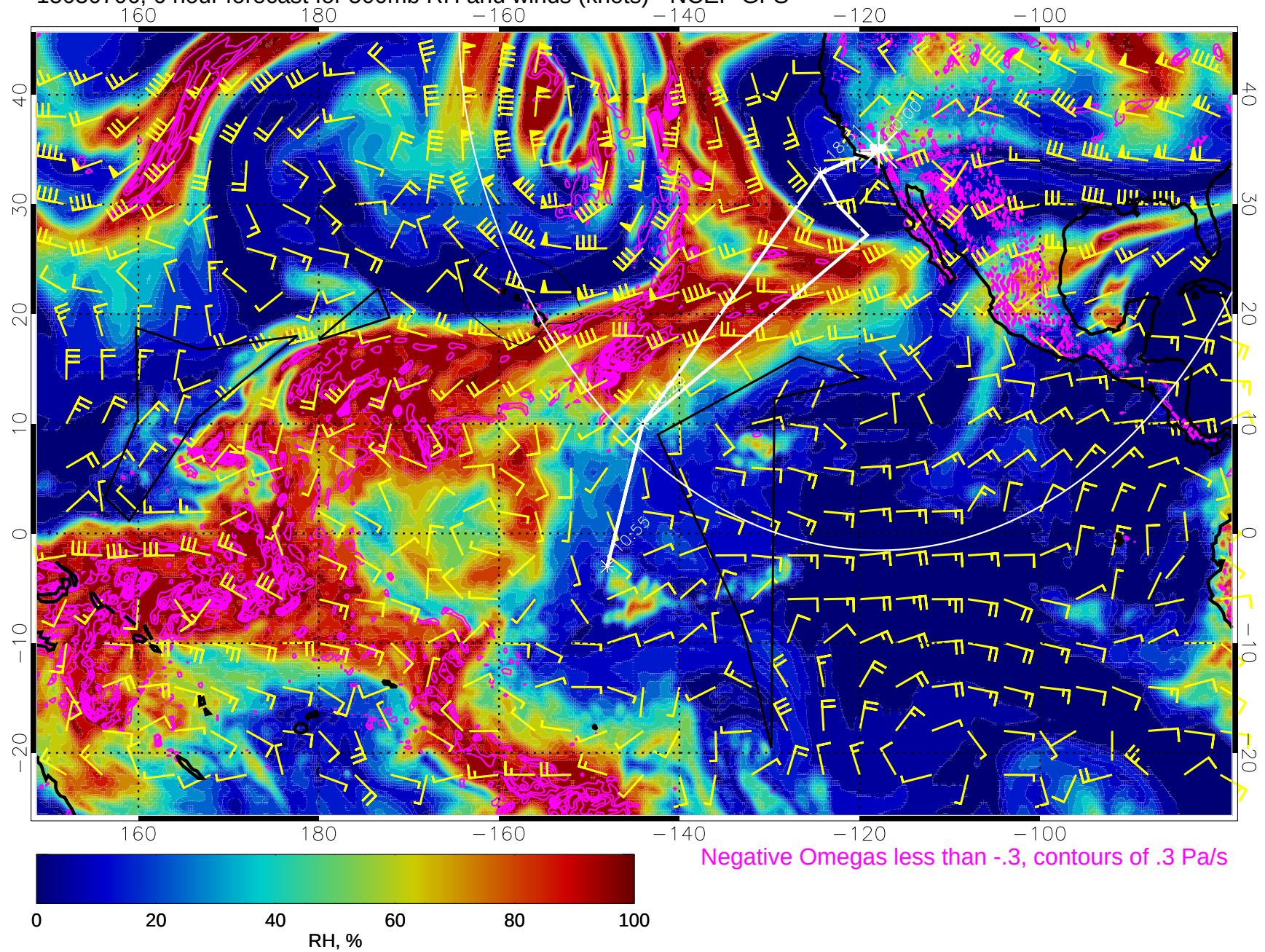
15030706, 6 hour forecast for 500mb RH and winds (knots) - NCEP GFS
