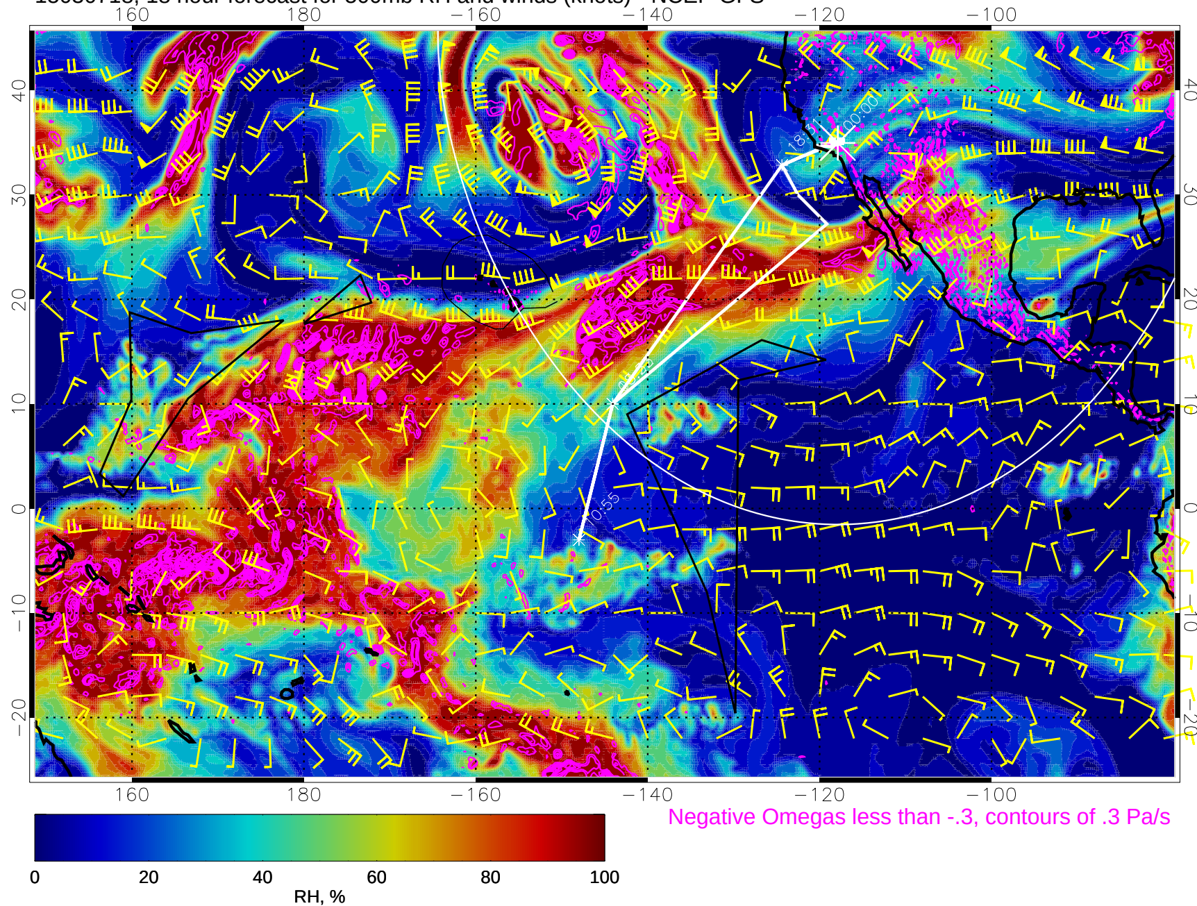
15030718, 18 hour forecast for 500mb RH and winds (knots) - NCEP GFS
