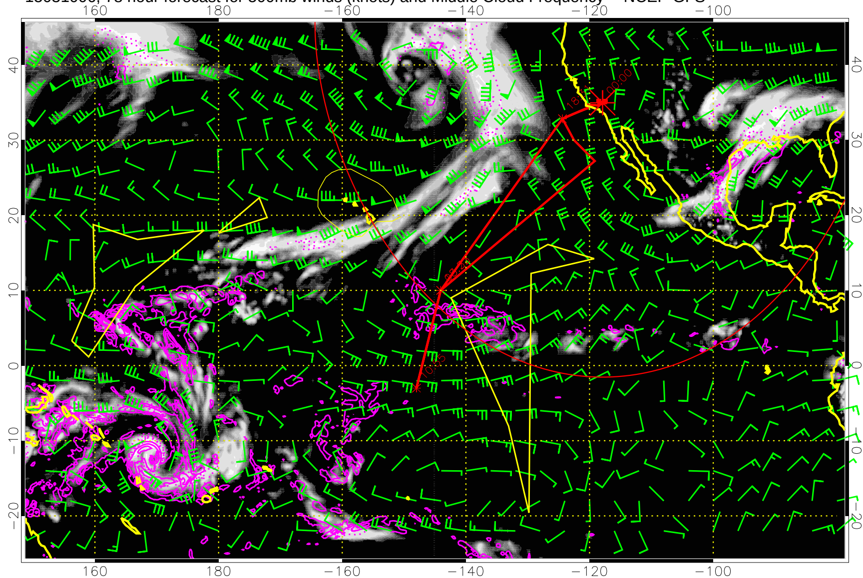
15031006, 78 hour forecast for 500mb winds (knots) and Middle Cloud Frequency -- NCEP GFS
