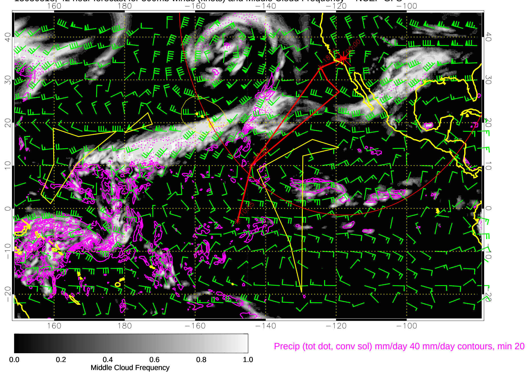
15030818, 42 hour forecast for 500mb winds (knots) and Middle Cloud Frequency -- NCEP GFS
