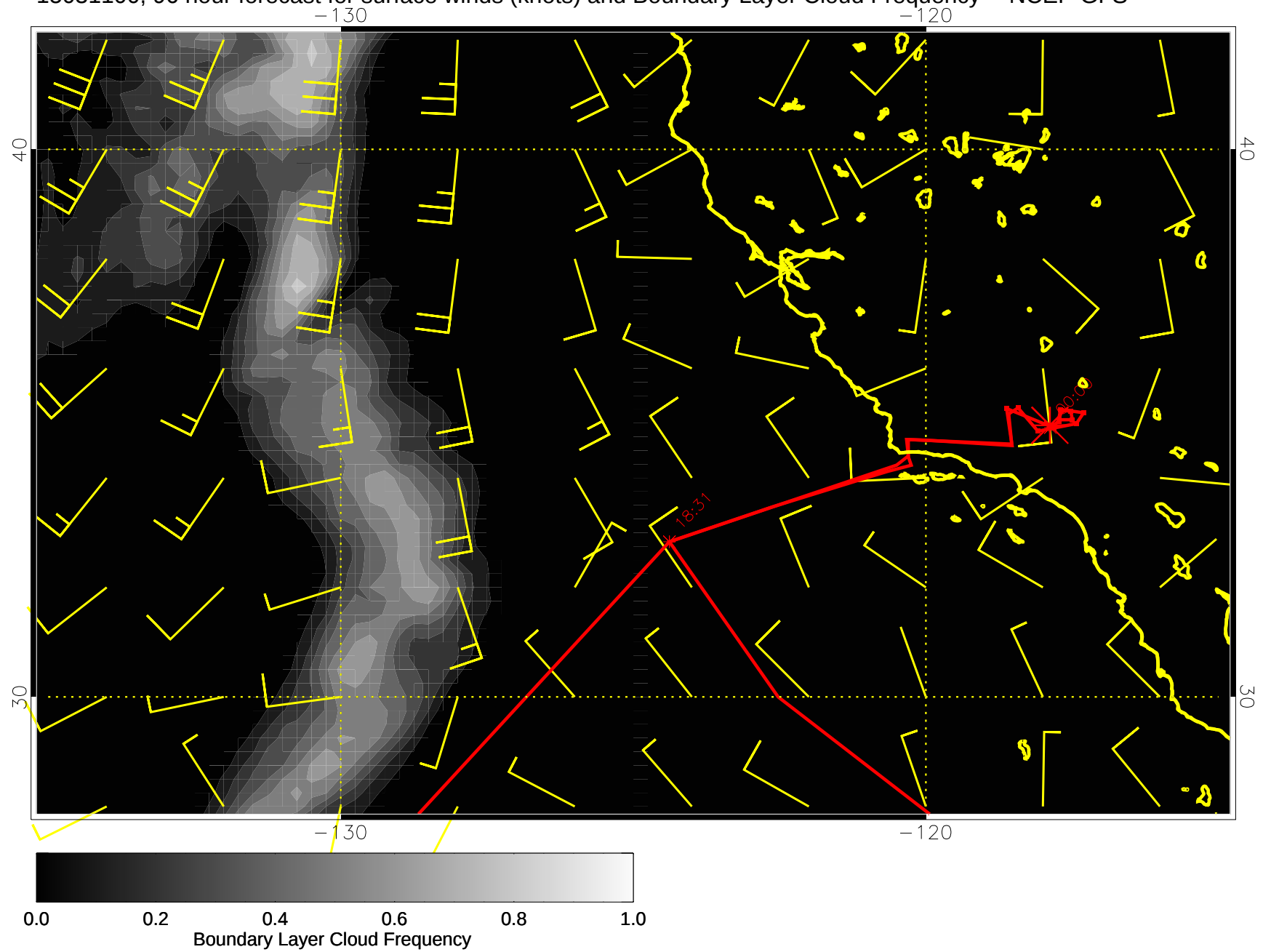
15031100, 96 hour forecast for surface winds (knots) and Boundary Layer Cloud Frequency -- NCEP GFS
