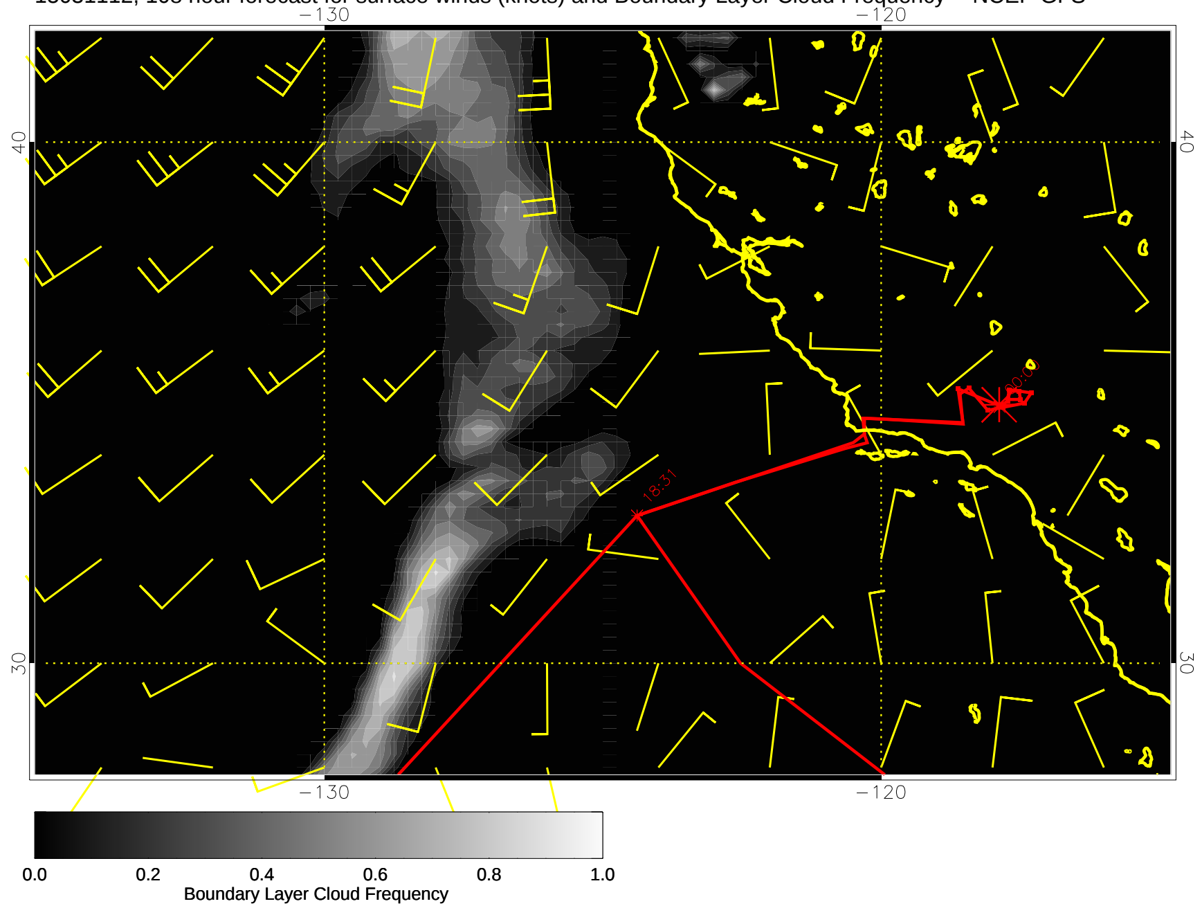
15031112, 108 hour forecast for surface winds (knots) and Boundary Layer Cloud Frequency -- NCEP GFS
