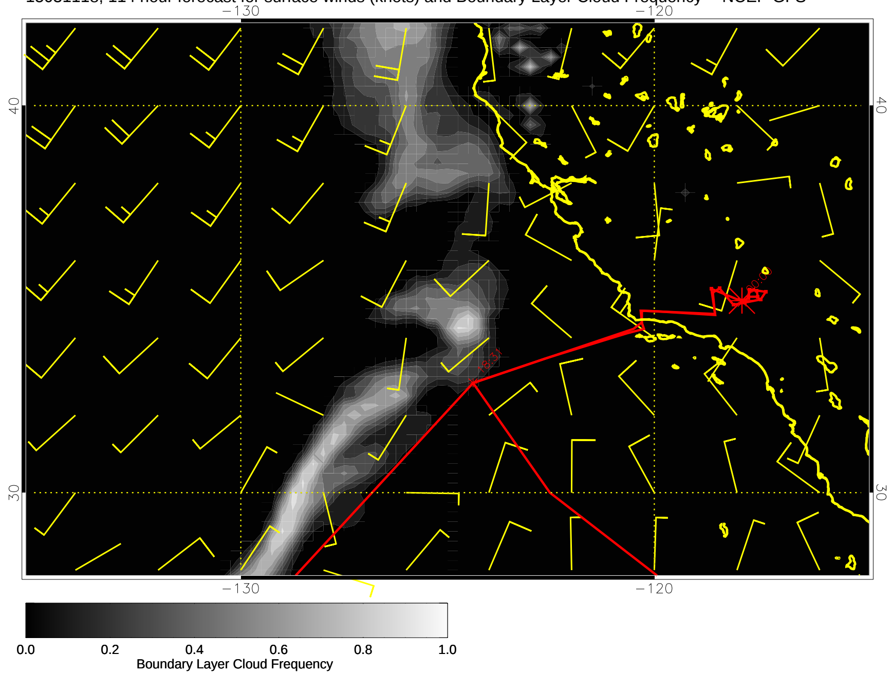
15031118, 114 hour forecast for surface winds (knots) and Boundary Layer Cloud Frequency -- NCEP GFS
