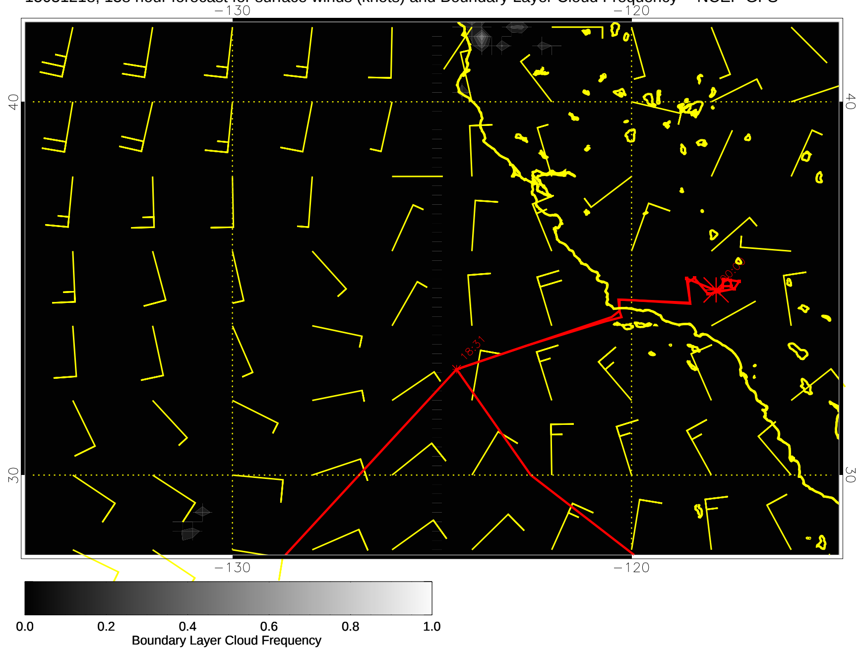
15031218, 138 hour forecast for surface winds (knots) and Boundary Layer Cloud Frequency -- NCEP GFS
