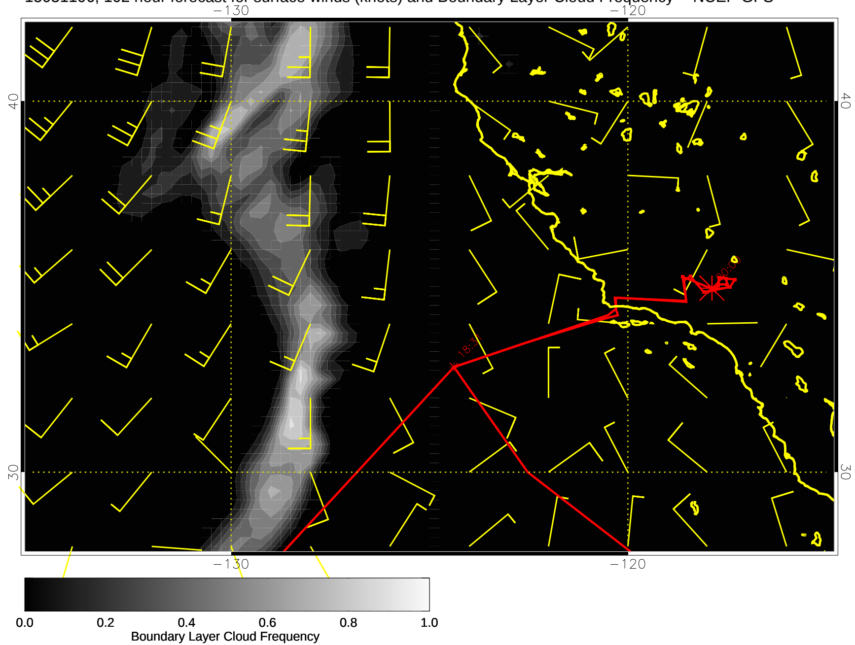
15031106, 102 hour forecast for surface winds (knots) and Boundary Layer Cloud Frequency -- NCEP GFS
