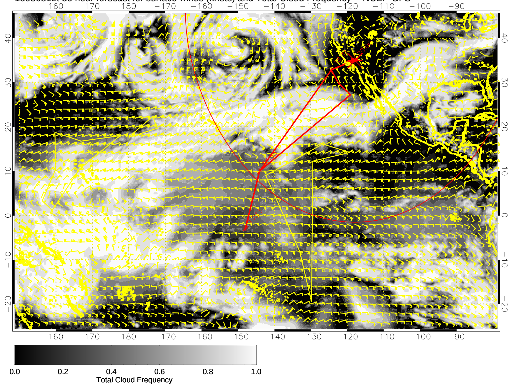
15030812, 36 hour forecast for surface winds (knots) and Total Cloud Frequency -- NCEP GFS
