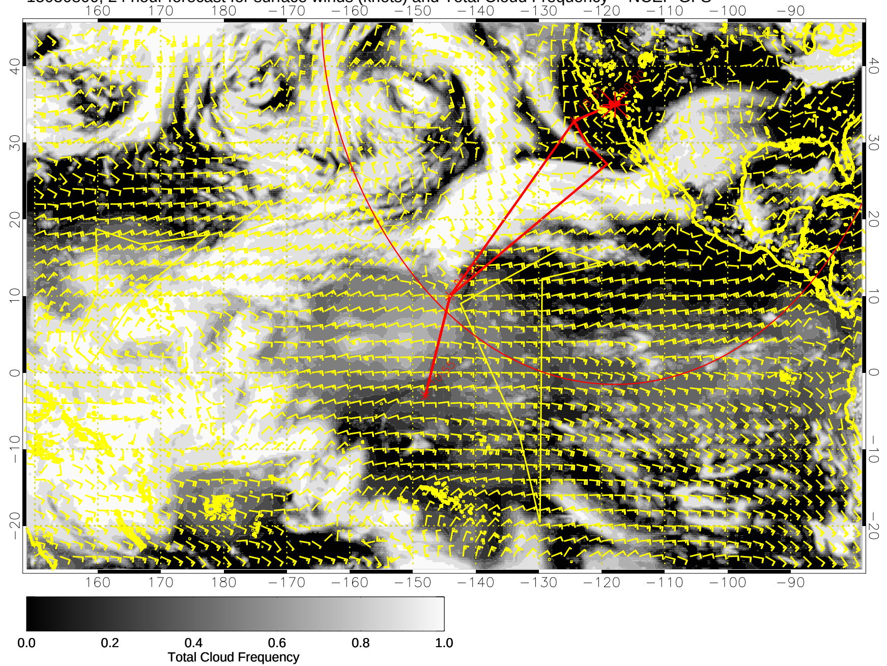
15030800, 24 hour forecast for surface winds (knots) and Total Cloud Frequency -- NCEP GFS
