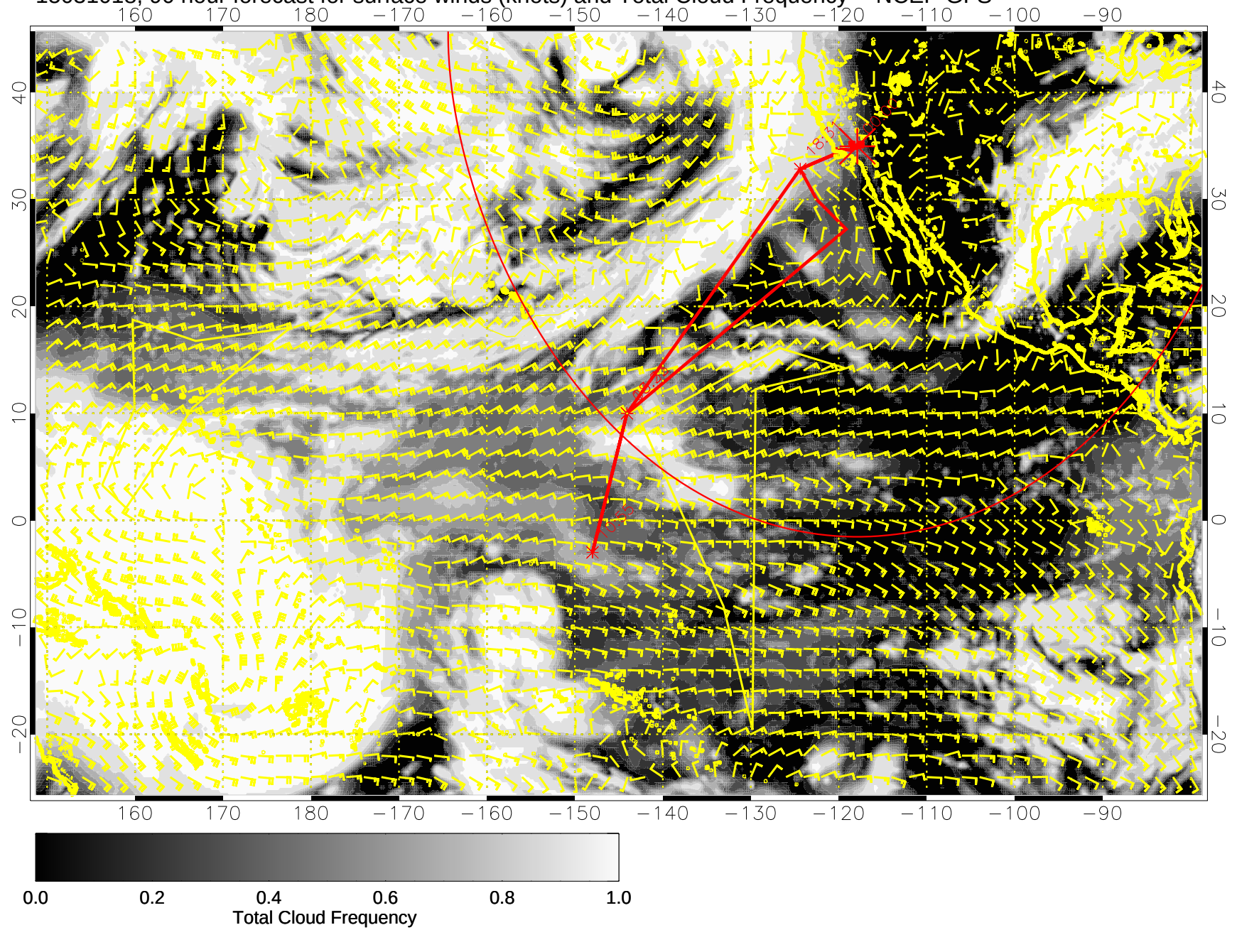
15031018, 90 hour forecast for surface winds (knots) and Total Cloud Frequency -- NCEP GFS
