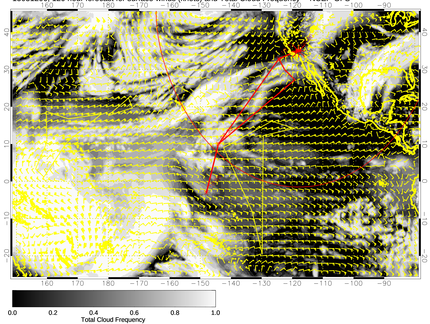
15031200, 120 hour forecast for surface winds (knots) and Total Cloud Frequency -- NCEP GFS
