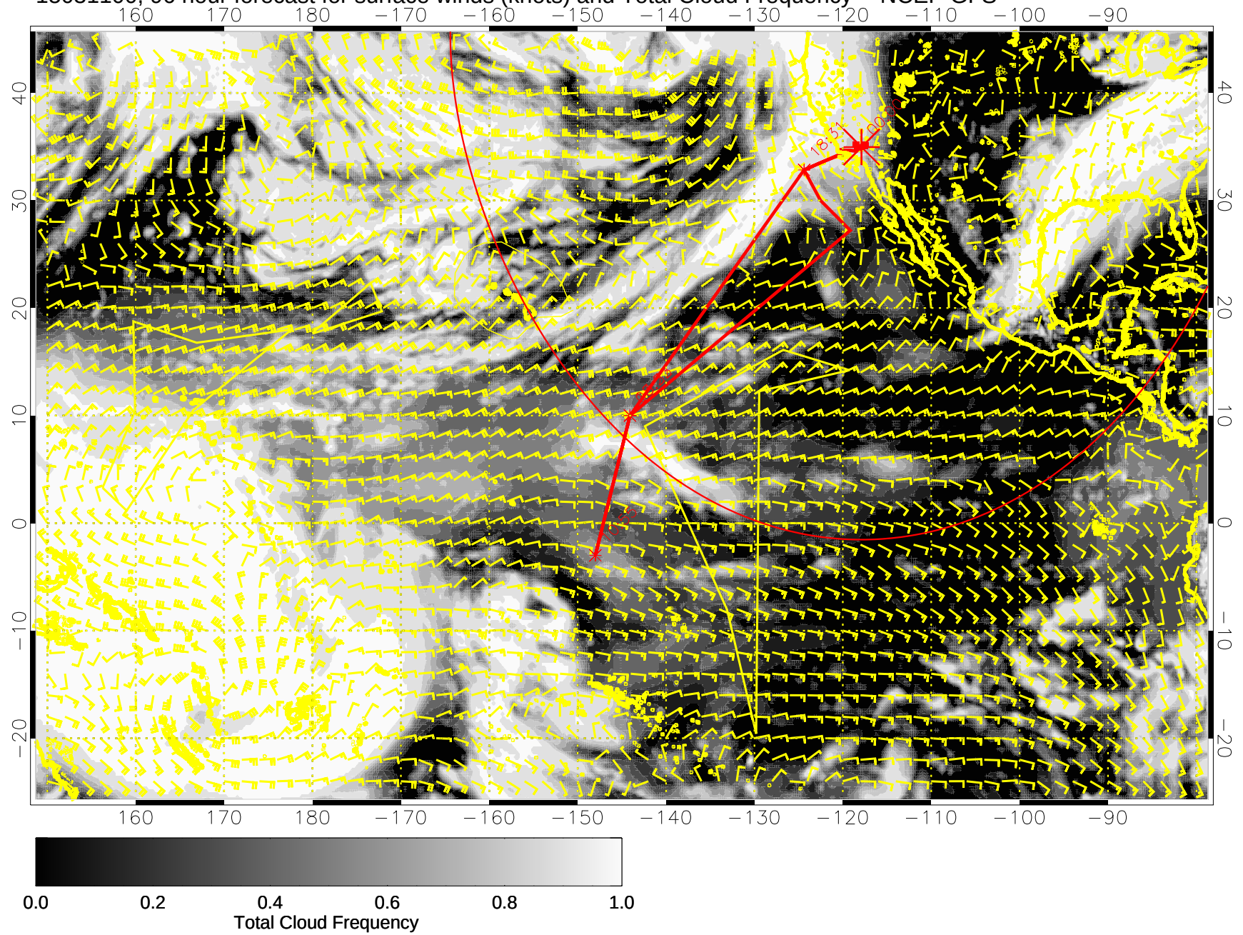
15031100, 96 hour forecast for surface winds (knots) and Total Cloud Frequency -- NCEP GFS
