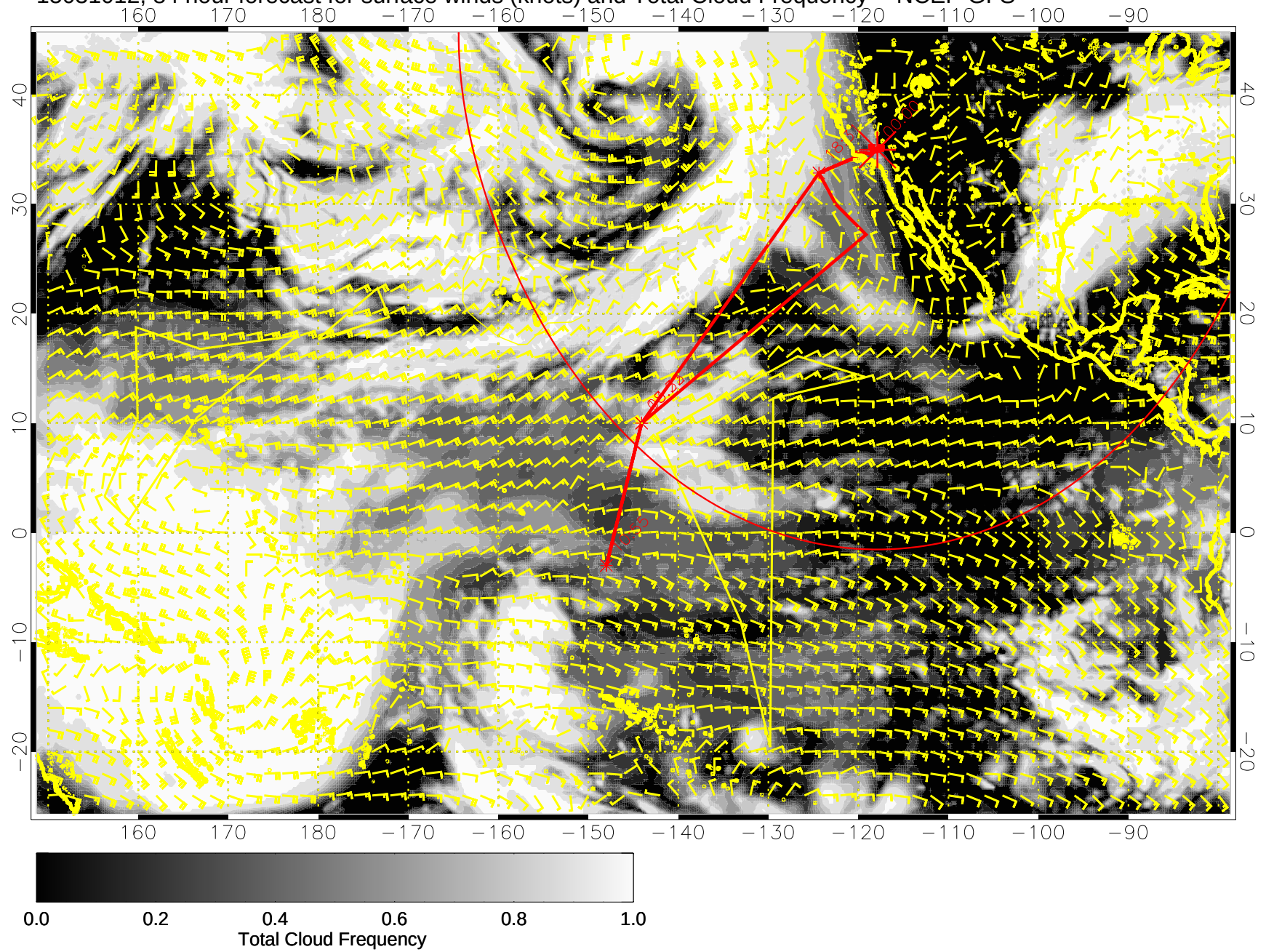
15031012, 84 hour forecast for surface winds (knots) and Total Cloud Frequency -- NCEP GFS
