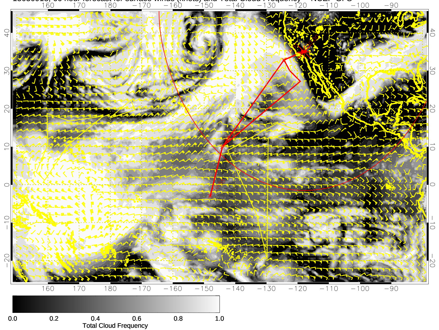
15030918, 66 hour forecast for surface winds (knots) and Total Cloud Frequency -- NCEP GFS
