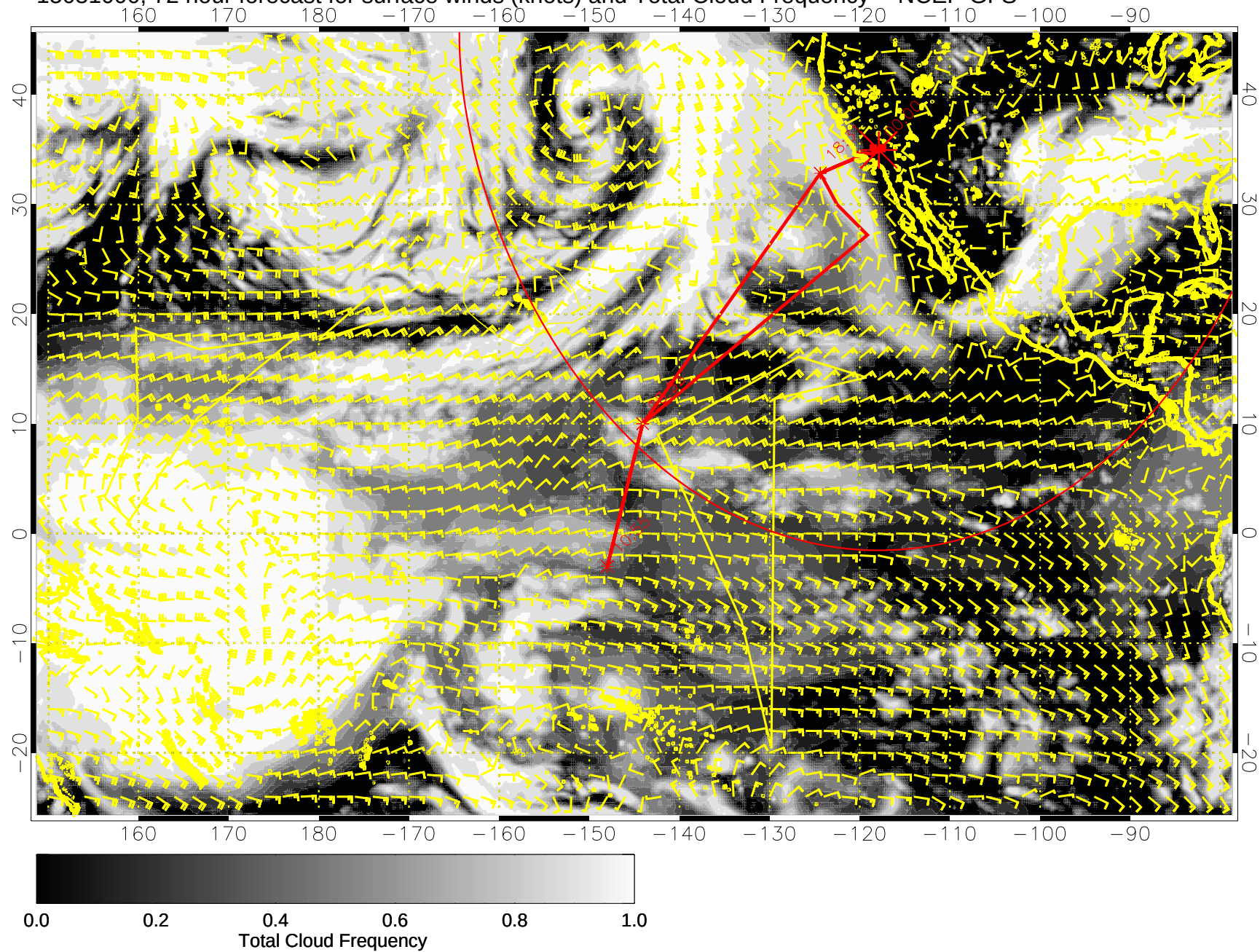
15031000, 72 hour forecast for surface winds (knots) and Total Cloud Frequency -- NCEP GFS
