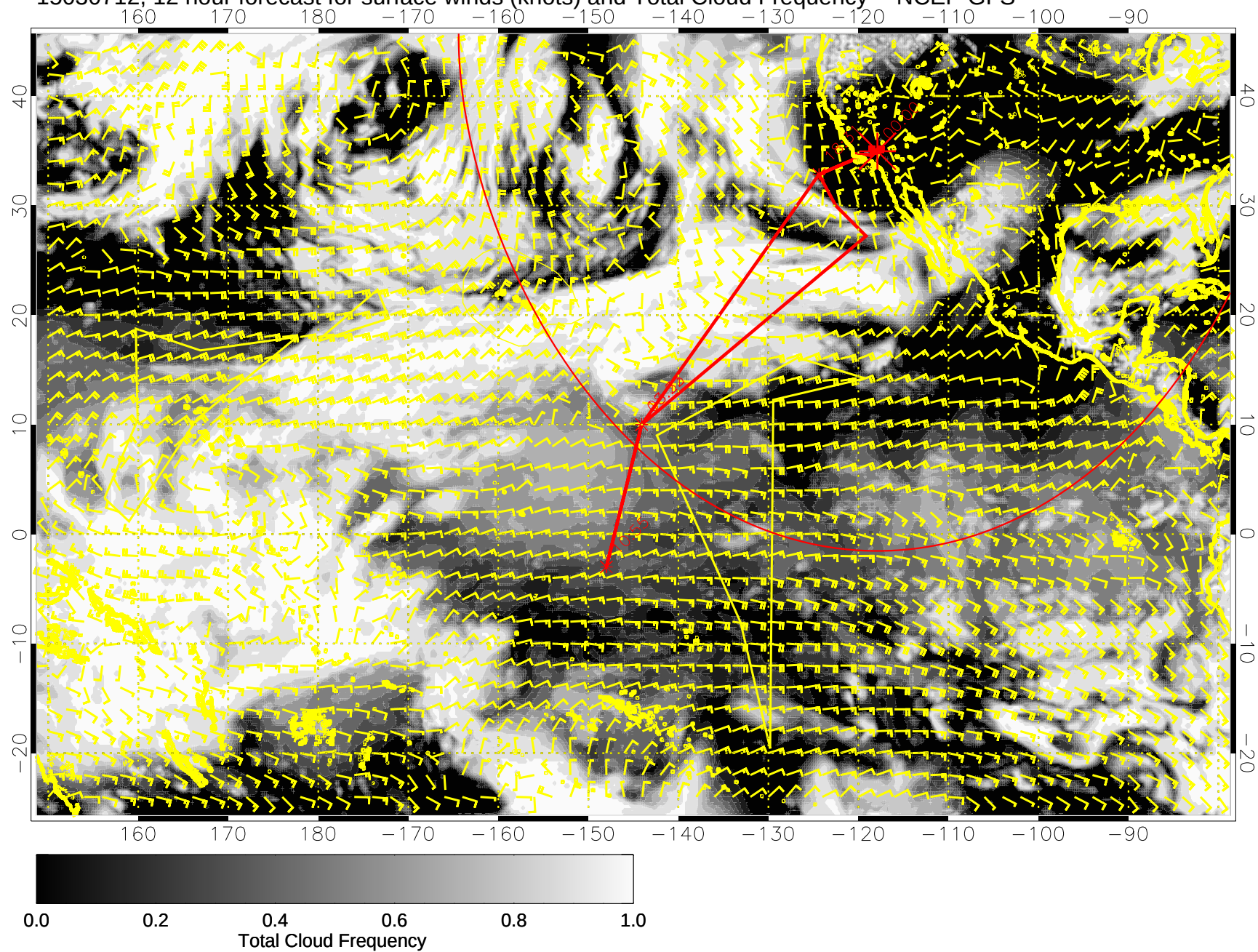
15030712, 12 hour forecast for surface winds (knots) and Total Cloud Frequency -- NCEP GFS
