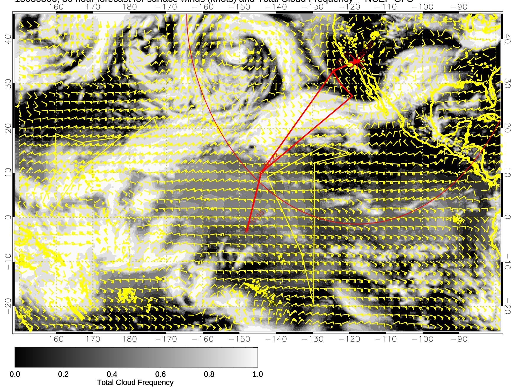
15030806, 30 hour forecast for surface winds (knots) and Total Cloud Frequency -- NCEP GFS
