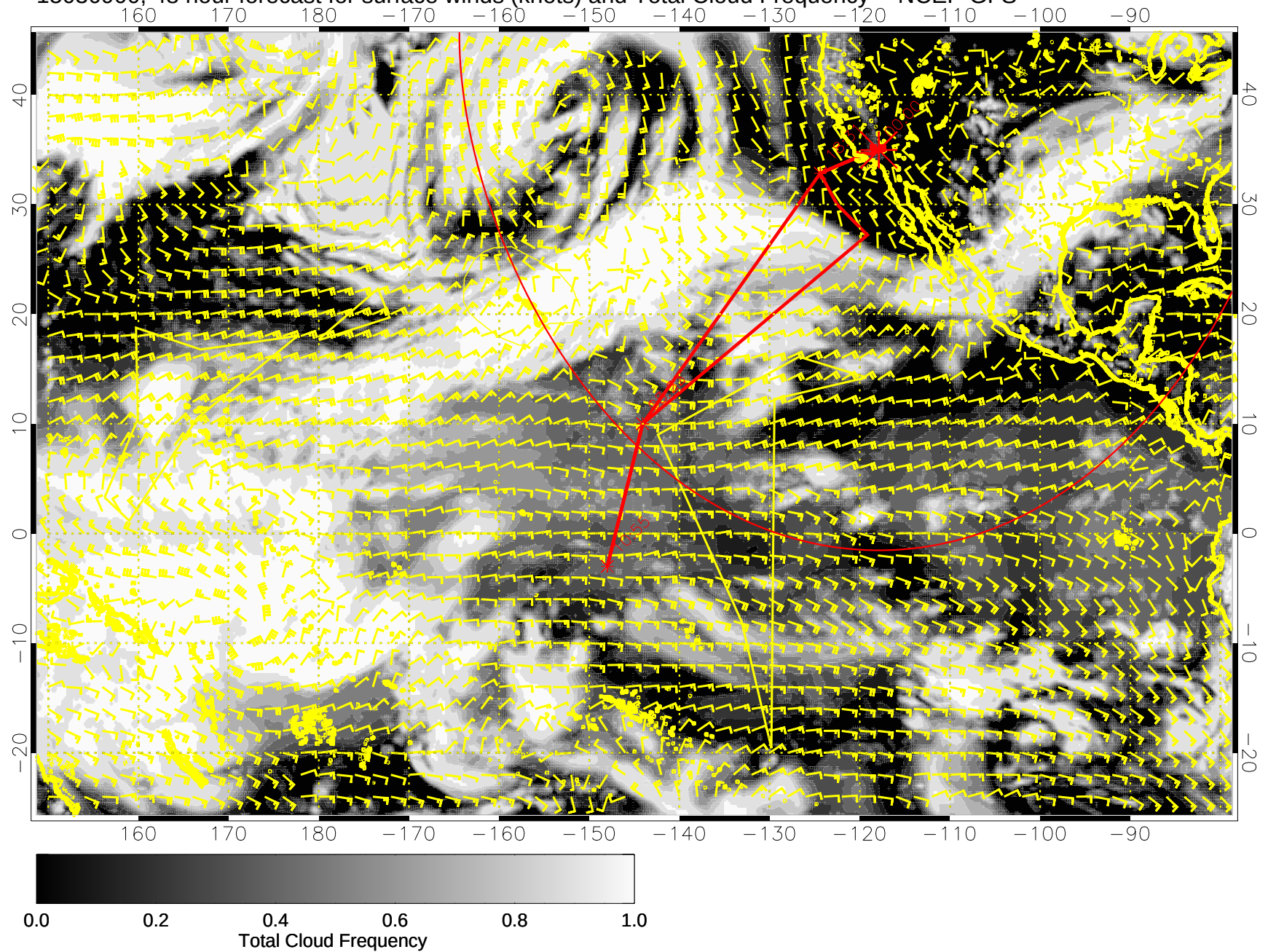
15030900, 48 hour forecast for surface winds (knots) and Total Cloud Frequency -- NCEP GFS
