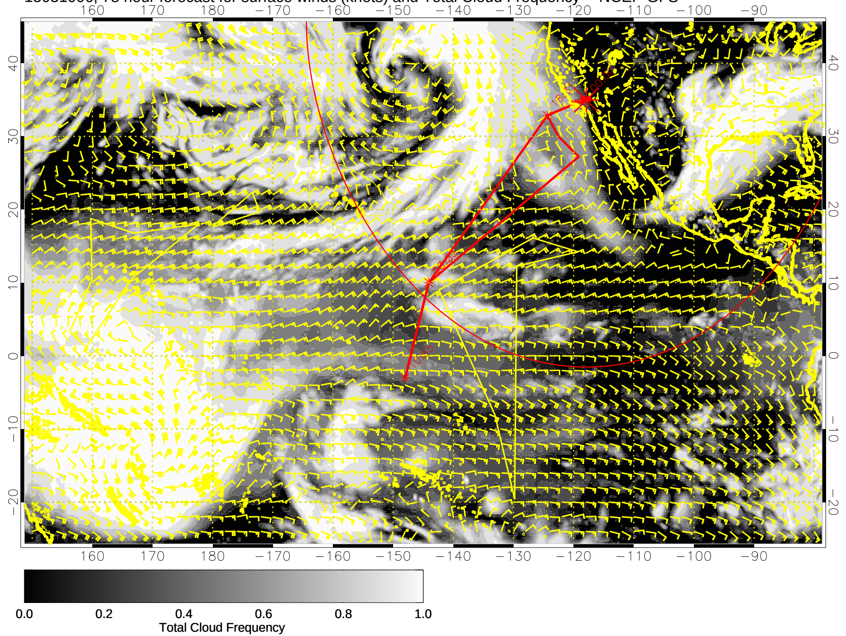
15031006, 78 hour forecast for surface winds (knots) and Total Cloud Frequency -- NCEP GFS
