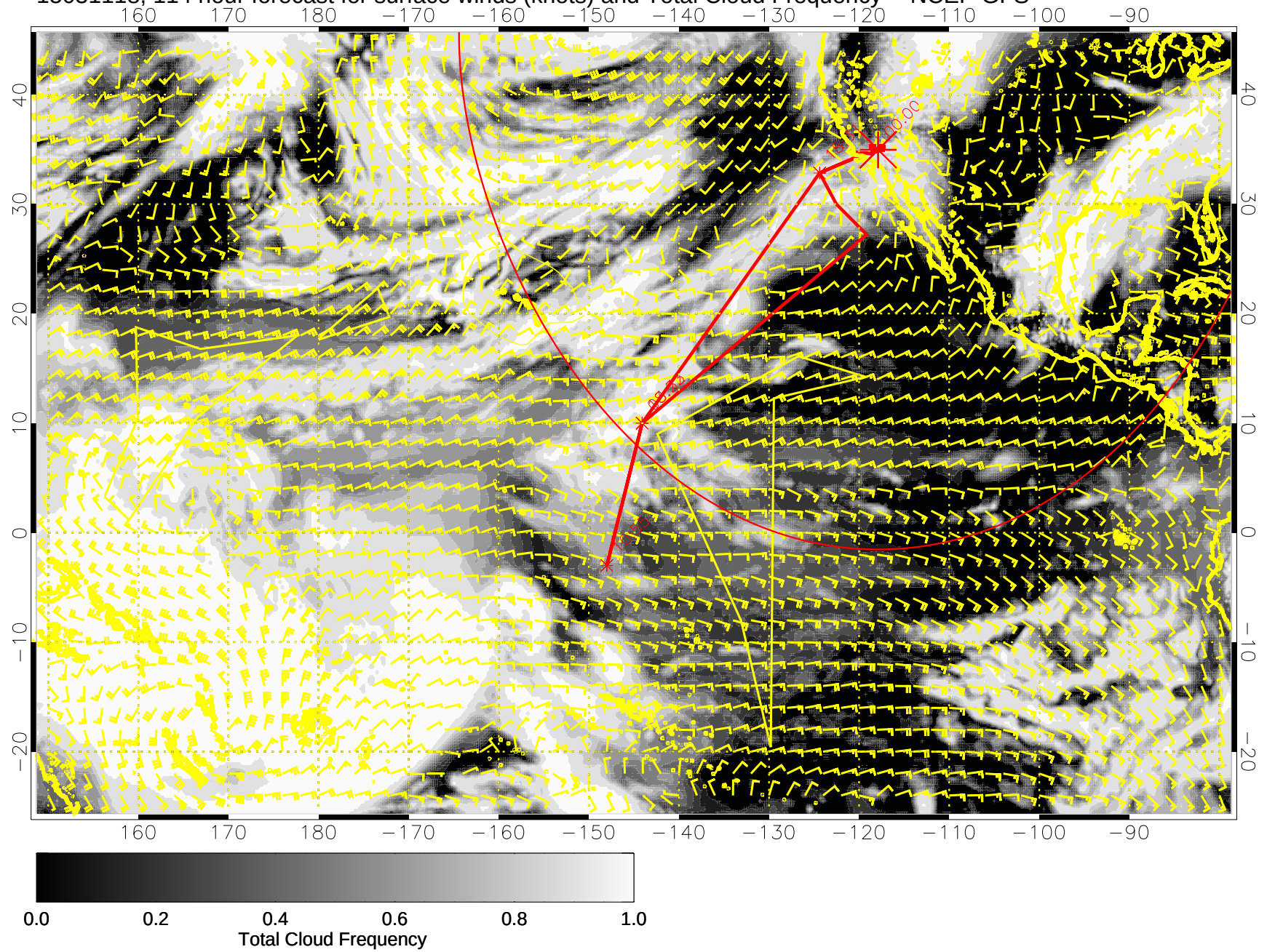
15031118, 114 hour forecast for surface winds (knots) and Total Cloud Frequency -- NCEP GFS
