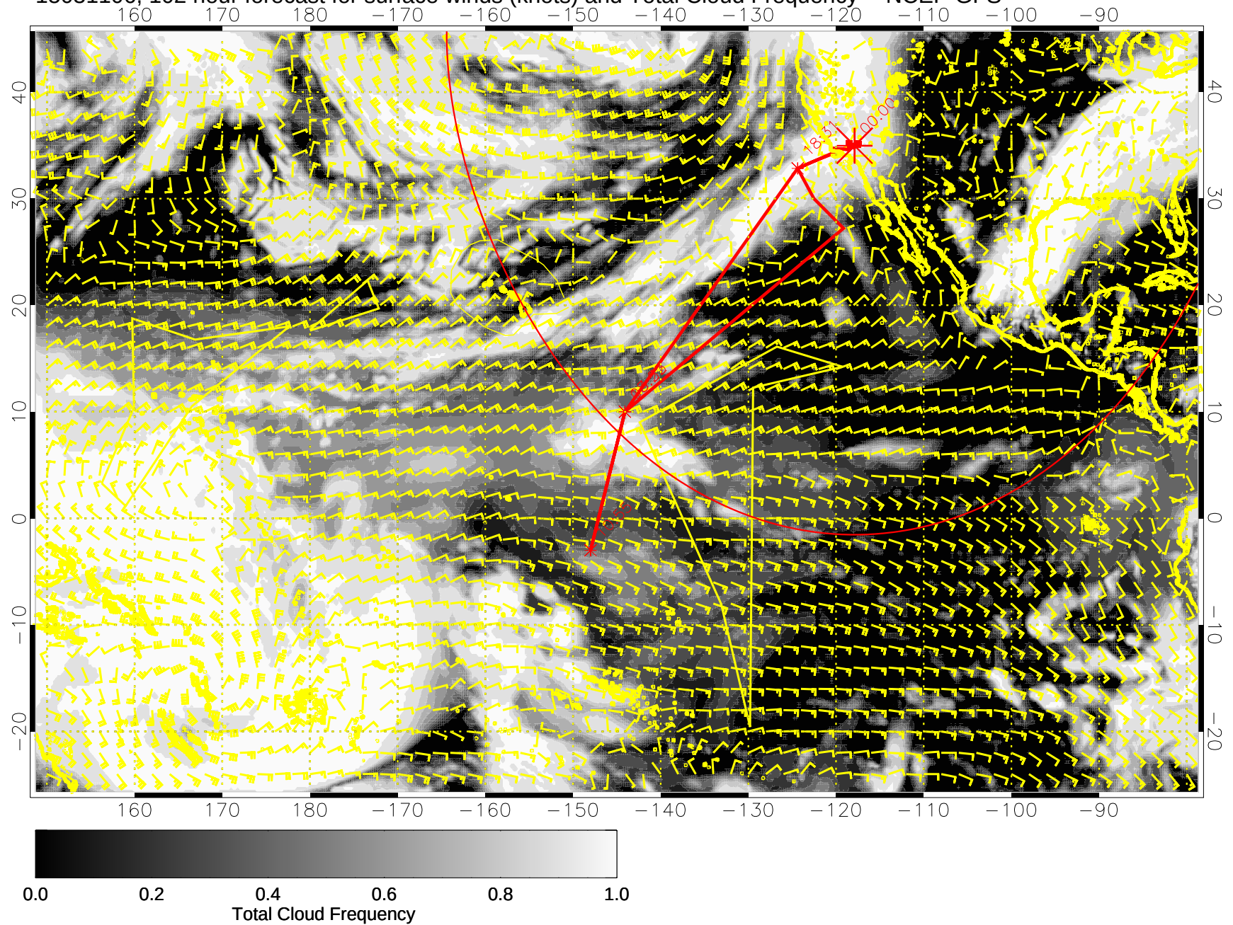
15031106, 102 hour forecast for surface winds (knots) and Total Cloud Frequency -- NCEP GFS
