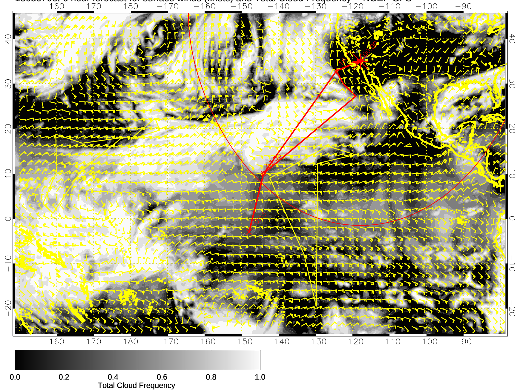
15030706, 6 hour forecast for surface winds (knots) and Total Cloud Frequency -- NCEP GFS
