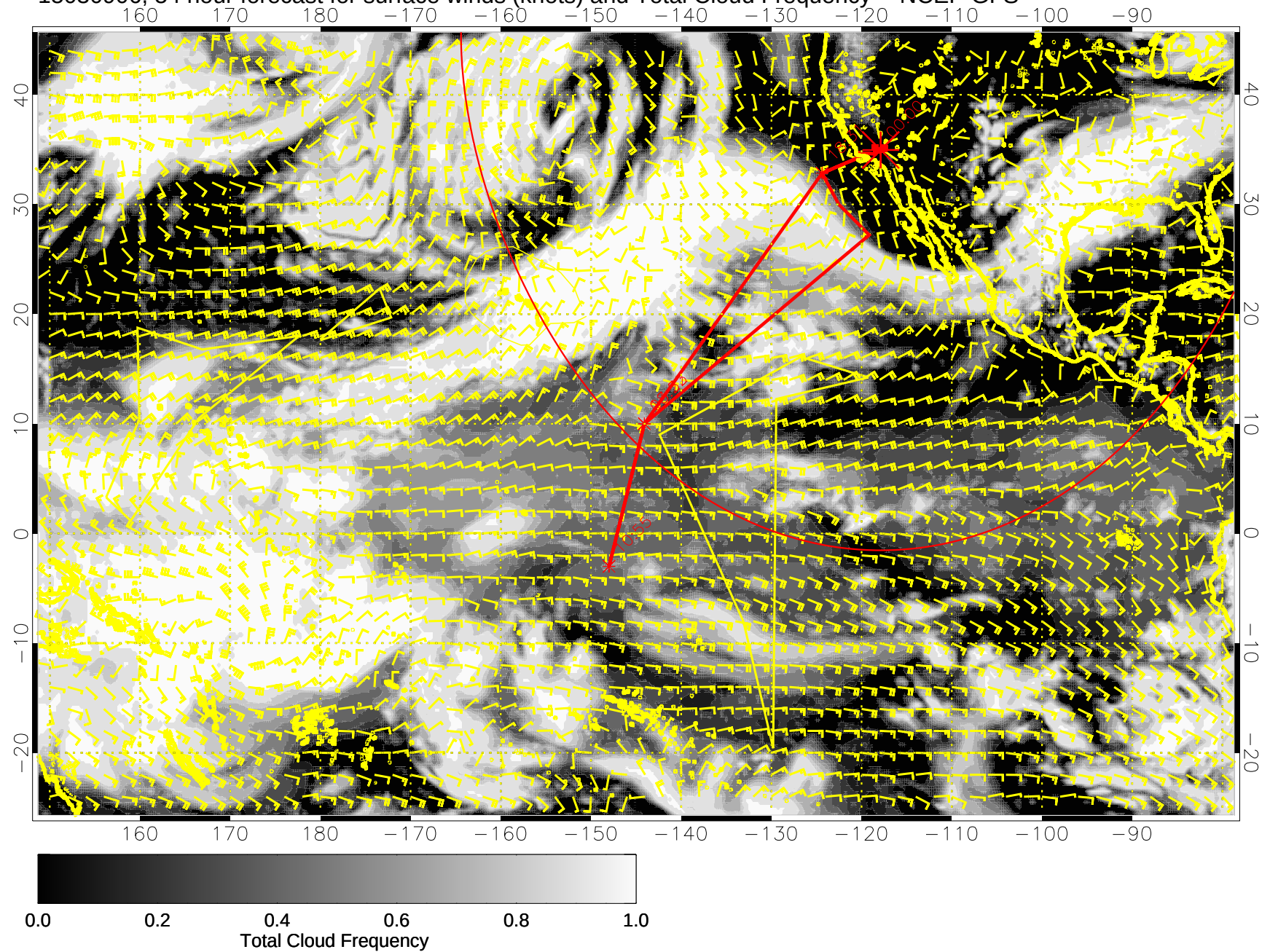
15030906, 54 hour forecast for surface winds (knots) and Total Cloud Frequency -- NCEP GFS
