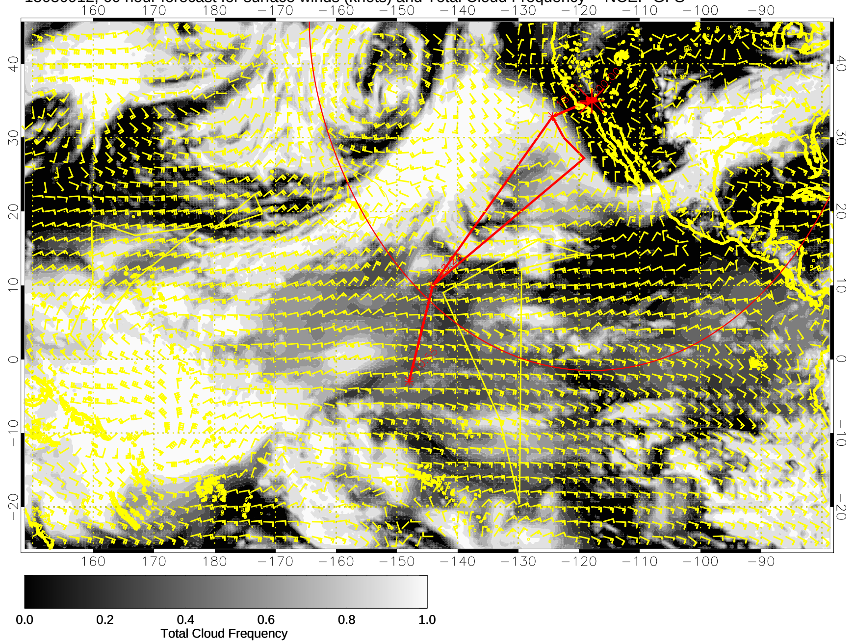
15030912, 60 hour forecast for surface winds (knots) and Total Cloud Frequency -- NCEP GFS
