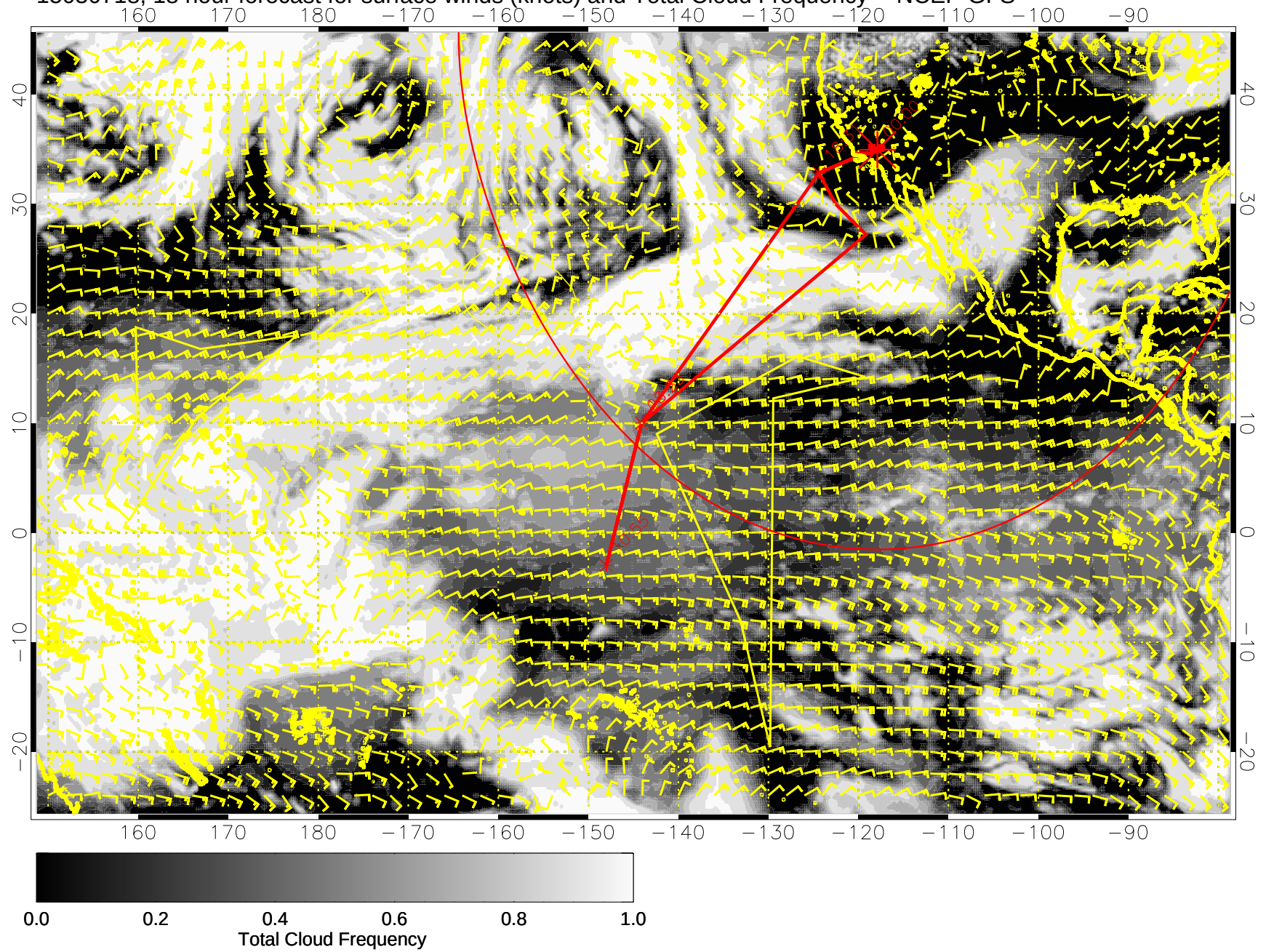
15030718, 18 hour forecast for surface winds (knots) and Total Cloud Frequency -- NCEP GFS
