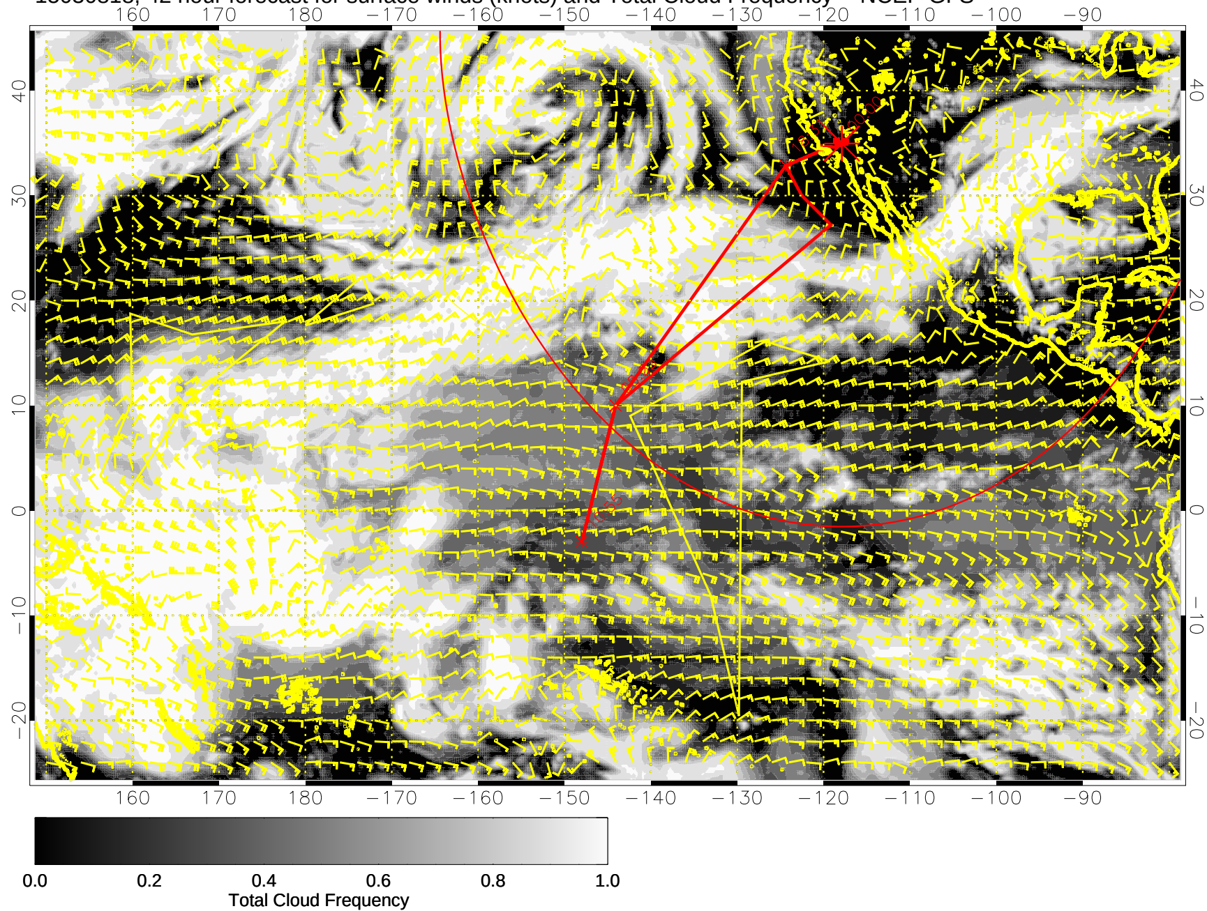
15030818, 42 hour forecast for surface winds (knots) and Total Cloud Frequency -- NCEP GFS
