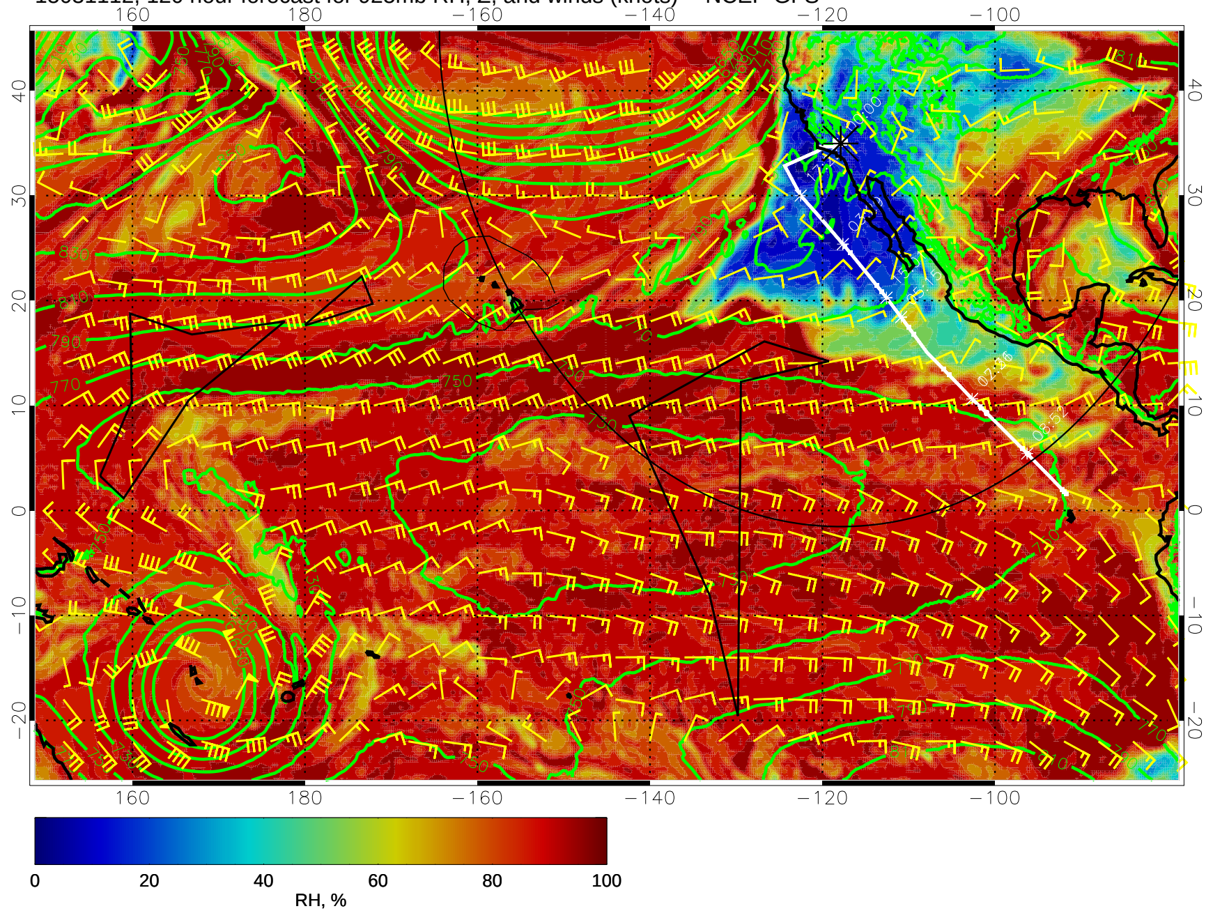
15031112, 120 hour forecast for 925mb RH, Z, and winds (knots) -- NCEP GFS
