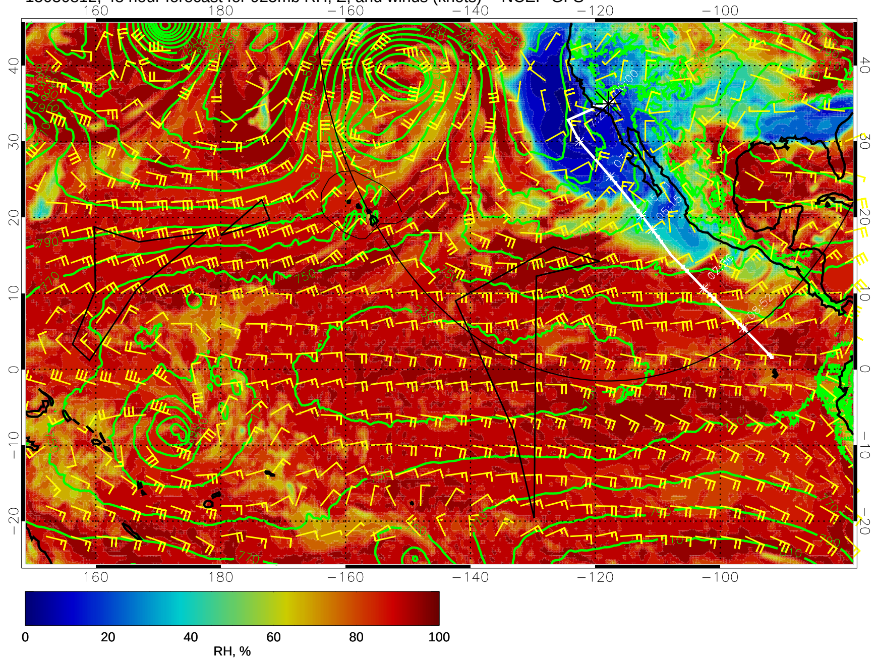
15030812, 48 hour forecast for 925mb RH, Z, and winds (knots) -- NCEP GFS
