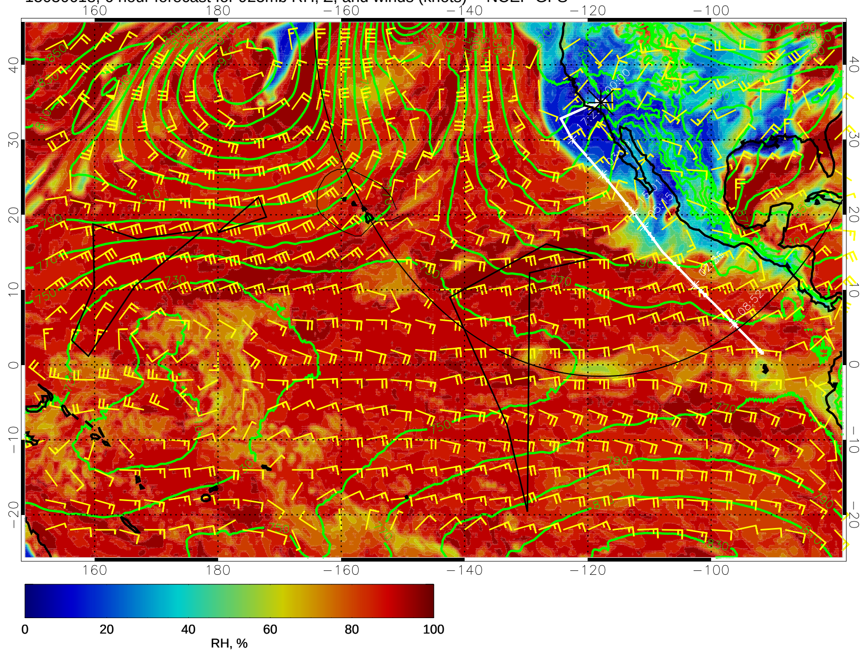
15030618, 6 hour forecast for 925mb RH, Z, and winds (knots) -- NCEP GFS
