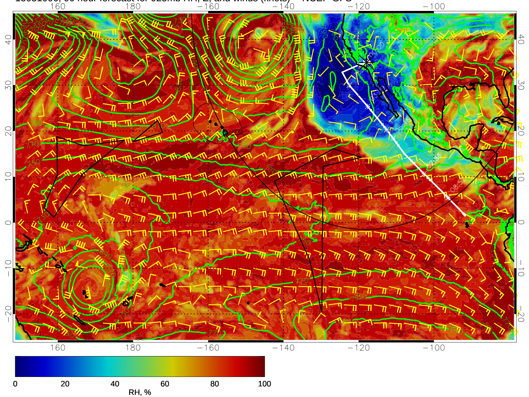
15031006, 90 hour forecast for 925mb RH, Z, and winds (knots) -- NCEP GFS
