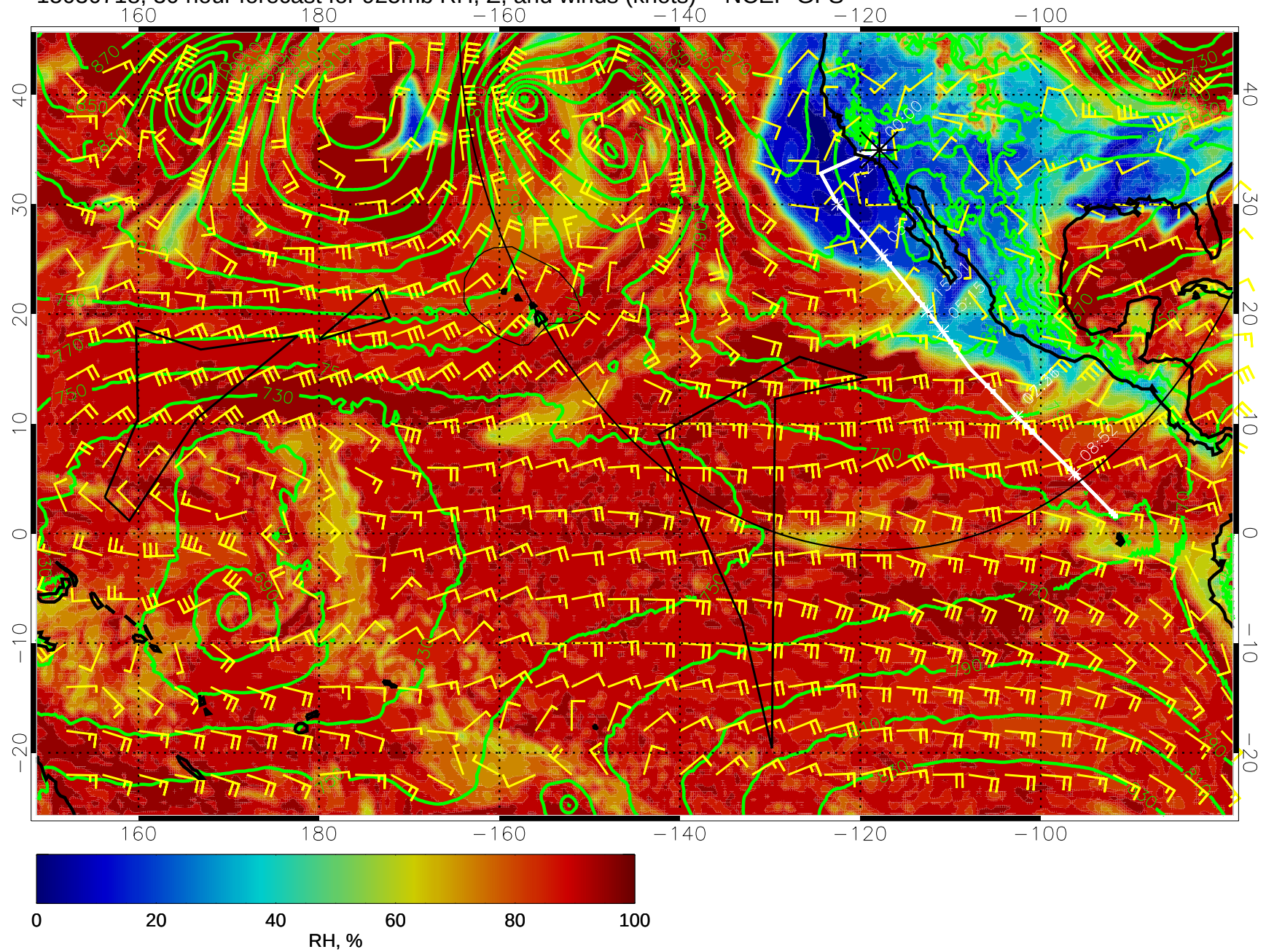
15030718, 30 hour forecast for 925mb RH, Z, and winds (knots) -- NCEP GFS
