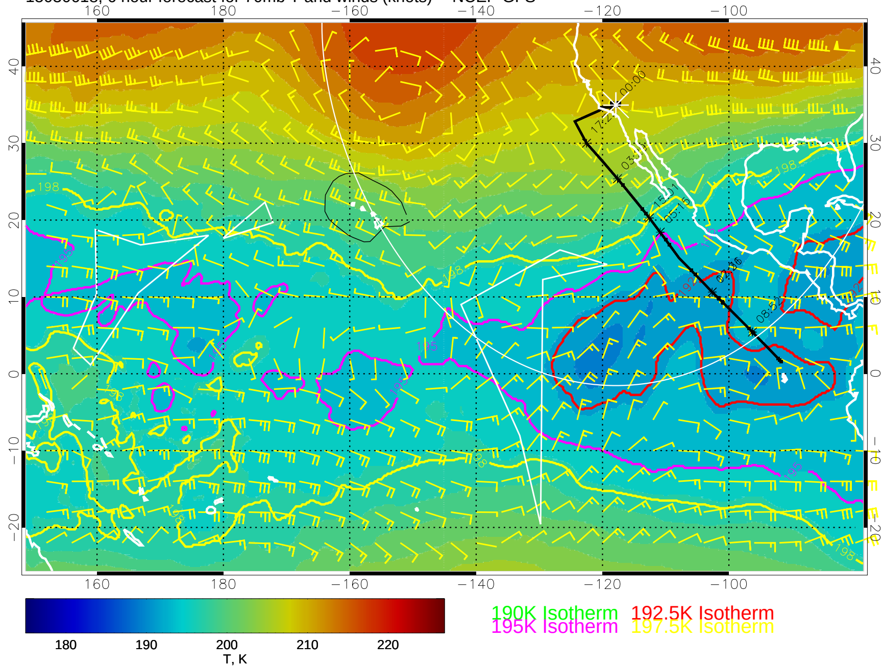
15030618, 6 hour forecast for 70mb T and winds (knots) -- NCEP GFS
