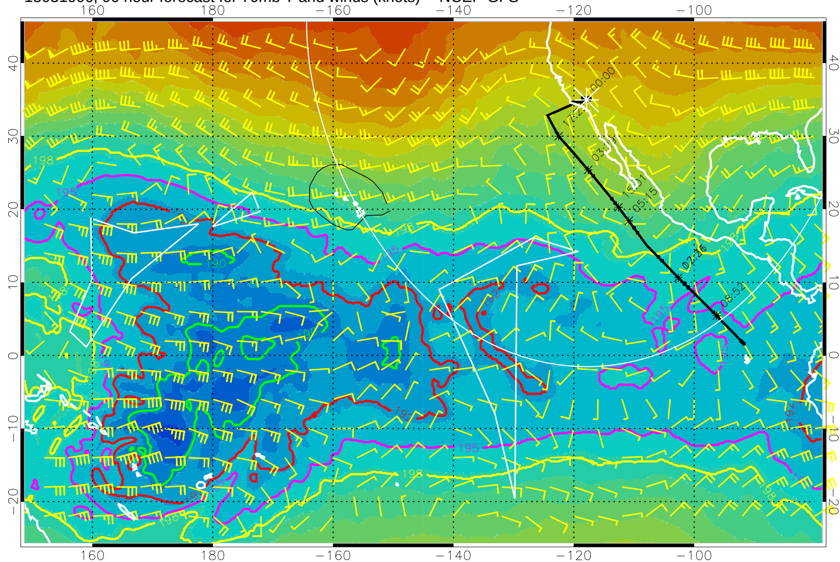
15031006, 90 hour forecast for 70mb T and winds (knots) -- NCEP GFS
