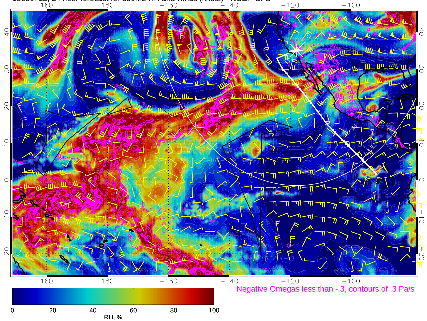
15030712, 24 hour forecast for 500mb RH and winds (knots) - NCEP GFS
