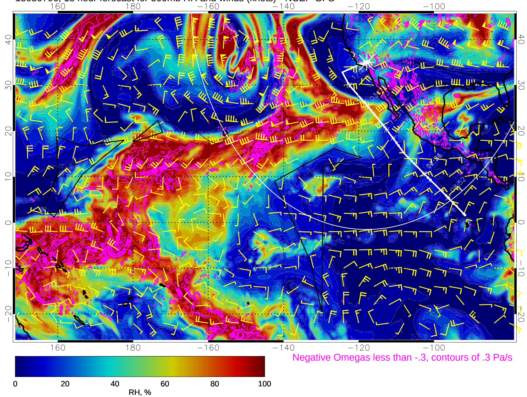
15030706, 18 hour forecast for 500mb RH and winds (knots) - NCEP GFS
