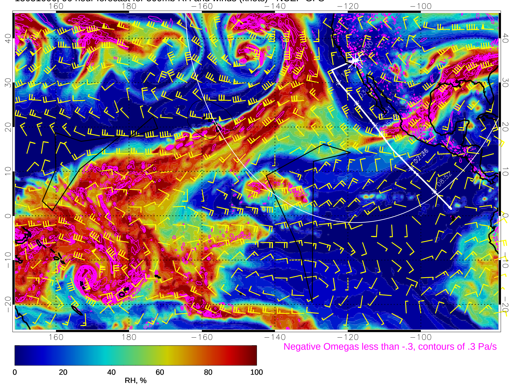
15031006, 90 hour forecast for 500mb RH and winds (knots) - NCEP GFS
