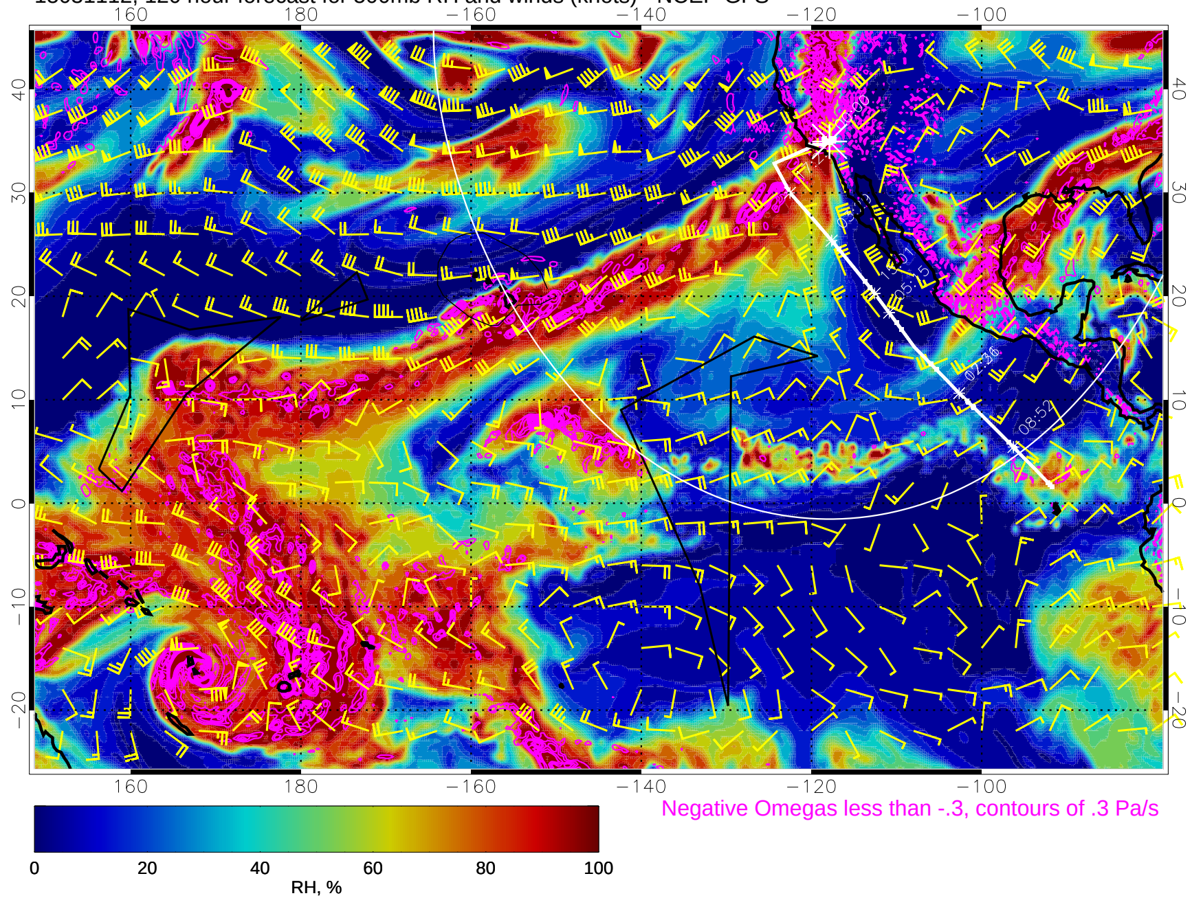
15031112, 120 hour forecast for 500mb RH and winds (knots) - NCEP GFS
