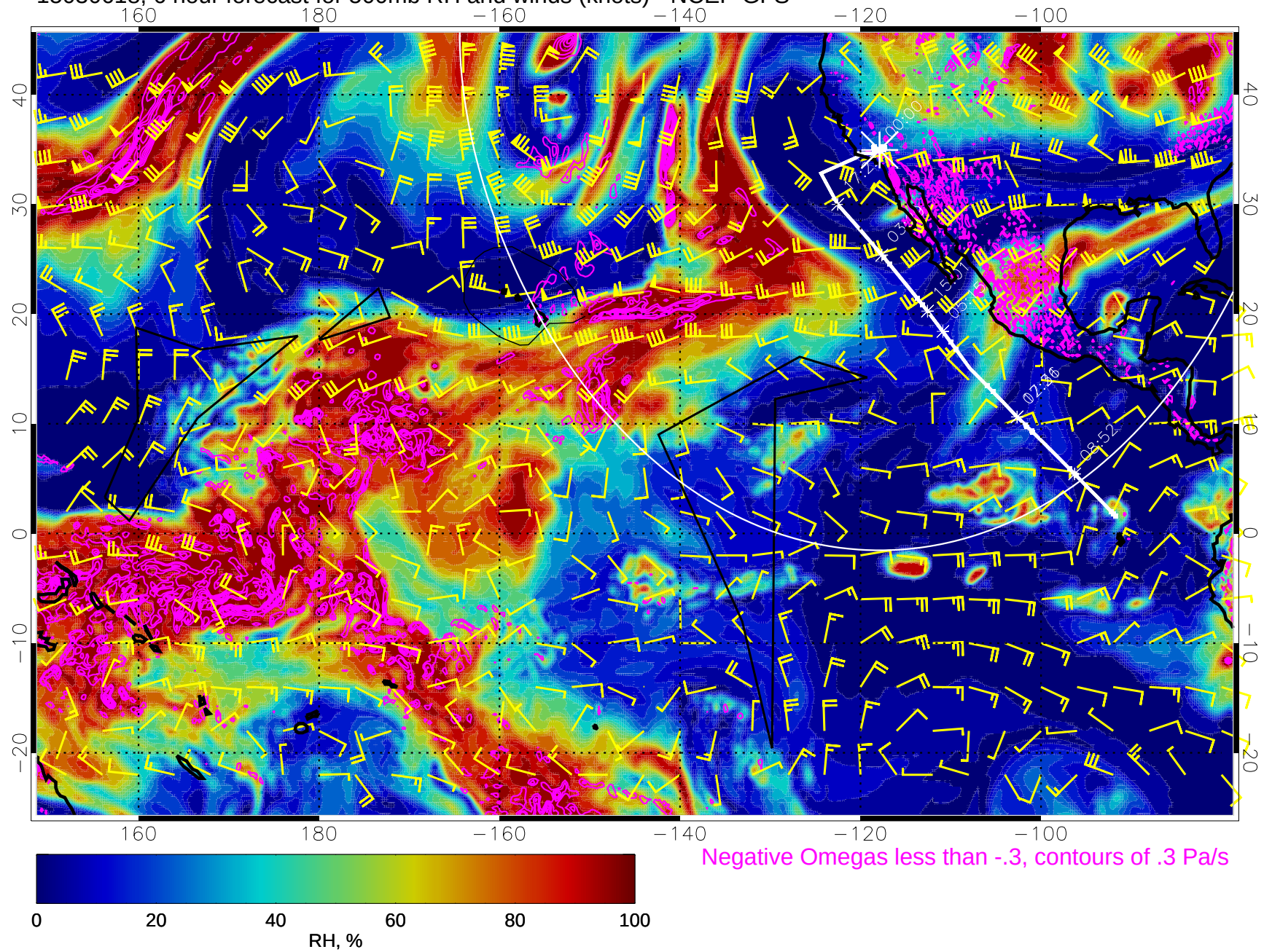
15030618, 6 hour forecast for 500mb RH and winds (knots) - NCEP GFS
