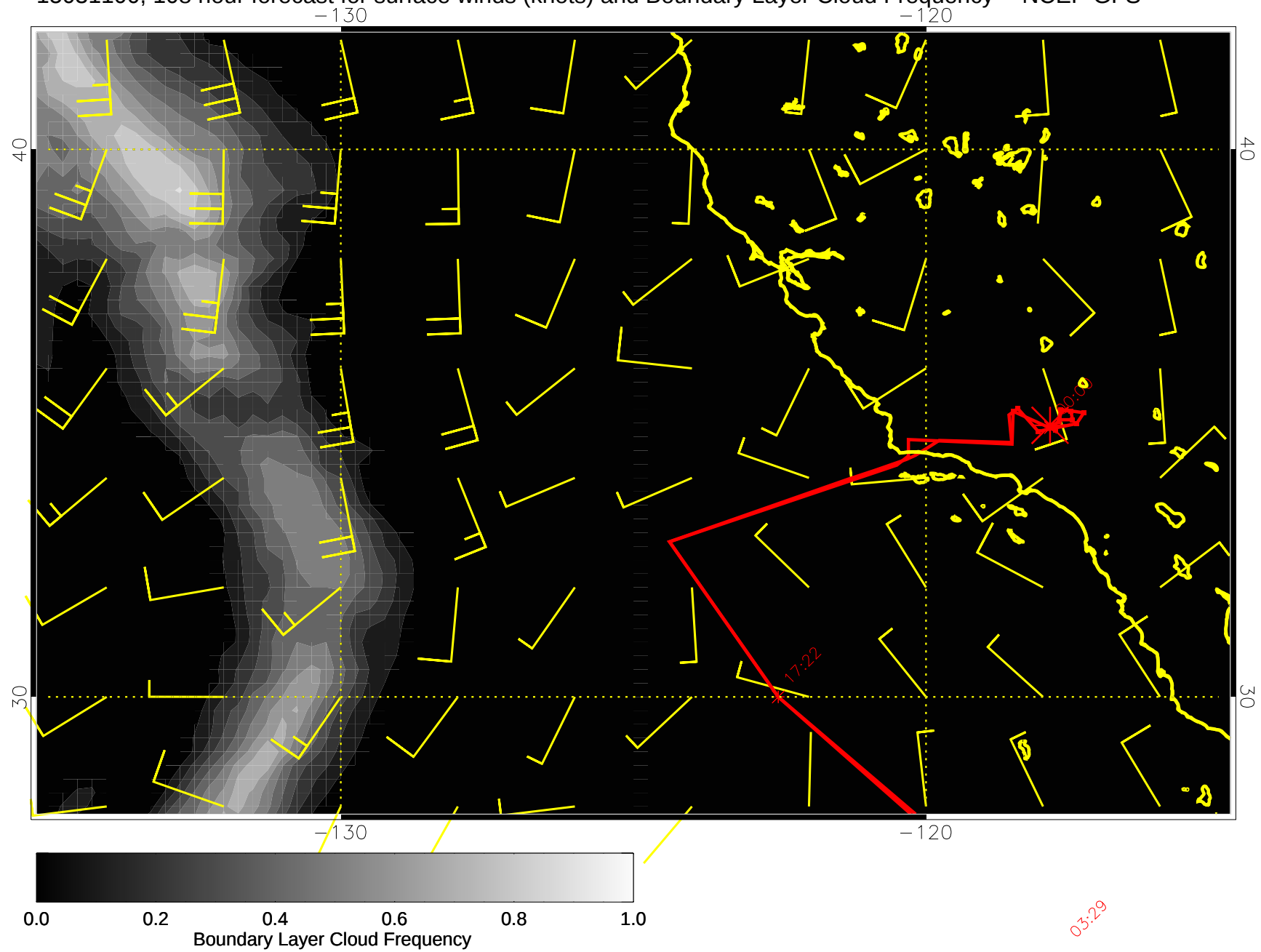
15031100, 108 hour forecast for surface winds (knots) and Boundary Layer Cloud Frequency -- NCEP GFS
