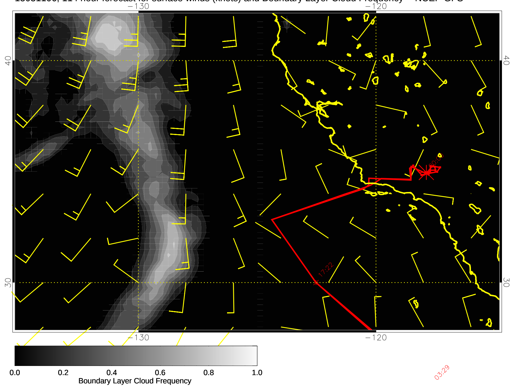
15031106, 114 hour forecast for surface winds (knots) and Boundary Layer Cloud Frequency -- NCEP GFS
