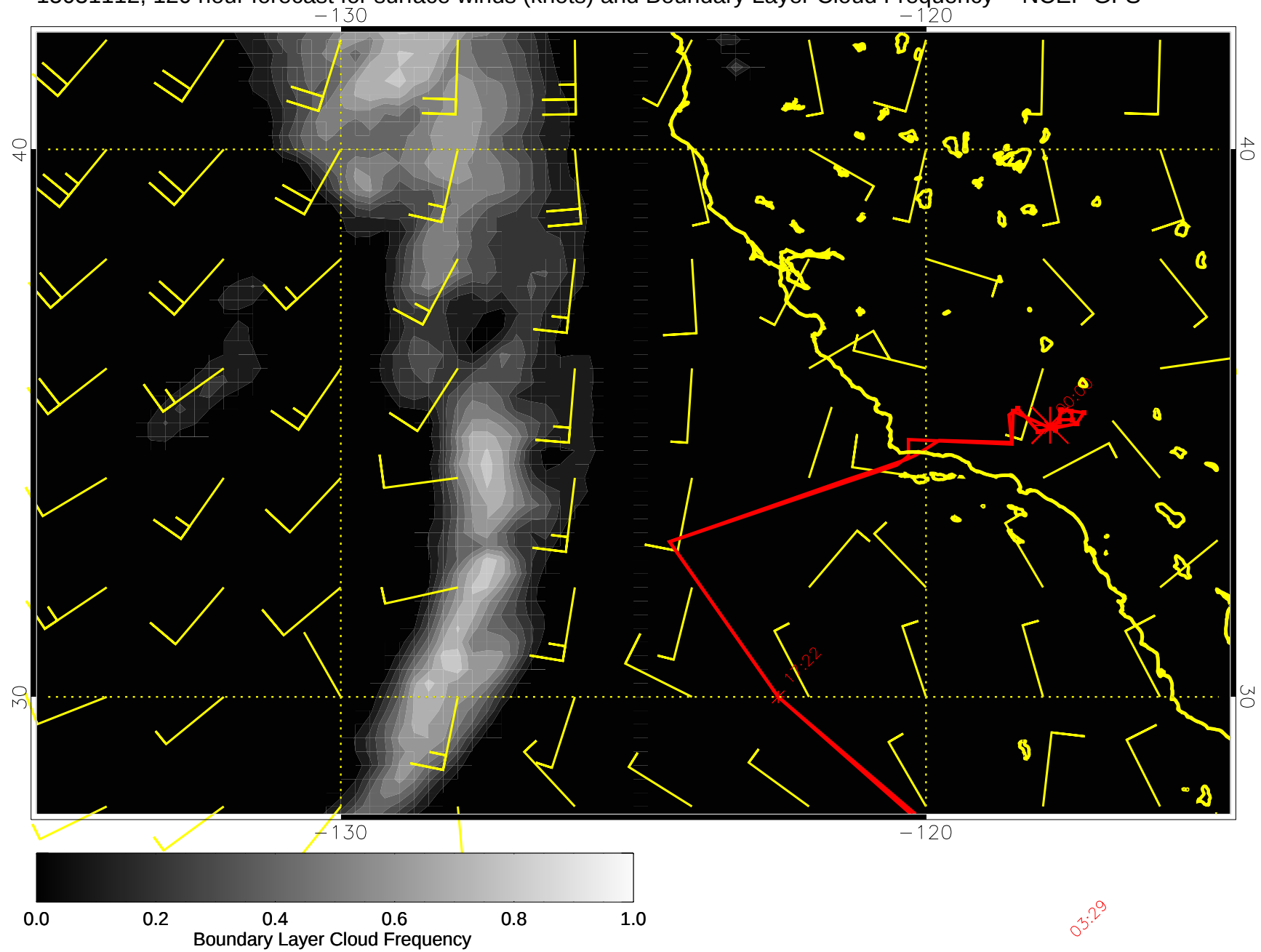
15031112, 120 hour forecast for surface winds (knots) and Boundary Layer Cloud Frequency -- NCEP GFS
