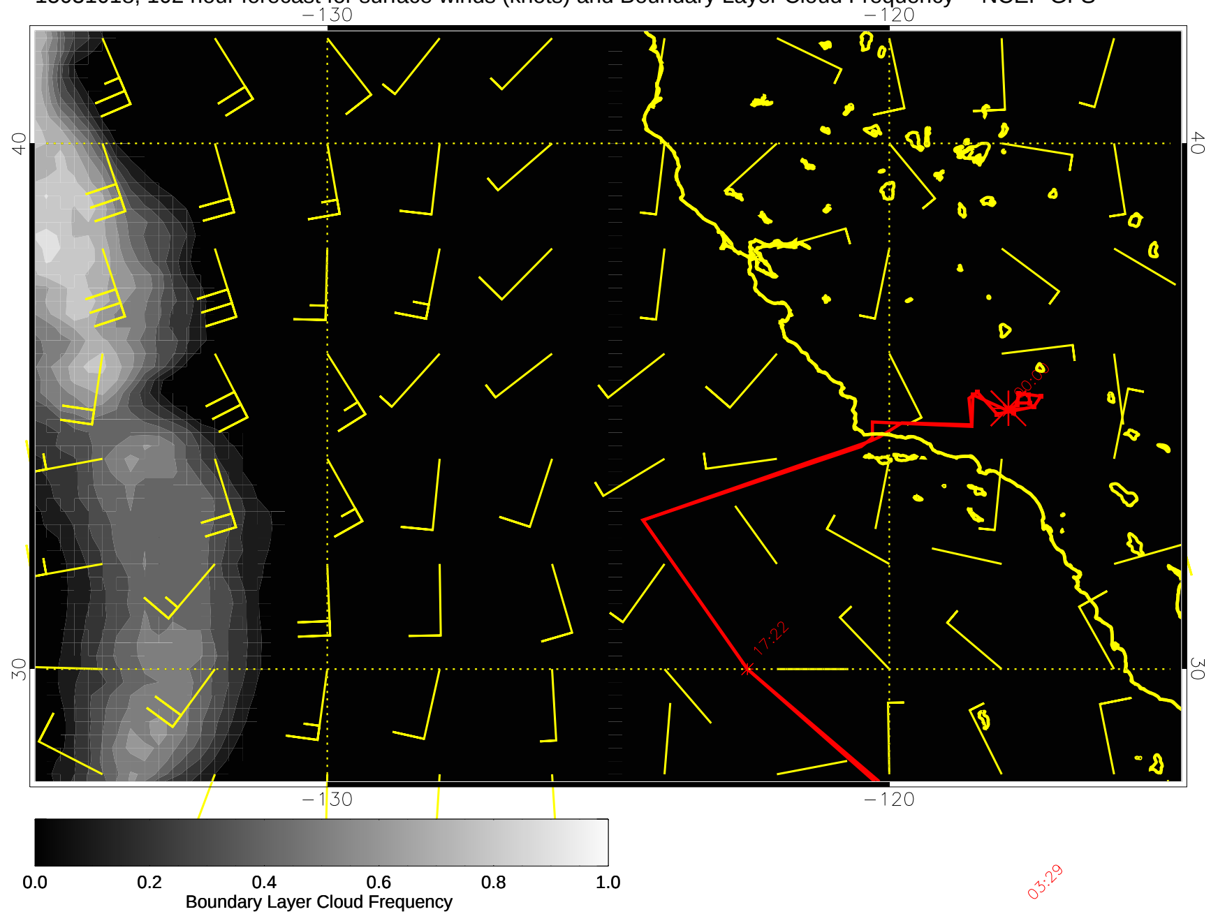
15031018, 102 hour forecast for surface winds (knots) and Boundary Layer Cloud Frequency -- NCEP GFS
