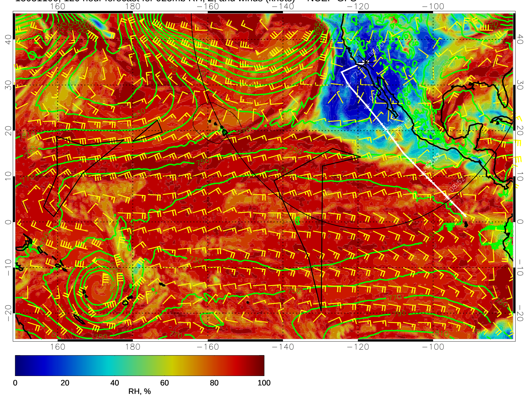
15031100, 120 hour forecast for 925mb RH, Z, and winds (knots) -- NCEP GFS
