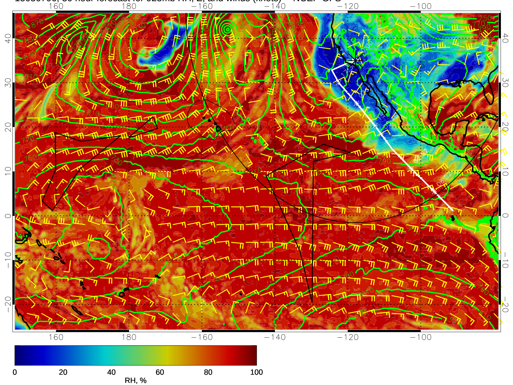
15030706, 30 hour forecast for 925mb RH, Z, and winds (knots) -- NCEP GFS
