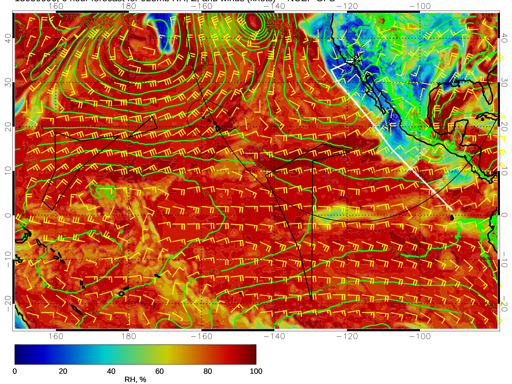
15030606, 6 hour forecast for 925mb RH, Z, and winds (knots) -- NCEP GFS
