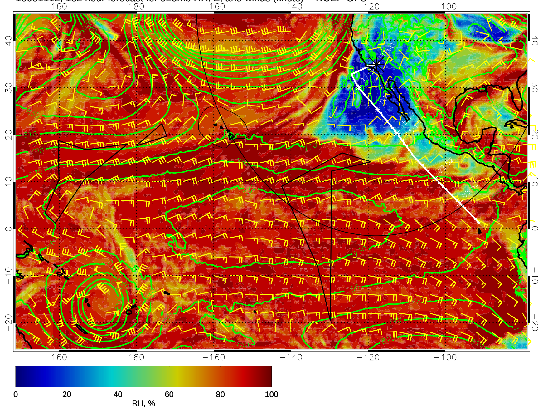
15031112, 132 hour forecast for 925mb RH, Z, and winds (knots) -- NCEP GFS
