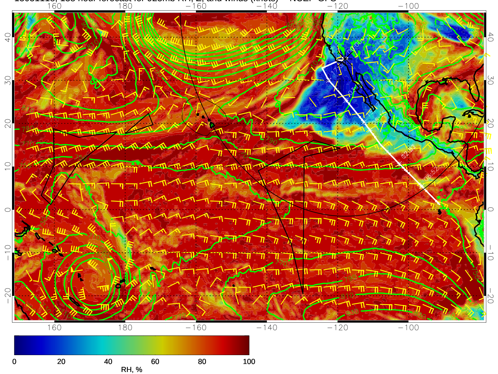
15031118, 138 hour forecast for 925mb RH, Z, and winds (knots) -- NCEP GFS
