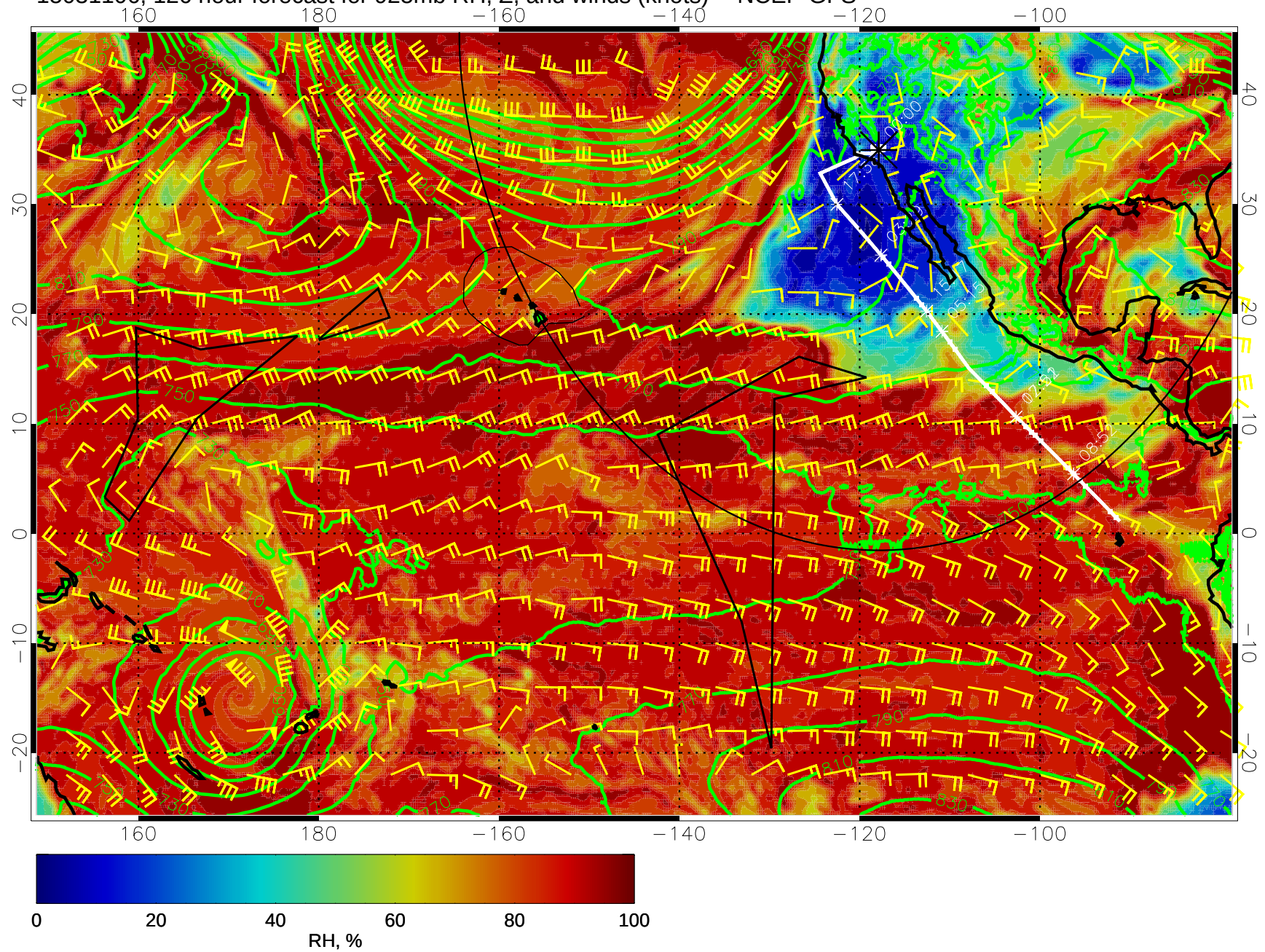
15031106, 126 hour forecast for 925mb RH, Z, and winds (knots) -- NCEP GFS
