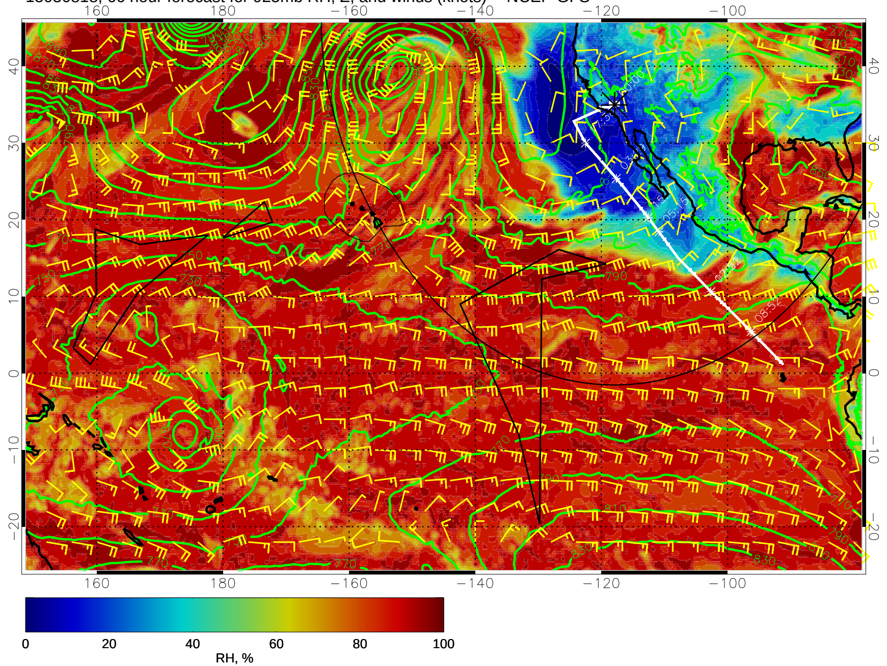
15030818, 66 hour forecast for 925mb RH, Z, and winds (knots) -- NCEP GFS
