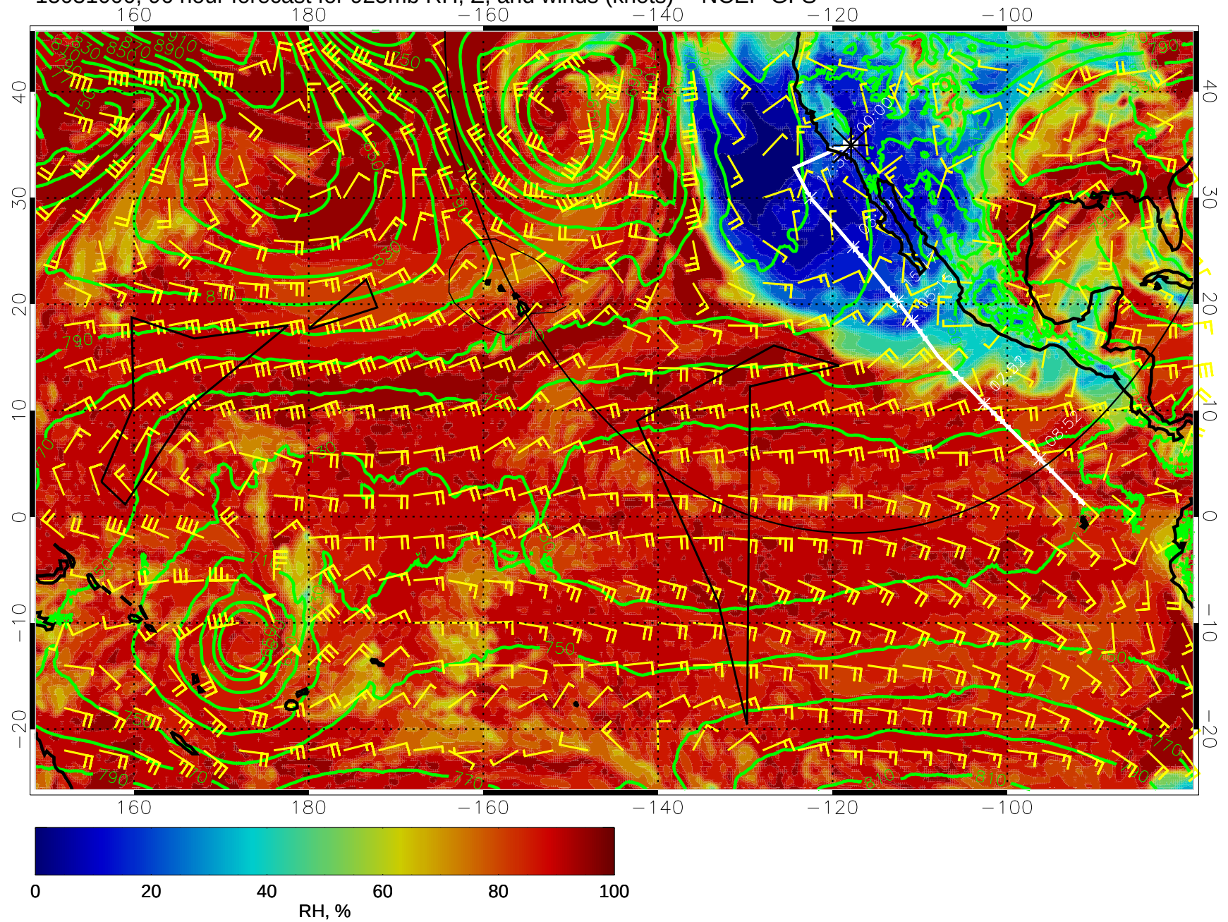
15031000, 96 hour forecast for 925mb RH, Z, and winds (knots) -- NCEP GFS
