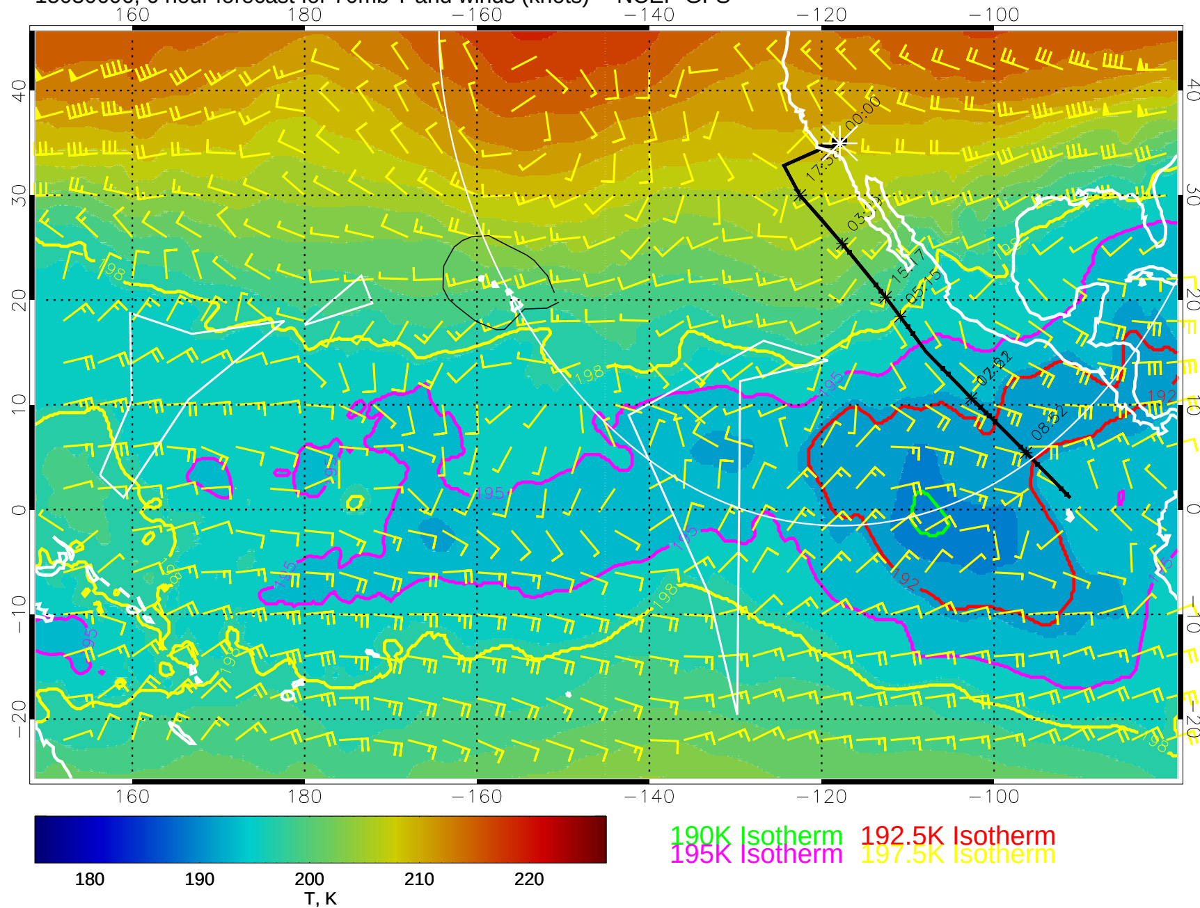
15030606, 6 hour forecast for 70mb T and winds (knots) -- NCEP GFS
