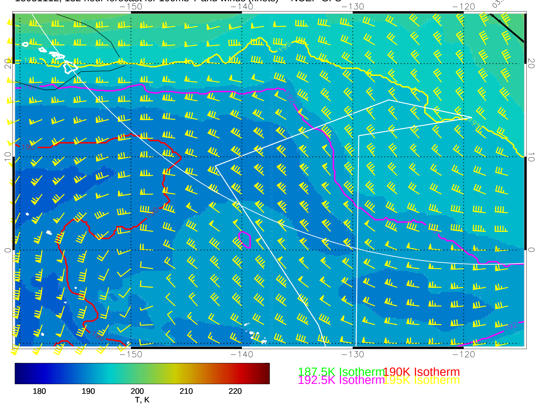
15031112, 132 hour forecast for 100mb T and winds (knots) -- NCEP GFS
