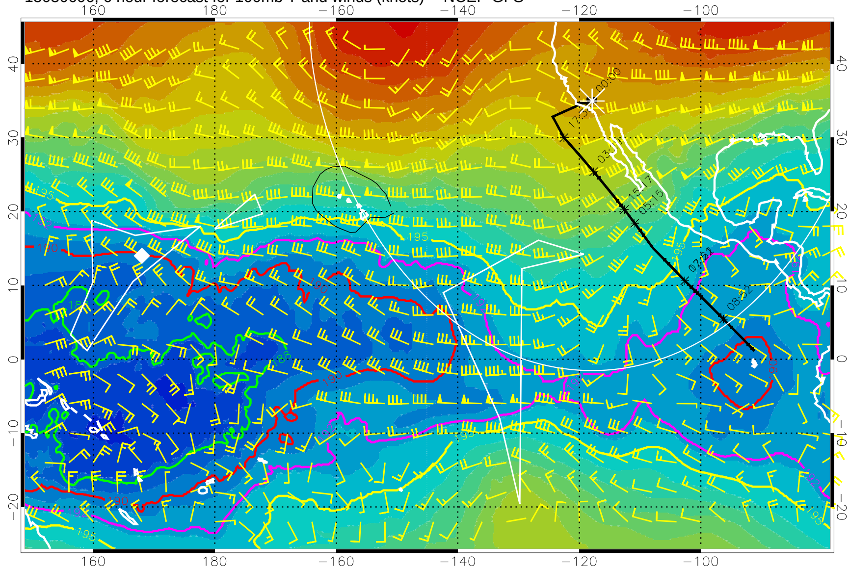
15030606, 6 hour forecast for 100mb T and winds (knots) -- NCEP GFS
