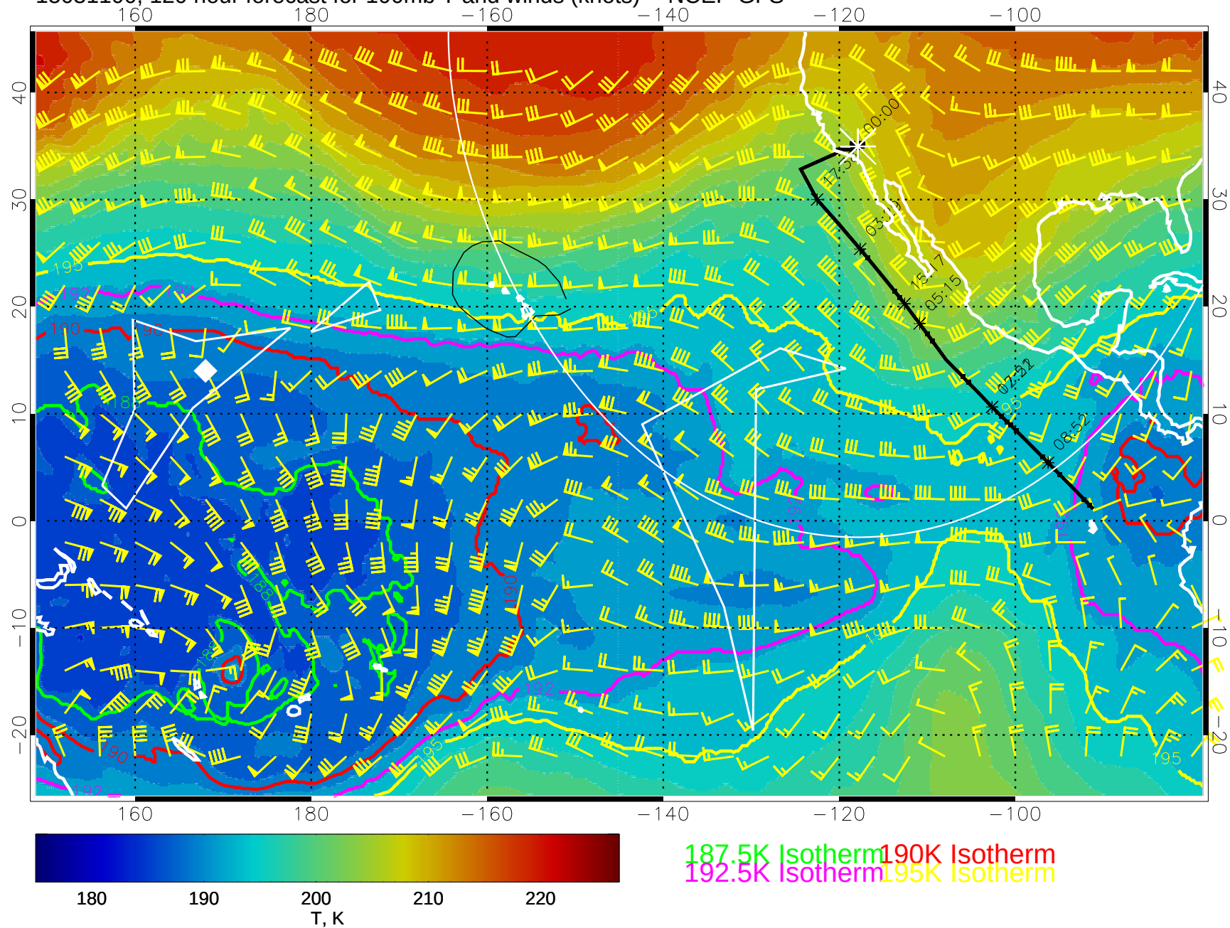
15031100, 120 hour forecast for 100mb T and winds (knots) -- NCEP GFS
