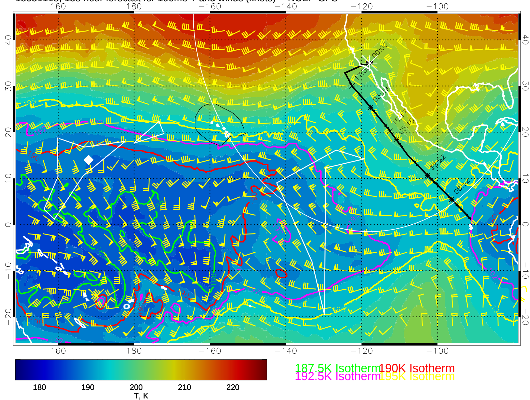
15031118, 138 hour forecast for 100mb T and winds (knots) -- NCEP GFS
