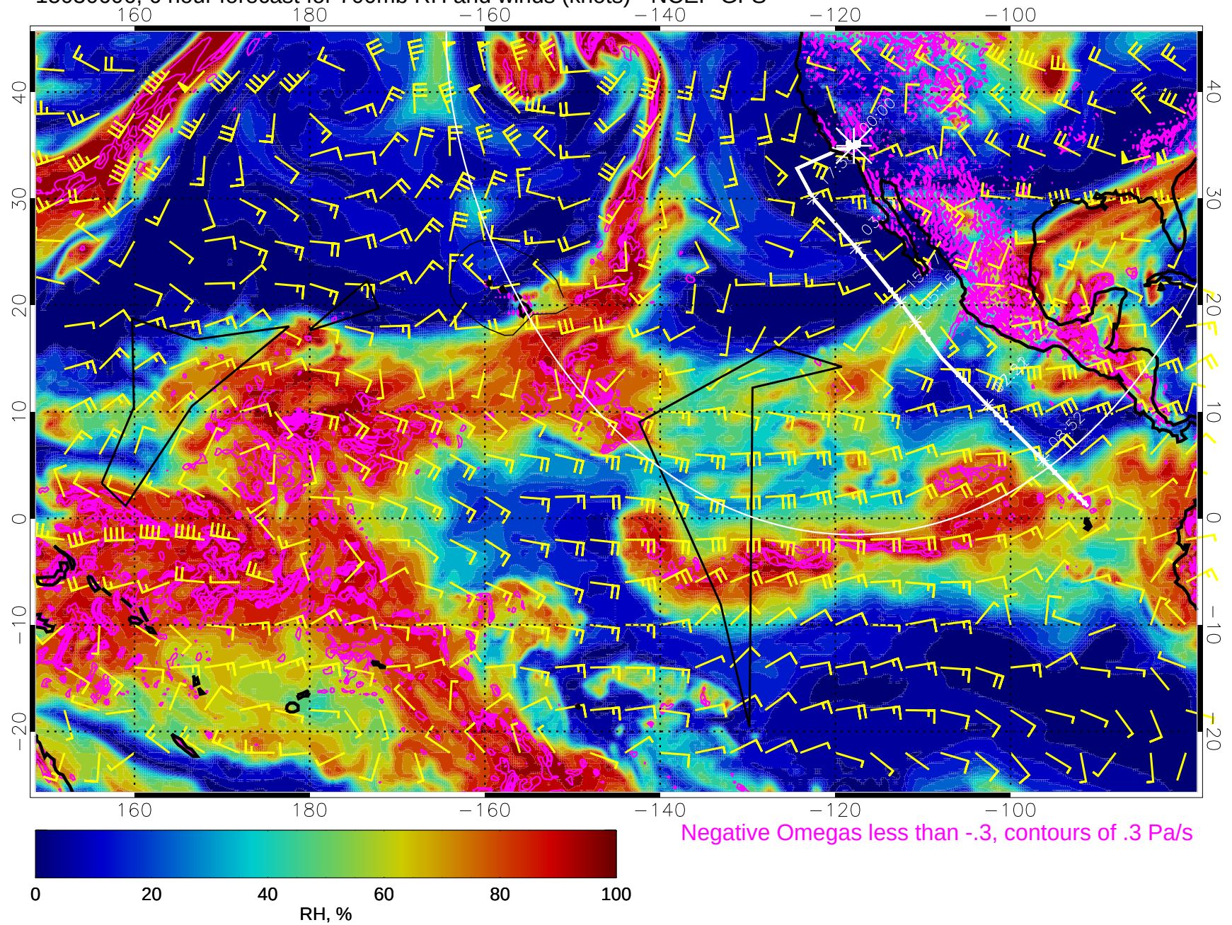
15030606, 6 hour forecast for 700mb RH and winds (knots) - NCEP GFS
