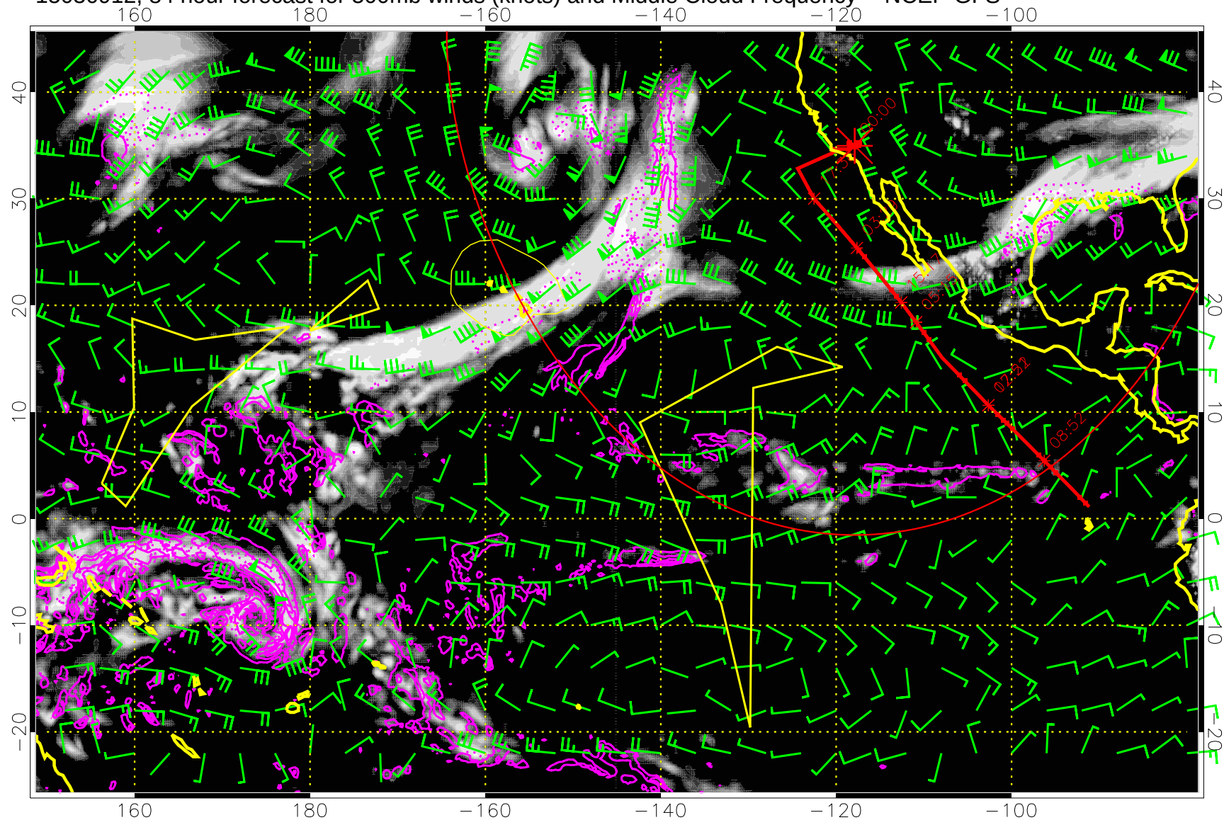
15030912, 84 hour forecast for 500mb winds (knots) and Middle Cloud Frequency -- NCEP GFS
