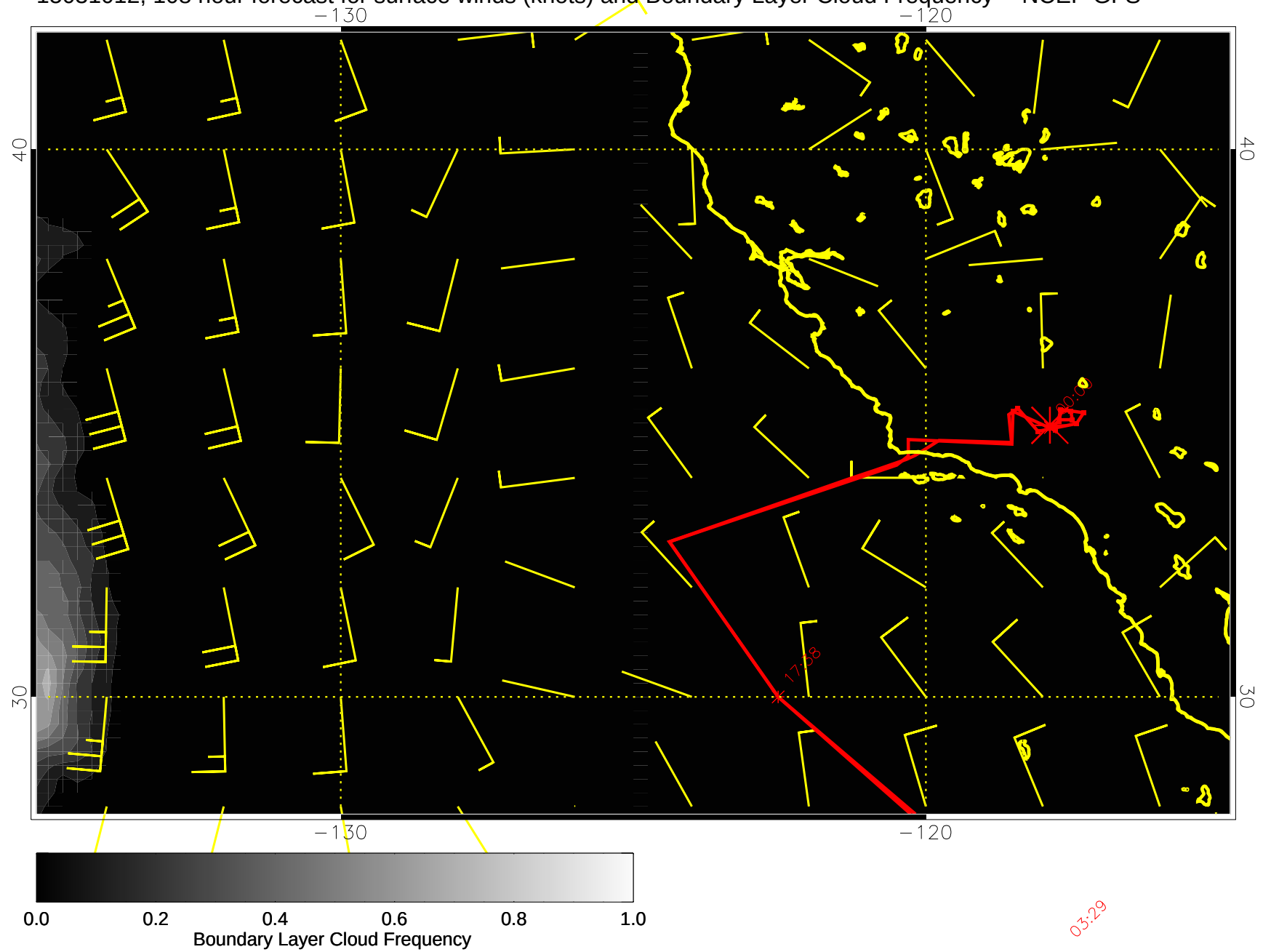
15031012, 108 hour forecast for surface winds (knots) and Boundary Layer Cloud Frequency -- NCEP GFS
