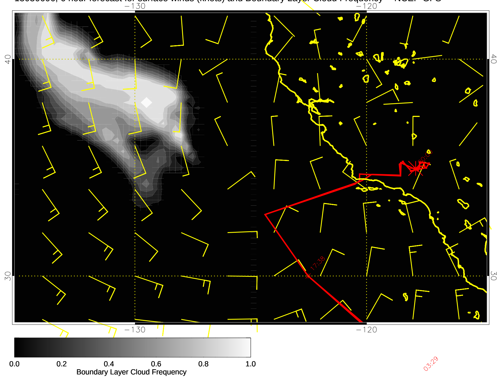
15030606, 6 hour forecast for surface winds (knots) and Boundary Layer Cloud Frequency -- NCEP GFS
