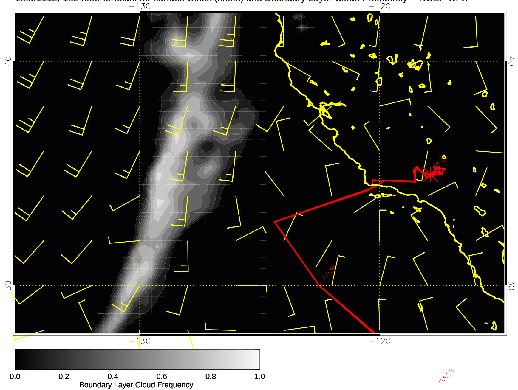
15031112, 132 hour forecast for surface winds (knots) and Boundary Layer Cloud Frequency -- NCEP GFS
