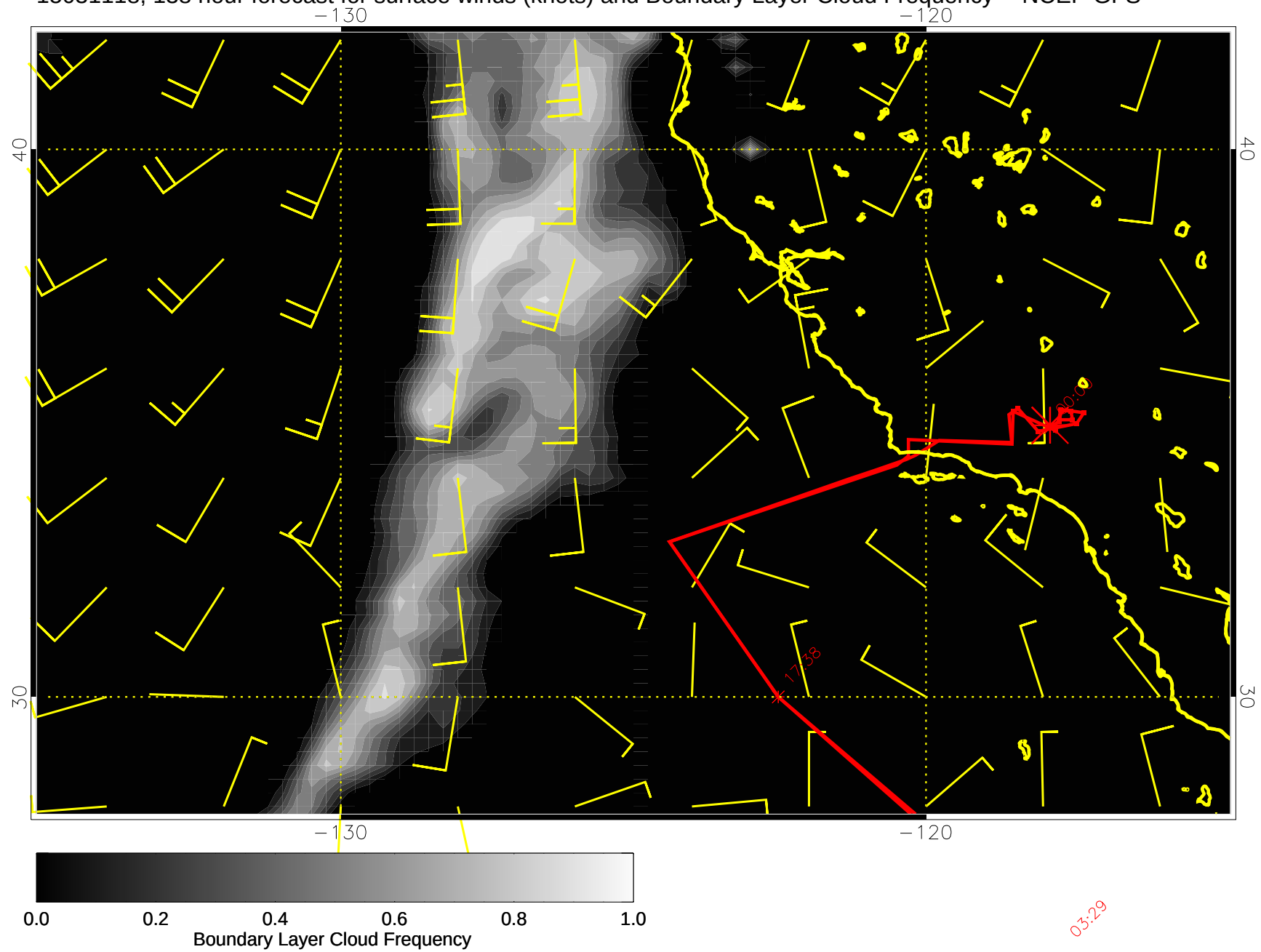
15031118, 138 hour forecast for surface winds (knots) and Boundary Layer Cloud Frequency -- NCEP GFS
