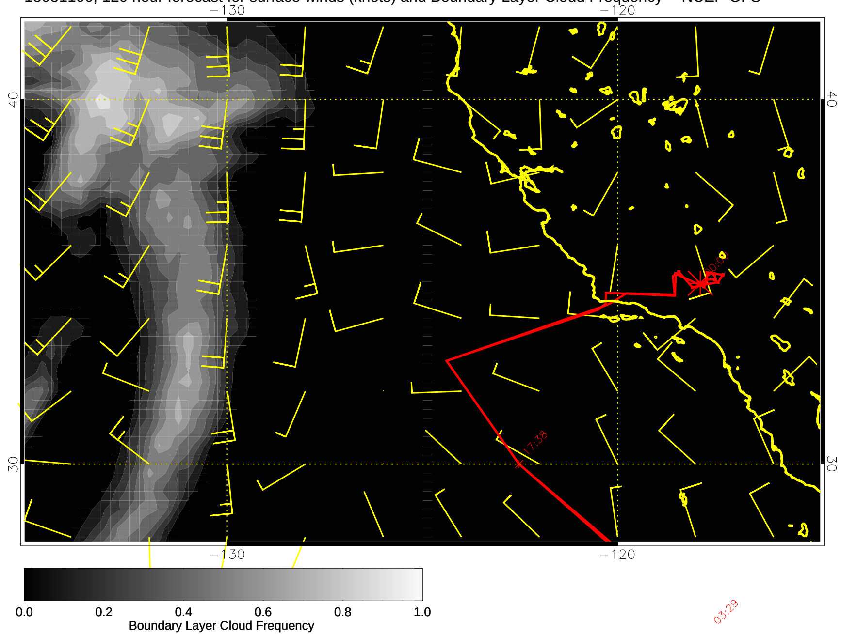
15031100, 120 hour forecast for surface winds (knots) and Boundary Layer Cloud Frequency -- NCEP GFS
