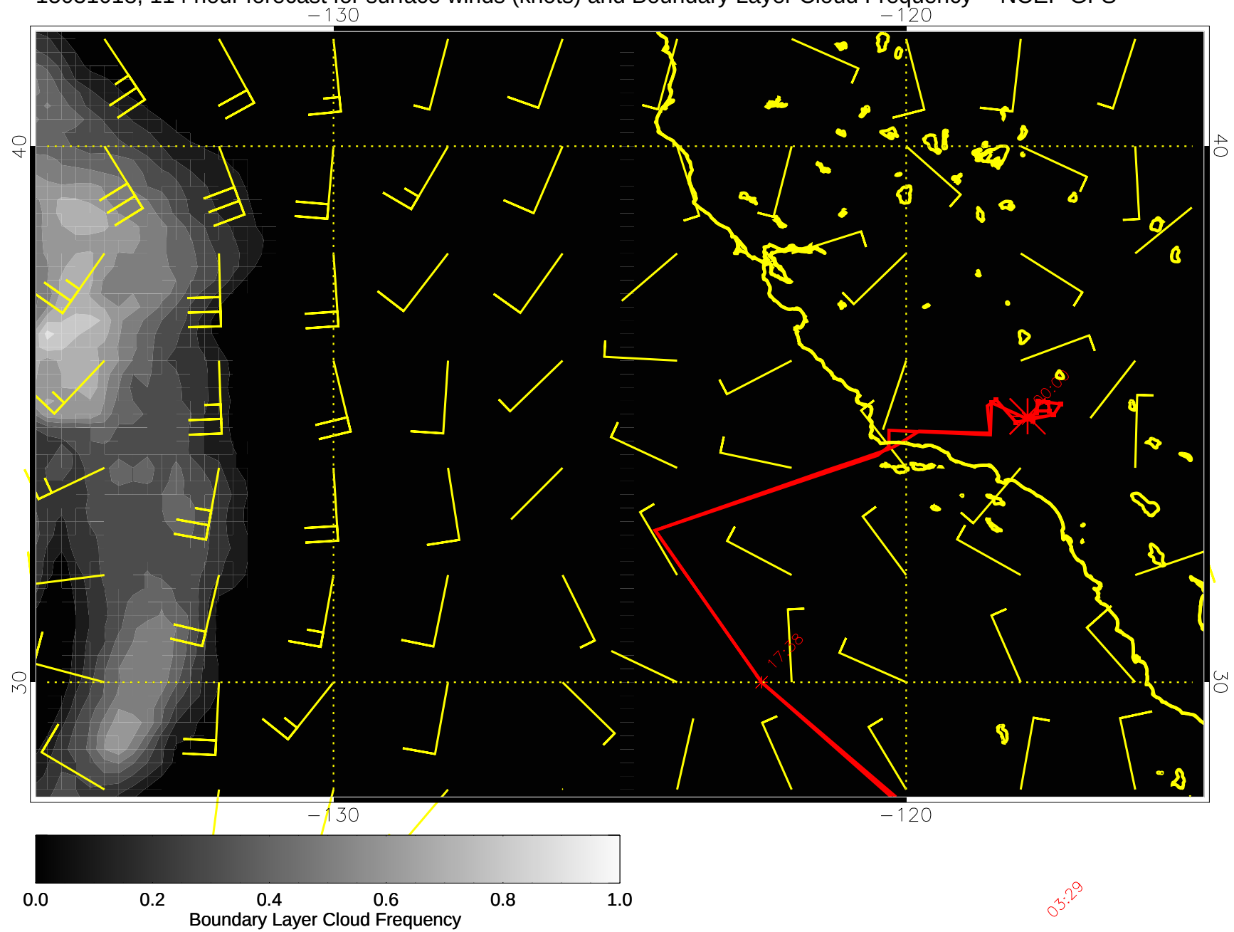
15031018, 114 hour forecast for surface winds (knots) and Boundary Layer Cloud Frequency -- NCEP GFS
