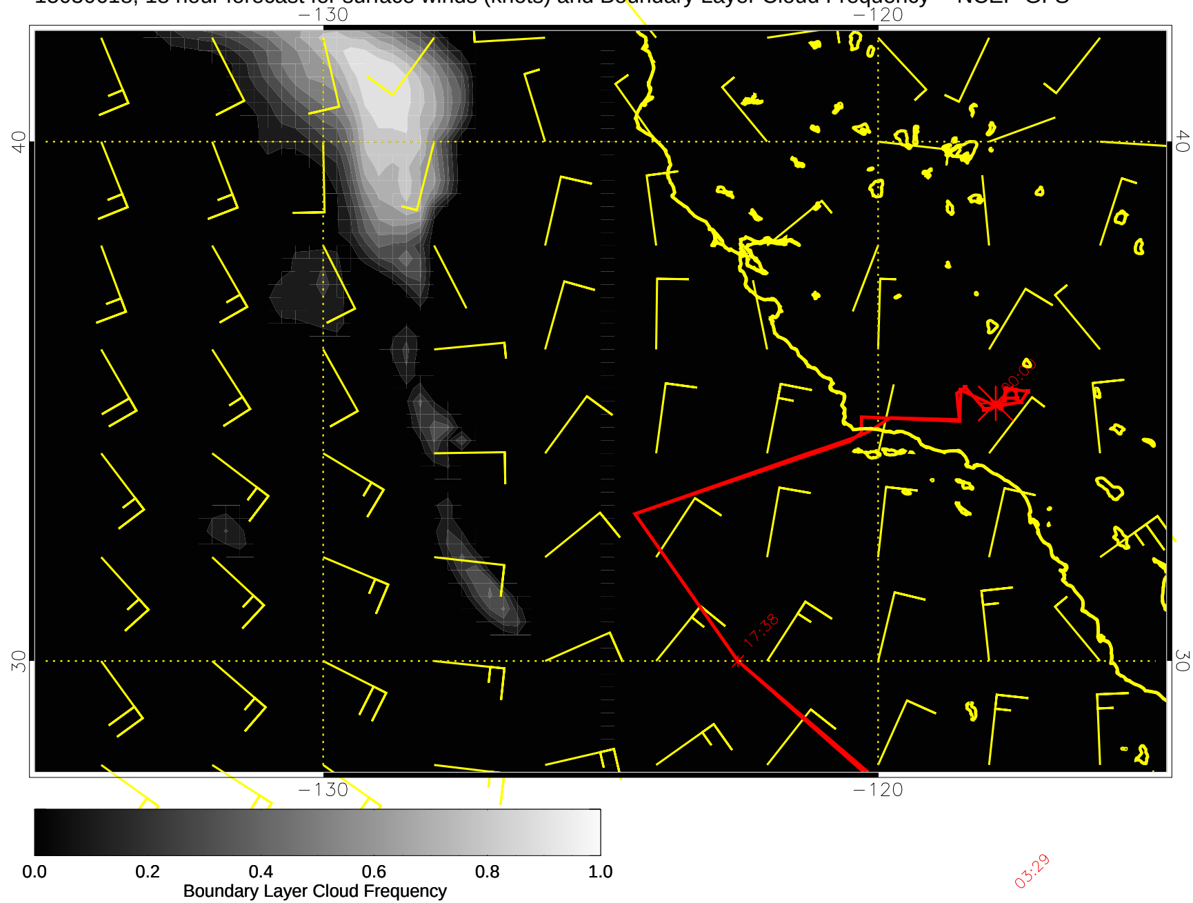
15030618, 18 hour forecast for surface winds (knots) and Boundary Layer Cloud Frequency -- NCEP GFS
