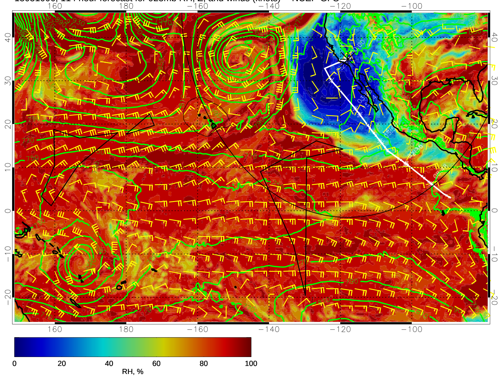
15031006, 114 hour forecast for 925mb RH, Z, and winds (knots) -- NCEP GFS
