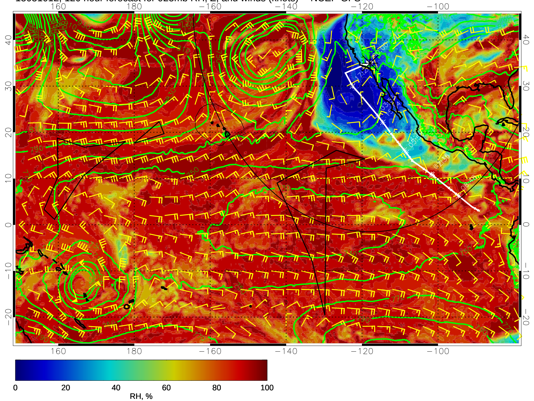
15031012, 120 hour forecast for 925mb RH, Z, and winds (knots) -- NCEP GFS
