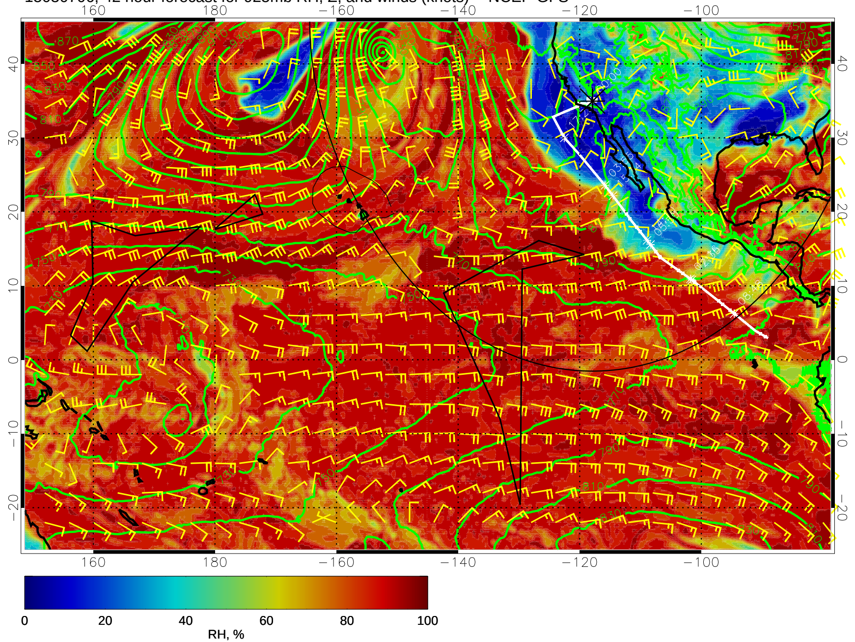
15030706, 42 hour forecast for 925mb RH, Z, and winds (knots) -- NCEP GFS
