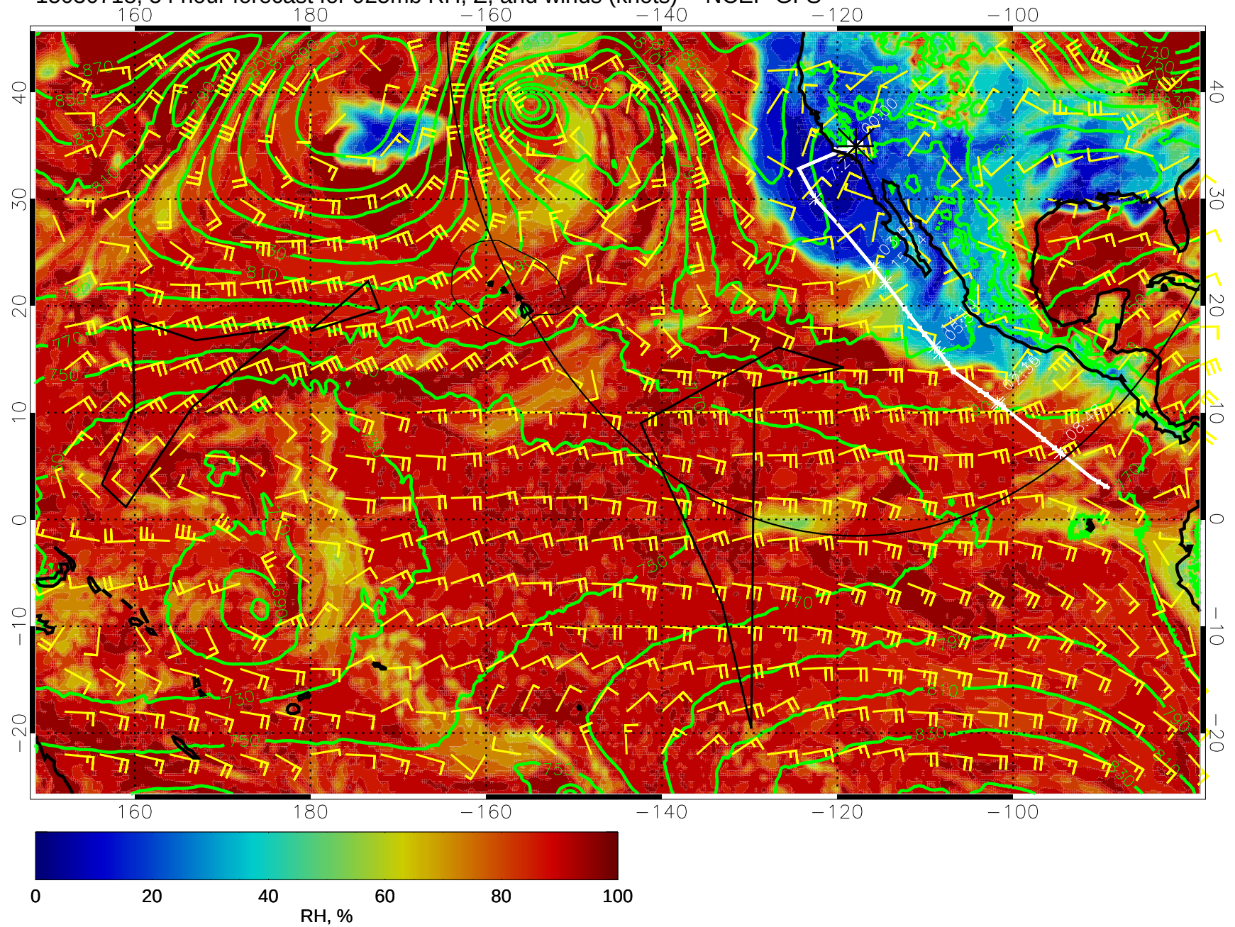
15030718, 54 hour forecast for 925mb RH, Z, and winds (knots) -- NCEP GFS
