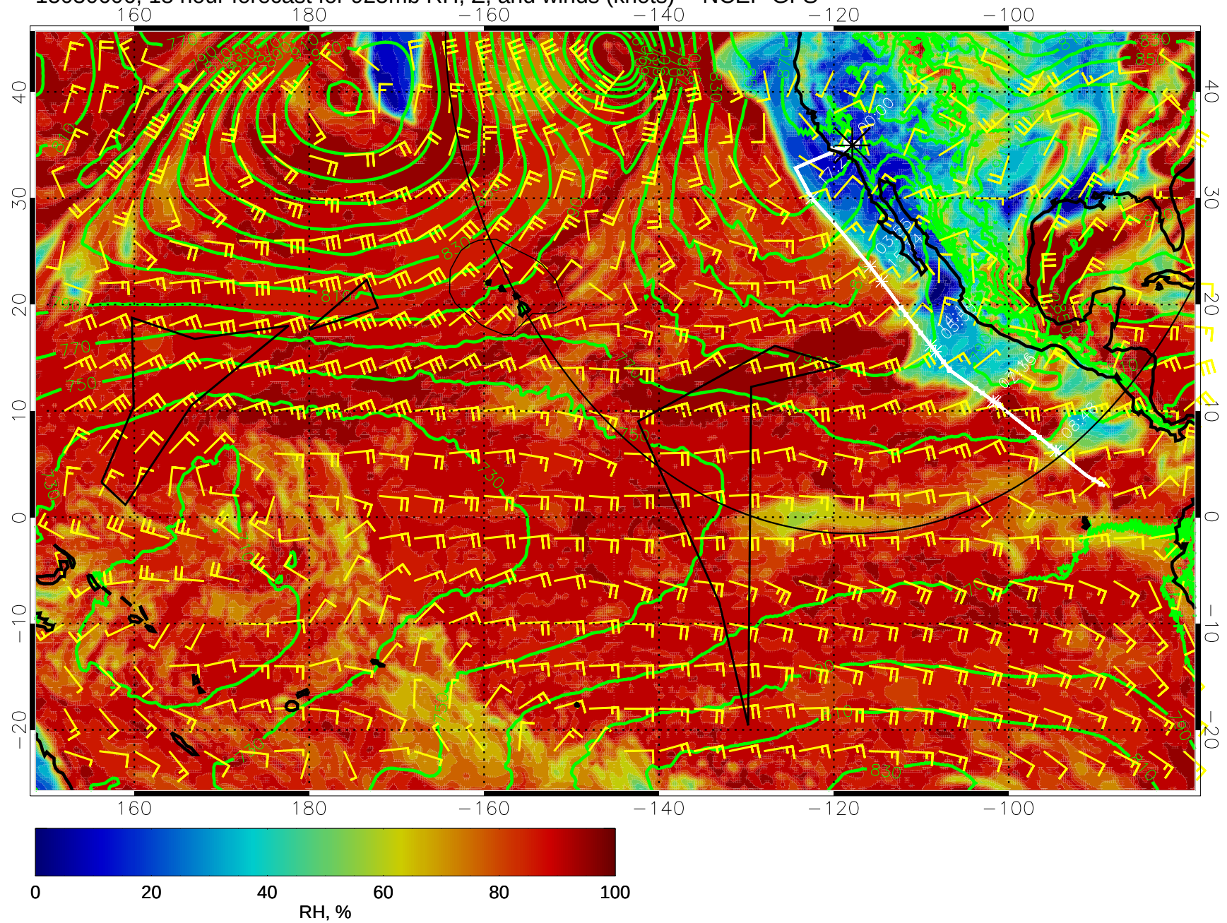
15030606, 18 hour forecast for 925mb RH, Z, and winds (knots) -- NCEP GFS
