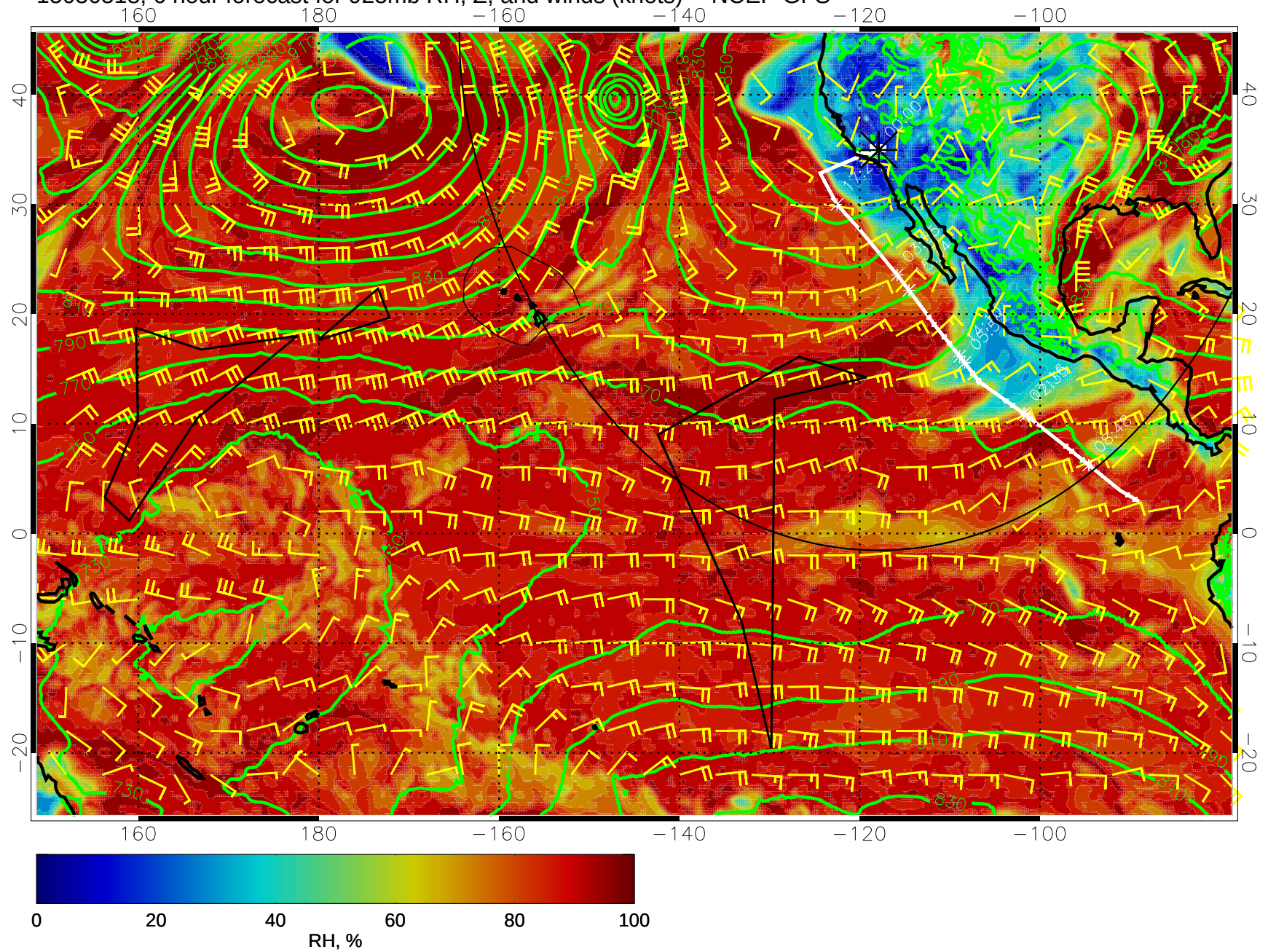
15030518, 6 hour forecast for 925mb RH, Z, and winds (knots) -- NCEP GFS
