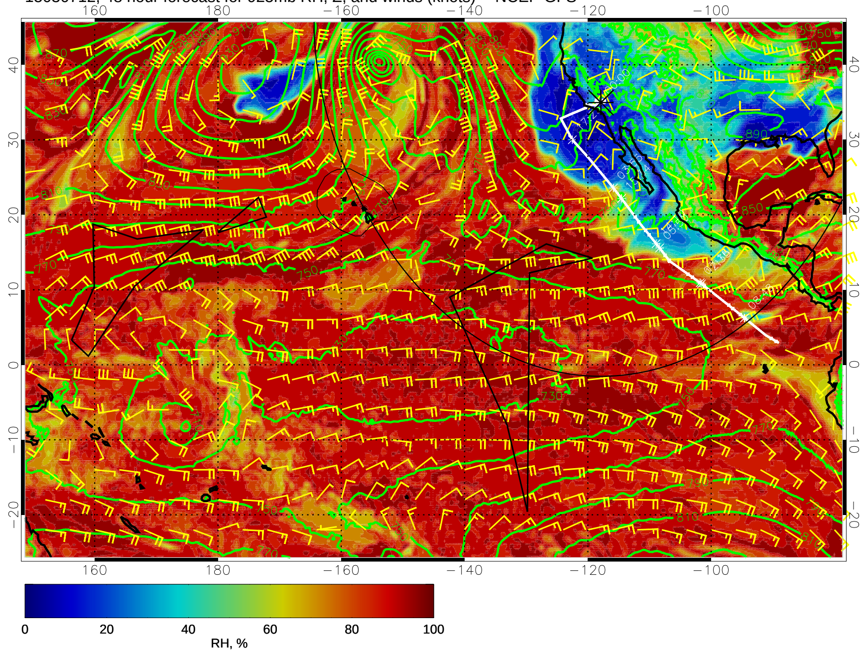
15030712, 48 hour forecast for 925mb RH, Z, and winds (knots) -- NCEP GFS
