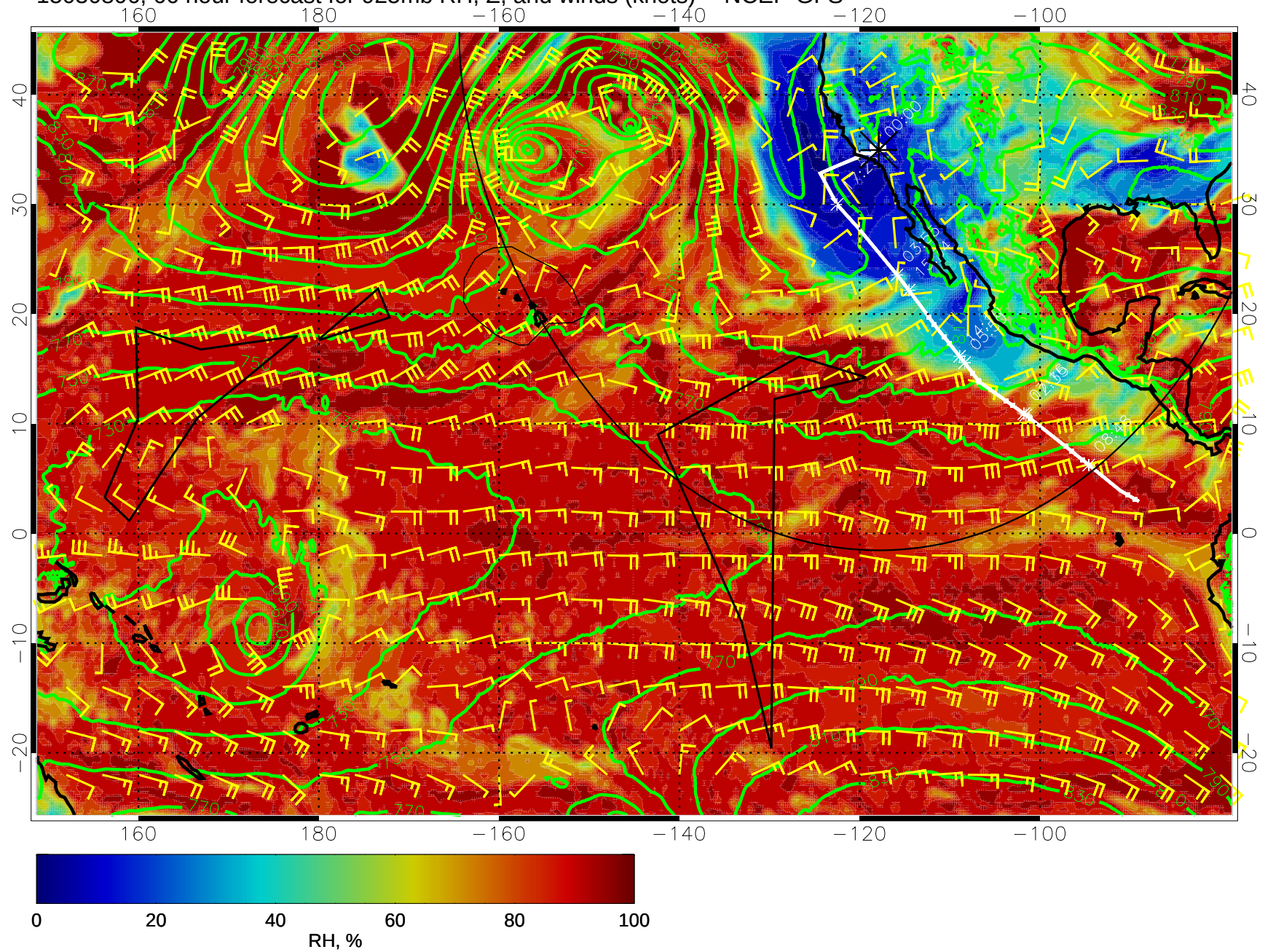
15030806, 66 hour forecast for 925mb RH, Z, and winds (knots) -- NCEP GFS
