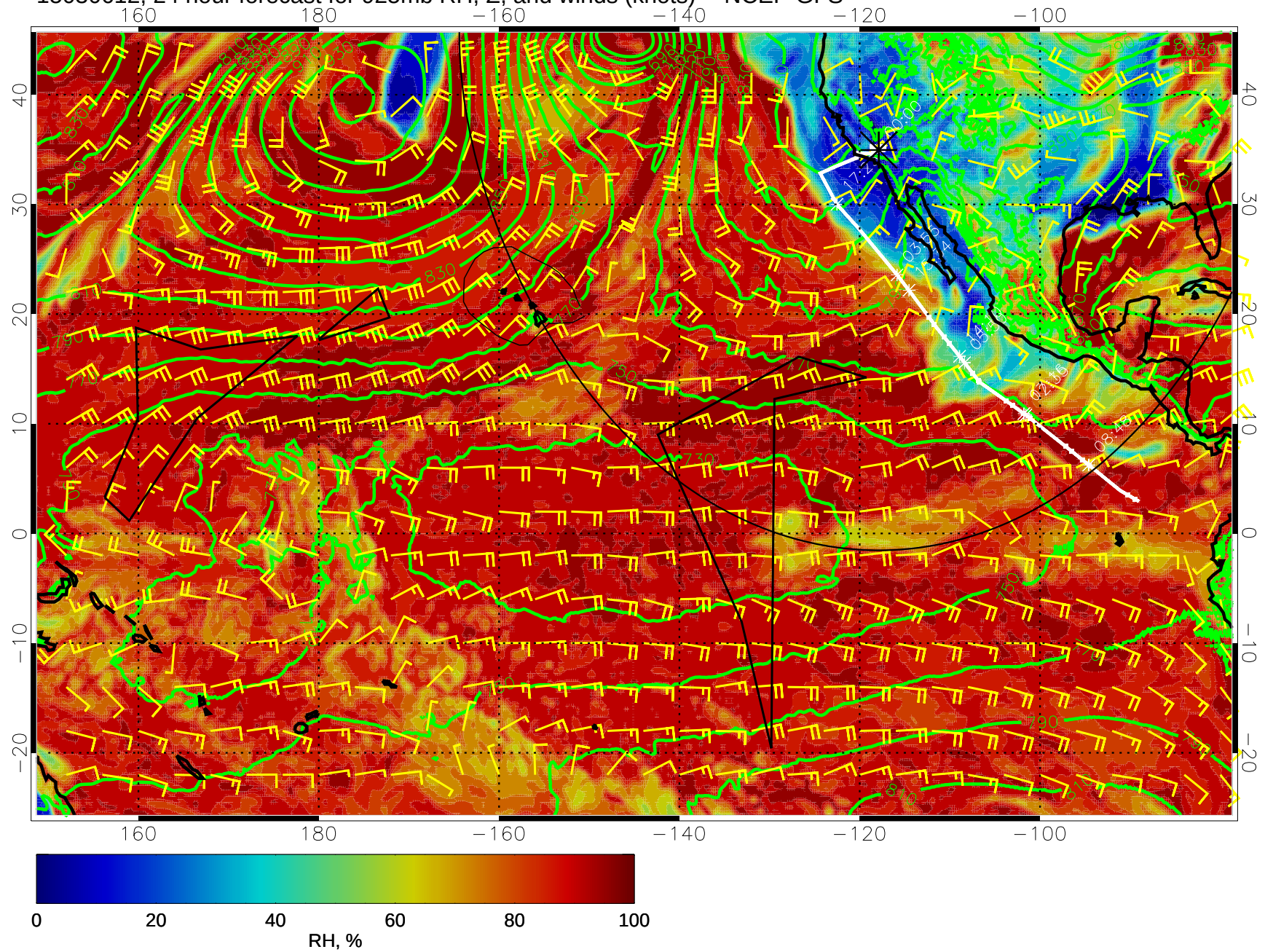
15030612, 24 hour forecast for 925mb RH, Z, and winds (knots) -- NCEP GFS
