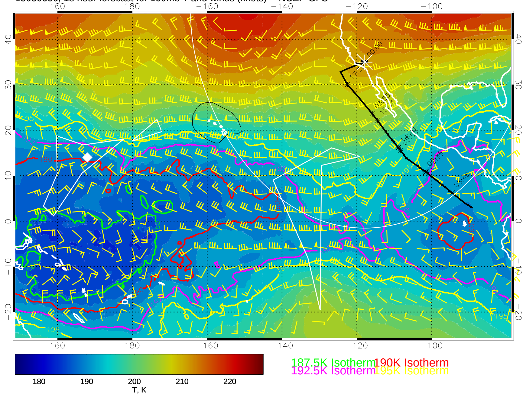
15030606, 18 hour forecast for 100mb T and winds (knots) -- NCEP GFS
