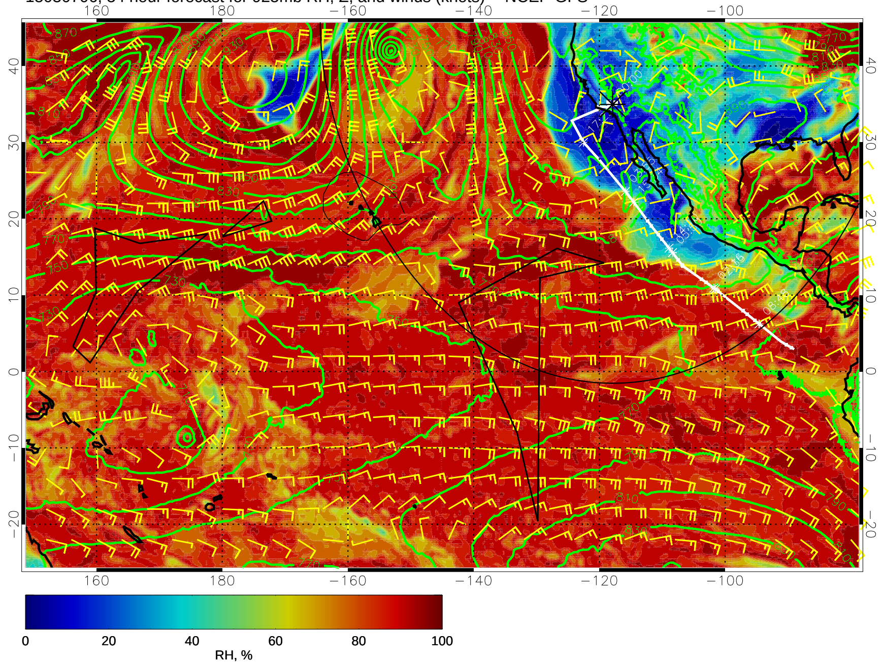
15030706, 54 hour forecast for 925mb RH, Z, and winds (knots) -- NCEP GFS
