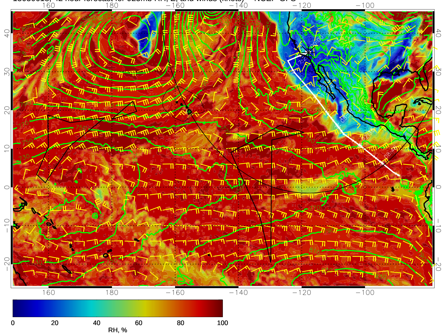
15030618, 42 hour forecast for 925mb RH, Z, and winds (knots) -- NCEP GFS
