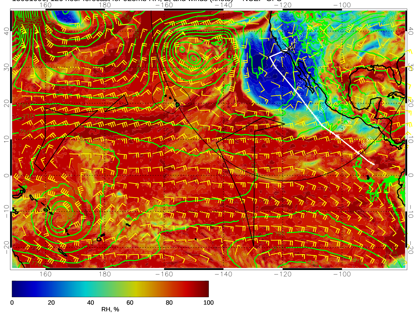
15031006, 126 hour forecast for 925mb RH, Z, and winds (knots) -- NCEP GFS
