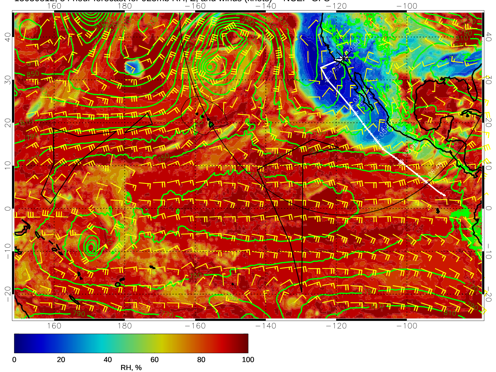
15030812, 84 hour forecast for 925mb RH, Z, and winds (knots) -- NCEP GFS
