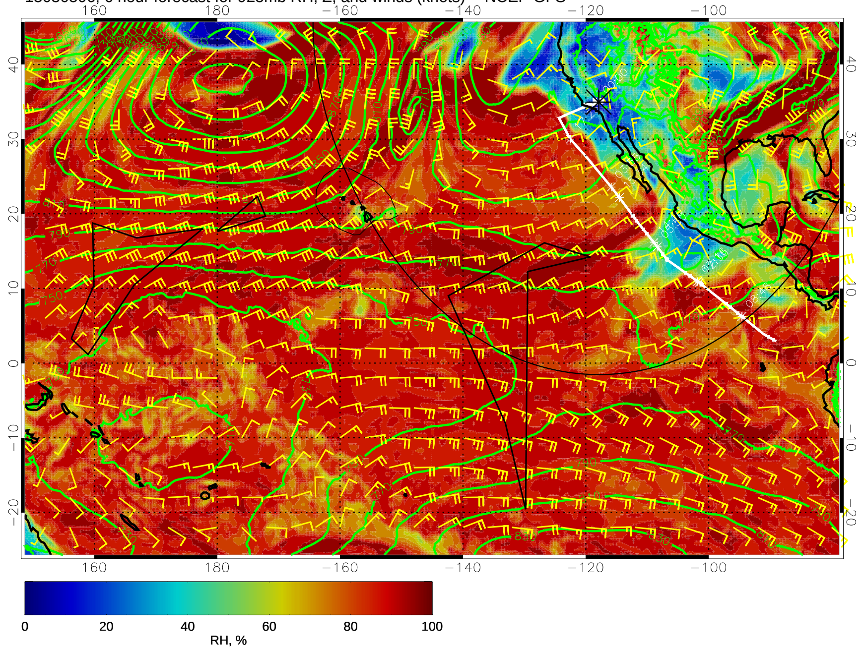
15030506, 6 hour forecast for 925mb RH, Z, and winds (knots) -- NCEP GFS
