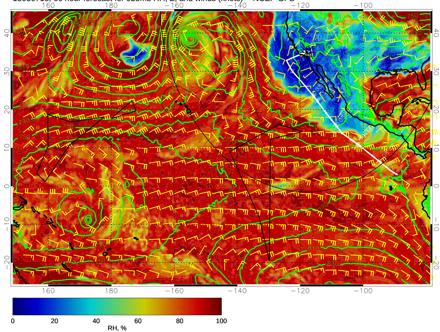
15030718, 66 hour forecast for 925mb RH, Z, and winds (knots) -- NCEP GFS
