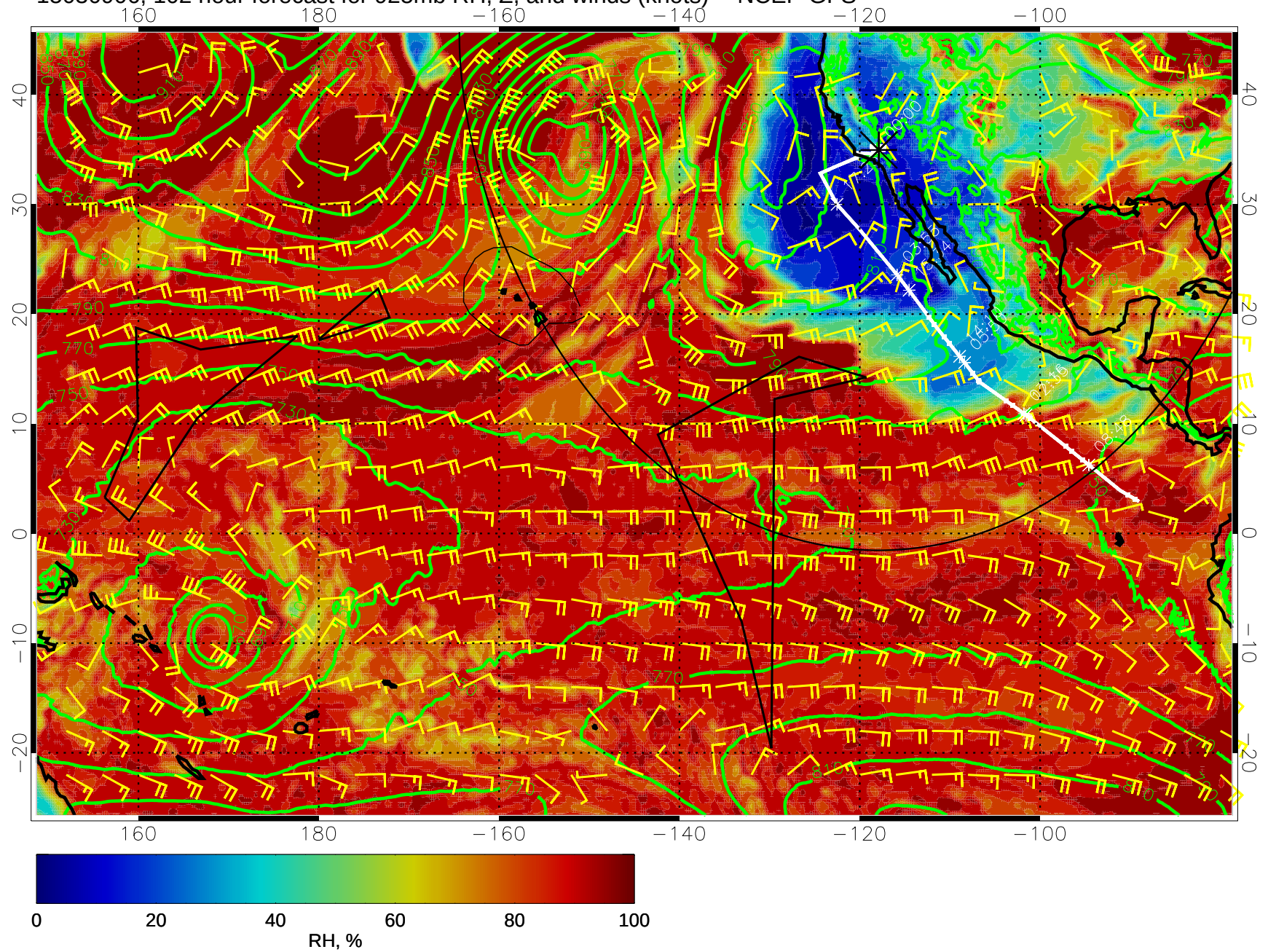
15030906, 102 hour forecast for 925mb RH, Z, and winds (knots) -- NCEP GFS
