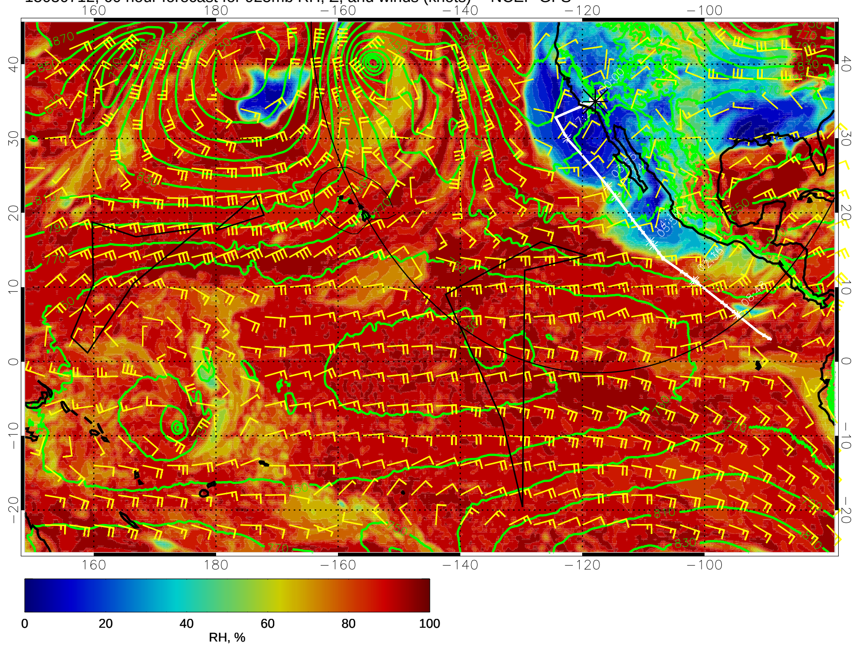
15030712, 60 hour forecast for 925mb RH, Z, and winds (knots) -- NCEP GFS
