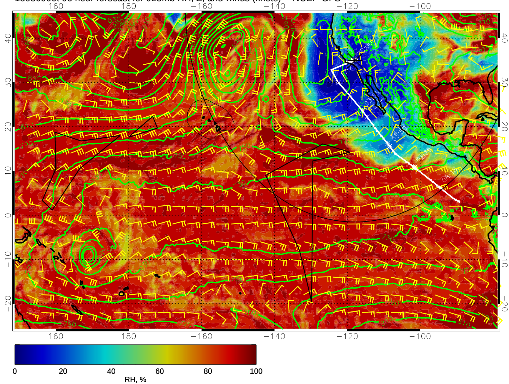
15030900, 96 hour forecast for 925mb RH, Z, and winds (knots) -- NCEP GFS
