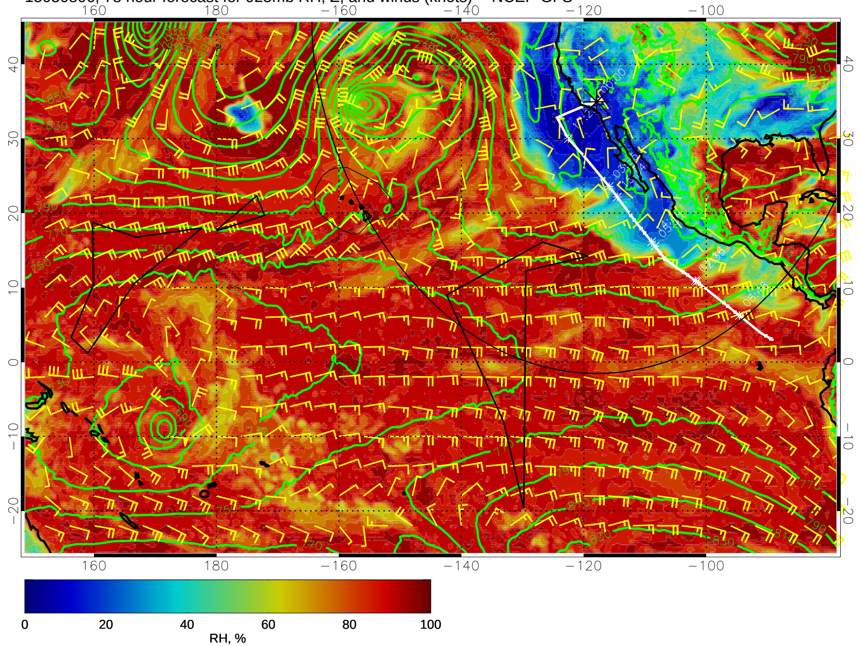
15030806, 78 hour forecast for 925mb RH, Z, and winds (knots) -- NCEP GFS
