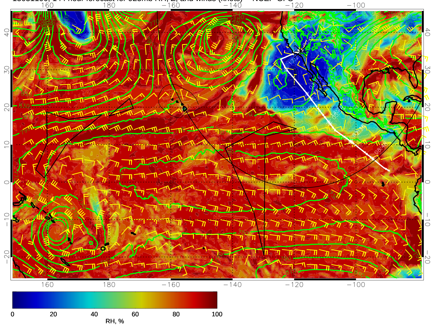
15031100, 144 hour forecast for 925mb RH, Z, and winds (knots) -- NCEP GFS
