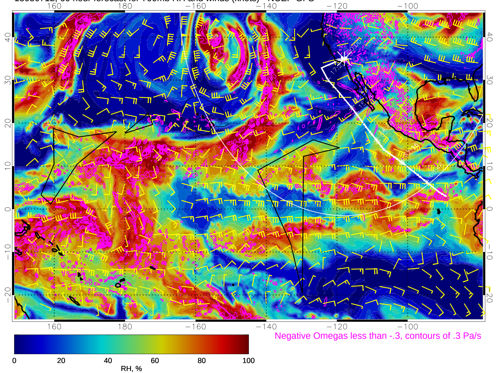
15030712, 60 hour forecast for 700mb RH and winds (knots) - NCEP GFS
