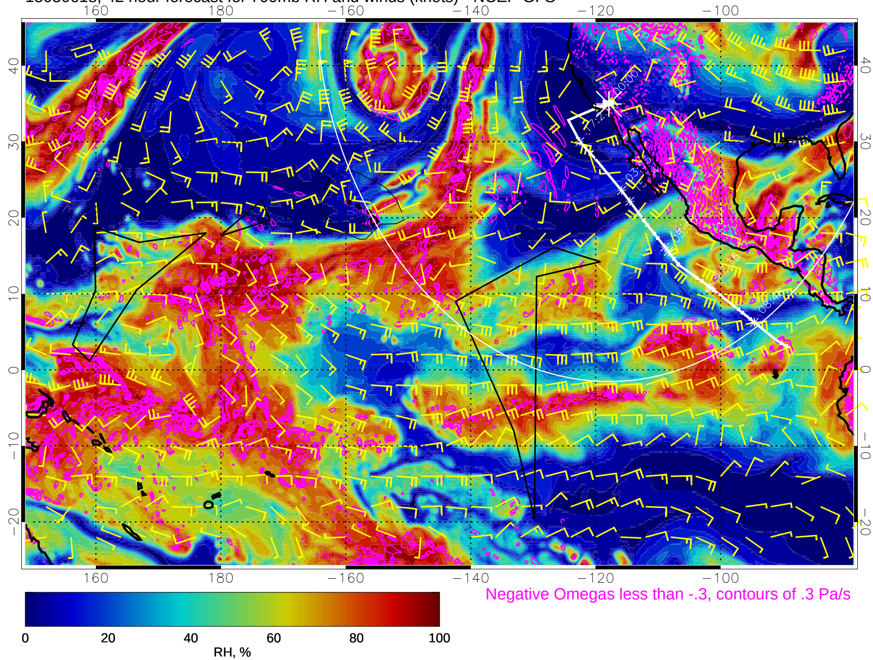
15030618, 42 hour forecast for 700mb RH and winds (knots) - NCEP GFS
