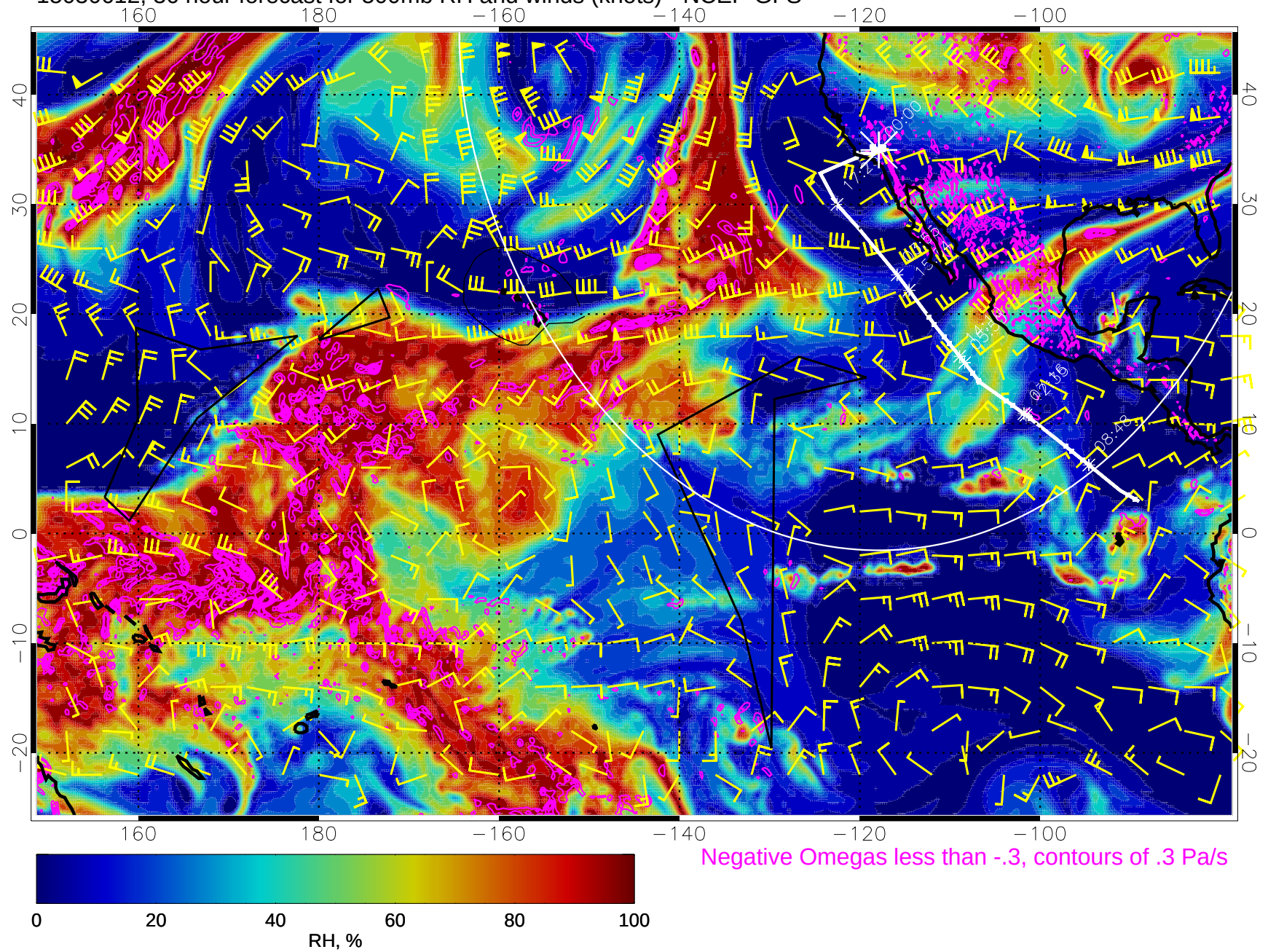
15030612, 36 hour forecast for 500mb RH and winds (knots) - NCEP GFS
