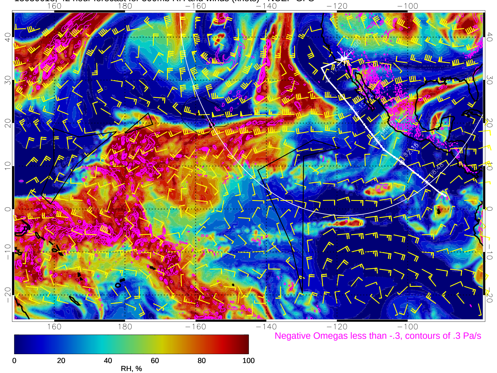
15030618, 42 hour forecast for 500mb RH and winds (knots) - NCEP GFS
