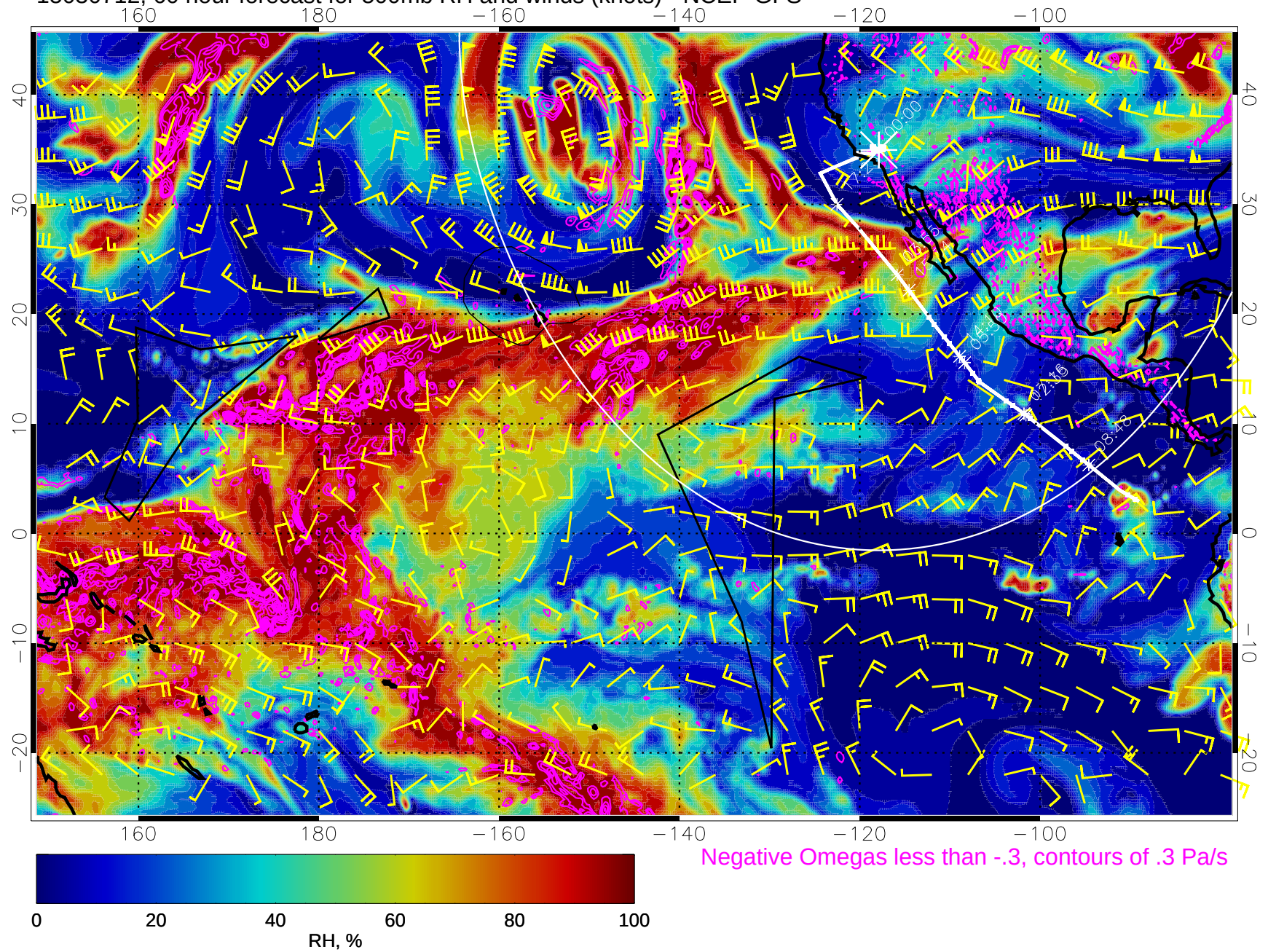
15030712, 60 hour forecast for 500mb RH and winds (knots) - NCEP GFS
