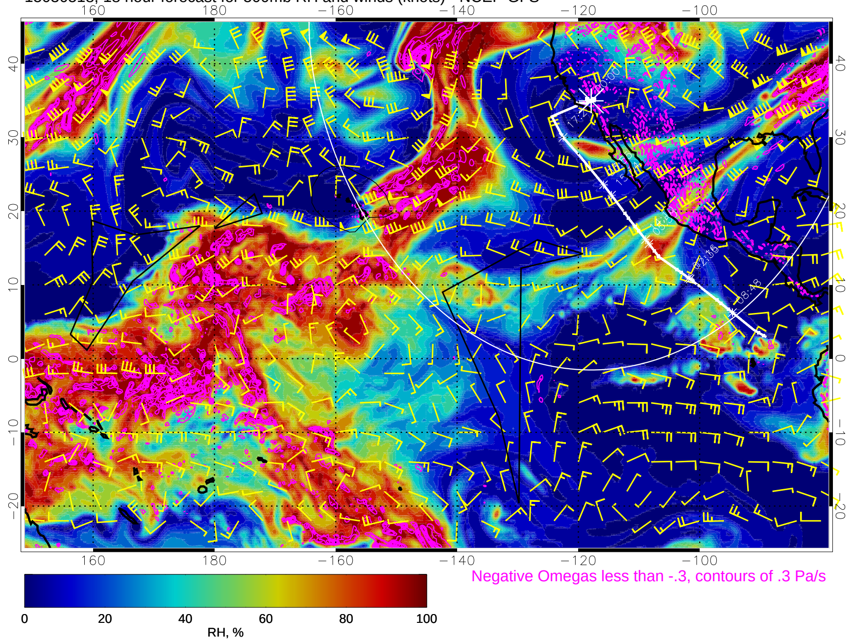
15030518, 18 hour forecast for 500mb RH and winds (knots) - NCEP GFS
