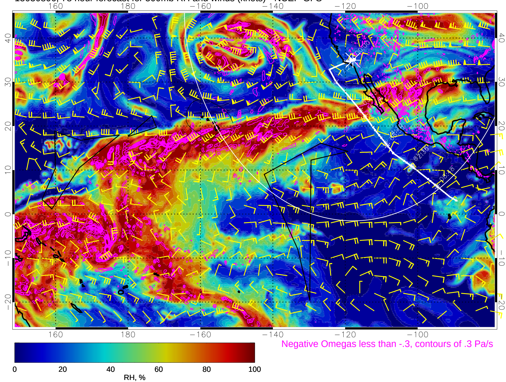
15030806, 78 hour forecast for 500mb RH and winds (knots) - NCEP GFS
