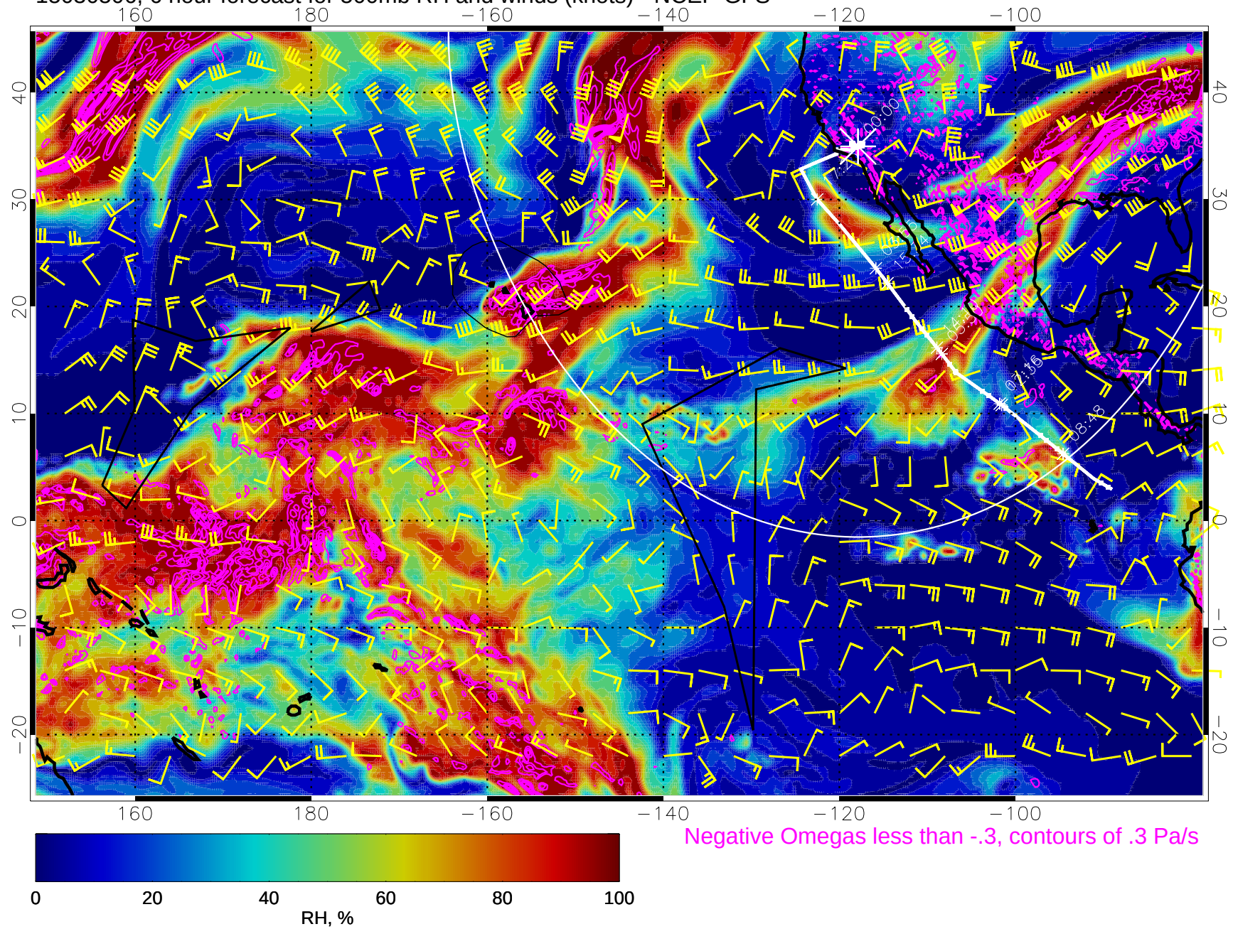
15030506, 6 hour forecast for 500mb RH and winds (knots) - NCEP GFS
