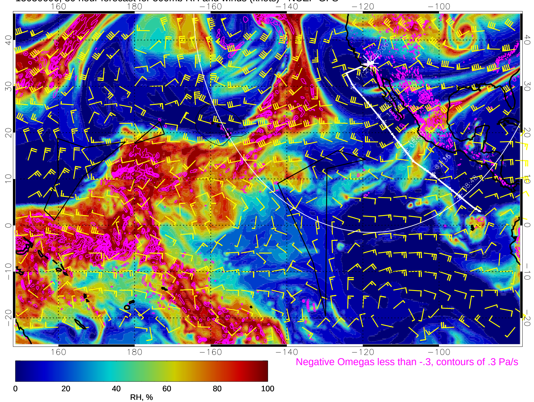
15030606, 30 hour forecast for 500mb RH and winds (knots) - NCEP GFS
