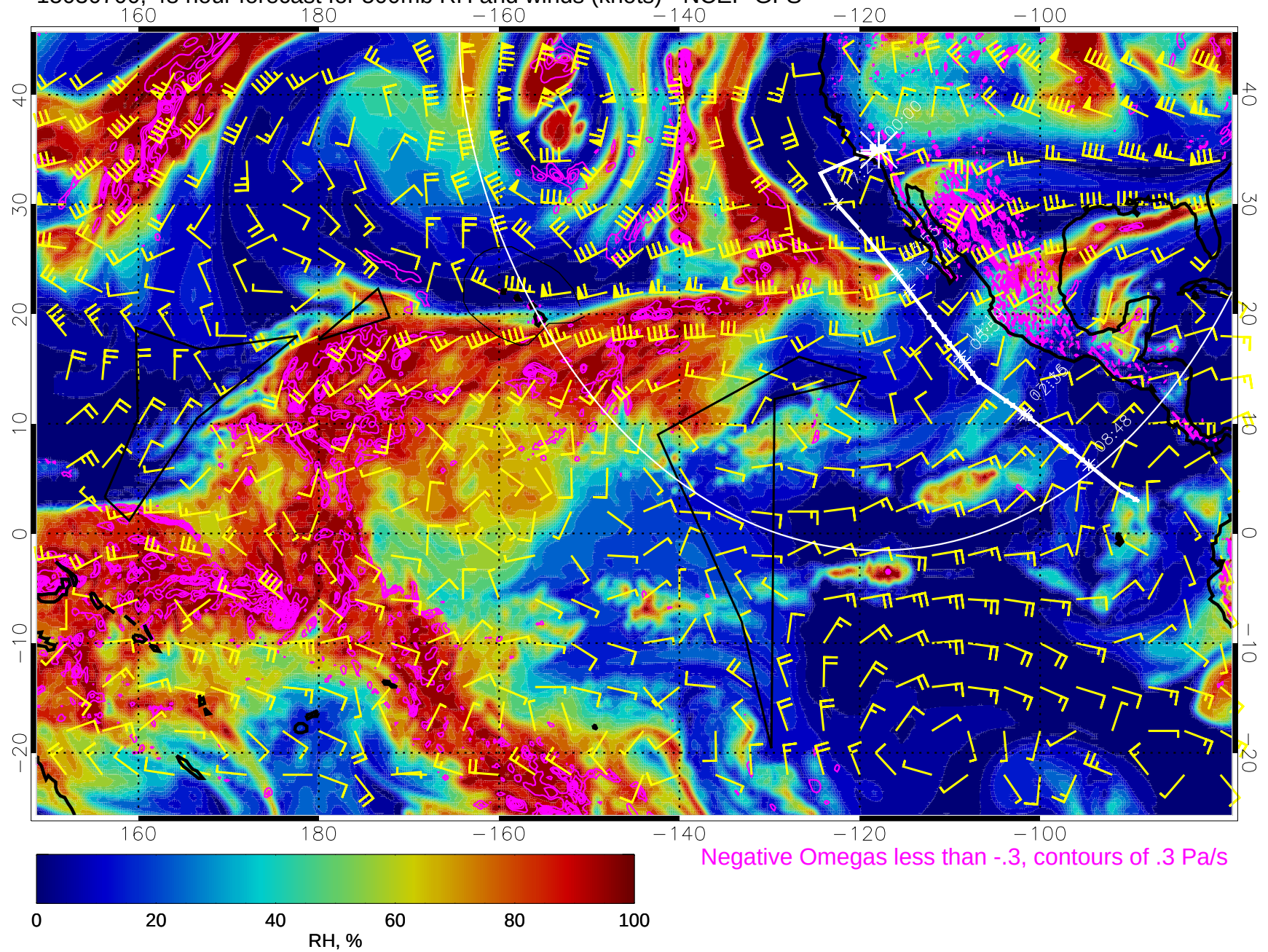
15030700, 48 hour forecast for 500mb RH and winds (knots) - NCEP GFS
