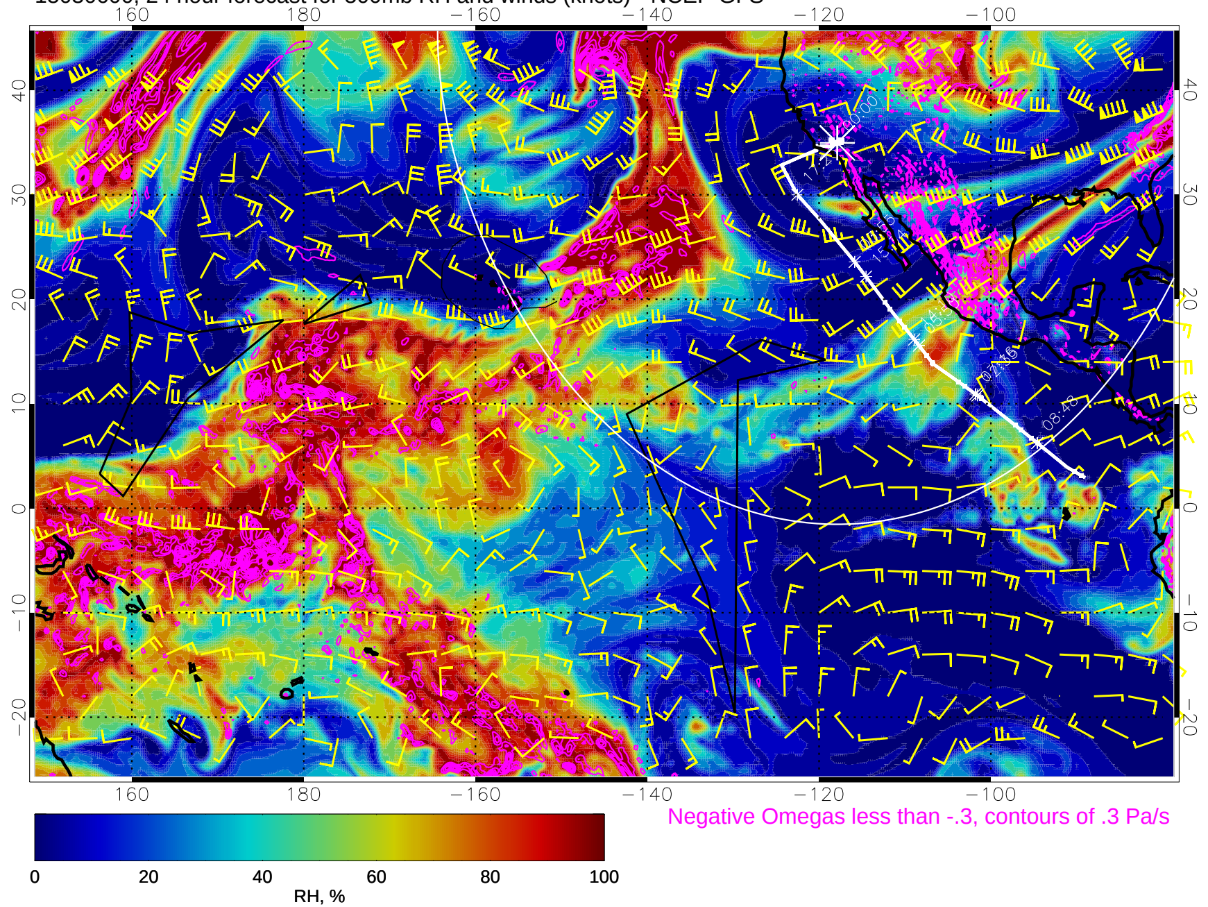
15030600, 24 hour forecast for 500mb RH and winds (knots) - NCEP GFS
