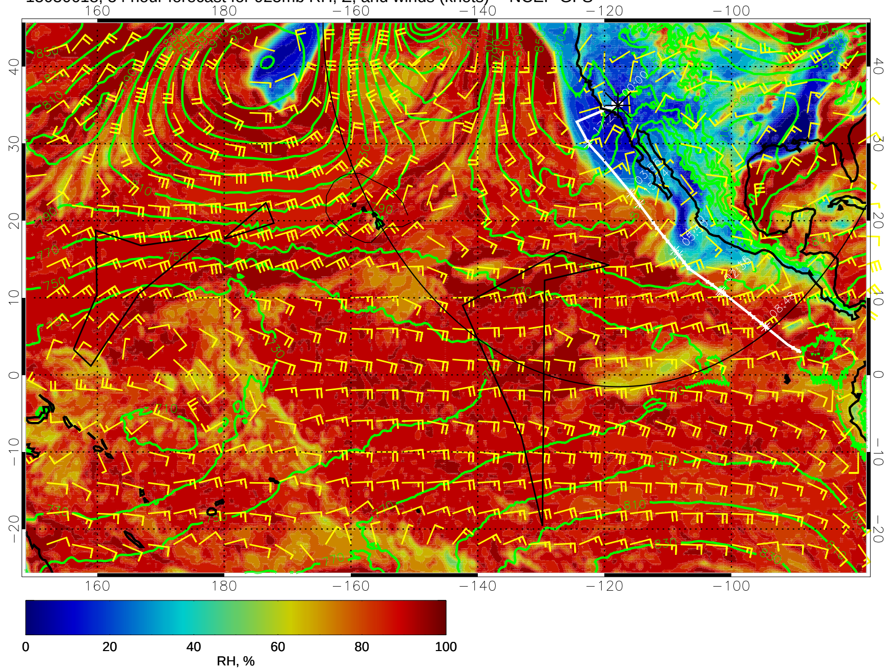
15030618, 54 hour forecast for 925mb RH, Z, and winds (knots) -- NCEP GFS
