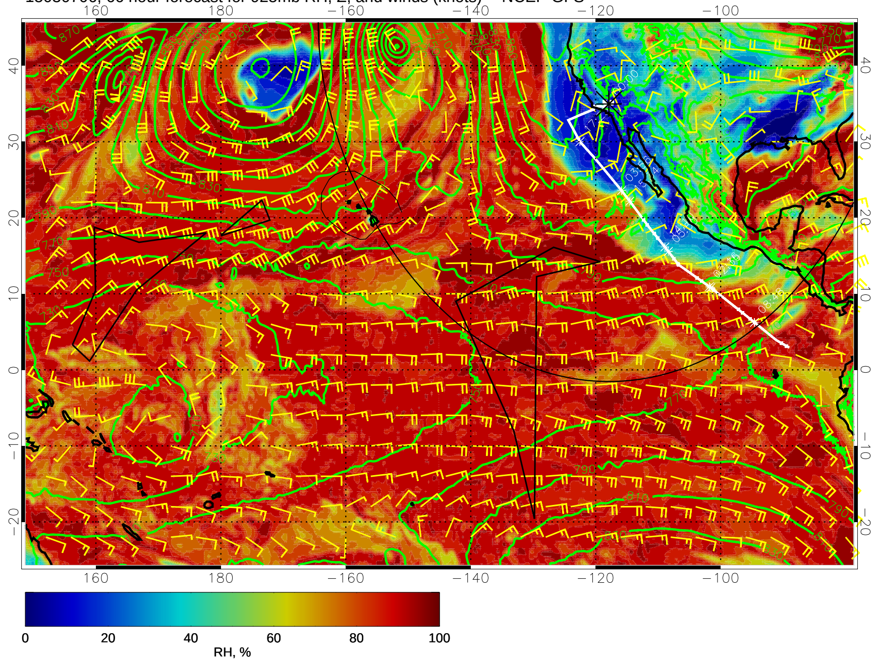
15030706, 66 hour forecast for 925mb RH, Z, and winds (knots) -- NCEP GFS
