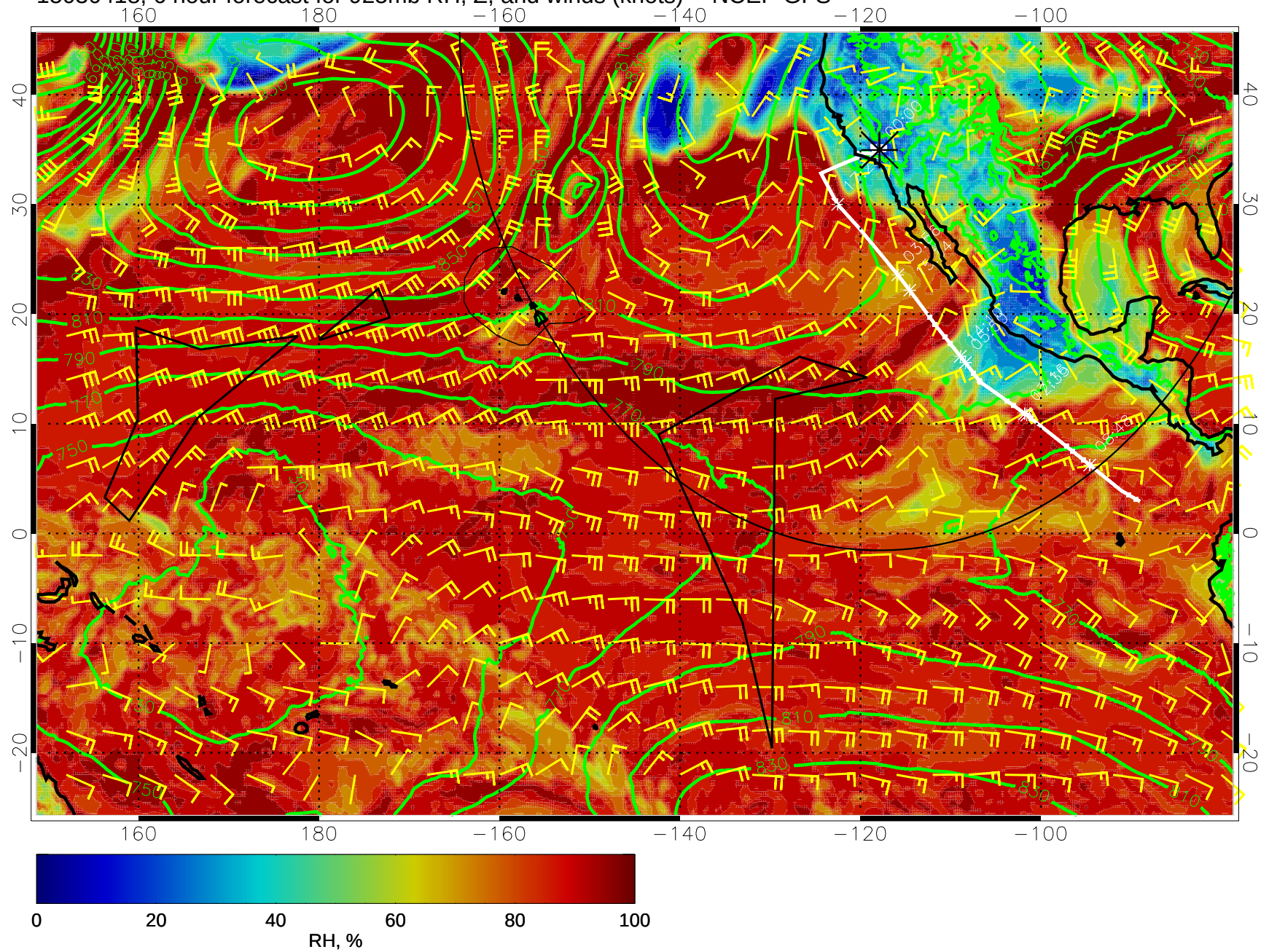
15030418, 6 hour forecast for 925mb RH, Z, and winds (knots) -- NCEP GFS
