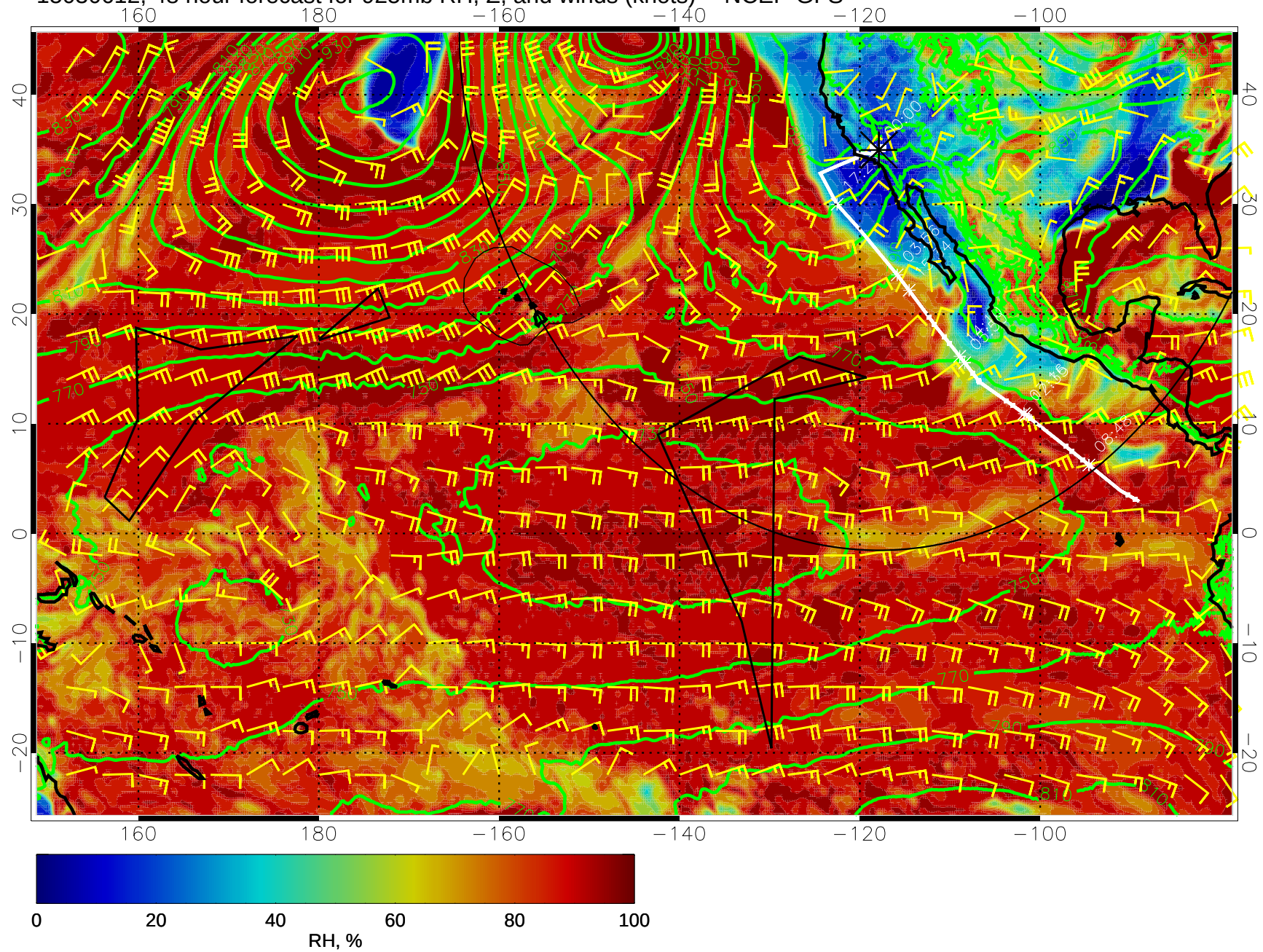
15030612, 48 hour forecast for 925mb RH, Z, and winds (knots) -- NCEP GFS
