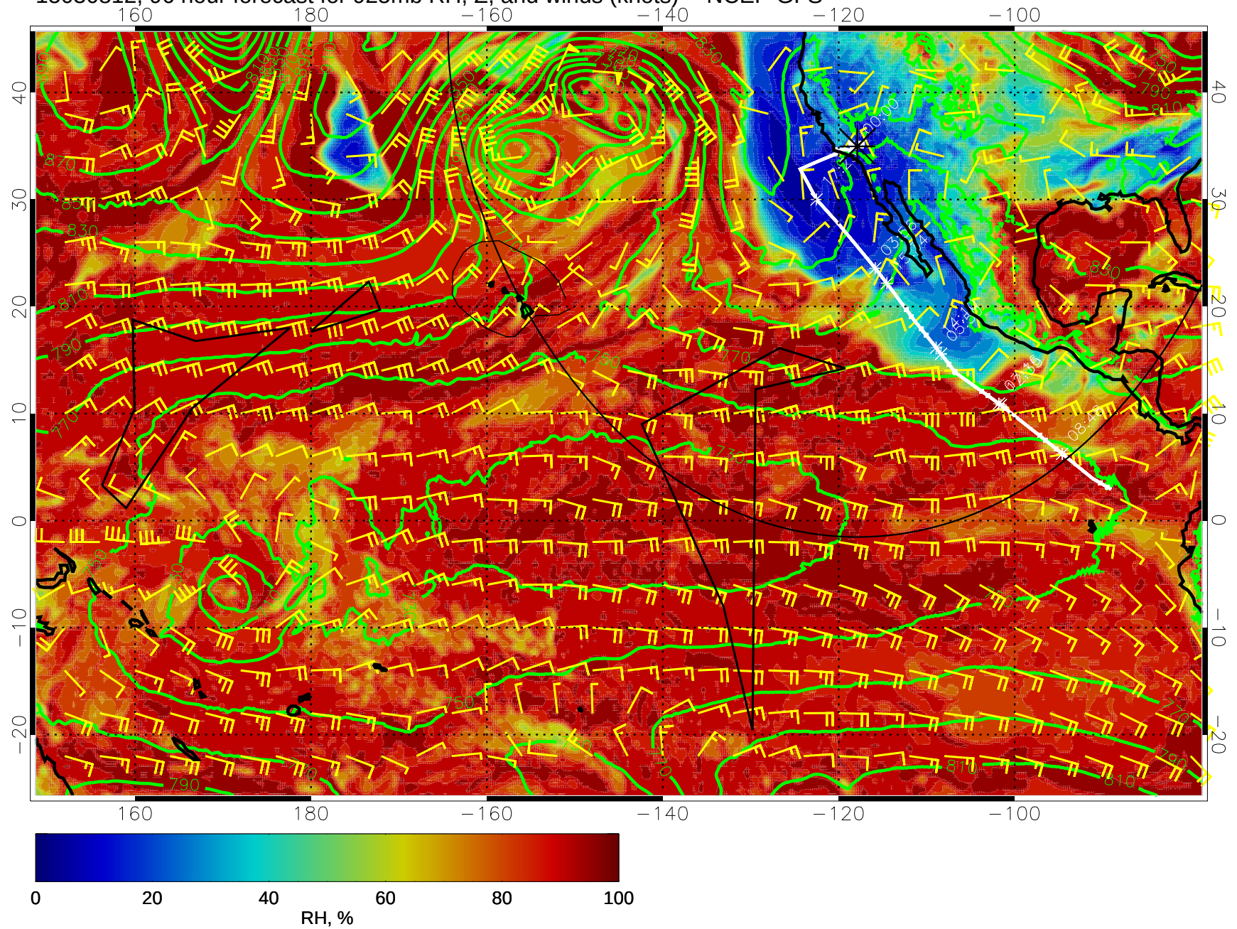
15030812, 96 hour forecast for 925mb RH, Z, and winds (knots) -- NCEP GFS
