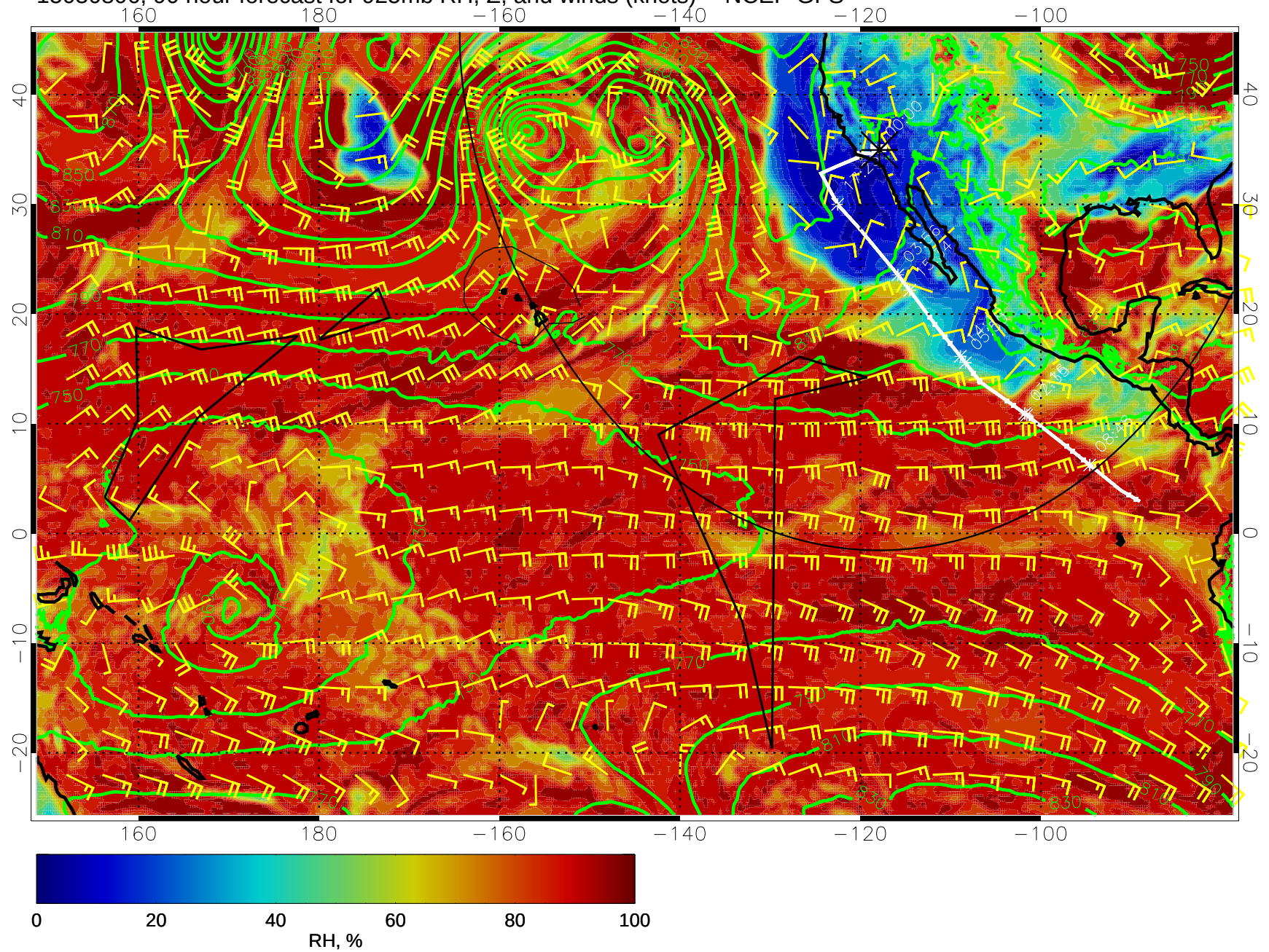
15030806, 90 hour forecast for 925mb RH, Z, and winds (knots) -- NCEP GFS
