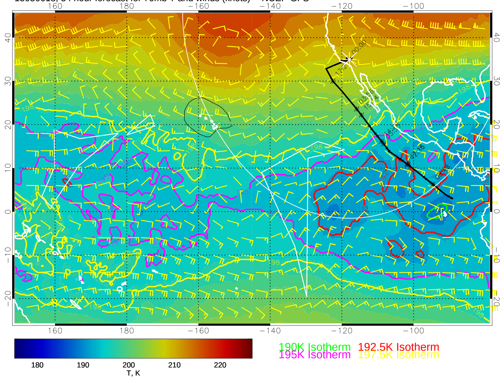
15030618, 54 hour forecast for 70mb T and winds (knots) -- NCEP GFS
