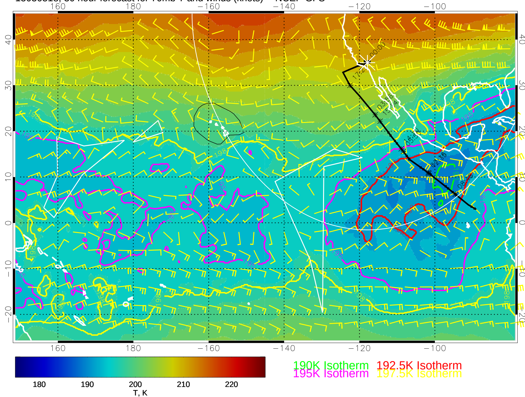
15030518, 30 hour forecast for 70mb T and winds (knots) -- NCEP GFS
