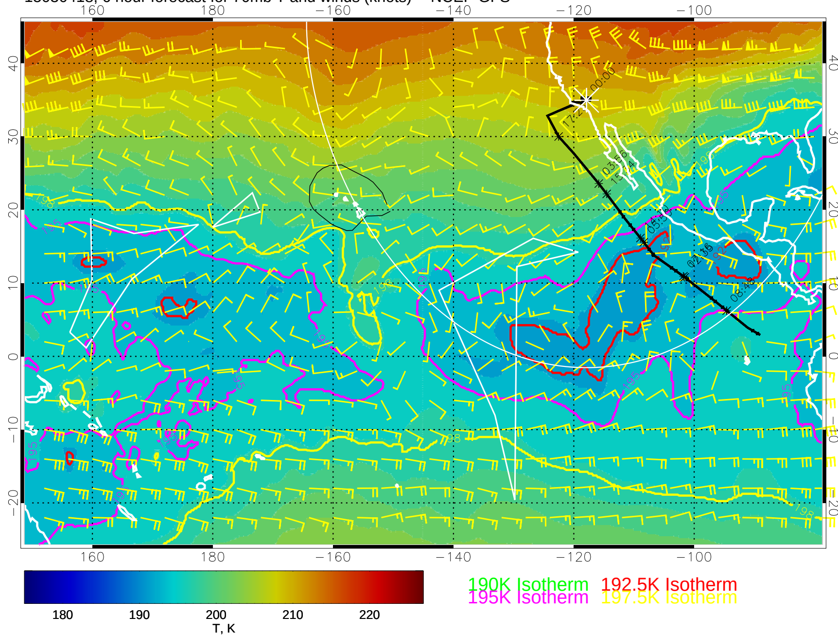
15030418, 6 hour forecast for 70mb T and winds (knots) -- NCEP GFS
