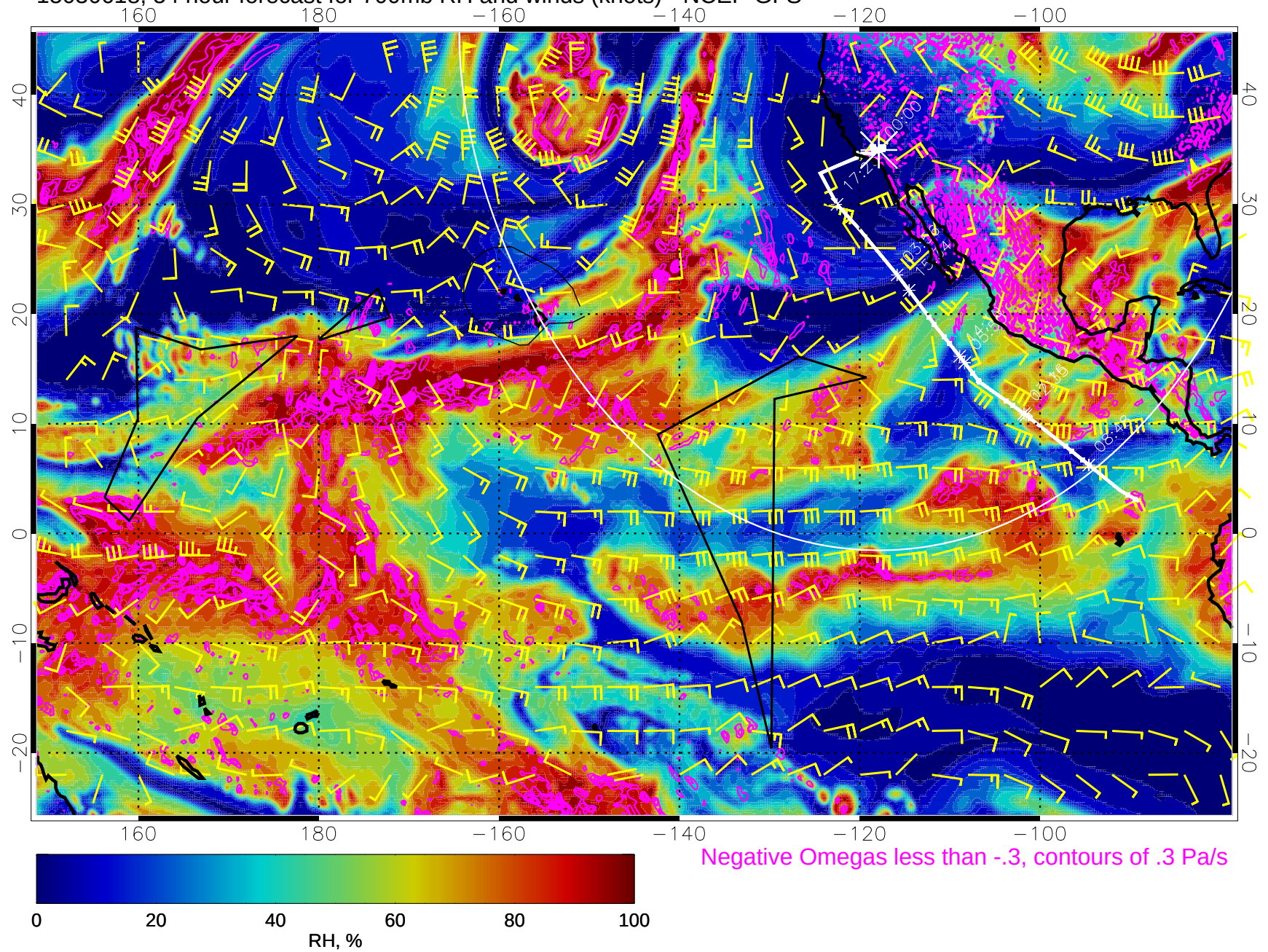
15030618, 54 hour forecast for 700mb RH and winds (knots) - NCEP GFS
