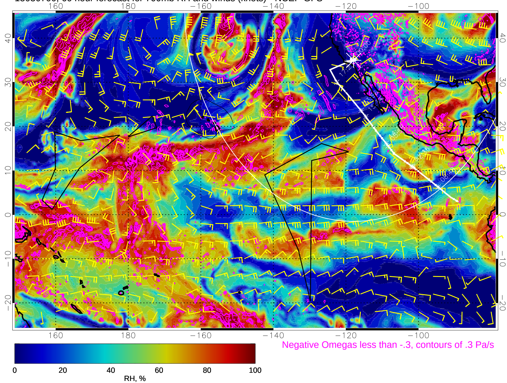
15030700, 60 hour forecast for 700mb RH and winds (knots) - NCEP GFS
