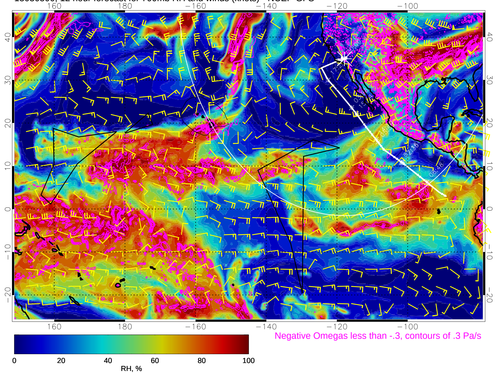
15030500, 12 hour forecast for 700mb RH and winds (knots) - NCEP GFS
