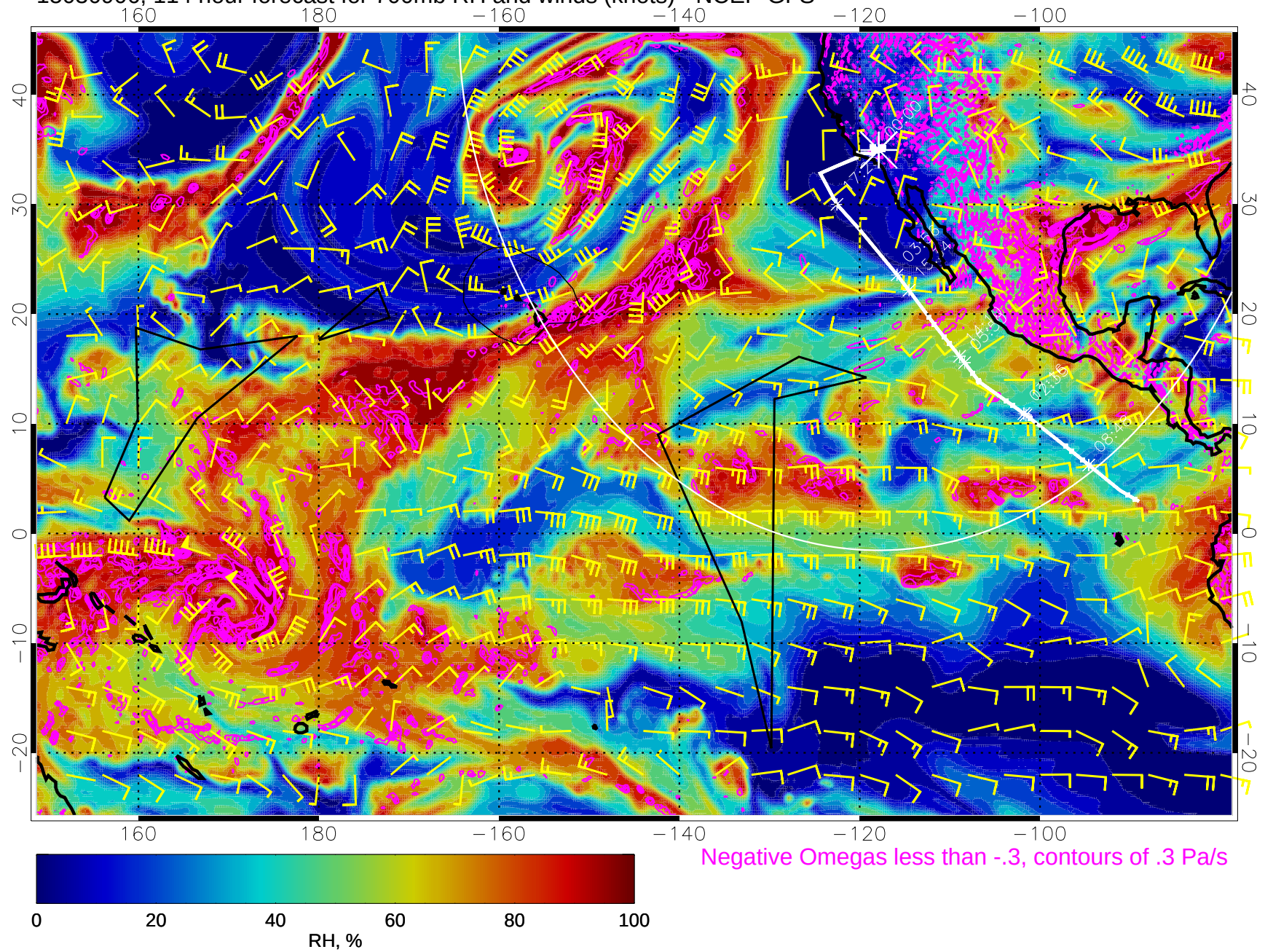
15030906, 114 hour forecast for 700mb RH and winds (knots) - NCEP GFS
