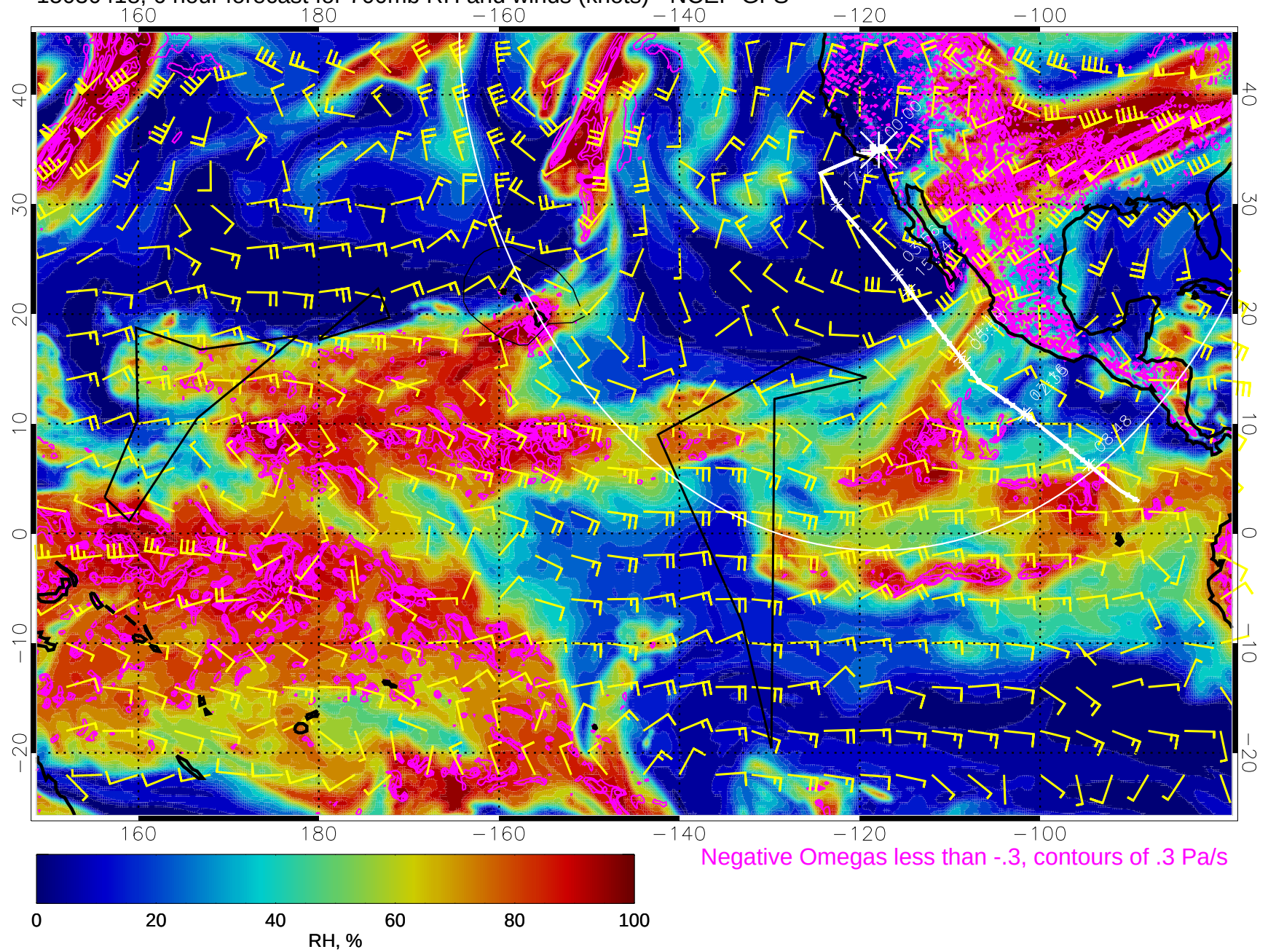
15030418, 6 hour forecast for 700mb RH and winds (knots) - NCEP GFS
