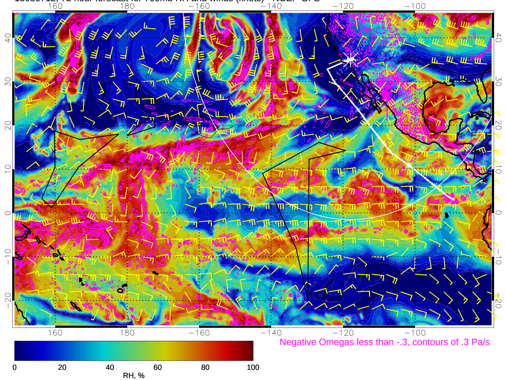
15030712, 72 hour forecast for 700mb RH and winds (knots) - NCEP GFS
