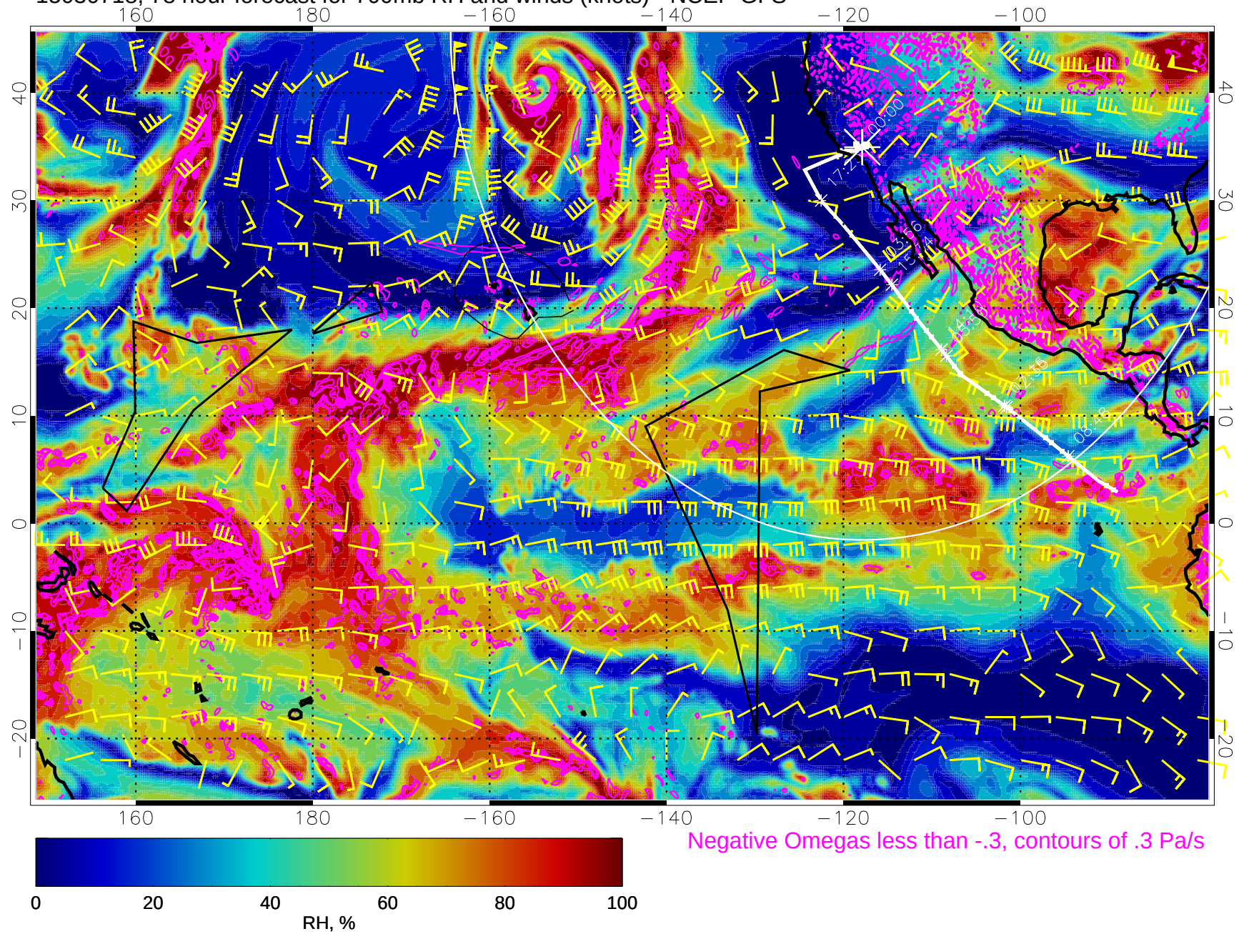
15030718, 78 hour forecast for 700mb RH and winds (knots) - NCEP GFS
