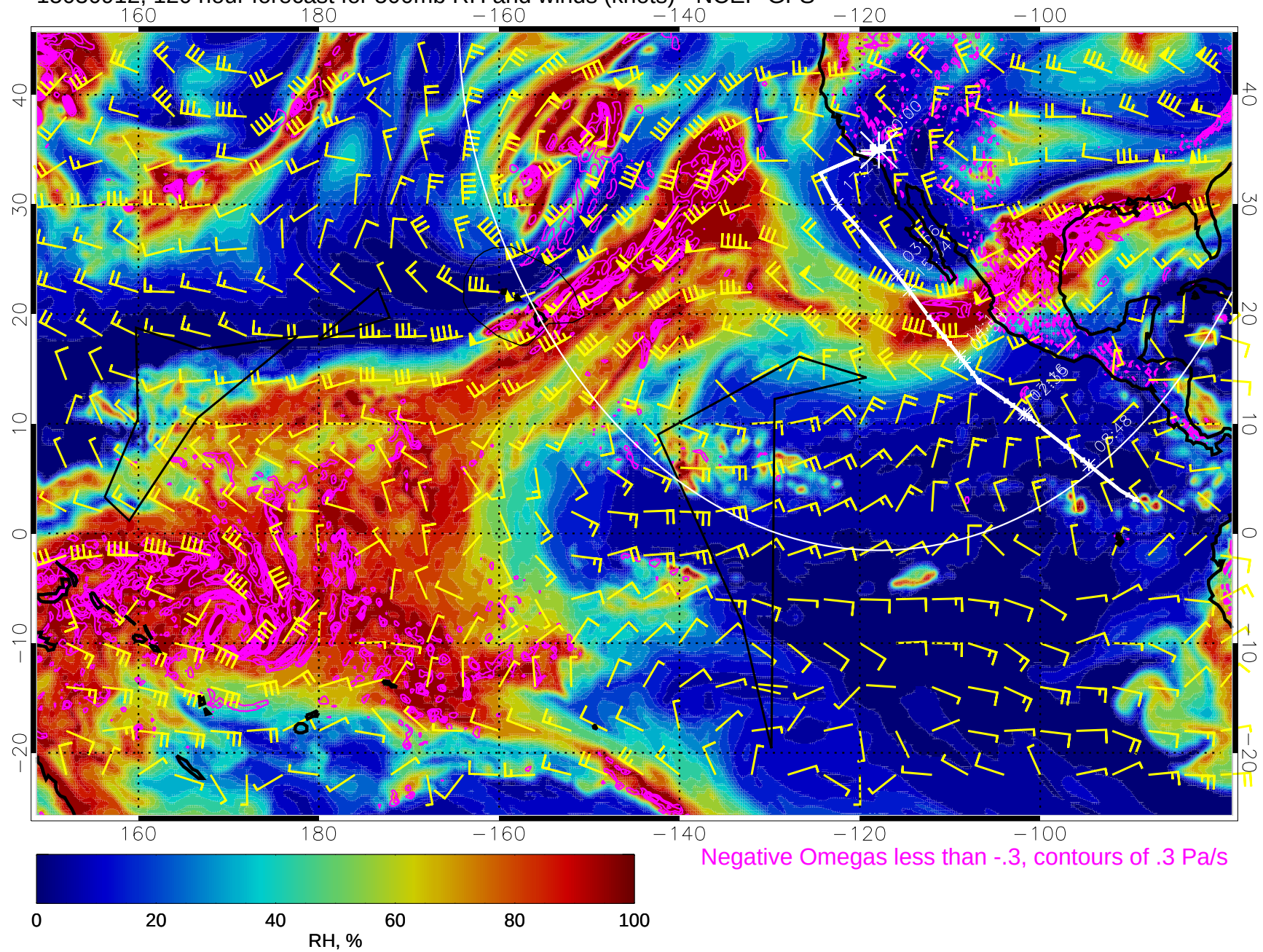
15030912, 120 hour forecast for 500mb RH and winds (knots) - NCEP GFS
