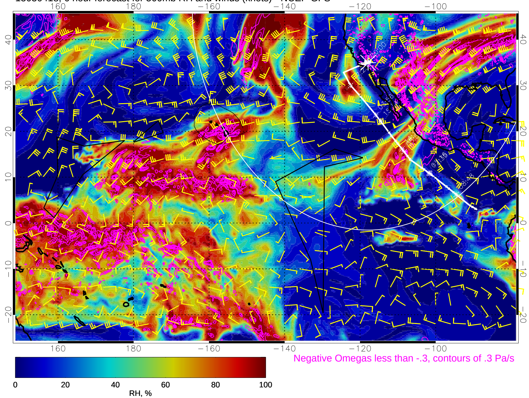
15030418, 6 hour forecast for 500mb RH and winds (knots) - NCEP GFS
