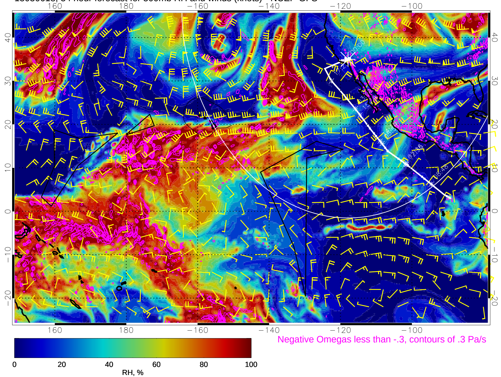
15030618, 54 hour forecast for 500mb RH and winds (knots) - NCEP GFS
