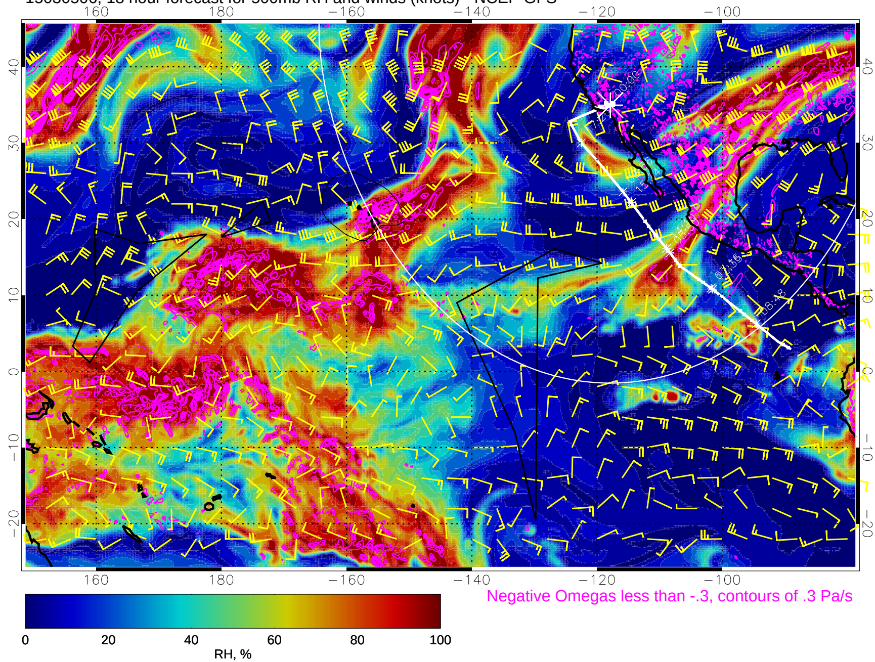
15030506, 18 hour forecast for 500mb RH and winds (knots) - NCEP GFS
