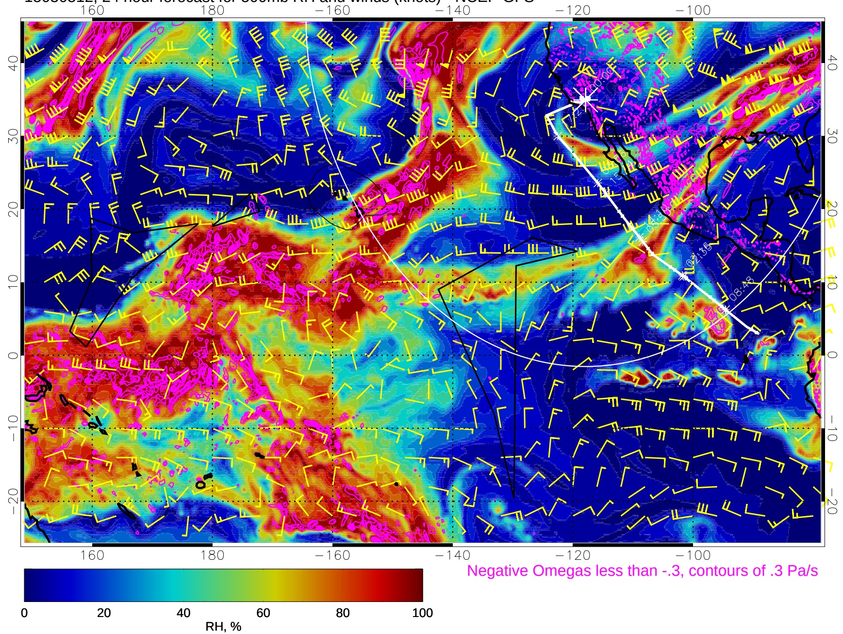
15030512, 24 hour forecast for 500mb RH and winds (knots) - NCEP GFS
