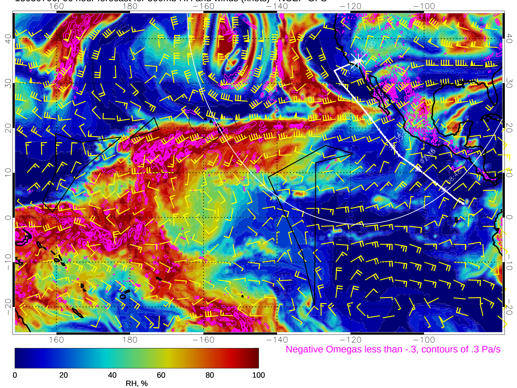
15030706, 66 hour forecast for 500mb RH and winds (knots) - NCEP GFS
