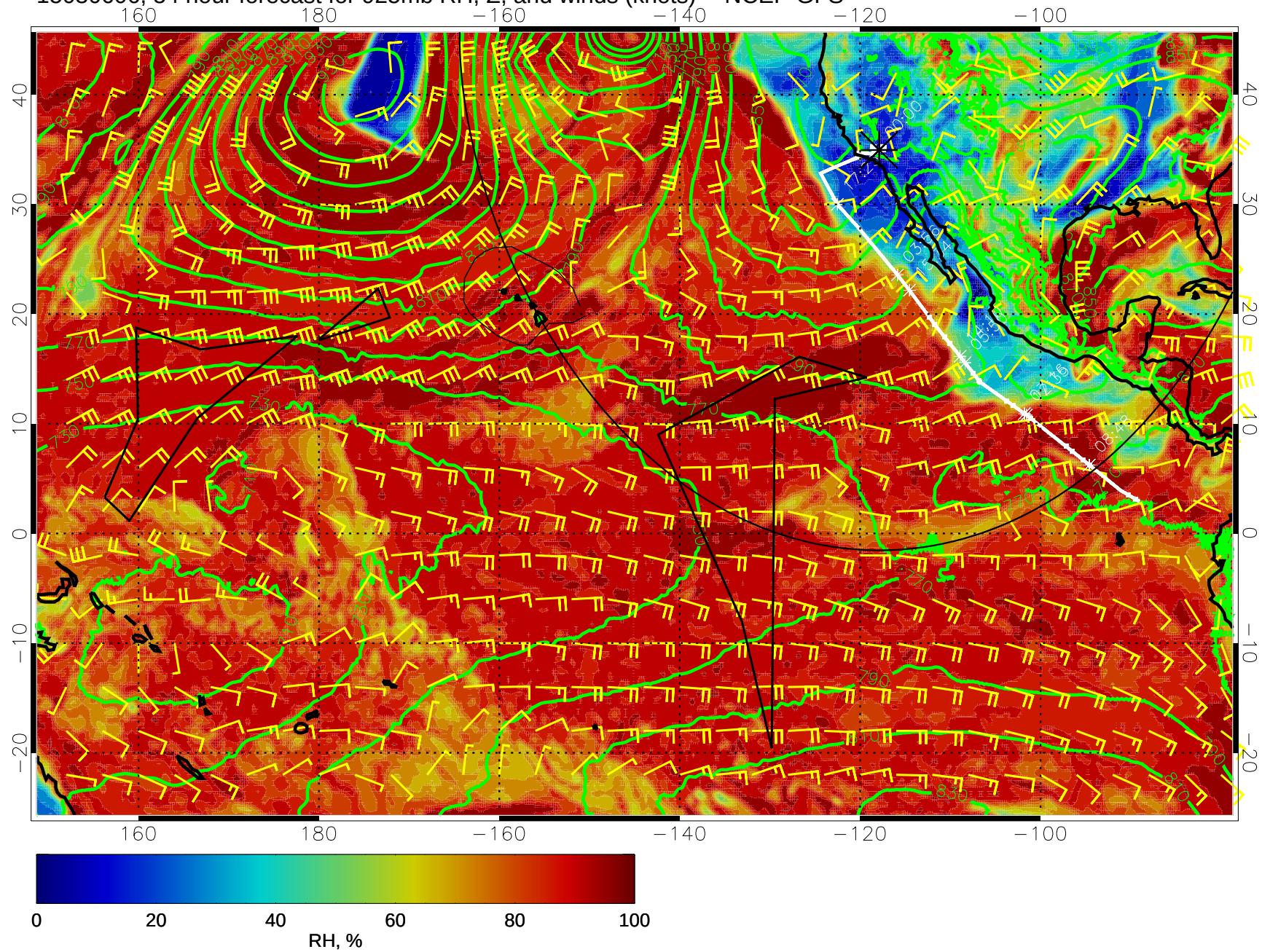
15030606, 54 hour forecast for 925mb RH, Z, and winds (knots) -- NCEP GFS
