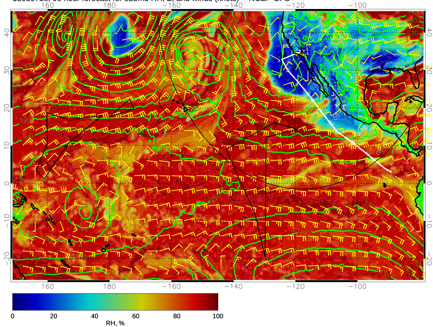
15030718, 90 hour forecast for 925mb RH, Z, and winds (knots) -- NCEP GFS
