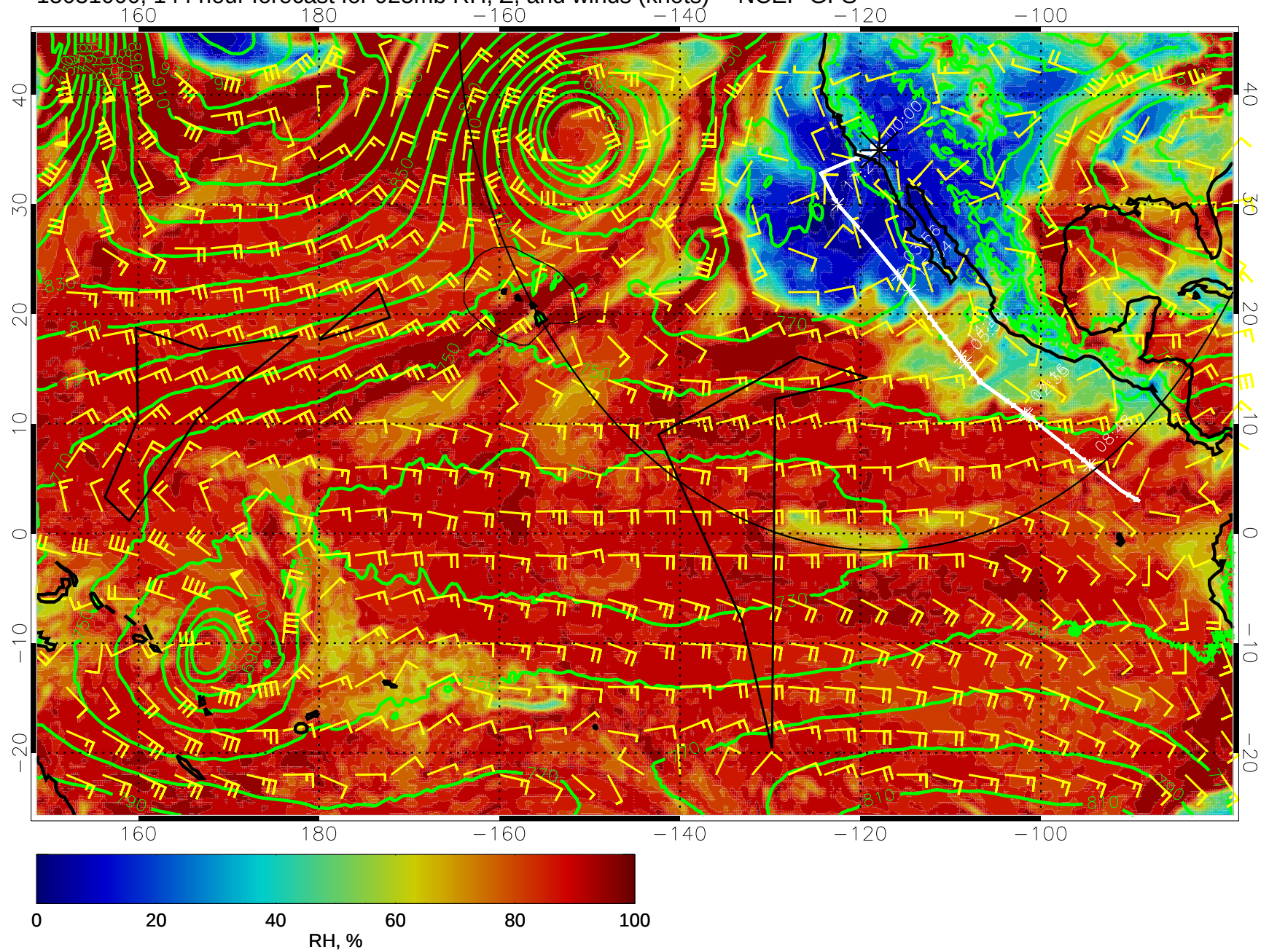
15031000, 144 hour forecast for 925mb RH, Z, and winds (knots) -- NCEP GFS
