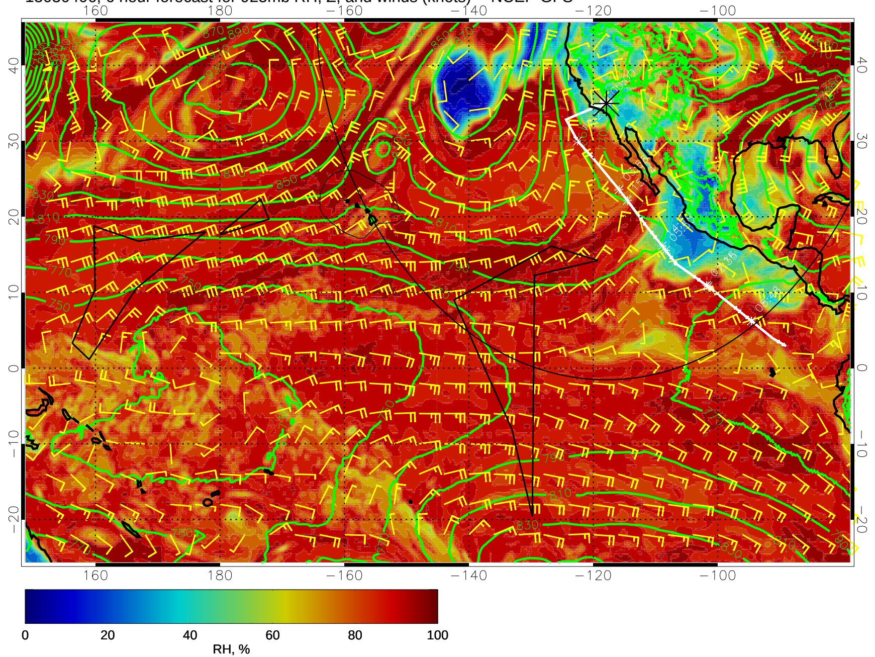
15030406, 6 hour forecast for 925mb RH, Z, and winds (knots) -- NCEP GFS
