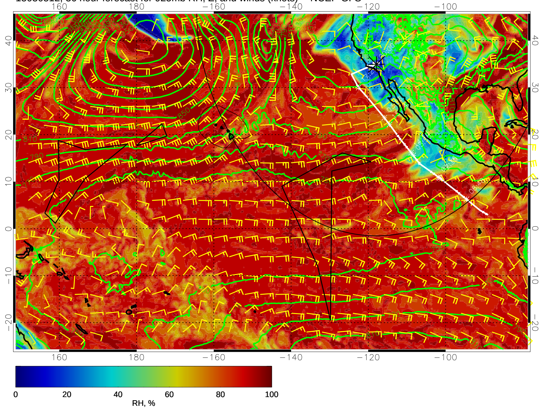
15030512, 36 hour forecast for 925mb RH, Z, and winds (knots) -- NCEP GFS
