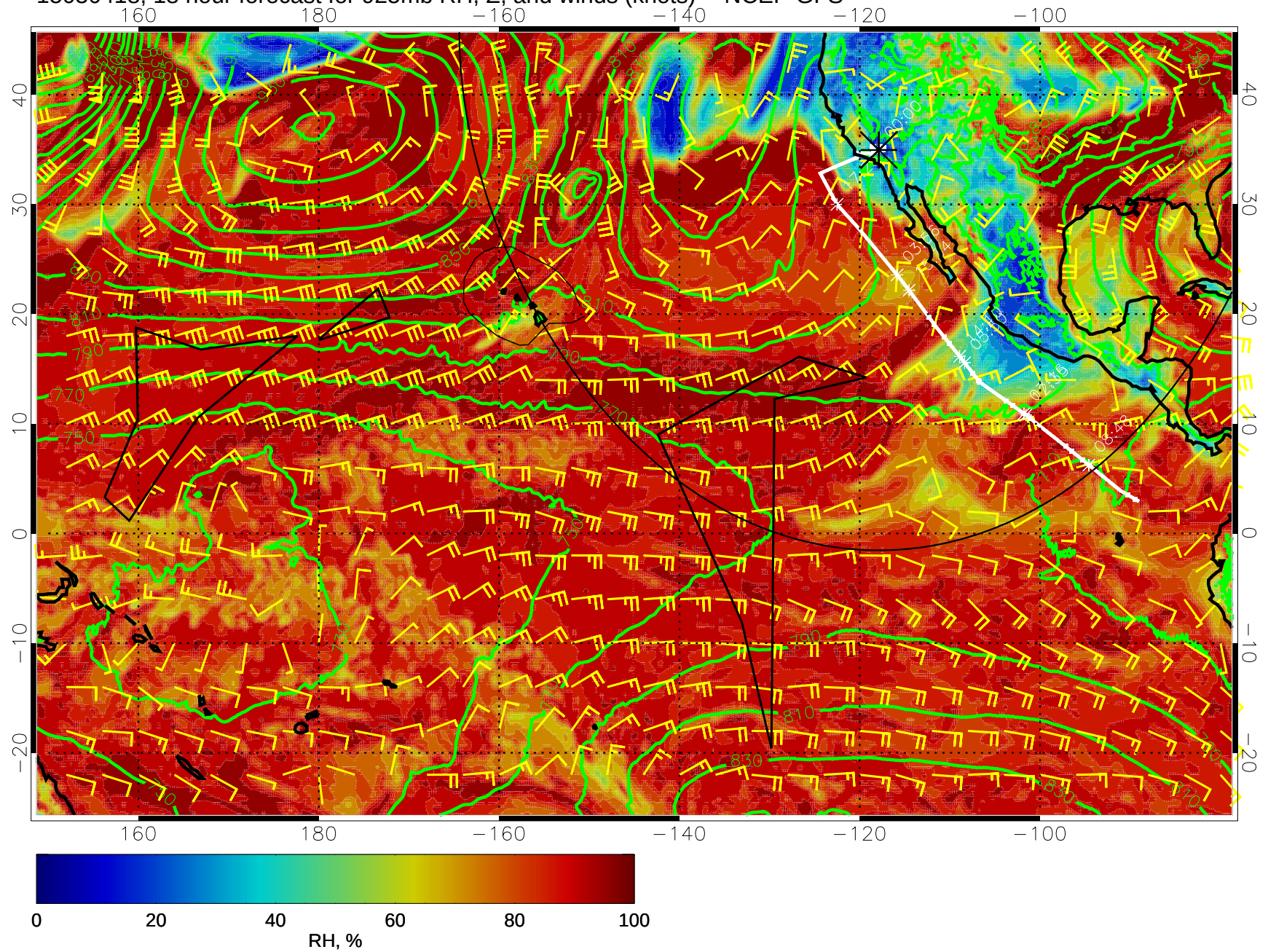
15030418, 18 hour forecast for 925mb RH, Z, and winds (knots) -- NCEP GFS
