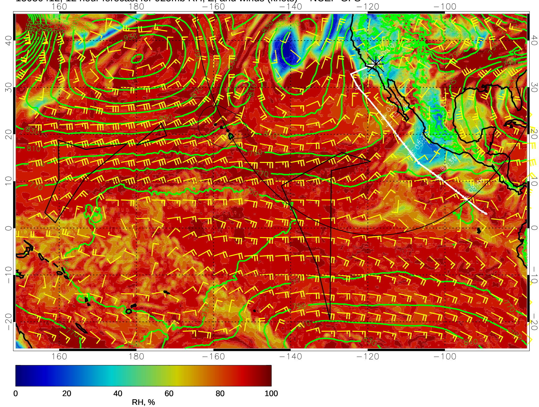
15030412, 12 hour forecast for 925mb RH, Z, and winds (knots) -- NCEP GFS
