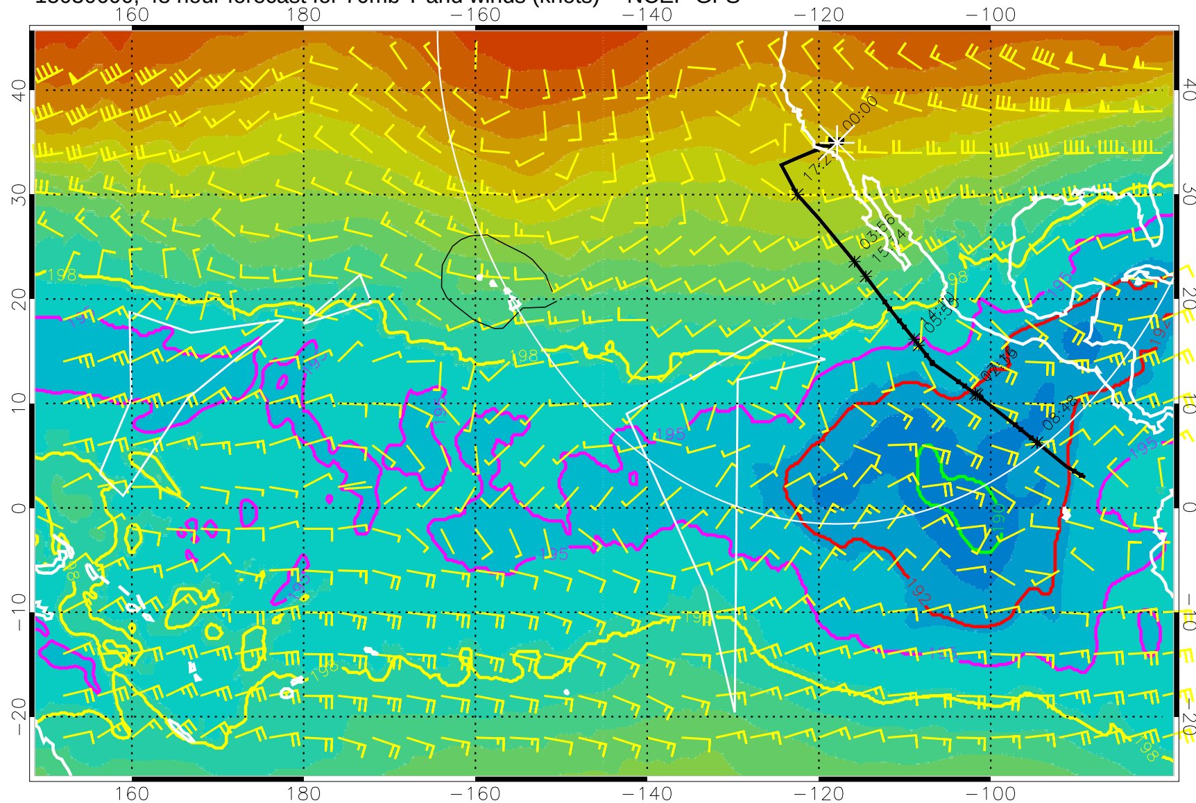
15030600, 48 hour forecast for 70mb T and winds (knots) -- NCEP GFS
