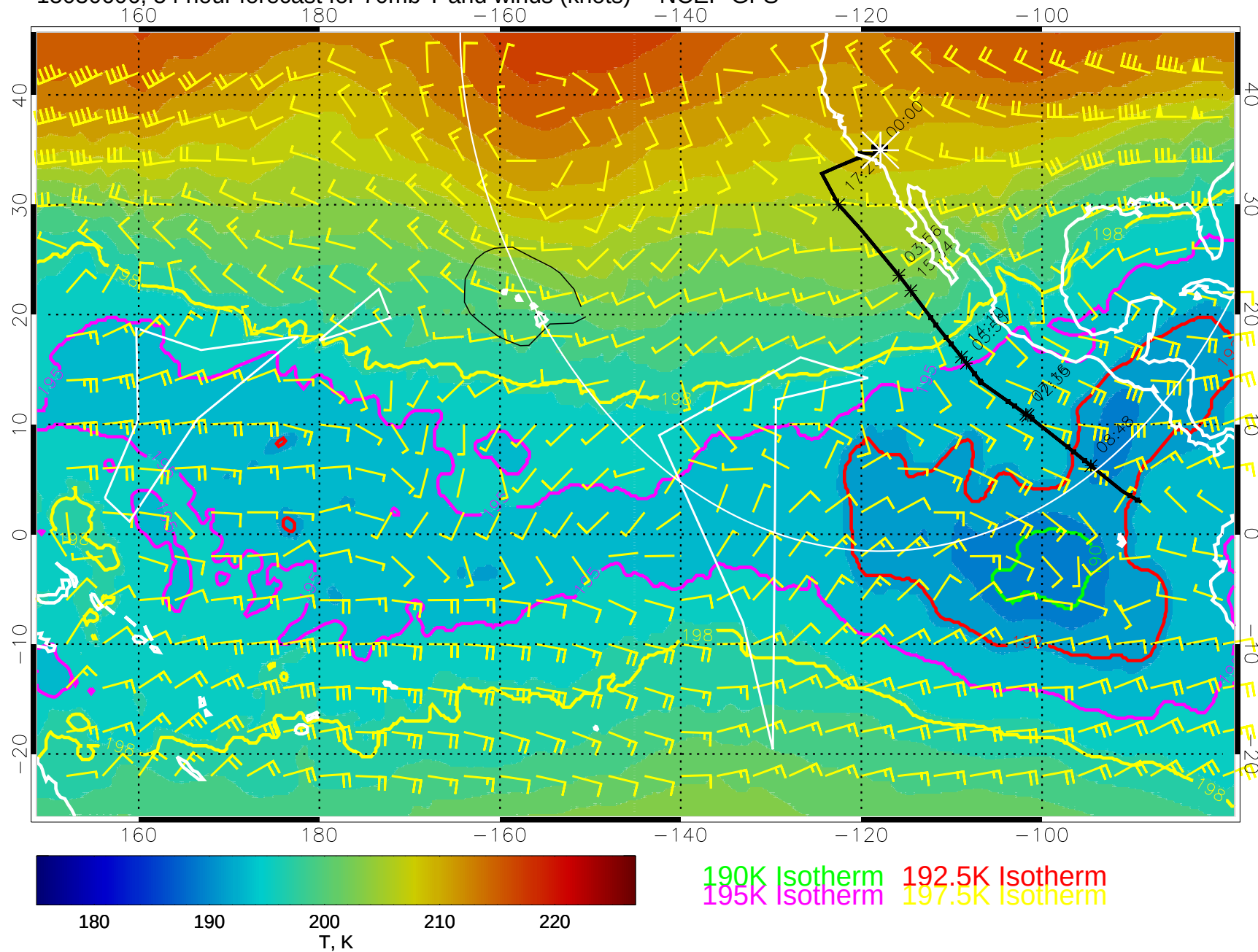
15030606, 54 hour forecast for 70mb T and winds (knots) -- NCEP GFS
