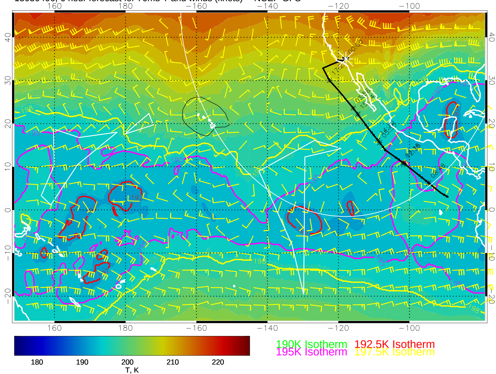
15030406, 6 hour forecast for 70mb T and winds (knots) -- NCEP GFS
