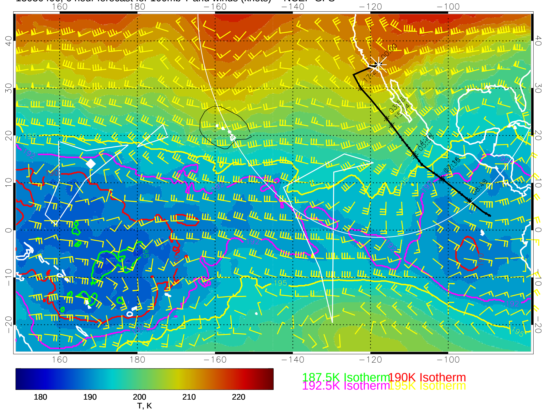
15030406, 6 hour forecast for 100mb T and winds (knots) -- NCEP GFS
