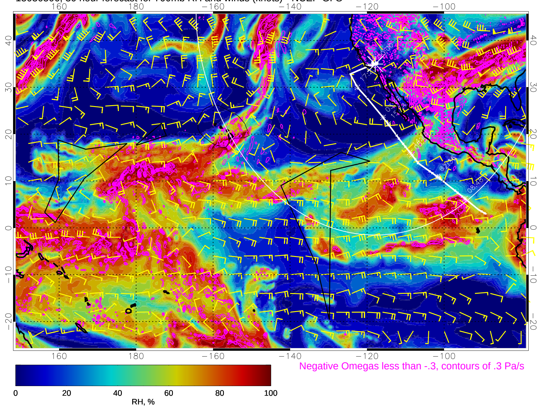
15030506, 30 hour forecast for 700mb RH and winds (knots) - NCEP GFS
