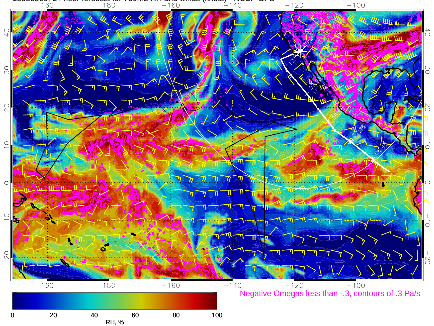
15030500, 24 hour forecast for 700mb RH and winds (knots) - NCEP GFS
