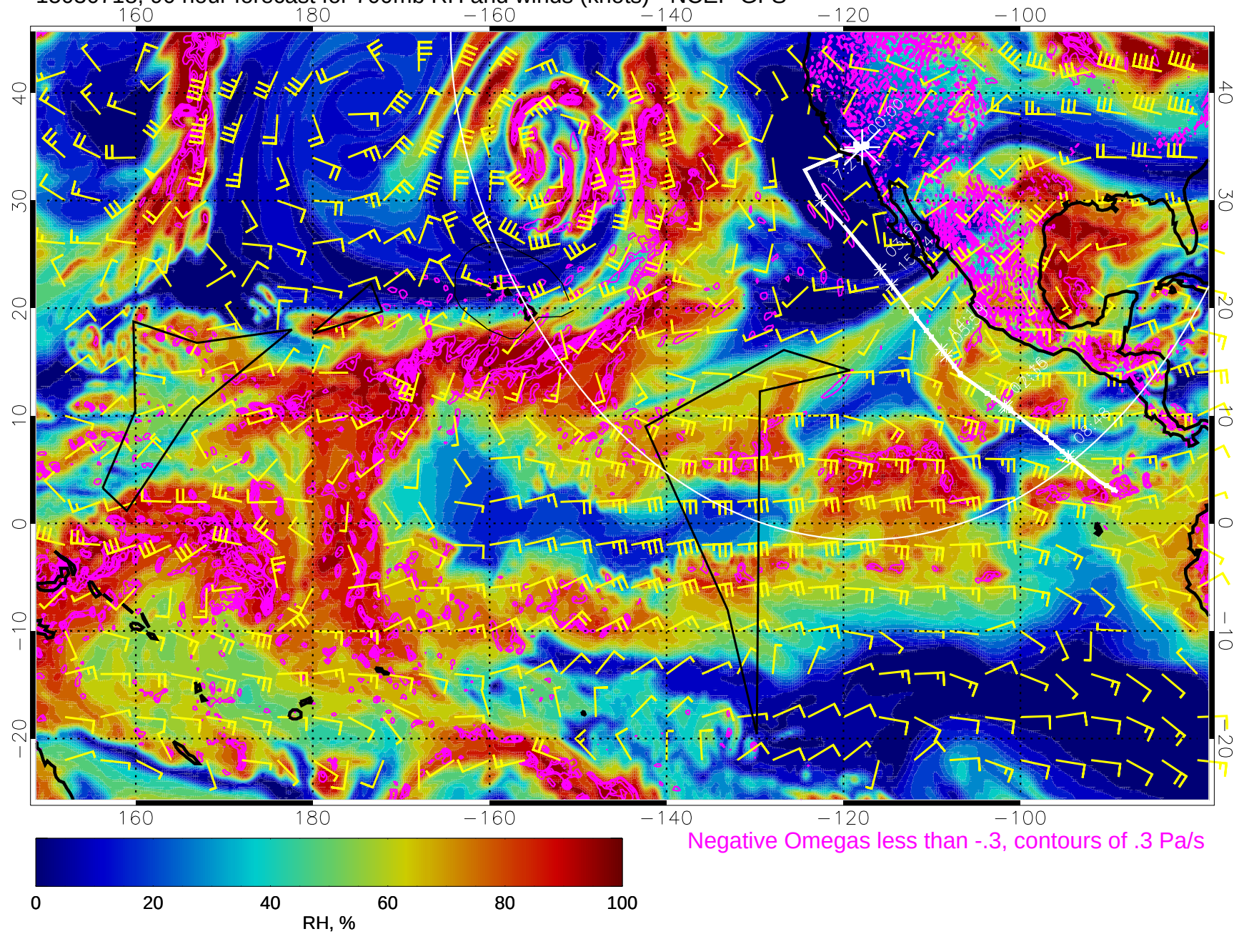
15030718, 90 hour forecast for 700mb RH and winds (knots) - NCEP GFS
