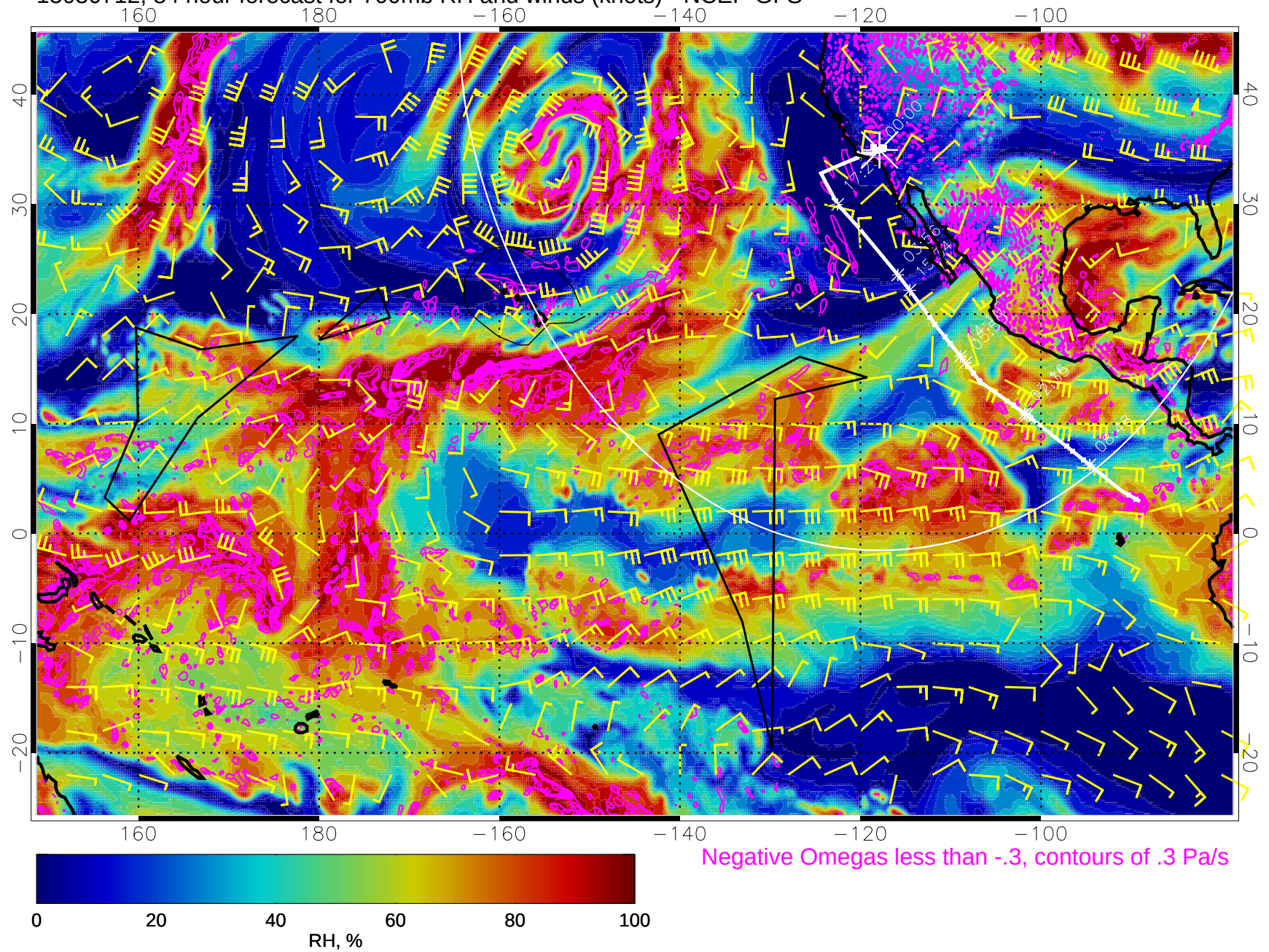
15030712, 84 hour forecast for 700mb RH and winds (knots) - NCEP GFS
