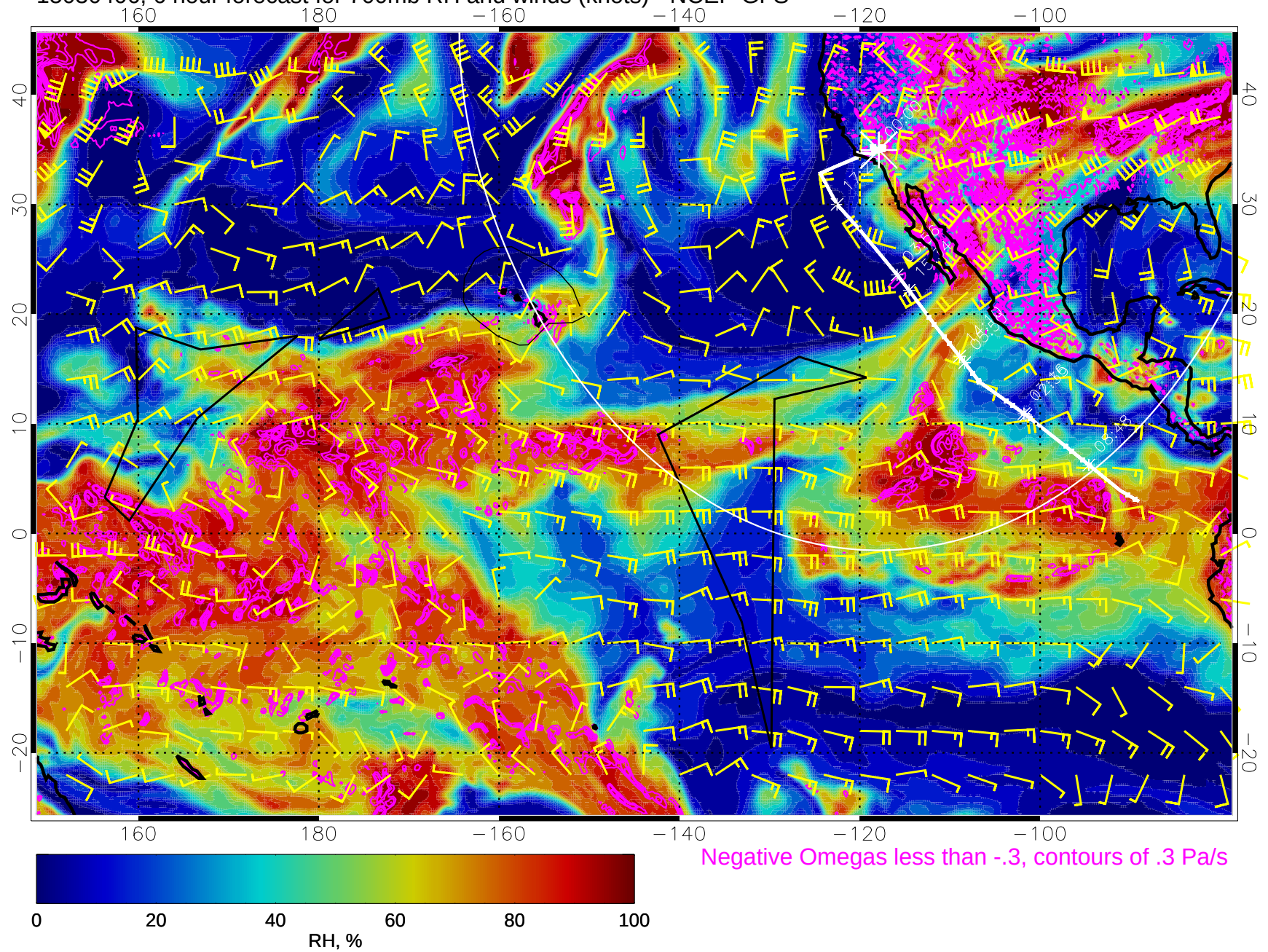
15030406, 6 hour forecast for 700mb RH and winds (knots) - NCEP GFS
