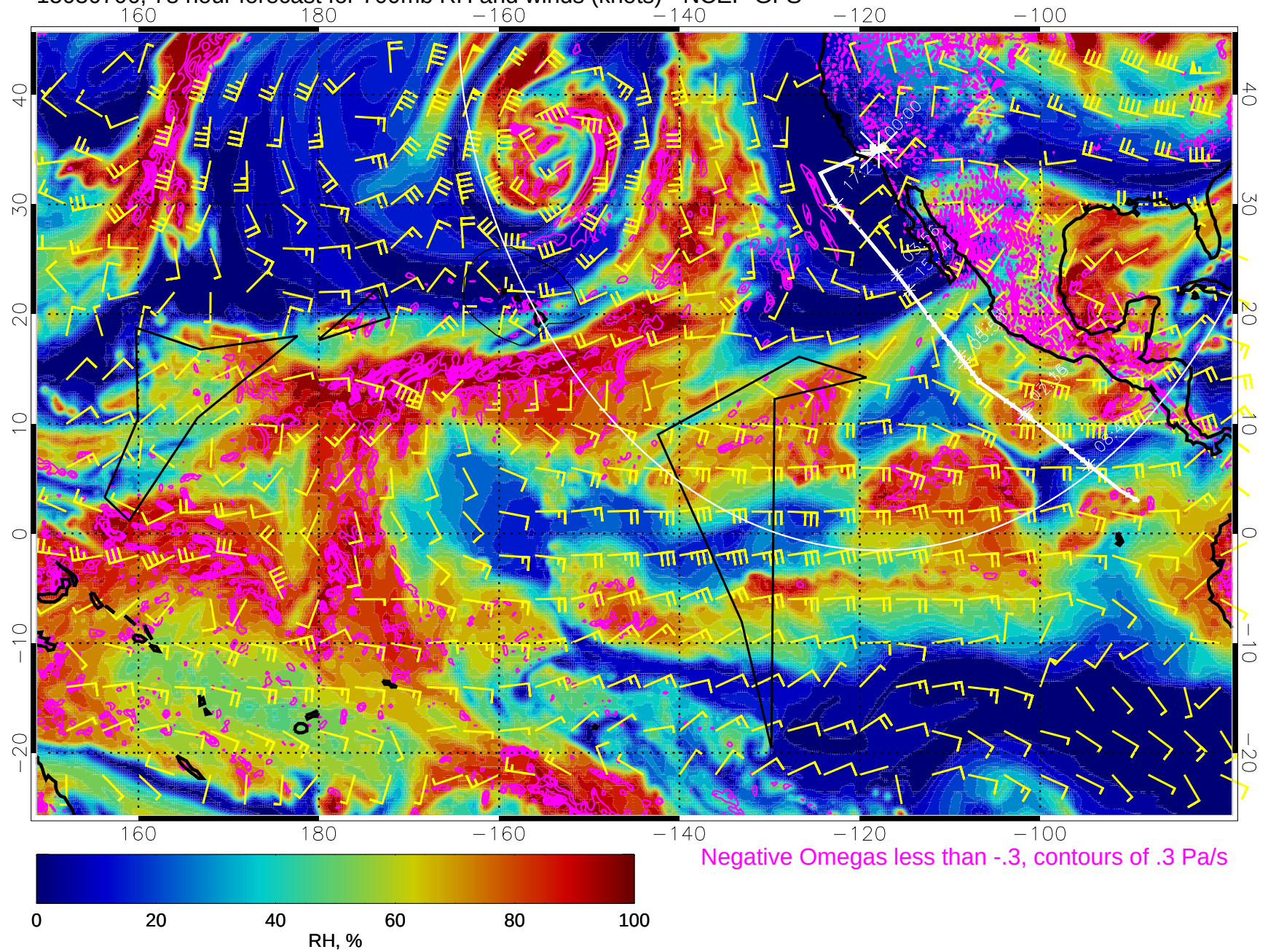
15030706, 78 hour forecast for 700mb RH and winds (knots) - NCEP GFS
