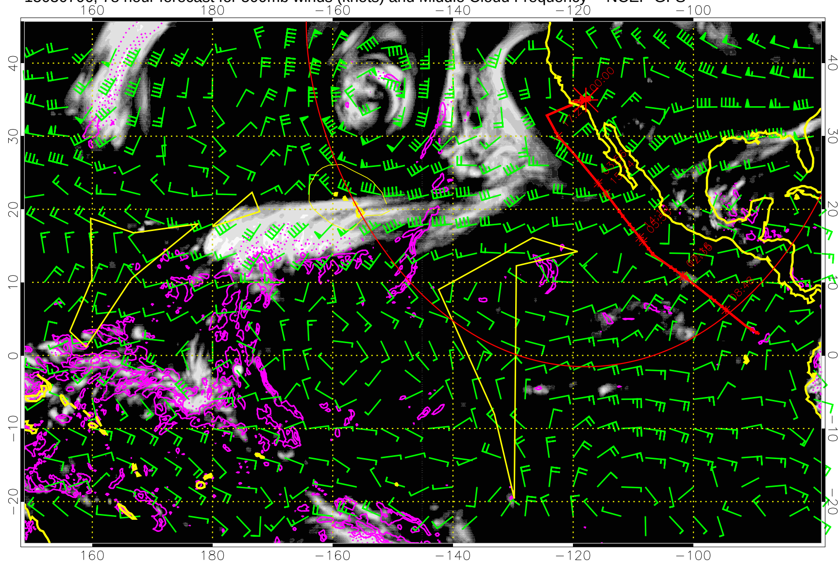
15030706, 78 hour forecast for 500mb winds (knots) and Middle Cloud Frequency -- NCEP GFS
