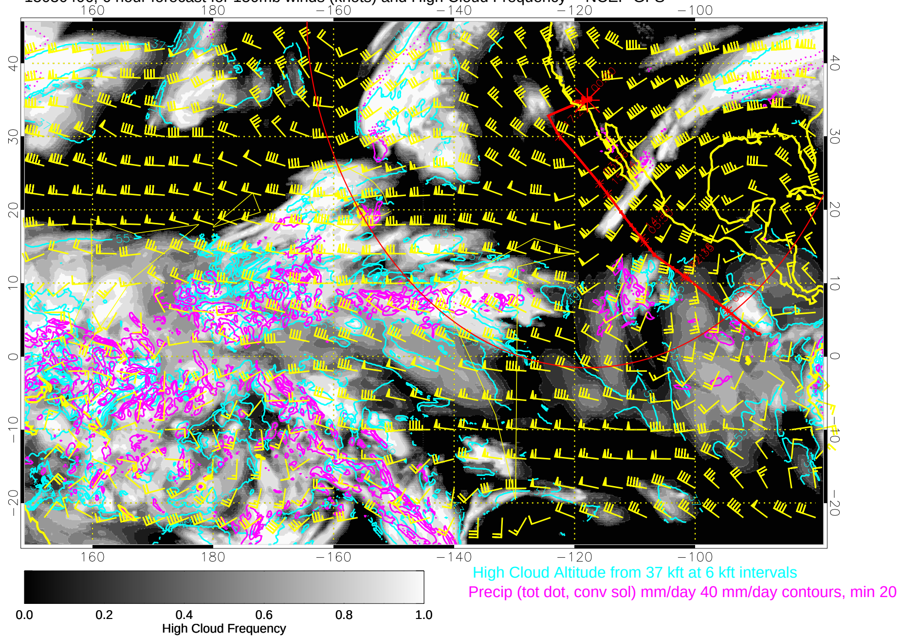
15030406, 6 hour forecast for 150mb winds (knots) and High Cloud Frequency -- NCEP GFS
