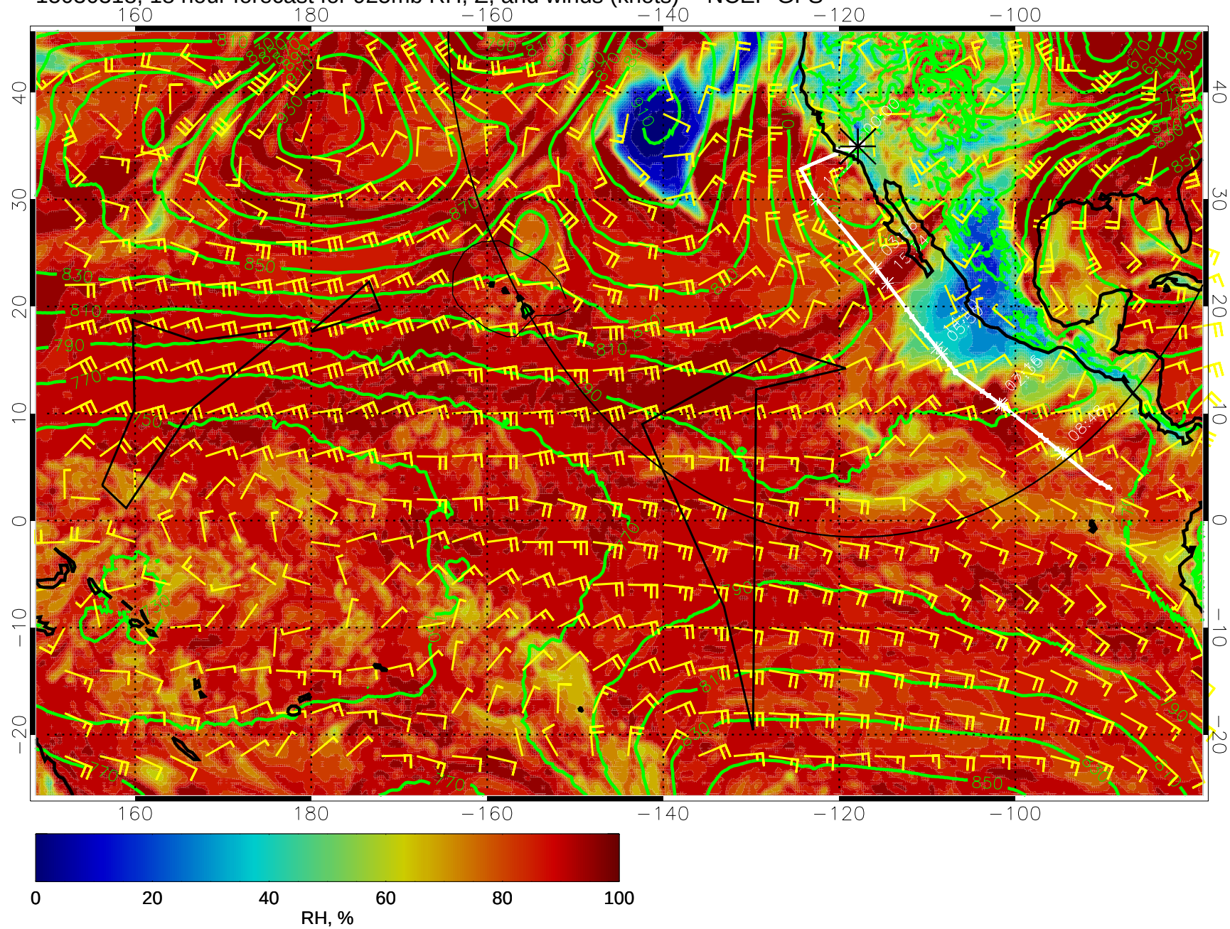
15030318, 18 hour forecast for 925mb RH, Z, and winds (knots) -- NCEP GFS
