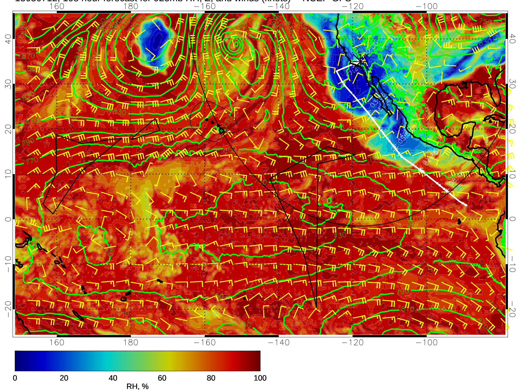
15030712, 108 hour forecast for 925mb RH, Z, and winds (knots) -- NCEP GFS
