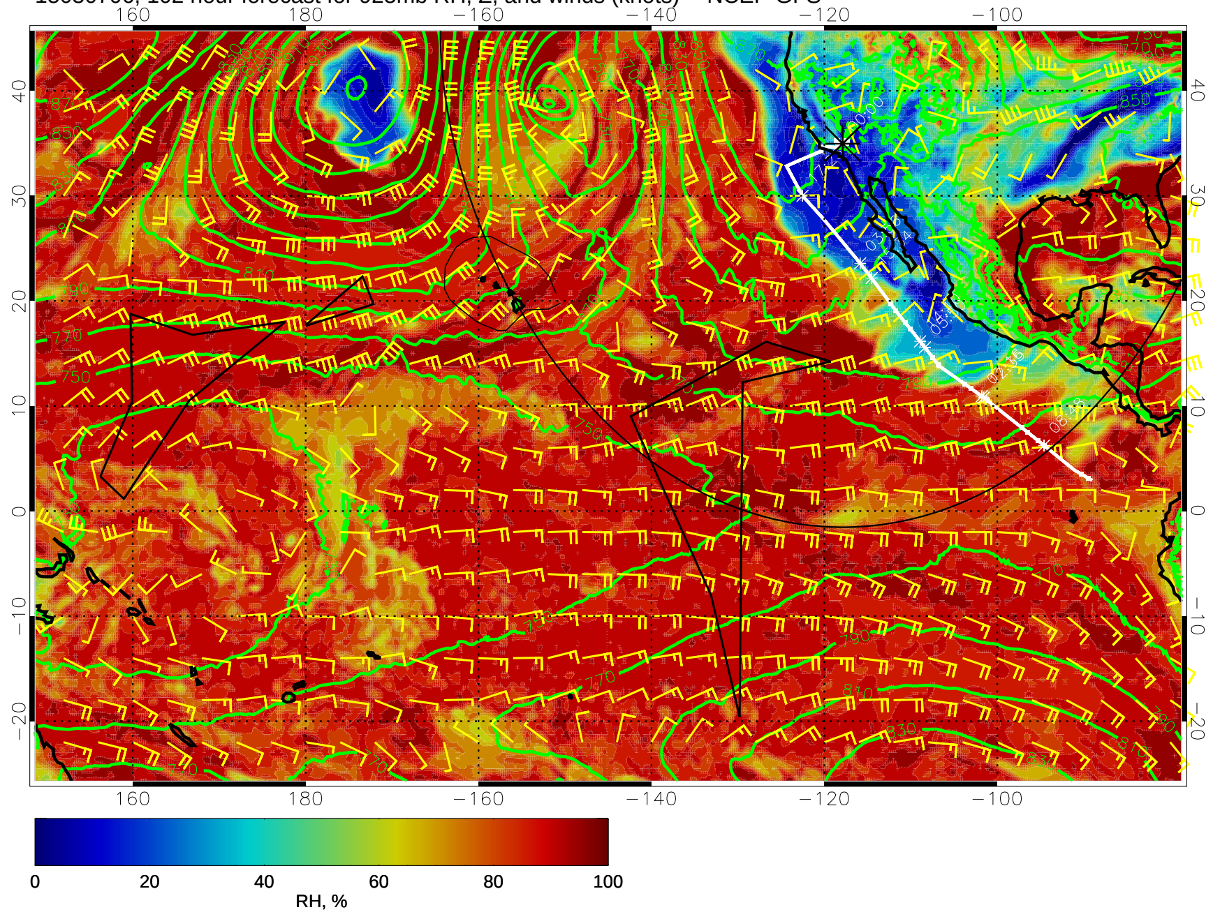
15030706, 102 hour forecast for 925mb RH, Z, and winds (knots) -- NCEP GFS
