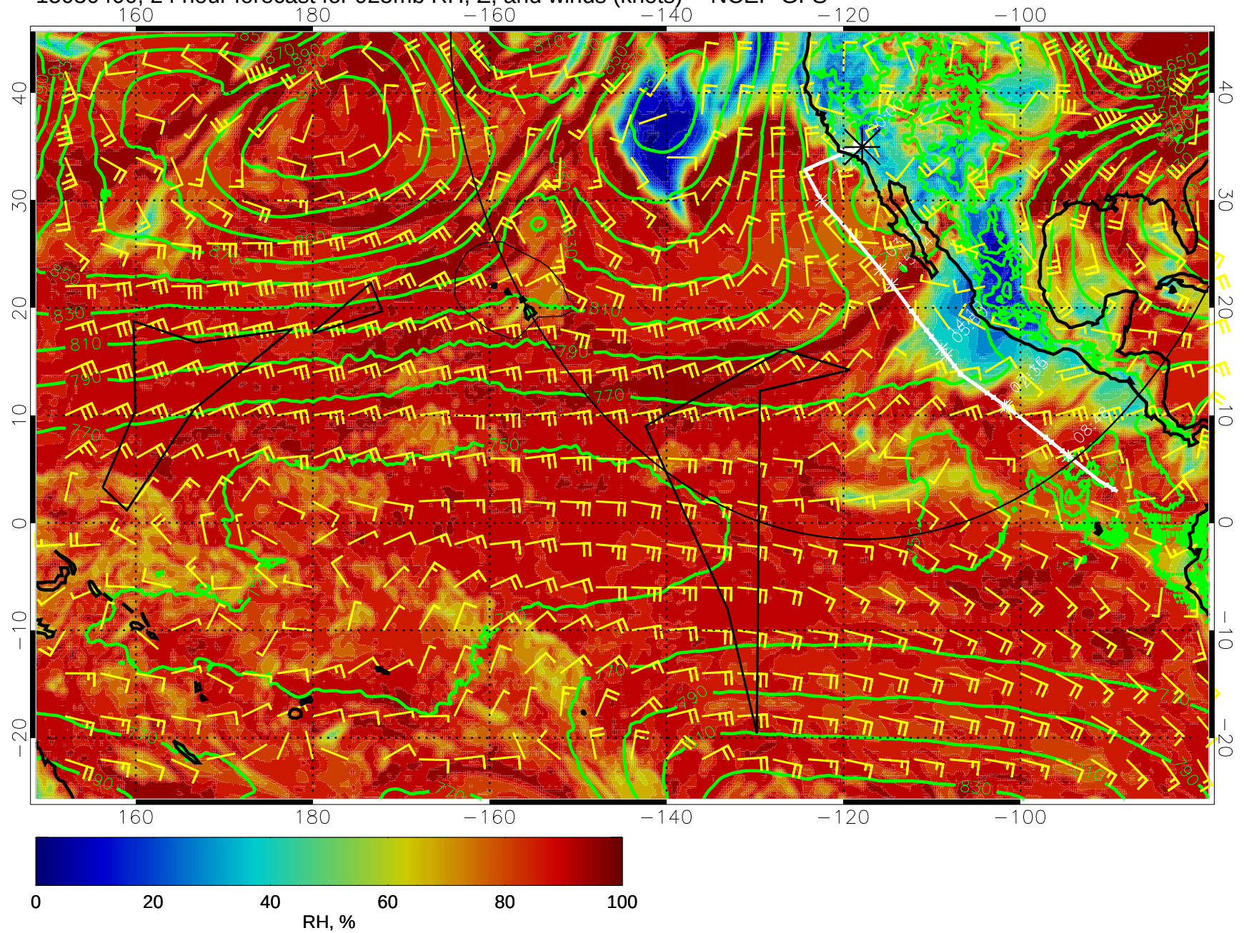
15030400, 24 hour forecast for 925mb RH, Z, and winds (knots) -- NCEP GFS
