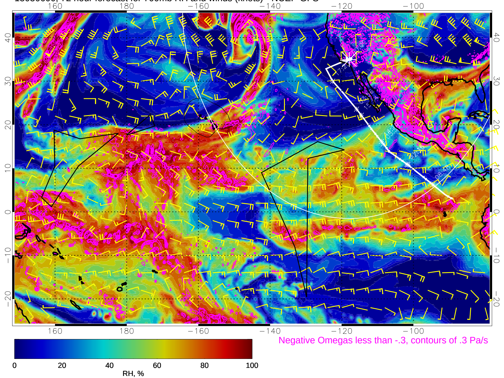
15030600, 72 hour forecast for 700mb RH and winds (knots) - NCEP GFS
