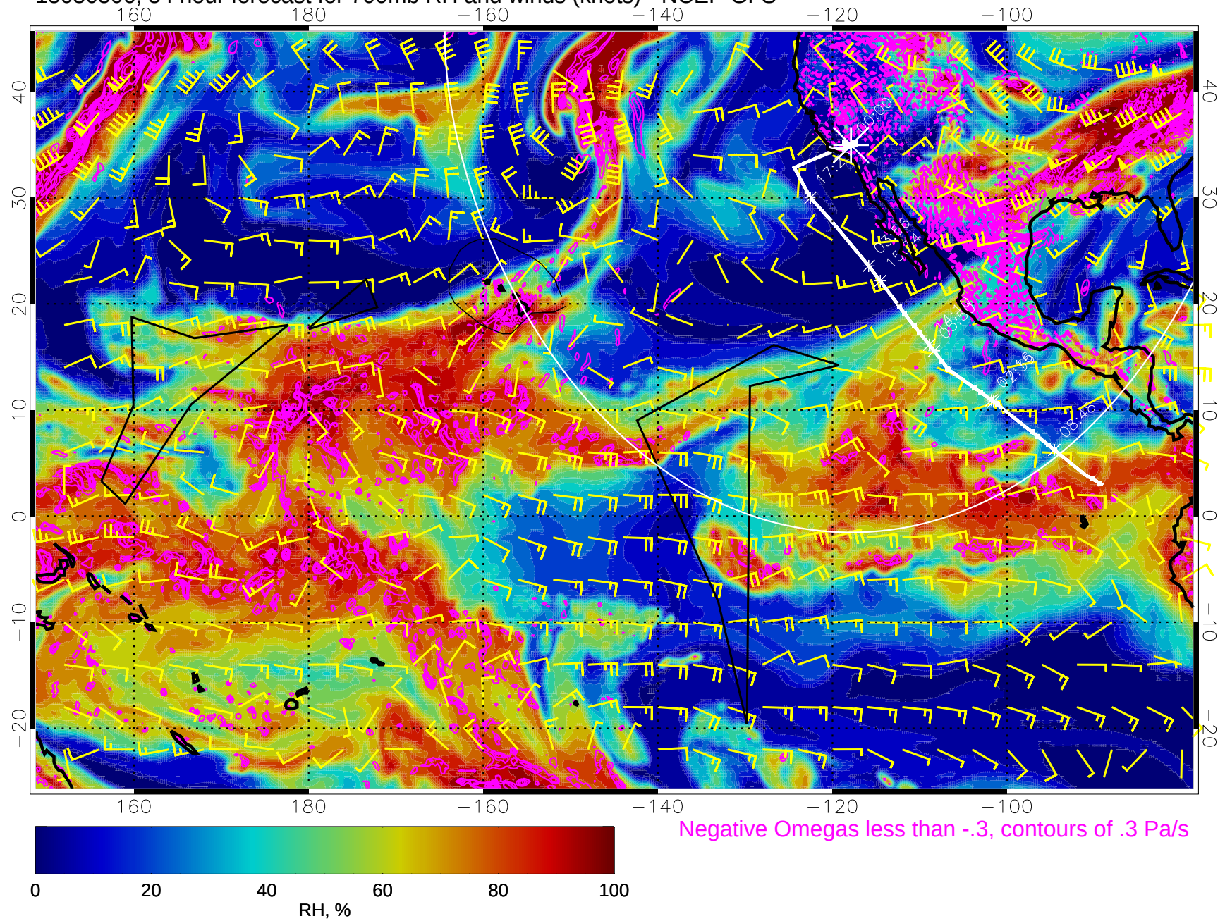
15030506, 54 hour forecast for 700mb RH and winds (knots) - NCEP GFS
