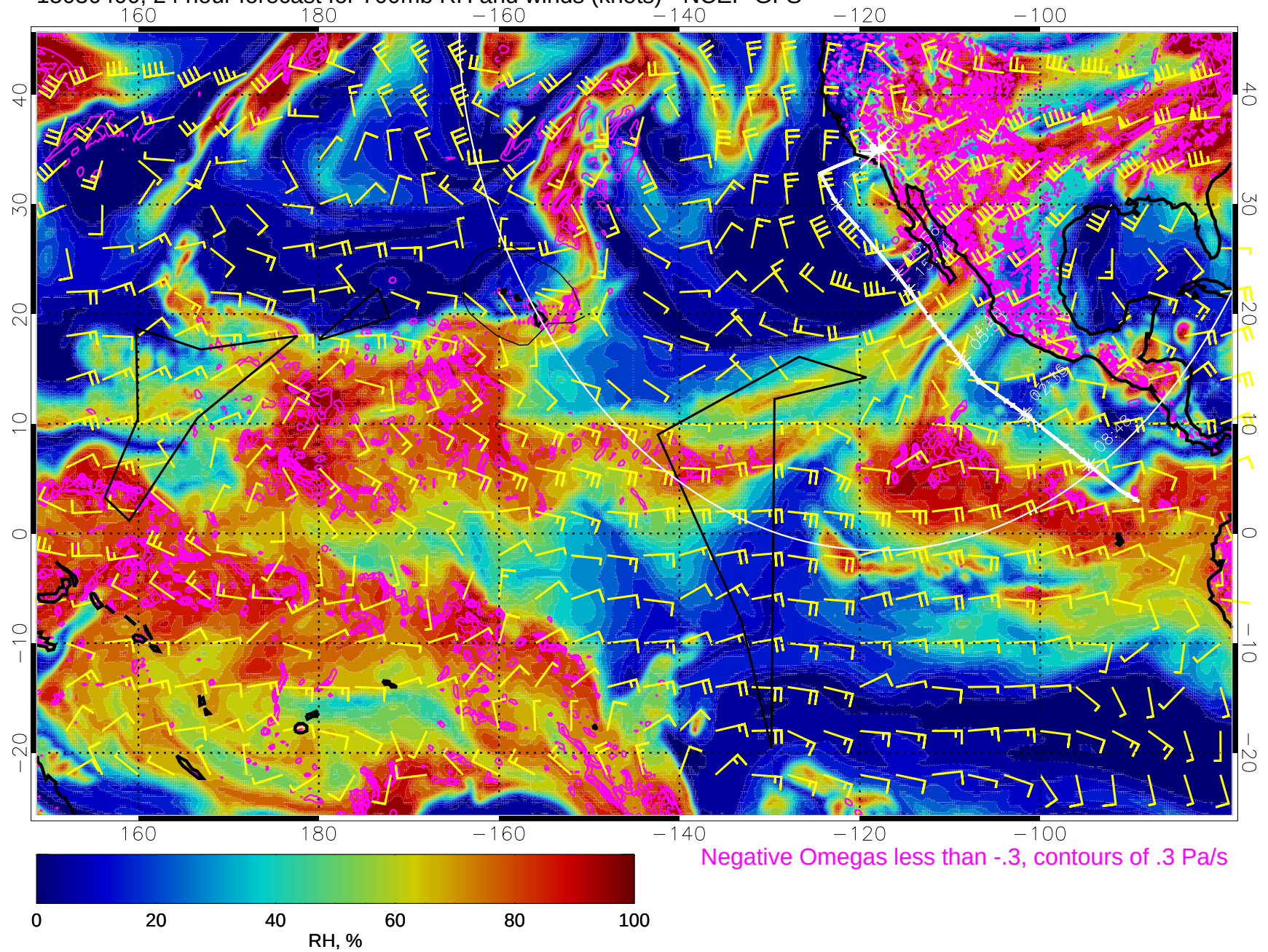
15030400, 24 hour forecast for 700mb RH and winds (knots) - NCEP GFS
