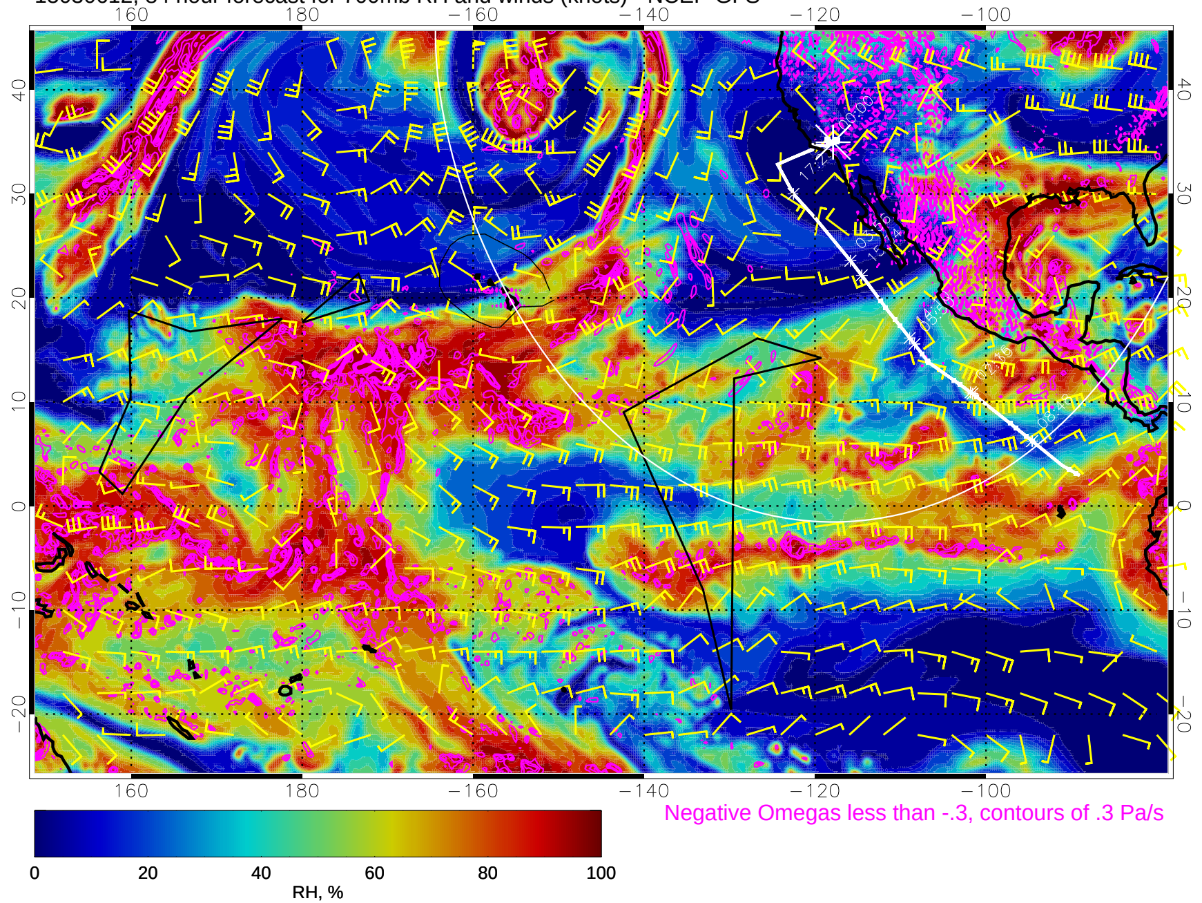
15030612, 84 hour forecast for 700mb RH and winds (knots) - NCEP GFS
