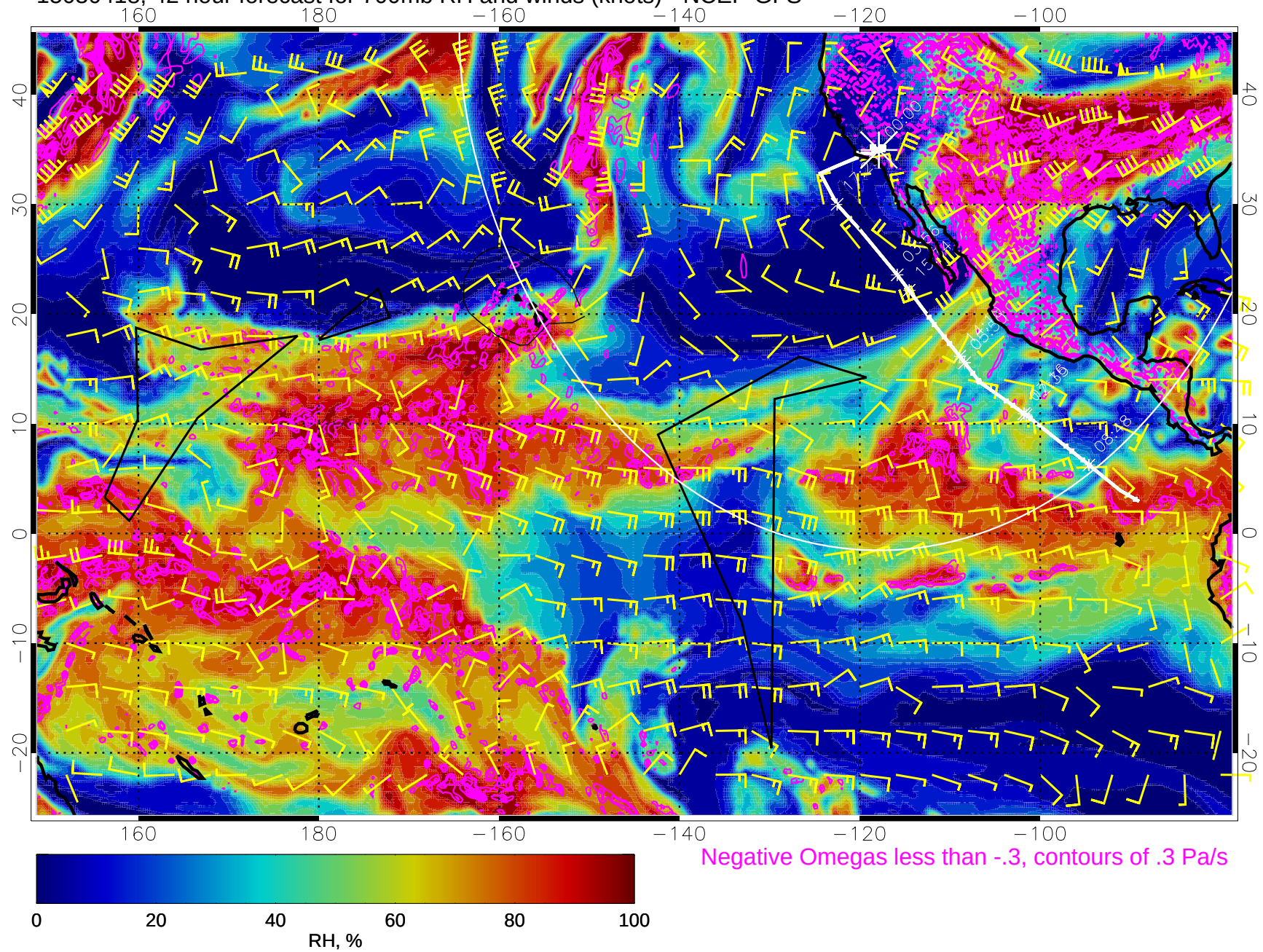
15030418, 42 hour forecast for 700mb RH and winds (knots) - NCEP GFS
