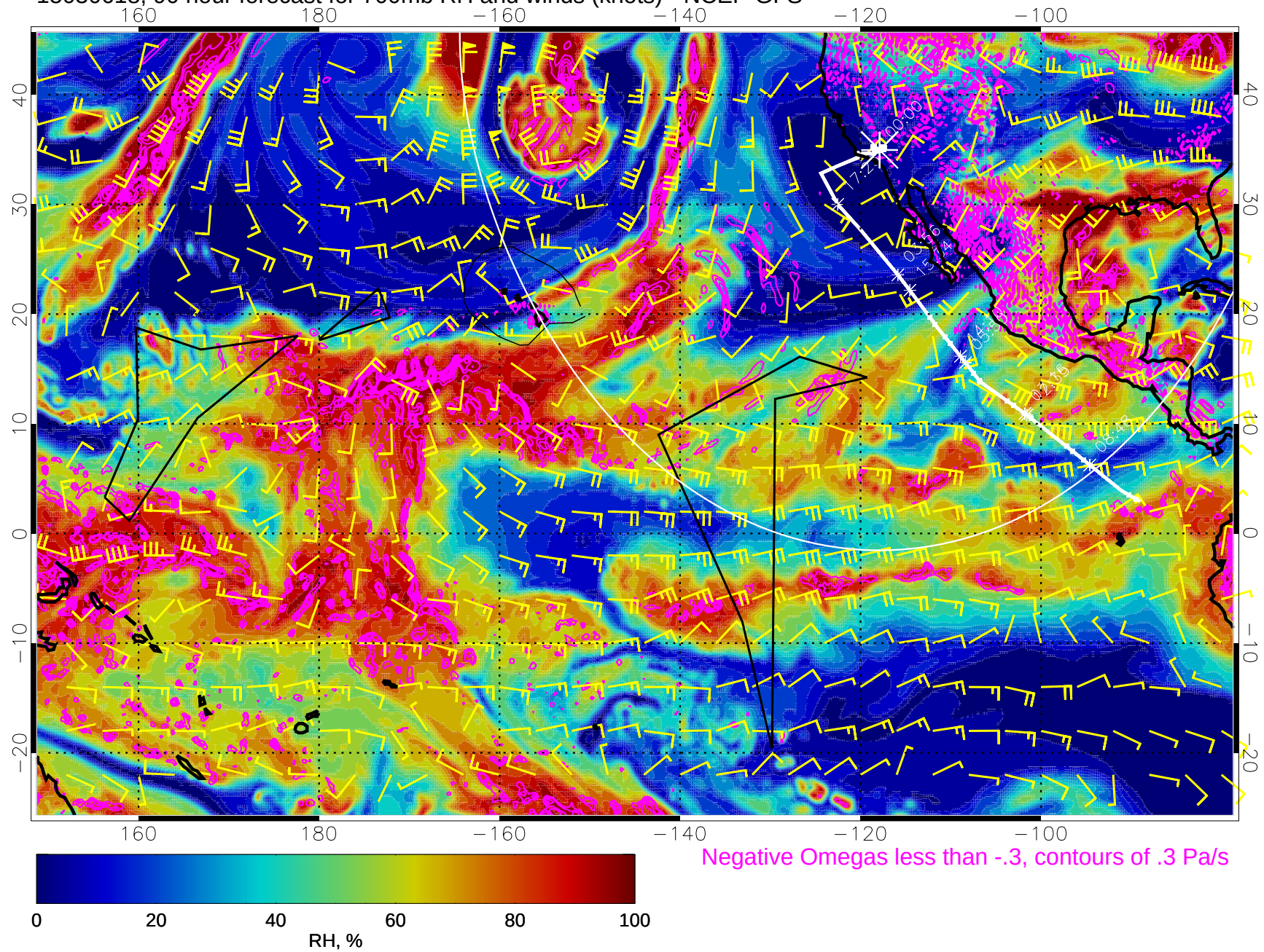
15030618, 90 hour forecast for 700mb RH and winds (knots) - NCEP GFS
