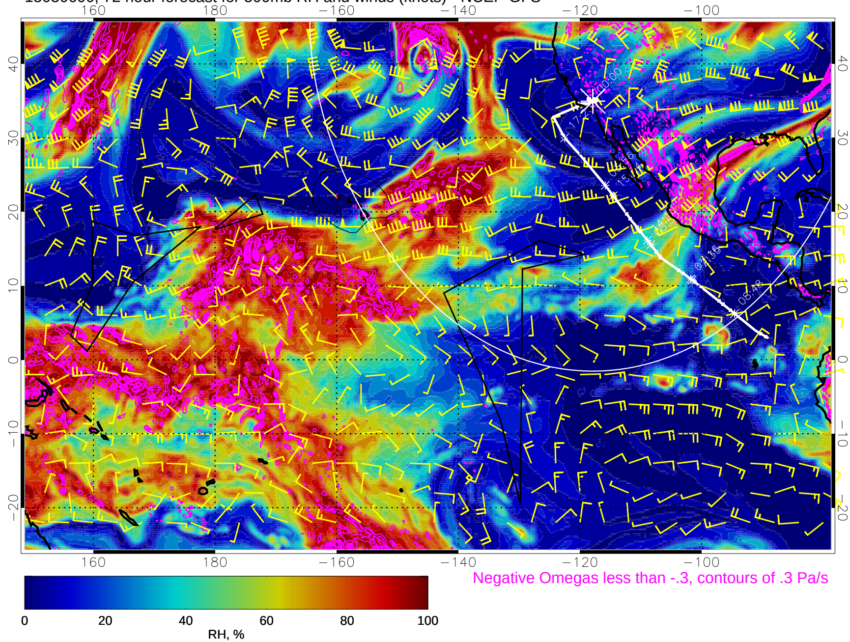
15030600, 72 hour forecast for 500mb RH and winds (knots) - NCEP GFS
