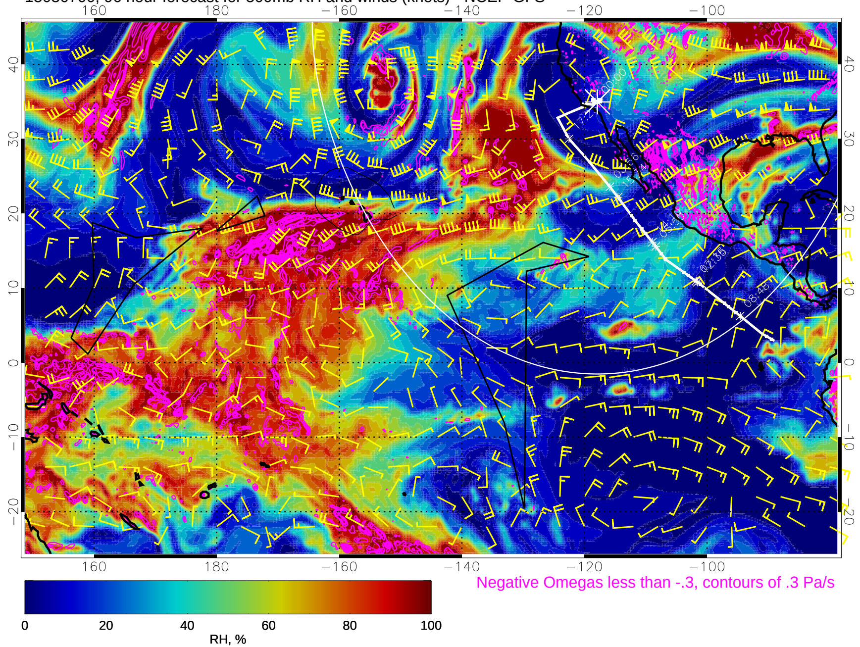
15030700, 96 hour forecast for 500mb RH and winds (knots) - NCEP GFS
