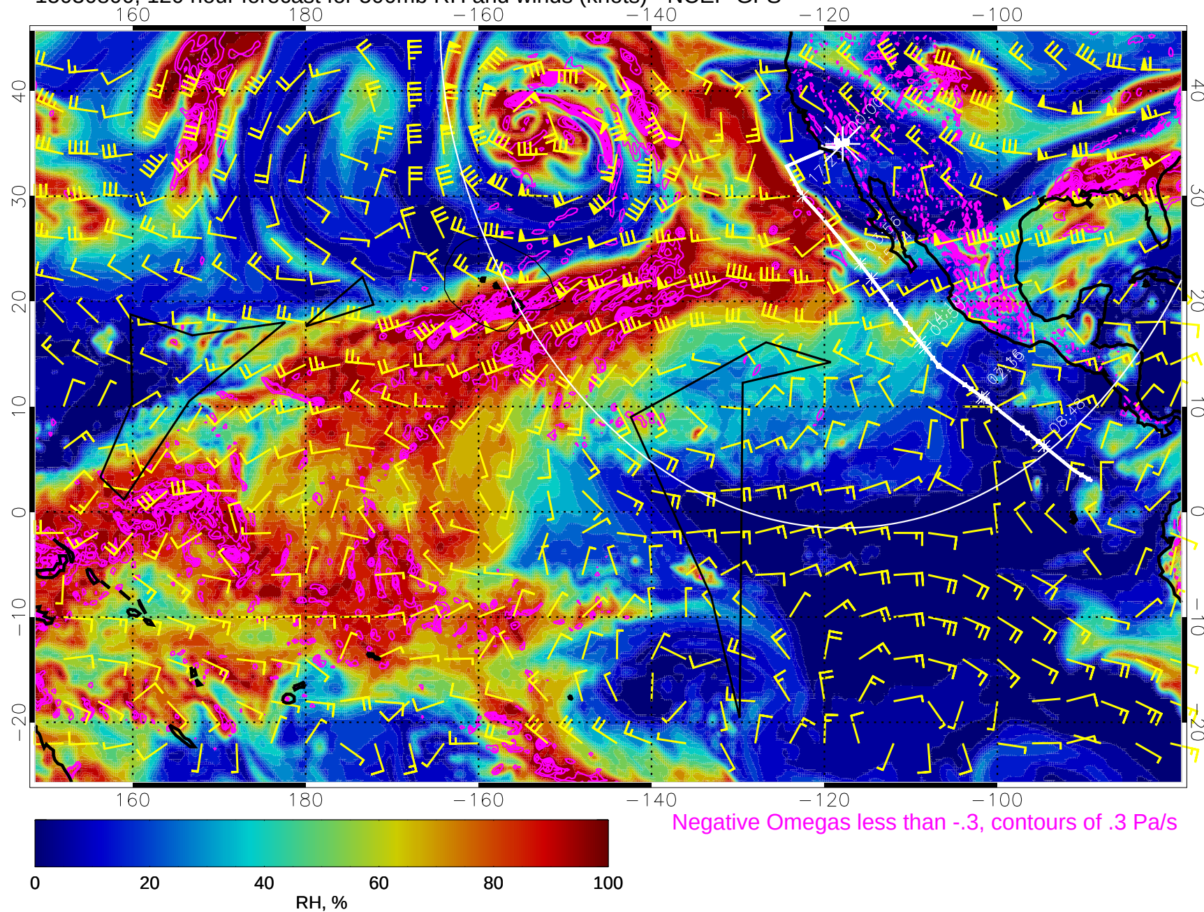
15030800, 120 hour forecast for 500mb RH and winds (knots) - NCEP GFS
