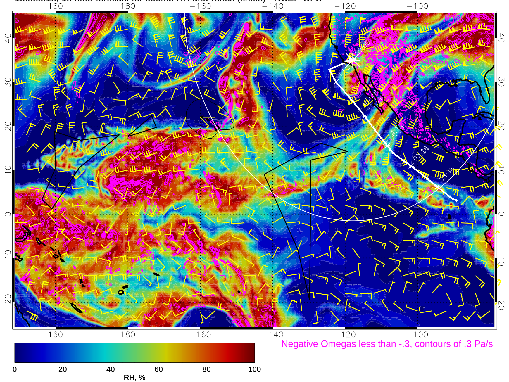
15030318, 18 hour forecast for 500mb RH and winds (knots) - NCEP GFS
