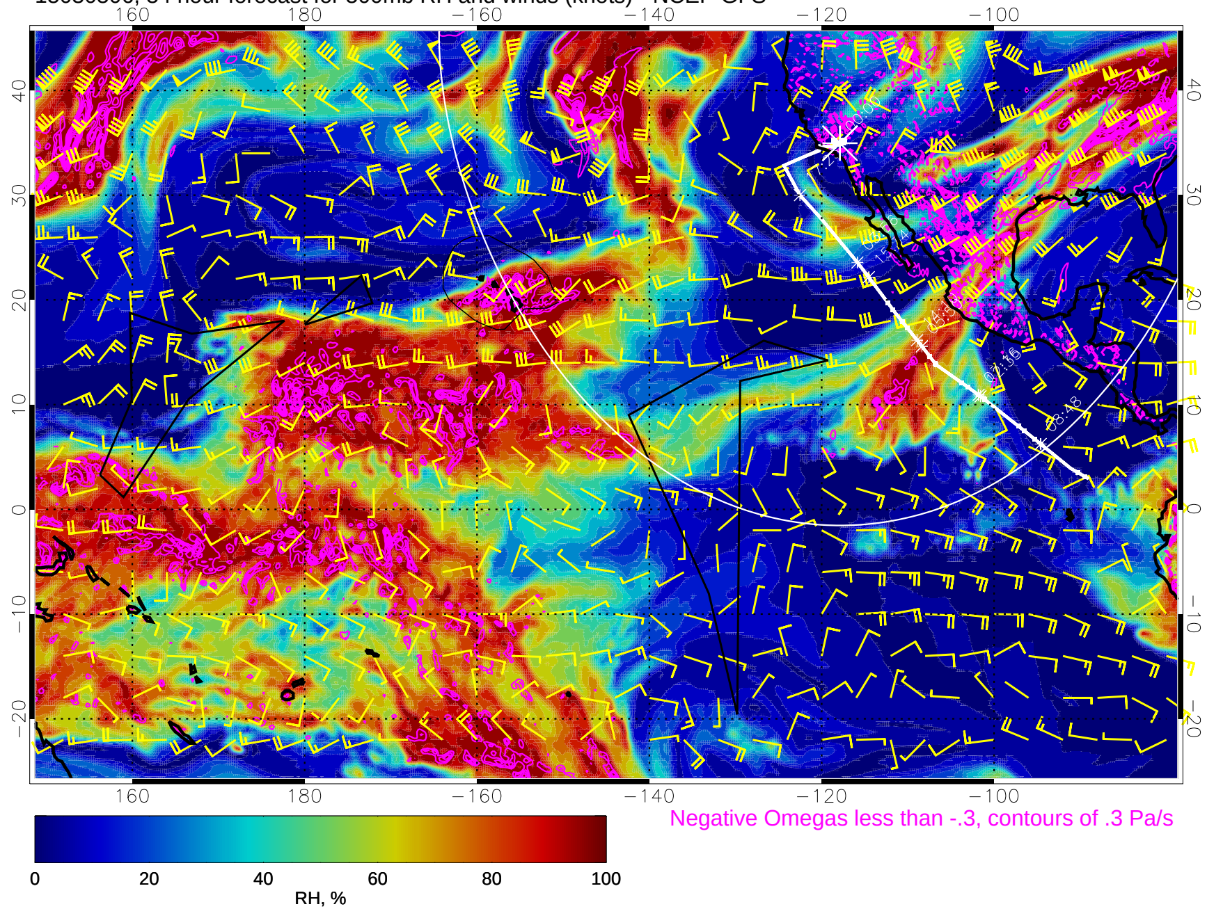
15030506, 54 hour forecast for 500mb RH and winds (knots) - NCEP GFS
