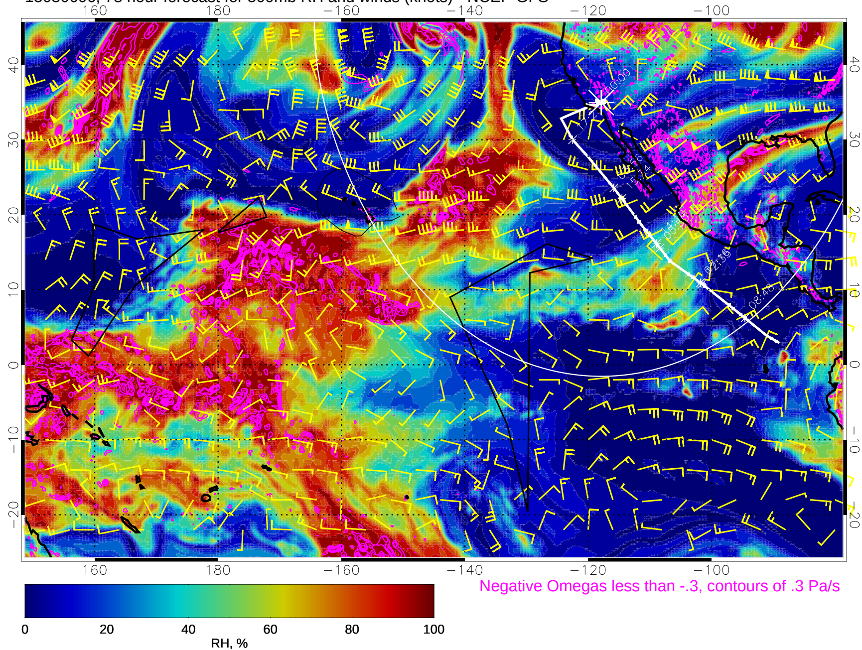
15030606, 78 hour forecast for 500mb RH and winds (knots) - NCEP GFS
