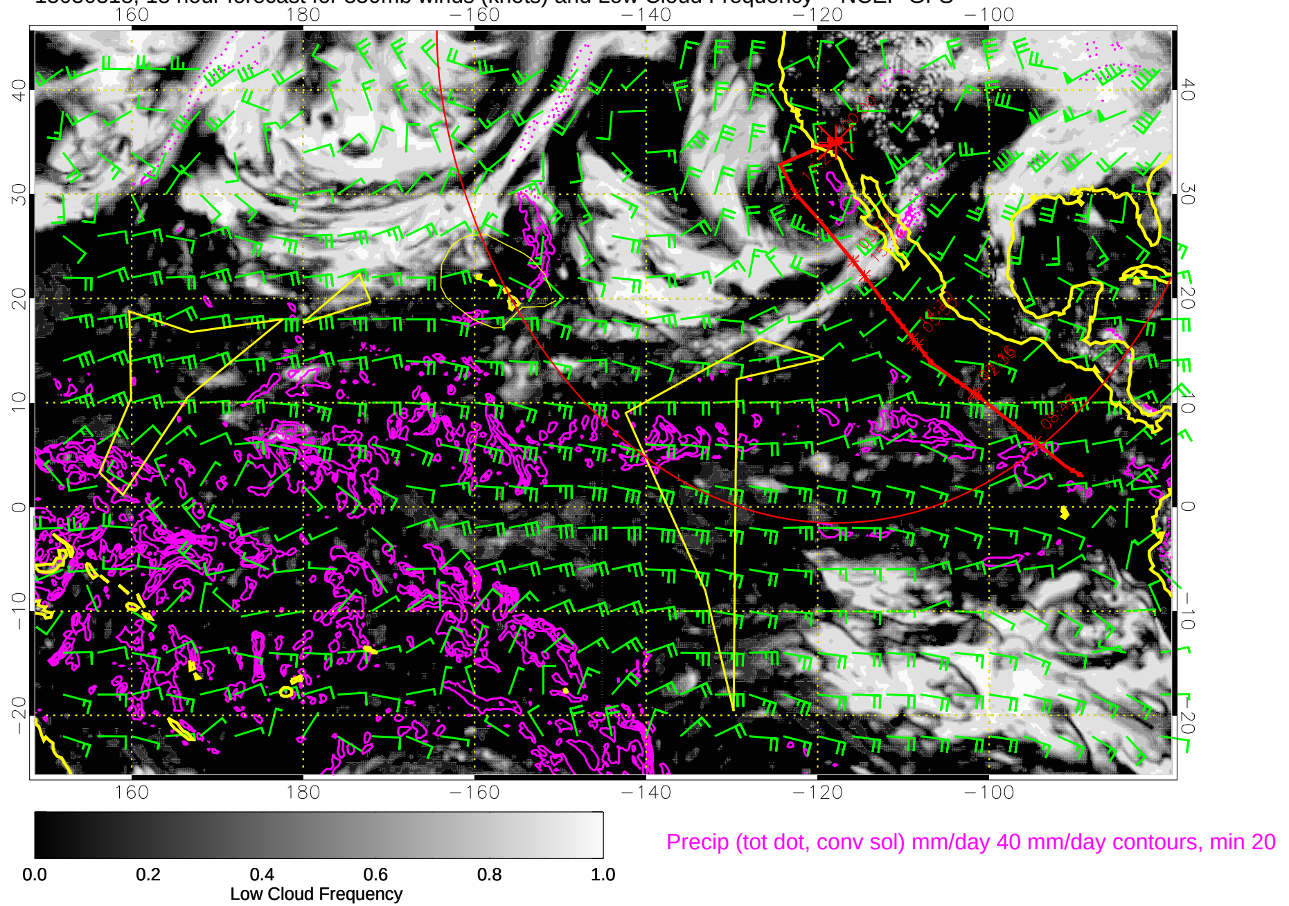
15030318, 18 hour forecast for 850mb winds (knots) and Low Cloud Frequency -- NCEP GFS
